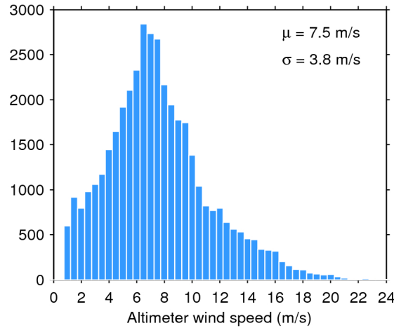
Figure 33. Histogram of flag-valid wind over oceans and lakes for 27/09/2019. The mean ( \mu ) and standard deviation ( \sigma ) are also shown. Note that values larger than 24 m/s are excluded from the histogram for the sake of readability but not from the computation of \mu and \sigma .
