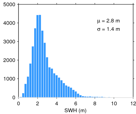
Figure 17. Histogram of flag-valid SWH over oceans and lakes for 27/09/2019. The mean ( \mu ) and standard deviation ( \sigma ) are also shown. Note that values larger than 12 m are excluded from the histogram for the sake of readability but not from the computation of \mu and \sigma .
