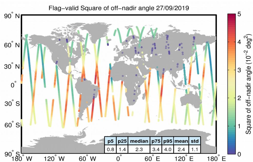
Figure 37. Geographical distribution of flag-valid mispointing data over oceans and lakes for 27/09/2019. The statistical values shown in the table refer to the mispointing in 10^{-2} \text{ deg}^2 and are calculated over all measurements shown in the figure.
