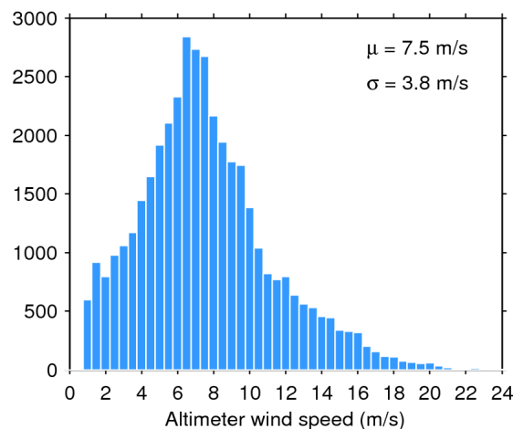
Figure 35. Histogram of science-valid wind over oceans and lakes for 27/09/2019. The mean ( \mu ) and standard deviation ( \sigma ) are also shown. Note that values larger than 24 m/s are excluded from the histogram for the sake of readability but not from the computation of \mu and \sigma .
