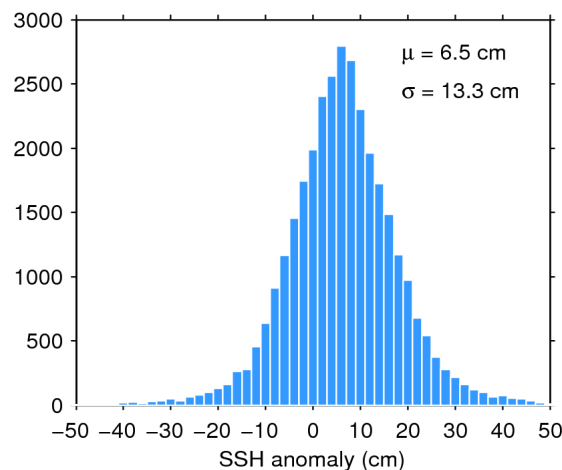
Figure 11. Histogram of science-valid SSH anomaly over oceans and lakes for 27/09/2019. The mean ( \mu ) and standard deviation ( \sigma ) are also shown. Note that values outside [-50 50] cm are excluded from the histogram for the sake of readability but not from the computation of \mu and \sigma .
