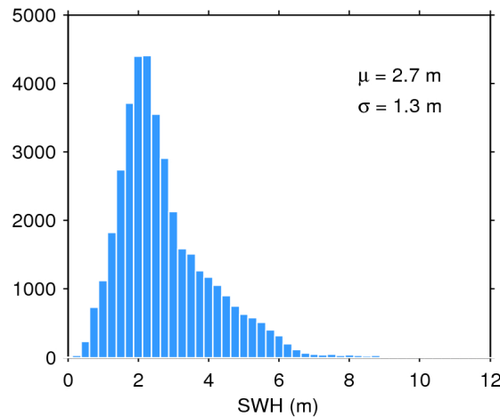
Figure 20. Histogram of science-valid SWH over oceans and lakes for 27/09/2019. The mean ( \mu ) and standard deviation ( \sigma ) are also shown. Note that values larger than 12 m are excluded from the histogram for the sake of readability but not from the computation of \mu and \sigma .
