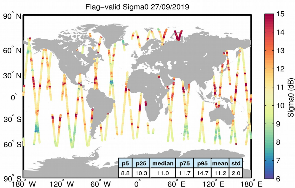
Figure 23. Geographical distribution of flag-valid sigma0 data over oceans and lakes for 27/09/2019. The statistical values shown in the table refer to the sigma0 in dB and are calculated over all measurements shown in the figure.
