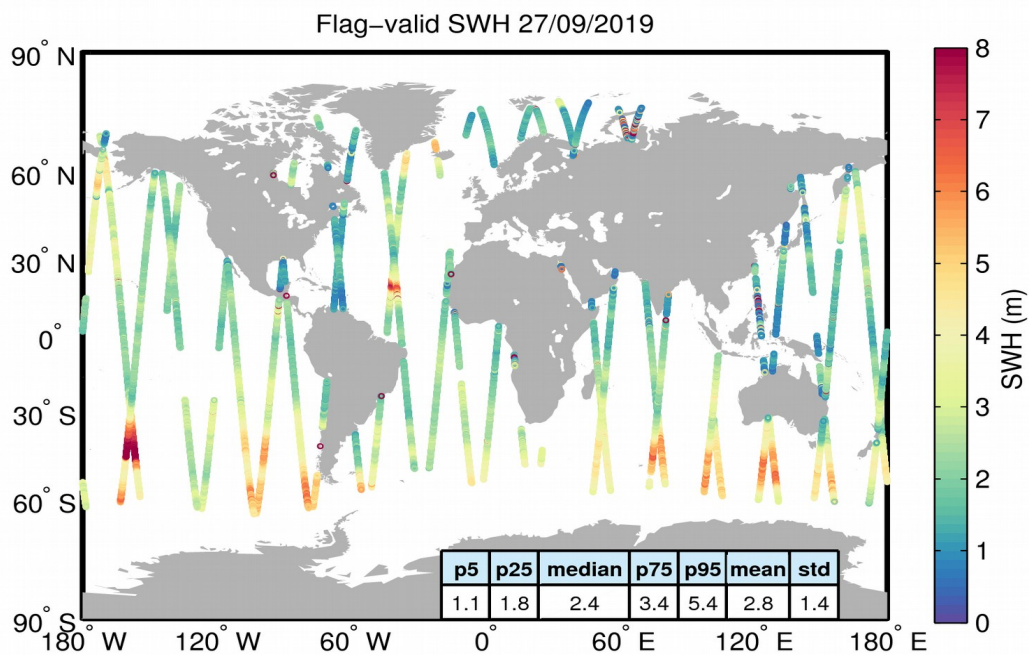
Figure 15. Geographical distribution of flag-valid SWH data over oceans and lakes for 27/09/2019. The statistical values shown in the table refer to the SWH in m and are calculated over all measurements shown in the figure.
