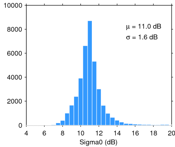
Figure 28. Histogram of science-valid sigma0 over oceans and lakes for 27/09/2019. The mean ( \mu ) and standard deviation ( \sigma ) are also shown. Note that values outside [4 20] dB are excluded from the histogram for the sake of readability but not from the computation of \mu and \sigma .
