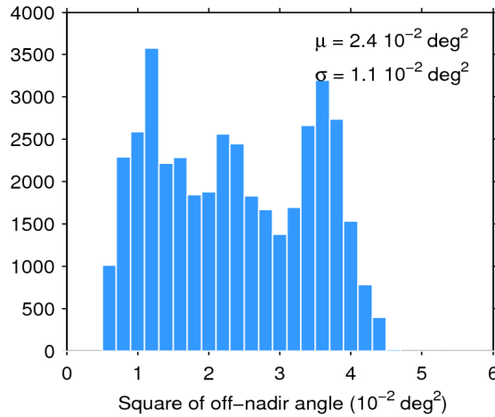
Figure 39. Histogram of flag-valid mispointing over oceans and lakes for 27/09/2019. The mean ( \mu ) and standard deviation ( \sigma ) are also shown. Note that values larger than 6 \cdot 10^{-2} \text{ deg}^2 are excluded from the histogram for the sake of readability but not from the computation of \mu and \sigma .
