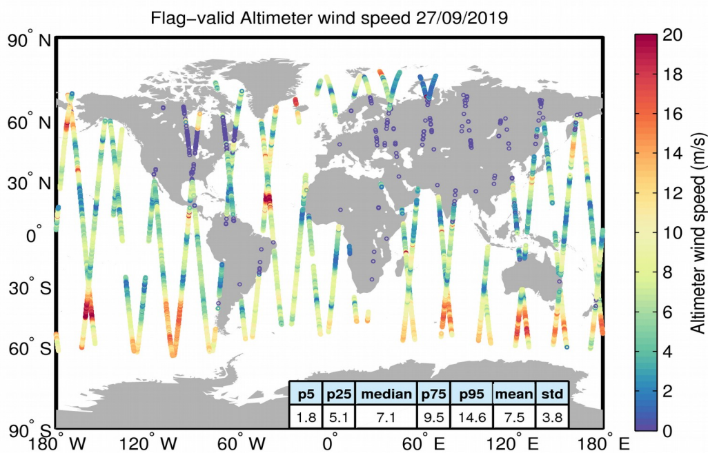
Figure 31. Geographical distribution of flag-valid wind data over oceans and lakes for 27/09/2019. The statistical values shown in the table refer to the wind in m/s and are calculated over all measurements shown in the figure.
