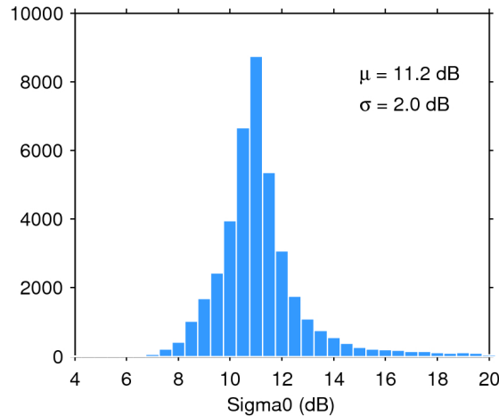
Figure 25. Histogram of flag-valid sigma0 over oceans and lakes for 27/09/2019. The mean ( \mu ) and standard deviation ( \sigma ) are also shown. Note that values outside [4 20] dB are excluded from the histogram for the sake of readability but not from the computation of \mu and \sigma .
