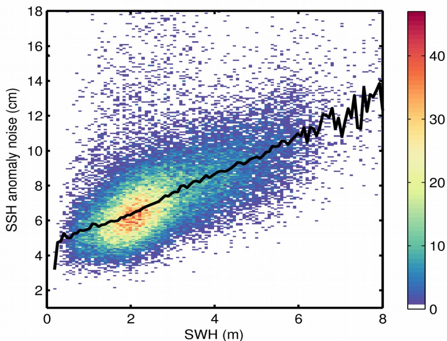
Figure 9. 2D histogram showing flag-valid SSH anomaly noise as a function of SWH for 27/09/2019. The black line denotes the median SSH anomaly noise as a function of SWH.
