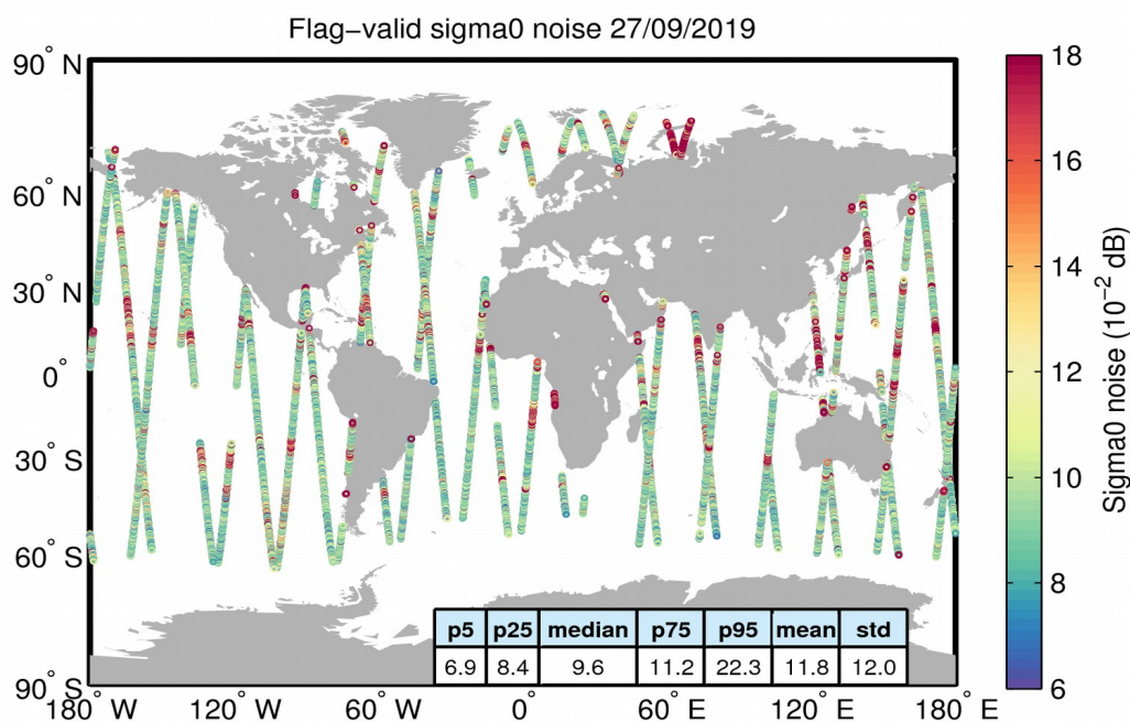
Figure 26. Geographical distribution of flag-valid 20-Hz sigma0 measurement noise over oceans and lakes for 27/09/2019. The statistical values shown in the table refer to the sigma0 noise and are calculated over all measurements shown in the figure.
