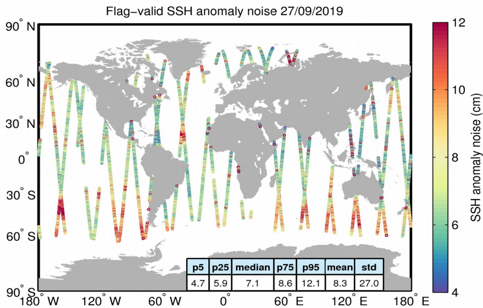
Figure 8. Geographical distribution of flag-valid 20-Hz SSH anomaly measurement noise over oceans and lakes for 27/09/2019. The statistical values shown in the table refer to the SSH anomaly noise and are calculated over all measurements shown in the figure.
