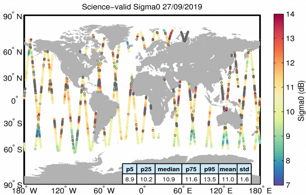
Figure 27. Geographical distribution of science-valid sigma0 data over oceans and lakes for 27/09/2019. The statistical values shown in the table refer to the sigma0 in dB and are calculated over all measurements shown in the figure. Gray circles denote records that have been rejected based on the editing criteria described in Table 4.
