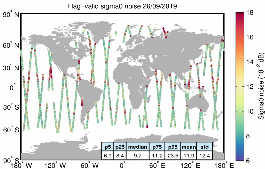
Figure 26. Geographical distribution of flag-valid 20-Hz sigma0 measurement noise over oceans and lakes for 26/09/2019. The statistical values shown in the table refer to the sigma0 noise and are calculated over all measurements shown in the figure.
