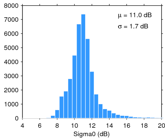
Figure 28. Histogram of science-valid sigma0 over oceans and lakes for 26/09/2019. The mean ( \mu ) and standard deviation ( \sigma ) are also shown. Note that values outside [4 20] dB are excluded from the histogram for the sake of readability but not from the computation of \mu and \sigma .
