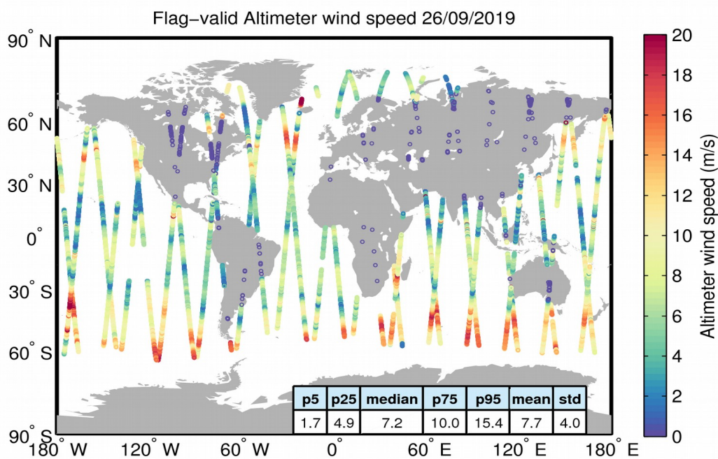
Figure 31. Geographical distribution of flag-valid wind data over oceans and lakes for 26/09/2019. The statistical values shown in the table refer to the wind in m/s and are calculated over all measurements shown in the figure.
