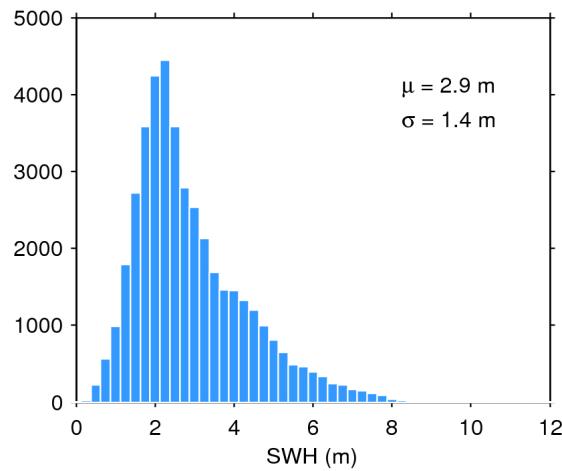
Figure 17. Histogram of flag-valid SWH over oceans and lakes for 26/09/2019. The mean ( \mu ) and standard deviation ( \sigma ) are also shown. Note that values larger than 12 m are excluded from the histogram for the sake of readability but not from the computation of \mu and \sigma .
