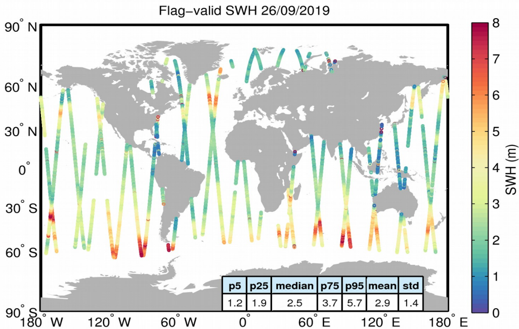
Figure 15. Geographical distribution of flag-valid SWH data over oceans and lakes for 26/09/2019. The statistical values shown in the table refer to the SWH in m and are calculated over all measurements shown in the figure.
