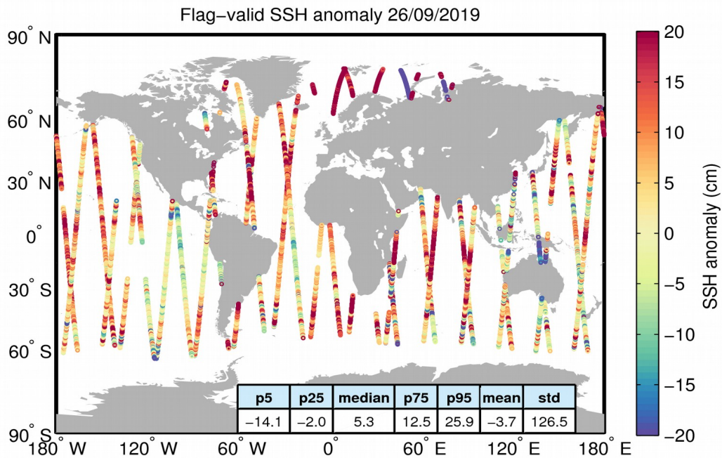
Figure 5. Geographical distribution of flag-valid 1-Hz SSH anomaly data over oceans and lakes for 26/09/2019. The statistical values shown in the table refer to the SSH anomaly in cm and are calculated over all measurements shown in the figure.
