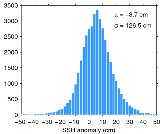
Figure 7. Histogram of flag-valid SSH anomaly over oceans and lakes for 26/09/2019. The mean ( \mu ) and standard deviation ( \sigma ) are also shown. Note that values outside [-50\ 50] cm are excluded from the histogram for the sake of readability but not from the computation of \mu and \sigma .
