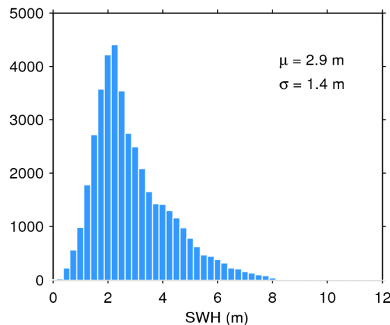
Figure 20. Histogram of science-valid SWH over oceans and lakes for 26/09/2019. The mean ( \mu ) and standard deviation ( \sigma ) are also shown. Note that values larger than 12 m are excluded from the histogram for the sake of readability but not from the computation of \mu and \sigma .
