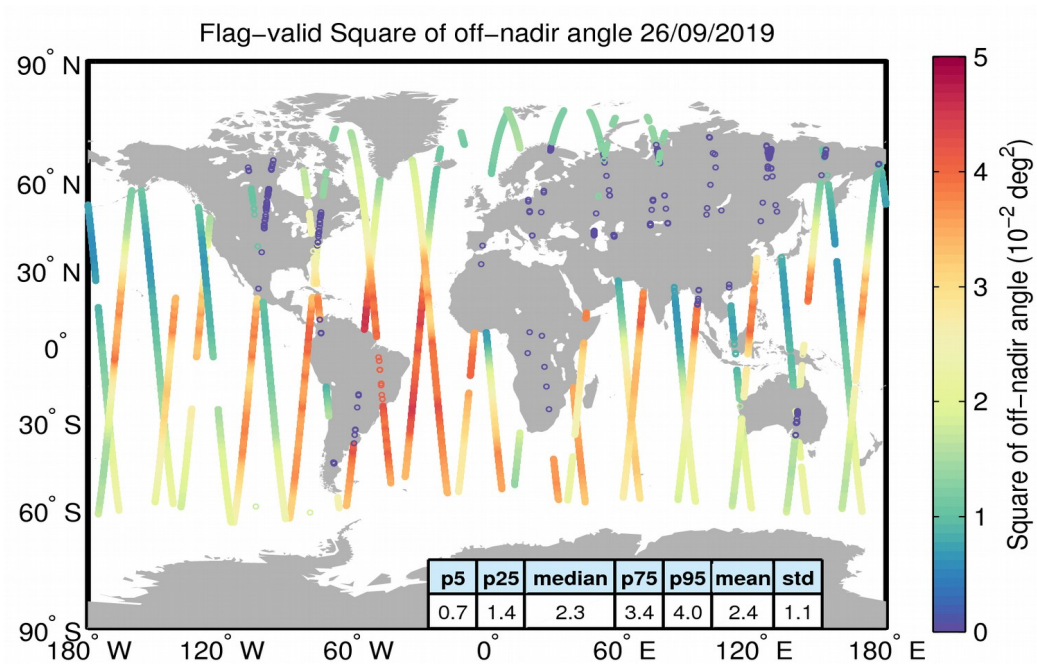
Figure 37. Geographical distribution of flag-valid mispointing data over oceans and lakes for 26/09/2019. The statistical values shown in the table refer to the mispointing in 10^{-2} deg 2 and are calculated over all measurements shown in the figure.
