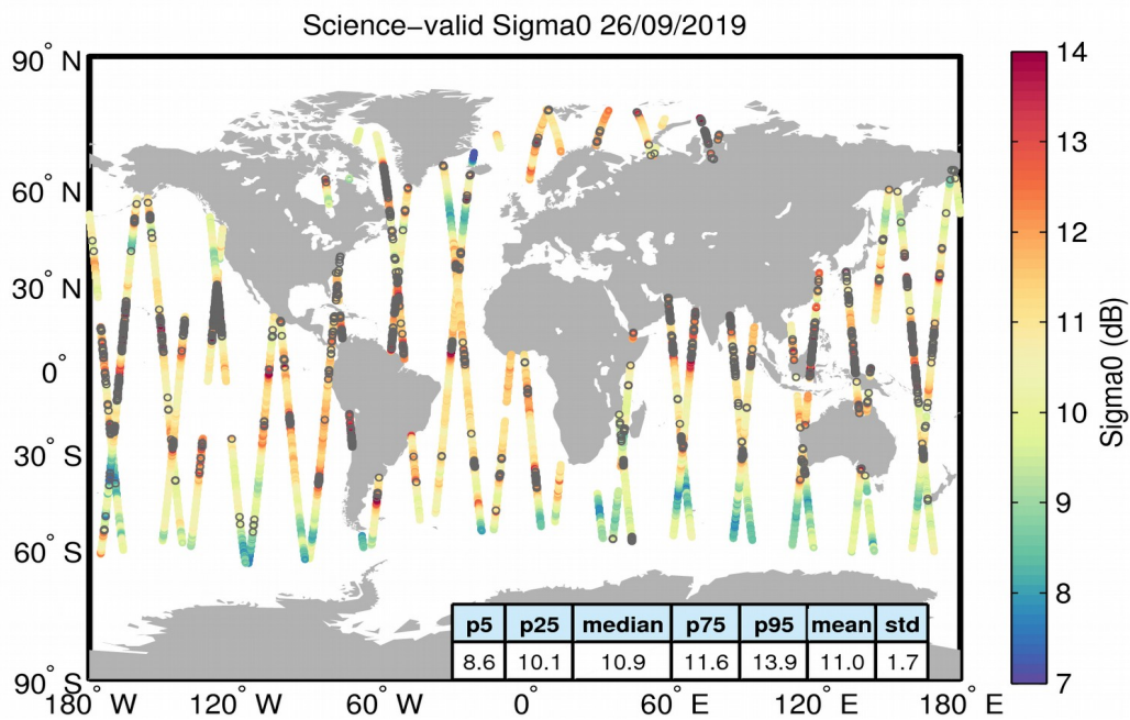
Figure 27. Geographical distribution of science-valid sigma0 data over oceans and lakes for 26/09/2019. The statistical values shown in the table refer to the sigma0 in dB and are calculated over all measurements shown in the figure. Gray circles denote records that have been rejected based on the editing criteria described in Table 4.
