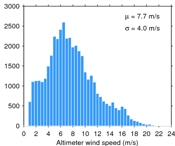
Figure 35. Histogram of science-valid wind over oceans and lakes for 26/09/2019. The mean ( \mu ) and standard deviation ( \sigma ) are also shown. Note that values larger than 24 m/s are excluded from the histogram for the sake of readability but not from the computation of \mu and \sigma .
