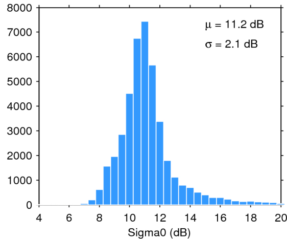
Figure 25. Histogram of flag-valid sigma0 over oceans and lakes for 26/09/2019. The mean ( \mu ) and standard deviation ( \sigma ) are also shown. Note that values outside [4 20] dB are excluded from the histogram for the sake of readability but not from the computation of \mu and \sigma .
