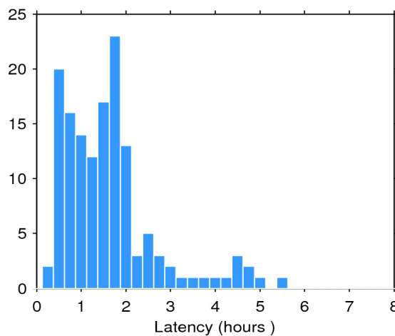
Figure 2. Histogram of the data latency for 26/09/2019. The y-axis denotes the number of files that are made available with a delay of x-hours with respect to the mean time of the records stored in the file.
