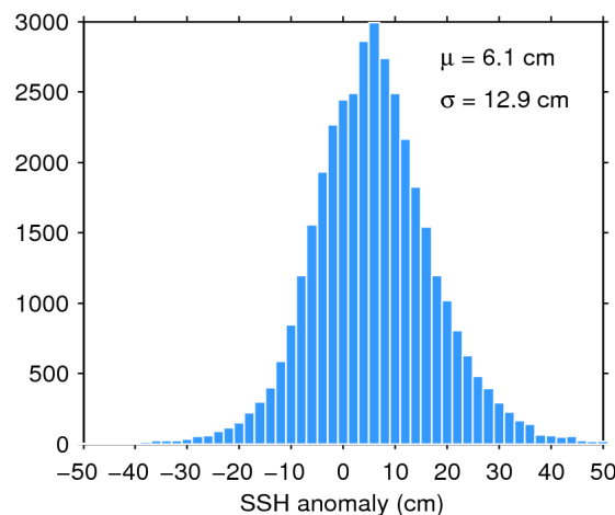
Figure 11. Histogram of science-valid SSH anomaly over oceans and lakes for 26/09/2019. The mean ( \mu ) and standard deviation ( \sigma ) are also shown. Note that values outside [-50 50] cm are excluded from the histogram for the sake of readability but not from the computation of \mu and \sigma .
