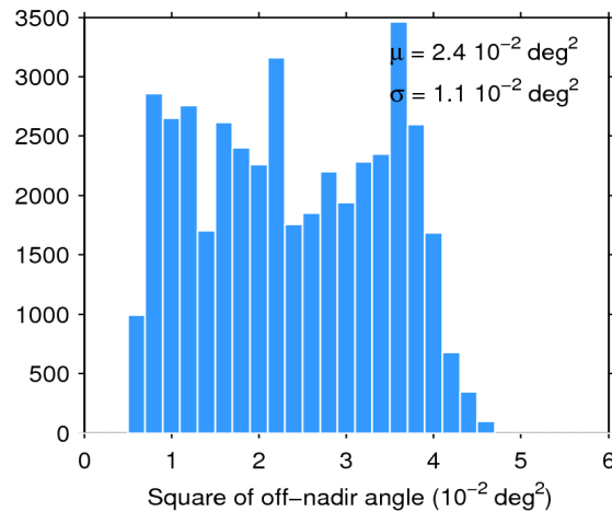
Figure 39. Histogram of flag-valid mispointing over oceans and lakes for 26/09/2019. The mean ( \mu ) and standard deviation ( \sigma ) are also shown. Note that values larger than 6 \cdot 10^{-2} \text{ deg}^2 are excluded from the histogram for the sake of readability but not from the computation of \mu and \sigma .
