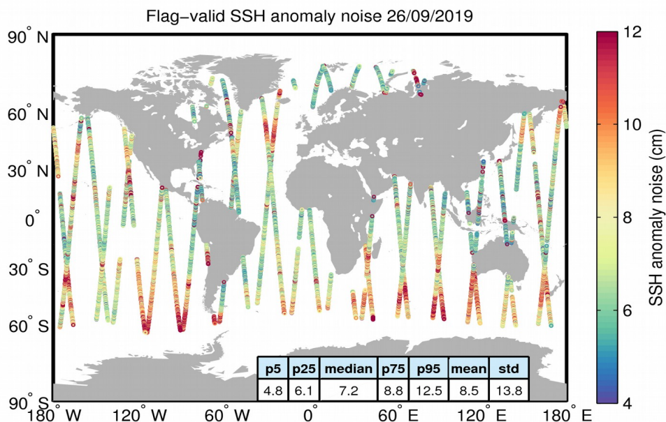
Figure 8. Geographical distribution of flag-valid 20-Hz SSH anomaly measurement noise over oceans and lakes for 26/09/2019. The statistical values shown in the table refer to the SSH anomaly noise and are calculated over all measurements shown in the figure.
