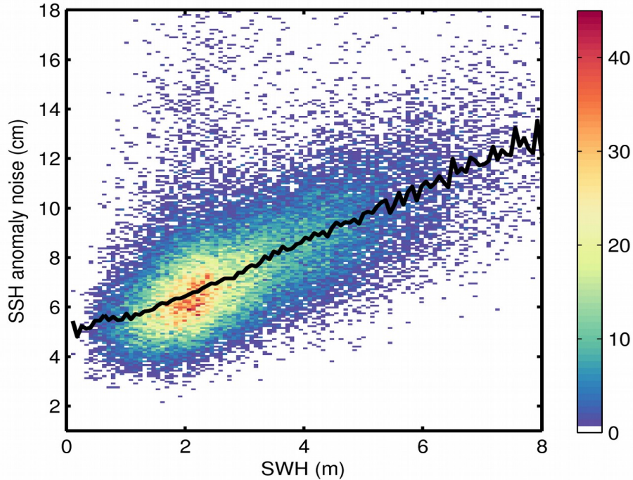
Figure 9. 2D histogram showing flag-valid SSH anomaly noise as a function of SWH for 26/09/2019. The black line denotes the median SSH anomaly noise as a function of SWH.
