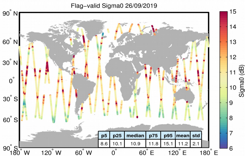
Figure 23. Geographical distribution of flag-valid sigma0 data over oceans and lakes for 26/09/2019. The statistical values shown in the table refer to the sigma0 in dB and are calculated over all measurements shown in the figure.
