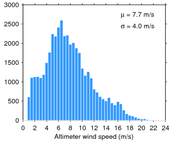
Figure 33. Histogram of flag-valid wind over oceans and lakes for 26/09/2019. The mean ( \mu ) and standard deviation ( \sigma ) are also shown. Note that values larger than 24 m/s are excluded from the histogram for the sake of readability but not from the computation of \mu and \sigma .
