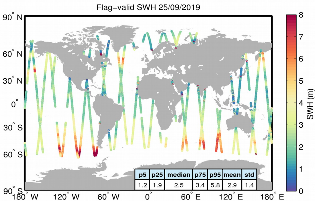
Figure 15. Geographical distribution of flag-valid SWH data over oceans and lakes for 25/09/2019. The statistical values shown in the table refer to the SWH in m and are calculated over all measurements shown in the figure.
