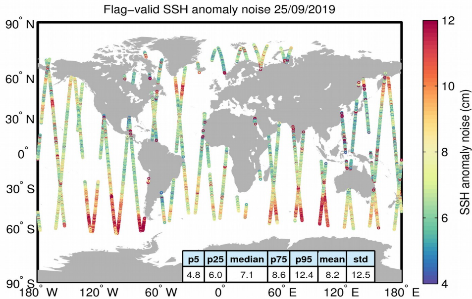
Figure 8. Geographical distribution of flag-valid 20-Hz SSH anomaly measurement noise over oceans and lakes for 25/09/2019. The statistical values shown in the table refer to the SSH anomaly noise and are calculated over all measurements shown in the figure.
