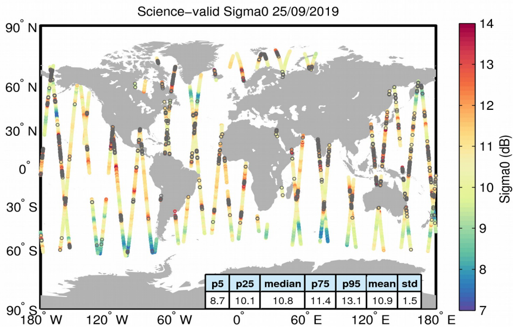
Figure 27. Geographical distribution of science-valid sigma0 data over oceans and lakes for 25/09/2019. The statistical values shown in the table refer to the sigma0 in dB and are calculated over all measurements shown in the figure. Gray circles denote records that have been rejected based on the editing criteria described in Table 4.
