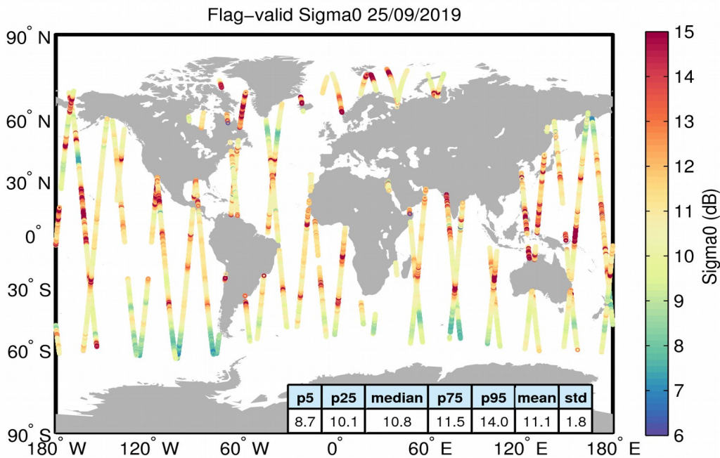
Figure 23. Geographical distribution of flag-valid sigma0 data over oceans and lakes for 25/09/2019. The statistical values shown in the table refer to the sigma0 in dB and are calculated over all measurements shown in the figure.
