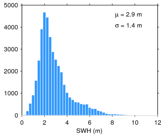
Figure 17. Histogram of flag-valid SWH over oceans and lakes for 25/09/2019. The mean ( \mu ) and standard deviation ( \sigma ) are also shown. Note that values larger than 12 m are excluded from the histogram for the sake of readability but not from the computation of \mu and \sigma .
