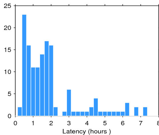
Figure 2. Histogram of the data latency for 25/09/2019. The y-axis denotes the number of files that are made available with a delay of x-hours with respect to the mean time of the records stored in the file.
