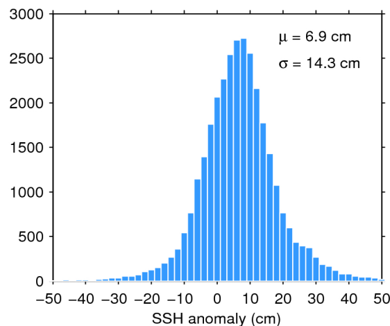
Figure 11. Histogram of science-valid SSH anomaly over oceans and lakes for 25/09/2019. The mean ( \mu ) and standard deviation ( \sigma ) are also shown. Note that values outside [-50 50] cm are excluded from the histogram for the sake of readability but not from the computation of \mu and \sigma .
