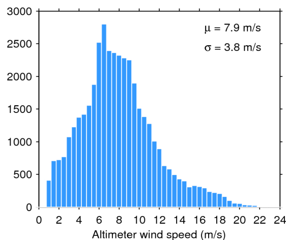
Figure 35. Histogram of science-valid wind over oceans and lakes for 25/09/2019. The mean ( \mu ) and standard deviation ( \sigma ) are also shown. Note that values larger than 24 m/s are excluded from the histogram for the sake of readability but not from the computation of \mu and \sigma .
