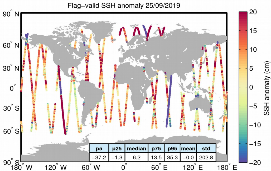
Figure 5. Geographical distribution of flag-valid 1-Hz SSH anomaly data over oceans and lakes for 25/09/2019. The statistical values shown in the table refer to the SSH anomaly in cm and are calculated over all measurements shown in the figure.
