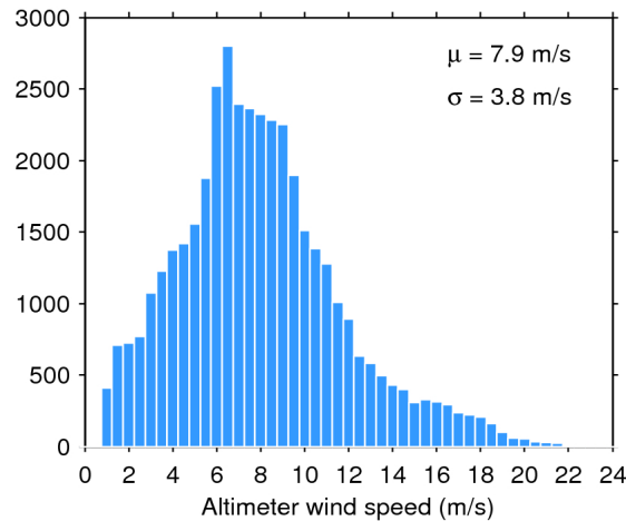
Figure 33. Histogram of flag-valid wind over oceans and lakes for 25/09/2019. The mean ( \mu ) and standard deviation ( \sigma ) are also shown. Note that values larger than 24 m/s are excluded from the histogram for the sake of readability but not from the computation of \mu and \sigma .
