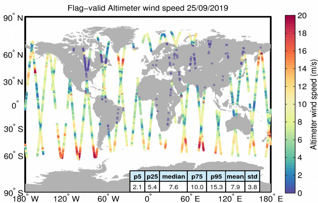
Figure 31. Geographical distribution of flag-valid wind data over oceans and lakes for 25/09/2019. The statistical values shown in the table refer to the wind in m/s and are calculated over all measurements shown in the figure.
