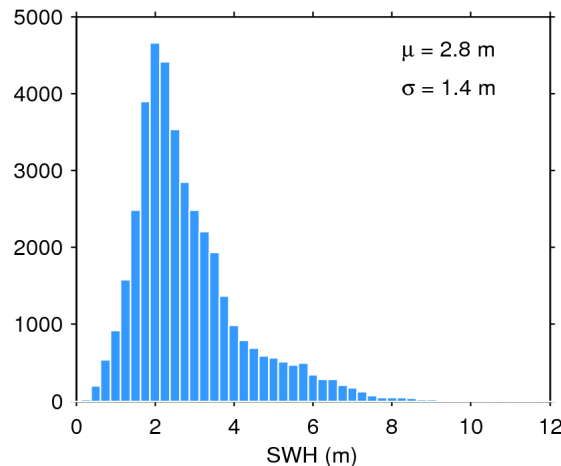
Figure 20. Histogram of science-valid SWH over oceans and lakes for 25/09/2019. The mean ( \mu ) and standard deviation ( \sigma ) are also shown. Note that values larger than 12 m are excluded from the histogram for the sake of readability but not from the computation of \mu and \sigma .
