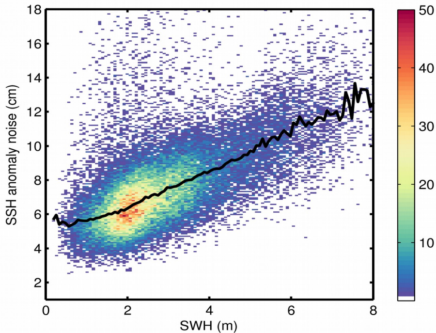
Figure 9. 2D histogram showing flag-valid SSH anomaly noise as a function of SWH for 25/09/2019. The black line denotes the median SSH anomaly noise as a function of SWH.
