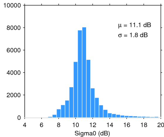
Figure 25. Histogram of flag-valid sigma0 over oceans and lakes for 25/09/2019. The mean ( \mu ) and standard deviation ( \sigma ) are also shown. Note that values outside [4 20] dB are excluded from the histogram for the sake of readability but not from the computation of \mu and \sigma .
