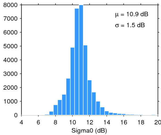
Figure 28. Histogram of science-valid sigma0 over oceans and lakes for 25/09/2019. The mean ( \mu ) and standard deviation ( \sigma ) are also shown. Note that values outside [4 20] dB are excluded from the histogram for the sake of readability but not from the computation of \mu and \sigma .
