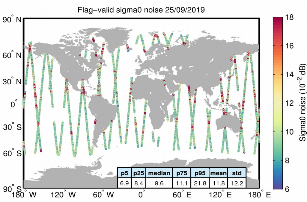
Figure 26. Geographical distribution of flag-valid 20-Hz sigma0 measurement noise over oceans and lakes for 25/09/2019. The statistical values shown in the table refer to the sigma0 noise and are calculated over all measurements shown in the figure.
