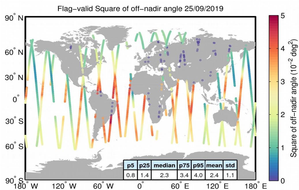
Figure 37. Geographical distribution of flag-valid mispointing data over oceans and lakes for 25/09/2019. The statistical values shown in the table refer to the mispointing in 10^{-2} \text{ deg}^2 and are calculated over all measurements shown in the figure.
