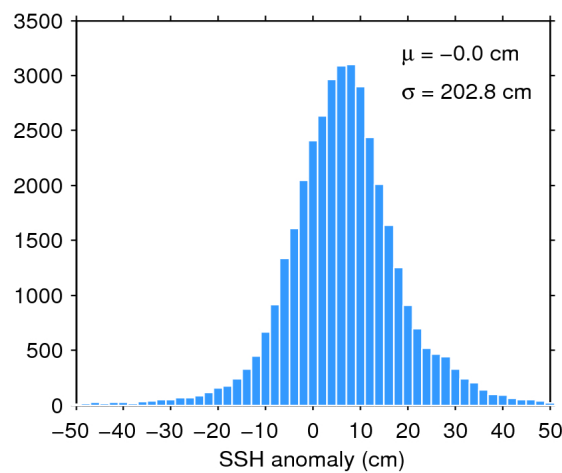
Figure 7. Histogram of flag-valid SSH anomaly over oceans and lakes for 25/09/2019. The mean ( \mu ) and standard deviation ( \sigma ) are also shown. Note that values outside [-50 50] cm are excluded from the histogram for the sake of readability but not from the computation of \mu and \sigma .
