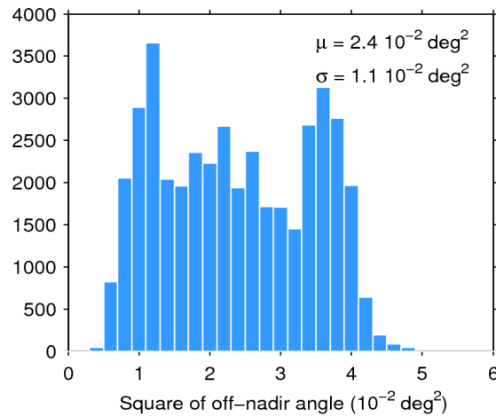
Figure 39. Histogram of flag-valid mispointing over oceans and lakes for 25/09/2019. The mean ( \mu ) and standard deviation ( \sigma ) are also shown. Note that values larger than 6 \cdot 10^{-2} \text{ deg}^2 are excluded from the histogram for the sake of readability but not from the computation of \mu and \sigma .
