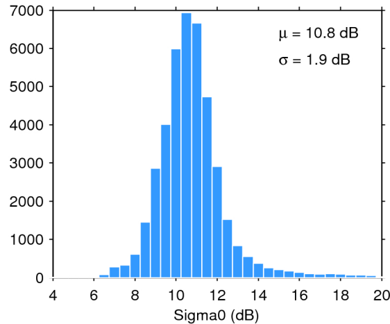
Figure 25. Histogram of flag-valid sigma0 over oceans and lakes for 24/09/2019. The mean ( \mu ) and standard deviation ( \sigma ) are also shown. Note that values outside [4 20] dB are excluded from the histogram for the sake of readability but not from the computation of \mu and \sigma .
