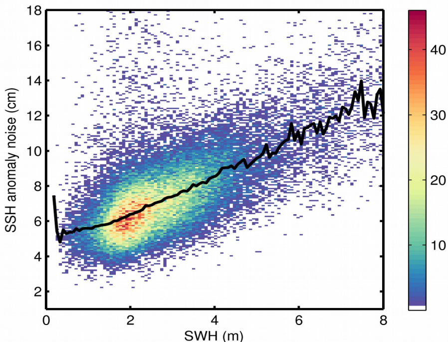
Figure 9. 2D histogram showing flag-valid SSH anomaly noise as a function of SWH for 24/09/2019. The black line denotes the median SSH anomaly noise as a function of SWH.
