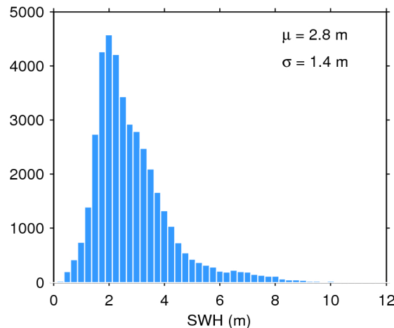
Figure 20. Histogram of science-valid SWH over oceans and lakes for 24/09/2019. The mean ( \mu ) and standard deviation ( \sigma ) are also shown. Note that values larger than 12 m are excluded from the histogram for the sake of readability but not from the computation of \mu and \sigma .
