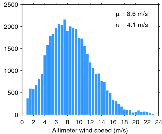
Figure 33. Histogram of flag-valid wind over oceans and lakes for 24/09/2019. The mean ( \mu ) and standard deviation ( \sigma ) are also shown. Note that values larger than 24 m/s are excluded from the histogram for the sake of readability but not from the computation of \mu and \sigma .
