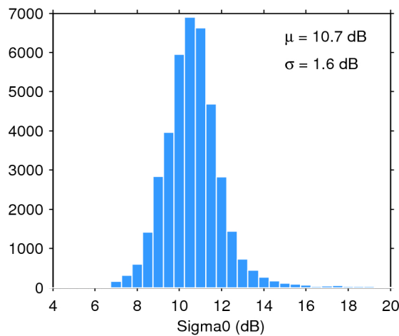
Figure 28. Histogram of science-valid sigma0 over oceans and lakes for 24/09/2019. The mean ( \mu ) and standard deviation ( \sigma ) are also shown. Note that values outside [4 20] dB are excluded from the histogram for the sake of readability but not from the computation of \mu and \sigma .
