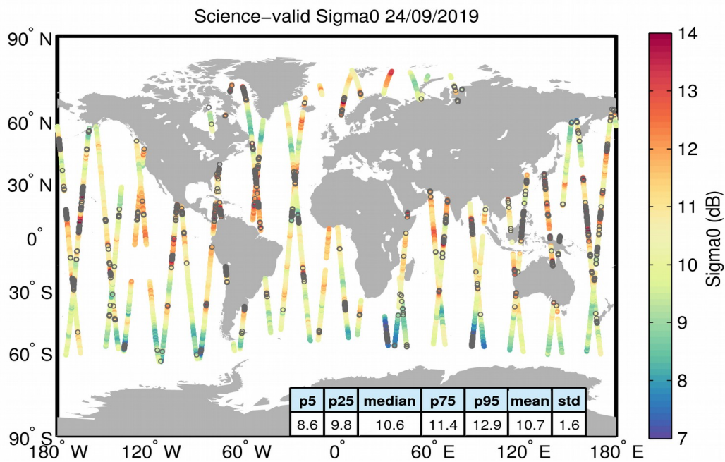
Figure 27. Geographical distribution of science-valid sigma0 data over oceans and lakes for 24/09/2019. The statistical values shown in the table refer to the sigma0 in dB and are calculated over all measurements shown in the figure. Gray circles denote records that have been rejected based on the editing criteria described in Table 4.
