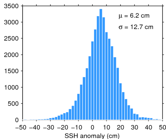
Figure 11. Histogram of science-valid SSH anomaly over oceans and lakes for 24/09/2019. The mean ( \mu ) and standard deviation ( \sigma ) are also shown. Note that values outside [-50 50] cm are excluded from the histogram for the sake of readability but not from the computation of \mu and \sigma .
