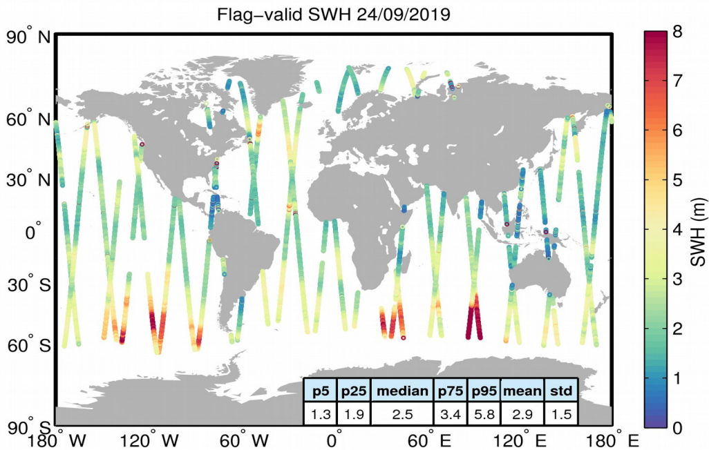
Figure 15. Geographical distribution of flag-valid SWH data over oceans and lakes for 24/09/2019. The statistical values shown in the table refer to the SWH in m and are calculated over all measurements shown in the figure.
