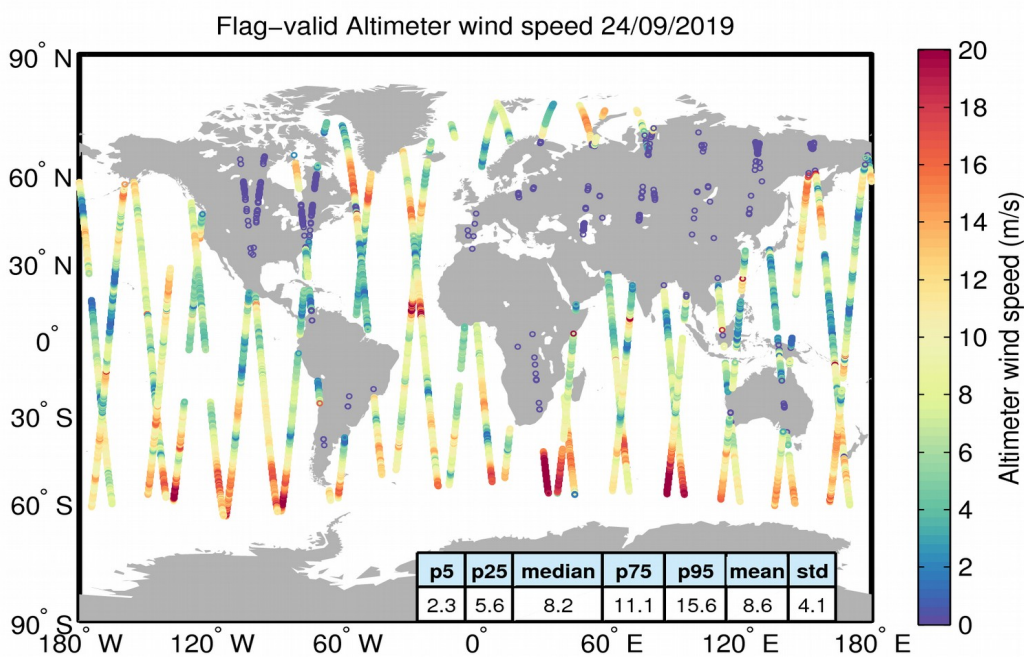
Figure 31. Geographical distribution of flag-valid wind data over oceans and lakes for 24/09/2019. The statistical values shown in the table refer to the wind in m/s and are calculated over all measurements shown in the figure.
