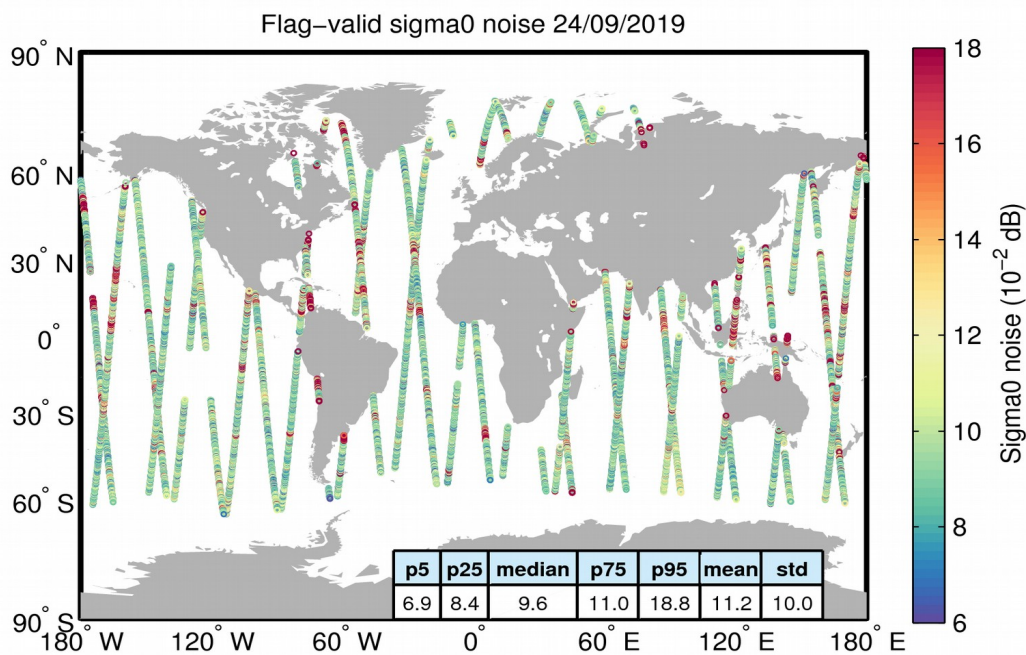
Figure 26. Geographical distribution of flag-valid 20-Hz sigma0 measurement noise over oceans and lakes for 24/09/2019. The statistical values shown in the table refer to the sigma0 noise and are calculated over all measurements shown in the figure.
