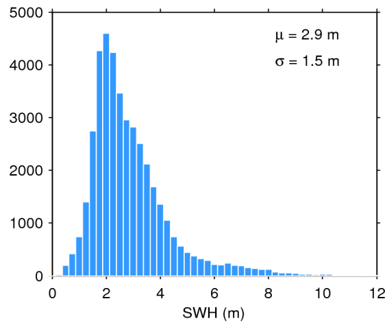
Figure 17. Histogram of flag-valid SWH over oceans and lakes for 24/09/2019. The mean ( \mu ) and standard deviation ( \sigma ) are also shown. Note that values larger than 12 m are excluded from the histogram for the sake of readability but not from the computation of \mu and \sigma .
