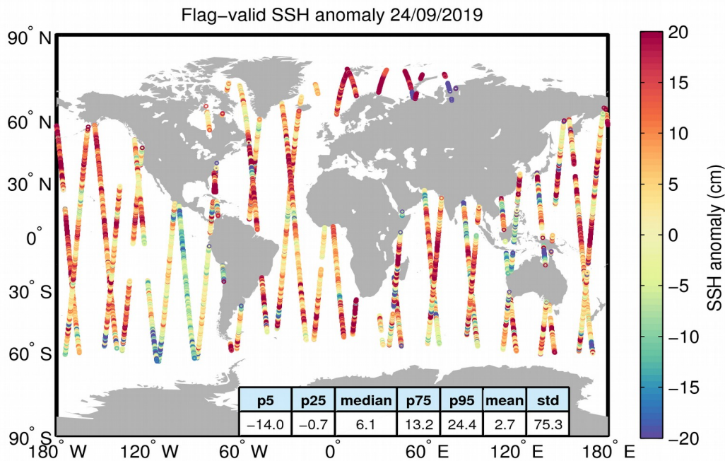
Figure 5. Geographical distribution of flag-valid 1-Hz SSH anomaly data over oceans and lakes for 24/09/2019. The statistical values shown in the table refer to the SSH anomaly in cm and are calculated over all measurements shown in the figure.
