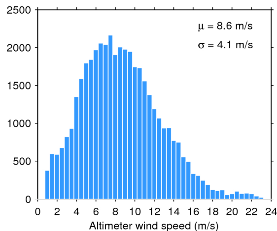
Figure 35. Histogram of science-valid wind over oceans and lakes for 24/09/2019. The mean ( \mu ) and standard deviation ( \sigma ) are also shown. Note that values larger than 24 m/s are excluded from the histogram for the sake of readability but not from the computation of \mu and \sigma .
