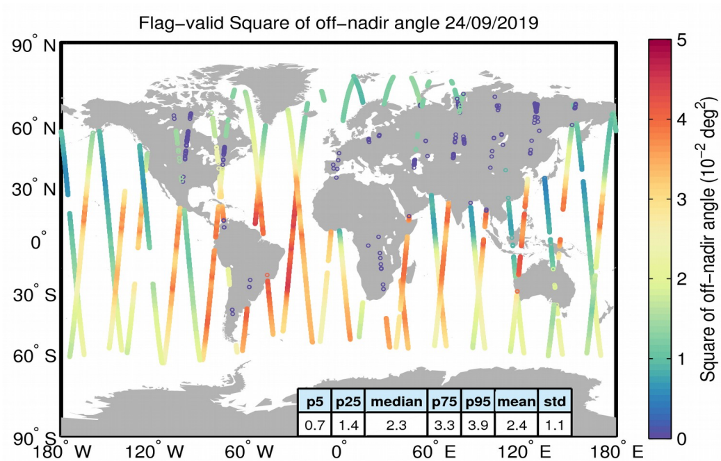
Figure 37. Geographical distribution of flag-valid mispointing data over oceans and lakes for 24/09/2019. The statistical values shown in the table refer to the mispointing in 10^{-2} deg 2 and are calculated over all measurements shown in the figure.
