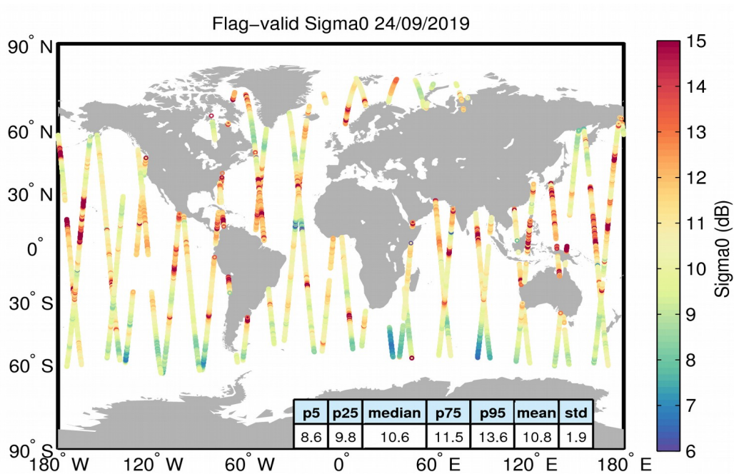
Figure 23. Geographical distribution of flag-valid sigma0 data over oceans and lakes for 24/09/2019. The statistical values shown in the table refer to the sigma0 in dB and are calculated over all measurements shown in the figure.
