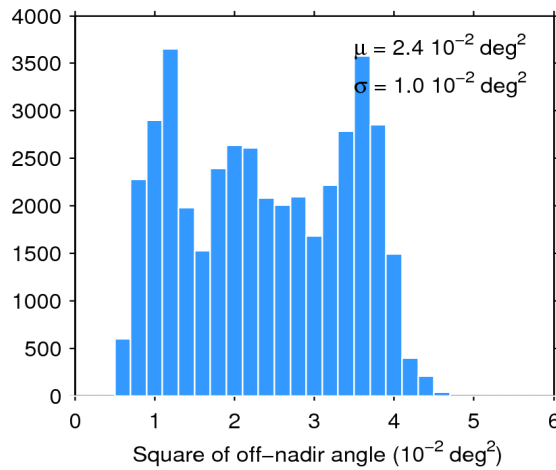
Figure 39. Histogram of flag-valid mispointing over oceans and lakes for 23/09/2019. The mean ( \mu ) and standard deviation ( \sigma ) are also shown. Note that values larger than 6 \cdot 10^{-2} \text{ deg}^2 are excluded from the histogram for the sake of readability but not from the computation of \mu and \sigma .
