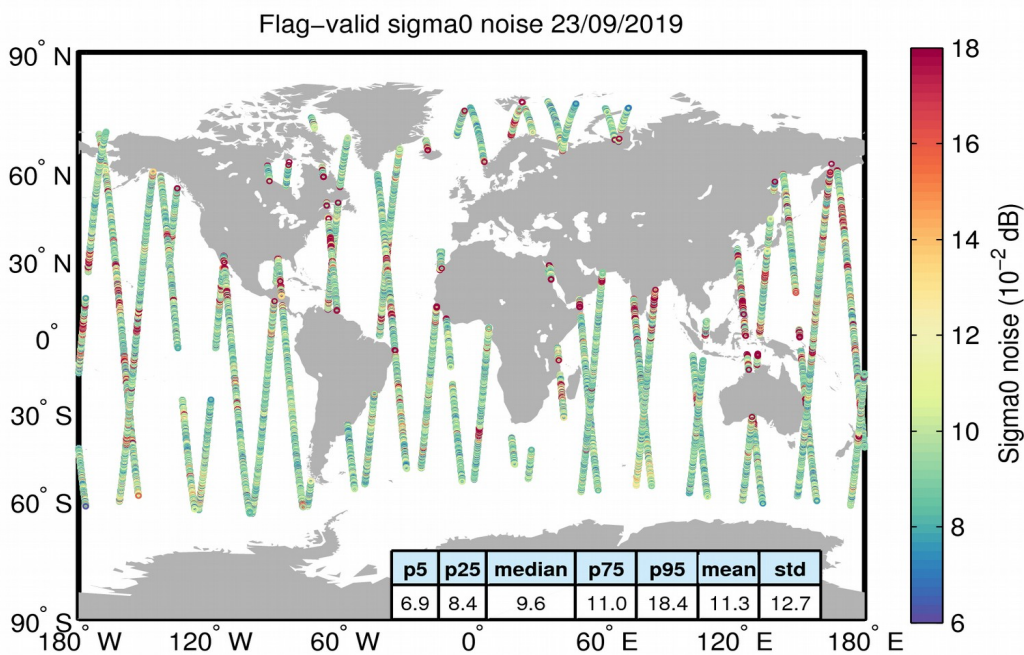
Figure 26. Geographical distribution of flag-valid 20-Hz sigma0 measurement noise over oceans and lakes for 23/09/2019. The statistical values shown in the table refer to the sigma0 noise and are calculated over all measurements shown in the figure.
