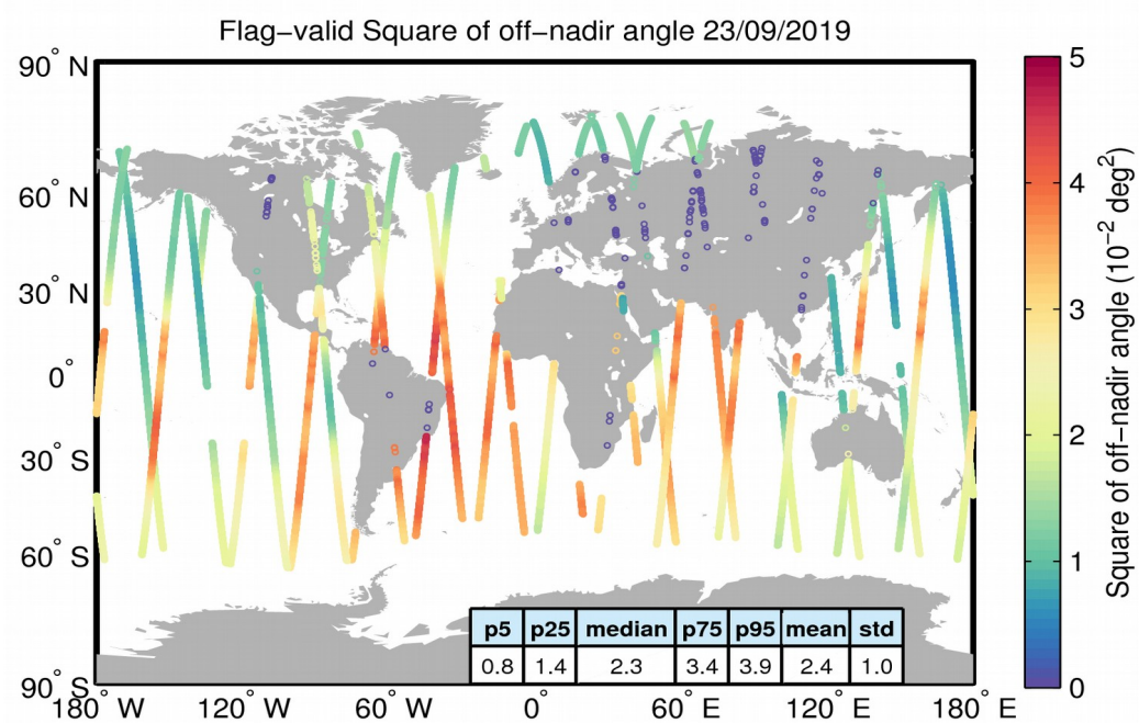
Figure 37. Geographical distribution of flag-valid mispointing data over oceans and lakes for 23/09/2019. The statistical values shown in the table refer to the mispointing in 10^{-2} \text{deg}^2 and are calculated over all measurements shown in the figure.
