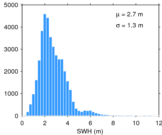
Figure 20. Histogram of science-valid SWH over oceans and lakes for 23/09/2019. The mean ( \mu ) and standard deviation ( \sigma ) are also shown. Note that values larger than 12 m are excluded from the histogram for the sake of readability but not from the computation of \mu and \sigma .
