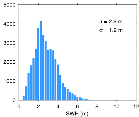
Figure 17. Histogram of flag-valid SWH over oceans and lakes for 21/09/2019. The mean ( \mu ) and standard deviation ( \sigma ) are also shown. Note that values larger than 12 m are excluded from the histogram for the sake of readability but not from the computation of \mu and \sigma .
