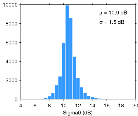
Figure 28. Histogram of science-valid sigma0 over oceans and lakes for 21/09/2019. The mean ( \mu ) and standard deviation ( \sigma ) are also shown. Note that values outside [4 20] dB are excluded from the histogram for the sake of readability but not from the computation of \mu and \sigma .
