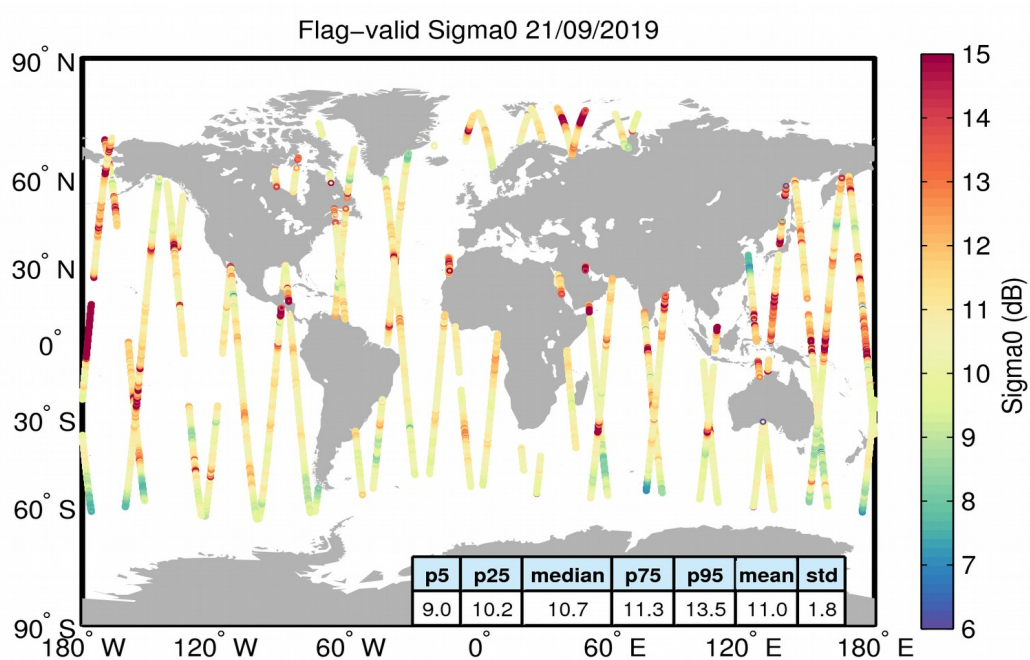
Figure 23. Geographical distribution of flag-valid sigma0 data over oceans and lakes for 21/09/2019. The statistical values shown in the table refer to the sigma0 in dB and are calculated over all measurements shown in the figure.
