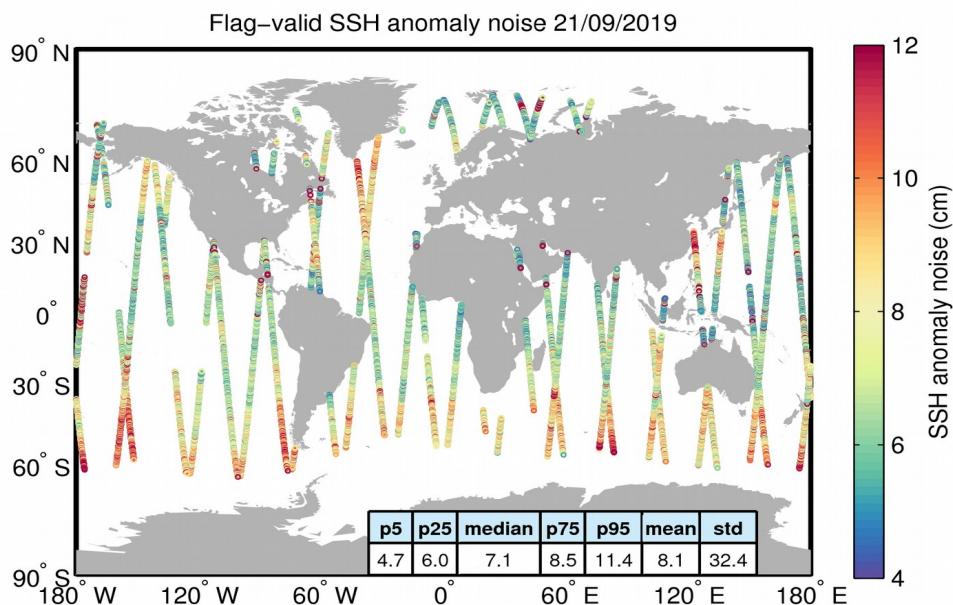
Figure 8. Geographical distribution of flag-valid 20-Hz SSH anomaly measurement noise over oceans and lakes for 21/09/2019. The statistical values shown in the table refer to the SSH anomaly noise and are calculated over all measurements shown in the figure.
