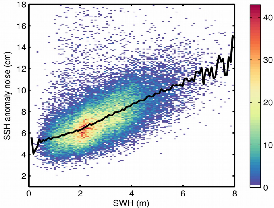
Figure 9. 2D histogram showing flag-valid SSH anomaly noise as a function of SWH for 21/09/2019. The black line denotes the median SSH anomaly noise as a function of SWH.
