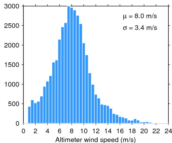
Figure 35. Histogram of science-valid wind over oceans and lakes for 21/09/2019. The mean ( \mu ) and standard deviation ( \sigma ) are also shown. Note that values larger than 24 m/s are excluded from the histogram for the sake of readability but not from the computation of \mu and \sigma .
