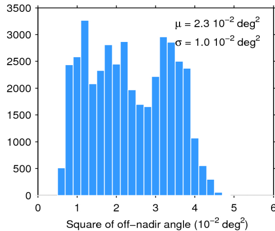
Figure 39. Histogram of flag-valid mispointing over oceans and lakes for 21/09/2019. The mean ( \mu ) and standard deviation ( \sigma ) are also shown. Note that values larger than 6 \cdot 10^{-2} \text{ deg}^2 are excluded from the histogram for the sake of readability but not from the computation of \mu and \sigma .
