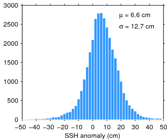
Figure 11. Histogram of science-valid SSH anomaly over oceans and lakes for 21/09/2019. The mean ( \mu ) and standard deviation ( \sigma ) are also shown. Note that values outside [-50 50] cm are excluded from the histogram for the sake of readability but not from the computation of \mu and \sigma .
