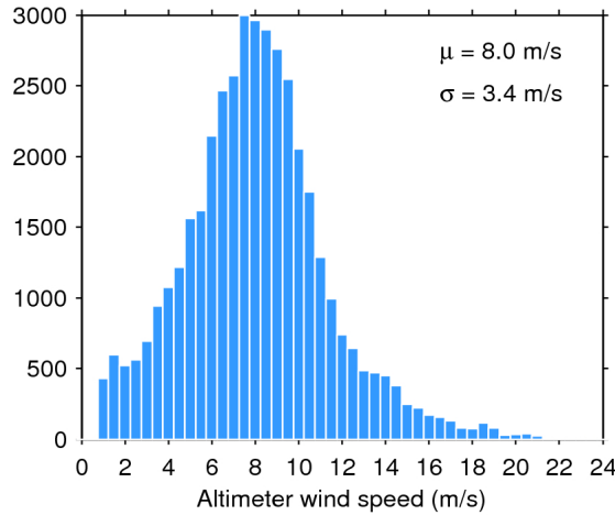
Figure 33. Histogram of flag-valid wind over oceans and lakes for 21/09/2019. The mean ( \mu ) and standard deviation ( \sigma ) are also shown. Note that values larger than 24 m/s are excluded from the histogram for the sake of readability but not from the computation of \mu and \sigma .
