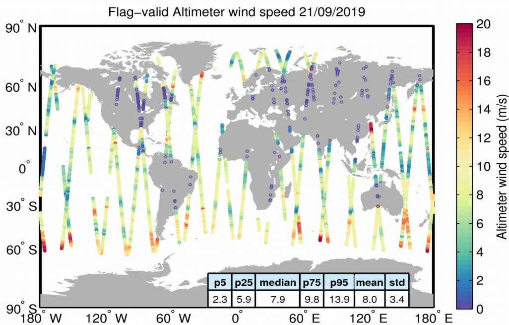
Figure 31. Geographical distribution of flag-valid wind data over oceans and lakes for 21/09/2019. The statistical values shown in the table refer to the wind in m/s and are calculated over all measurements shown in the figure.
