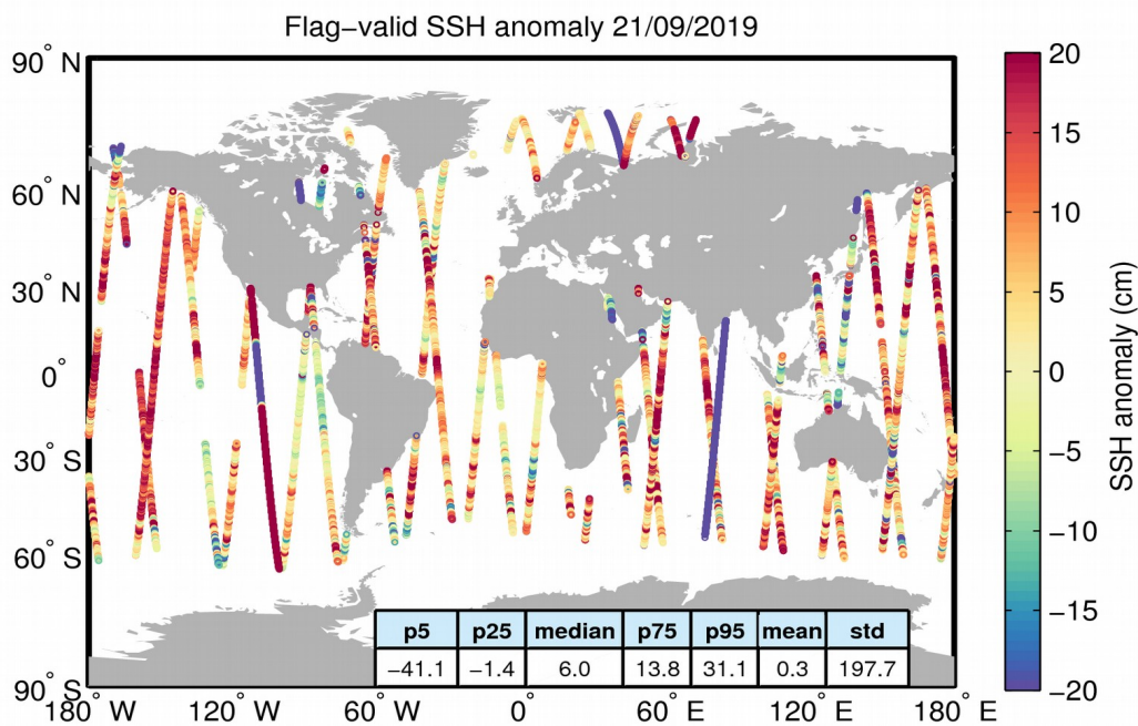
Figure 5. Geographical distribution of flag-valid 1-Hz SSH anomaly data over oceans and lakes for 21/09/2019. The statistical values shown in the table refer to the SSH anomaly in cm and are calculated over all measurements shown in the figure.
