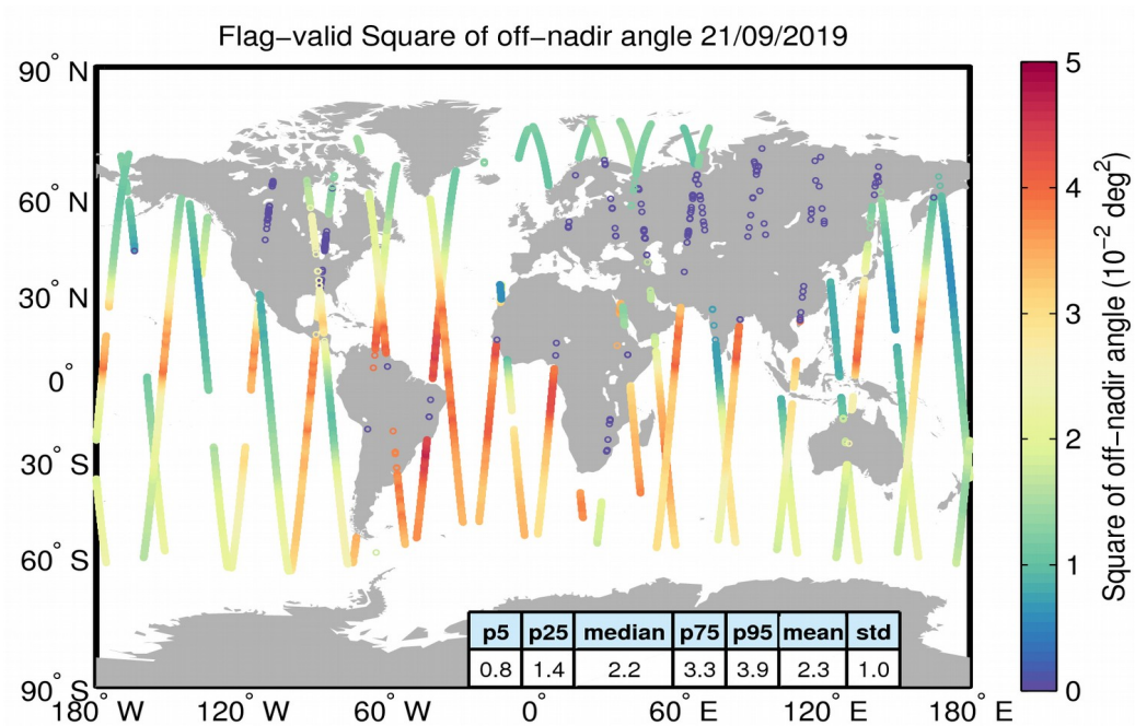
Figure 37. Geographical distribution of flag-valid mispointing data over oceans and lakes for 21/09/2019. The statistical values shown in the table refer to the mispointing in 10^{-2} deg 2 and are calculated over all measurements shown in the figure.
