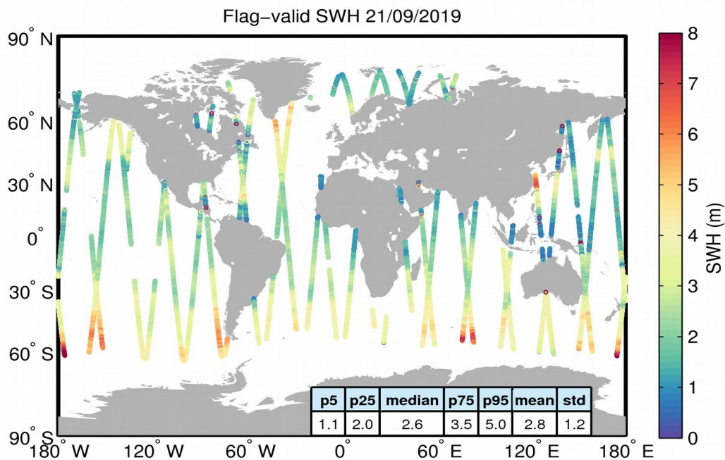
Figure 15. Geographical distribution of flag-valid SWH data over oceans and lakes for 21/09/2019. The statistical values shown in the table refer to the SWH in m and are calculated over all measurements shown in the figure.
