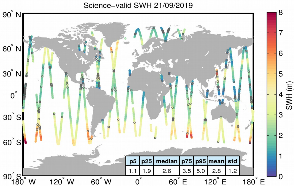
Figure 19. Geographical distribution of science-valid SWH data over oceans and lakes for 21/09/2019. The statistical values shown in the table refer to the SWH in m and are calculated over all measurements shown in the figure. Gray circles denote records that have been rejected based on the editing criteria described in Table 3.
