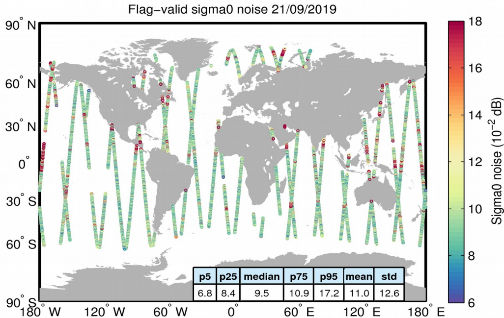
Figure 26. Geographical distribution of flag-valid 20-Hz sigma0 measurement noise over oceans and lakes for 21/09/2019. The statistical values shown in the table refer to the sigma0 noise and are calculated over all measurements shown in the figure.
