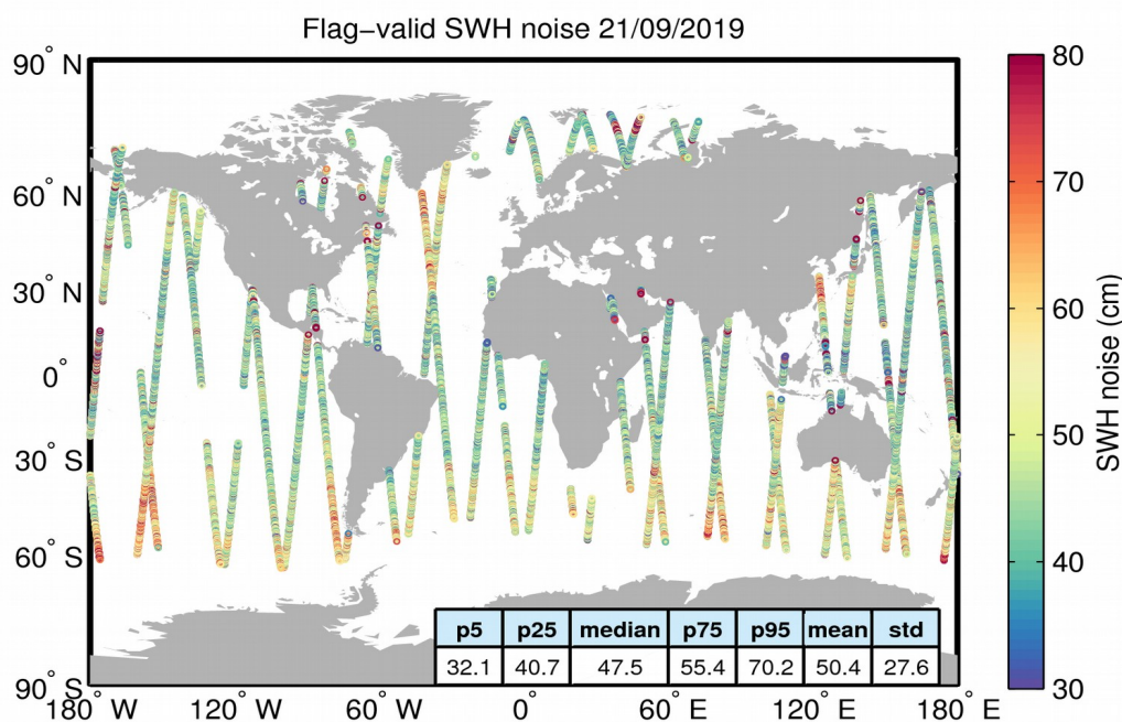
Figure 18. Geographical distribution of flag-valid 20-Hz SWH measurement noise over oceans and lakes for 21/09/2019. The statistical values shown in the figure refer to the SWH noise and are calculated over all measurements shown in the figure.
