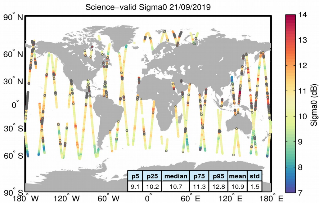
Figure 27. Geographical distribution of science-valid sigma0 data over oceans and lakes for 21/09/2019. The statistical values shown in the table refer to the sigma0 in dB and are calculated over all measurements shown in the figure. Gray circles denote records that have been rejected based on the editing criteria described in Table 4.
