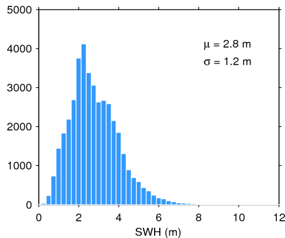
Figure 20. Histogram of science-valid SWH over oceans and lakes for 21/09/2019. The mean ( \mu ) and standard deviation ( \sigma ) are also shown. Note that values larger than 12 m are excluded from the histogram for the sake of readability but not from the computation of \mu and \sigma .
