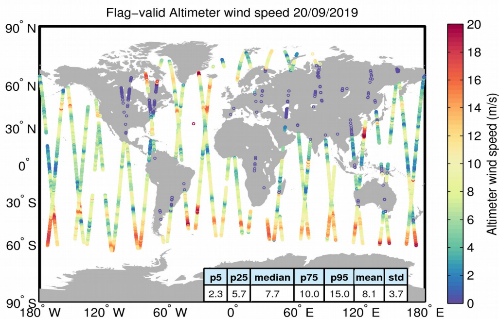
Figure 31. Geographical distribution of flag-valid wind data over oceans and lakes for 20/09/2019. The statistical values shown in the table refer to the wind in m/s and are calculated over all measurements shown in the figure.
