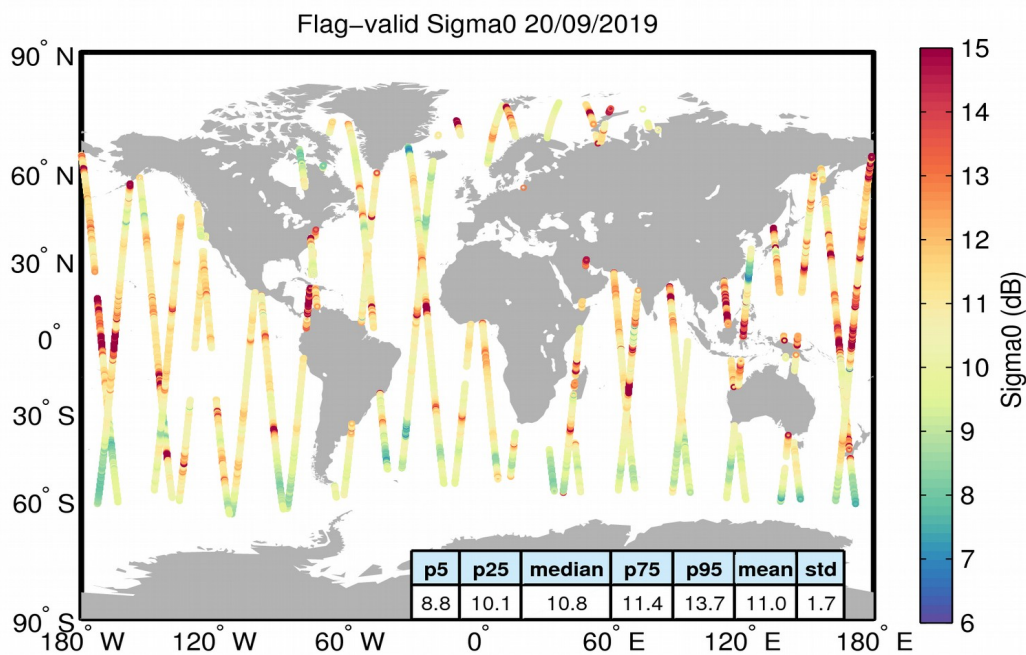
Figure 23. Geographical distribution of flag-valid sigma0 data over oceans and lakes for 20/09/2019. The statistical values shown in the table refer to the sigma0 in dB and are calculated over all measurements shown in the figure.
