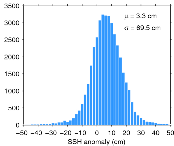
Figure 7. Histogram of flag-valid SSH anomaly over oceans and lakes for 20/09/2019. The mean ( \mu ) and standard deviation ( \sigma ) are also shown. Note that values outside [-50\ 50] cm are excluded from the histogram for the sake of readability but not from the computation of \mu and \sigma .
