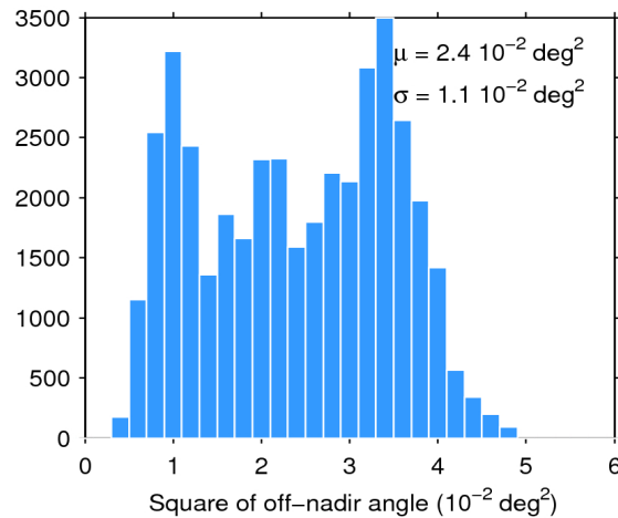
Figure 39. Histogram of flag-valid mispointing over oceans and lakes for 20/09/2019. The mean ( \mu ) and standard deviation ( \sigma ) are also shown. Note that values larger than 6 \cdot 10^{-2} \text{ deg}^2 are excluded from the histogram for the sake of readability but not from the computation of \mu and \sigma .
