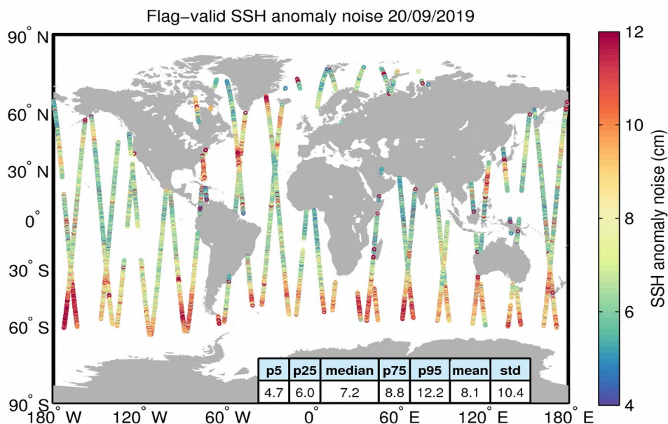
Figure 8. Geographical distribution of flag-valid 20-Hz SSH anomaly measurement noise over oceans and lakes for 20/09/2019. The statistical values shown in the table refer to the SSH anomaly noise and are calculated over all measurements shown in the figure.
