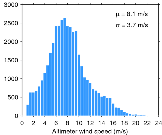
Figure 33. Histogram of flag-valid wind over oceans and lakes for 20/09/2019. The mean ( \mu ) and standard deviation ( \sigma ) are also shown. Note that values larger than 24 m/s are excluded from the histogram for the sake of readability but not from the computation of \mu and \sigma .
