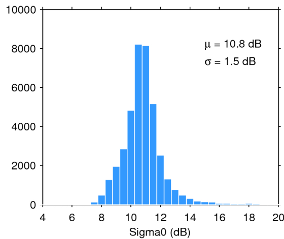
Figure 28. Histogram of science-valid sigma0 over oceans and lakes for 20/09/2019. The mean ( \mu ) and standard deviation ( \sigma ) are also shown. Note that values outside [4 20] dB are excluded from the histogram for the sake of readability but not from the computation of \mu and \sigma .
