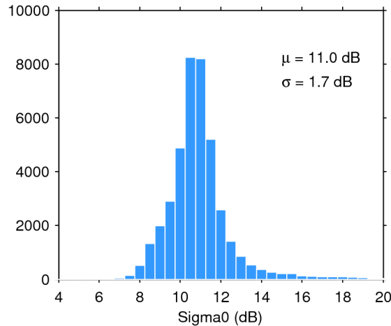
Figure 25. Histogram of flag-valid sigma0 over oceans and lakes for 20/09/2019. The mean ( \mu ) and standard deviation ( \sigma ) are also shown. Note that values outside [4 20] dB are excluded from the histogram for the sake of readability but not from the computation of \mu and \sigma .
