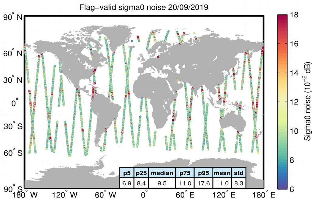
Figure 26. Geographical distribution of flag-valid 20-Hz sigma0 measurement noise over oceans and lakes for 20/09/2019. The statistical values shown in the table refer to the sigma0 noise and are calculated over all measurements shown in the figure.
