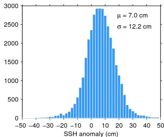
Figure 11. Histogram of science-valid SSH anomaly over oceans and lakes for 20/09/2019. The mean ( \mu ) and standard deviation ( \sigma ) are also shown. Note that values outside [-50 50] cm are excluded from the histogram for the sake of readability but not from the computation of \mu and \sigma .
