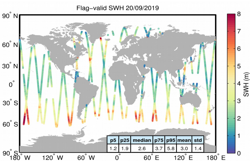
Figure 15. Geographical distribution of flag-valid SWH data over oceans and lakes for 20/09/2019. The statistical values shown in the table refer to the SWH in m and are calculated over all measurements shown in the figure.
