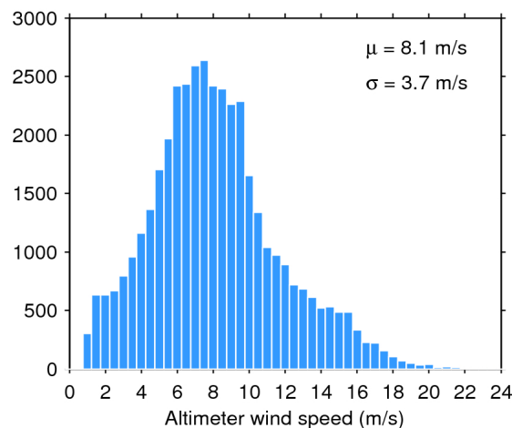
Figure 35. Histogram of science-valid wind over oceans and lakes for 20/09/2019. The mean ( \mu ) and standard deviation ( \sigma ) are also shown. Note that values larger than 24 m/s are excluded from the histogram for the sake of readability but not from the computation of \mu and \sigma .
