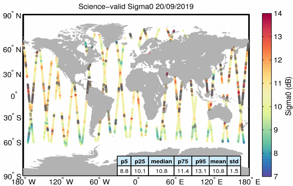
Figure 27. Geographical distribution of science-valid sigma0 data over oceans and lakes for 20/09/2019. The statistical values shown in the table refer to the sigma0 in dB and are calculated over all measurements shown in the figure. Gray circles denote records that have been rejected based on the editing criteria described in Table 4.
