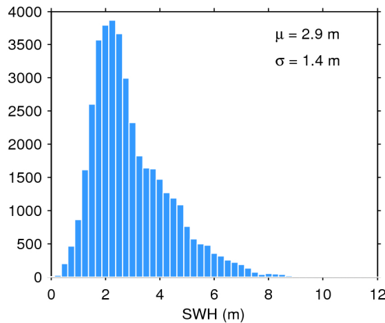
Figure 20. Histogram of science-valid SWH over oceans and lakes for 20/09/2019. The mean ( \mu ) and standard deviation ( \sigma ) are also shown. Note that values larger than 12 m are excluded from the histogram for the sake of readability but not from the computation of \mu and \sigma .
