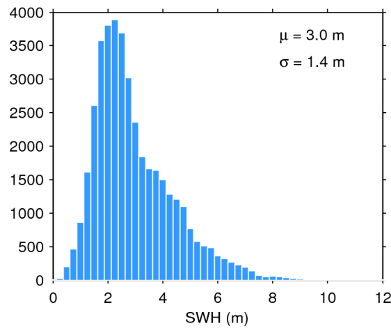
Figure 17. Histogram of flag-valid SWH over oceans and lakes for 20/09/2019. The mean ( \mu ) and standard deviation ( \sigma ) are also shown. Note that values larger than 12 m are excluded from the histogram for the sake of readability but not from the computation of \mu and \sigma .
