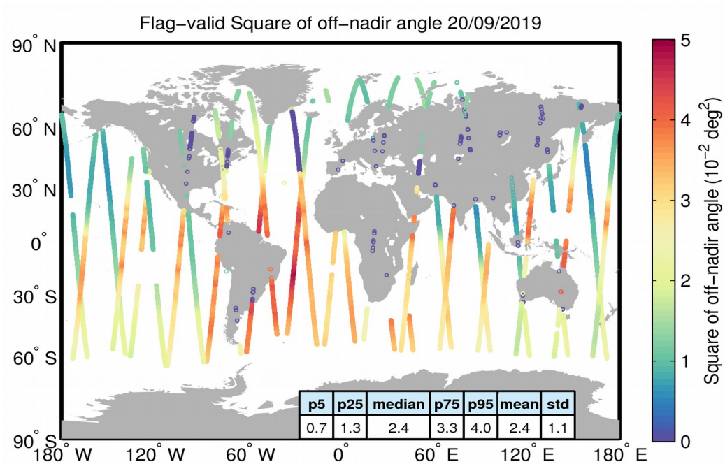
Figure 37. Geographical distribution of flag-valid mispointing data over oceans and lakes for 20/09/2019. The statistical values shown in the table refer to the mispointing in 10^{-2} \text{ deg}^2 and are calculated over all measurements shown in the figure.
