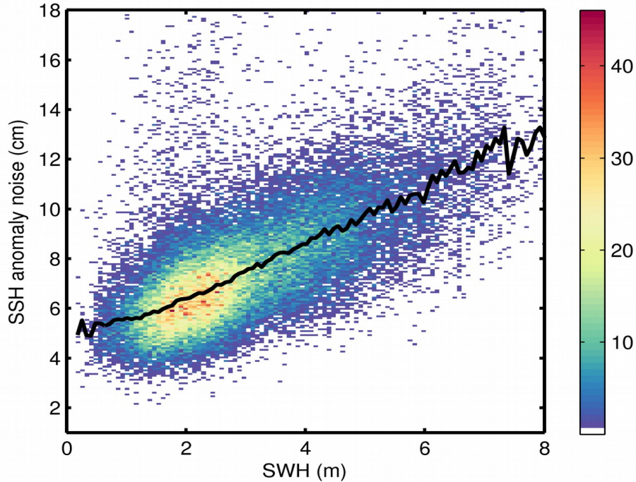
Figure 9. 2D histogram showing flag-valid SSH anomaly noise as a function of SWH for 20/09/2019. The black line denotes the median SSH anomaly noise as a function of SWH.
