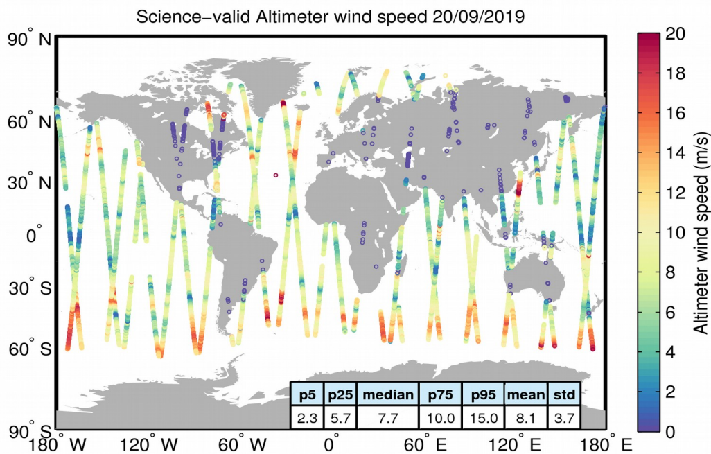
Figure 34. Geographical distribution of science-valid wind data over oceans and lakes for 20/09/2019. The statistical values shown in the table refer to the wind in m/s and are calculated over all measurements shown in the figure. Gray circles denote records that have been rejected based on the editing criteria described in Table 5.
