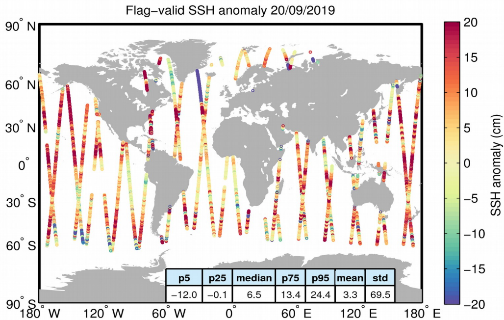
Figure 5. Geographical distribution of flag-valid 1-Hz SSH anomaly data over oceans and lakes for 20/09/2019. The statistical values shown in the table refer to the SSH anomaly in cm and are calculated over all measurements shown in the figure.
