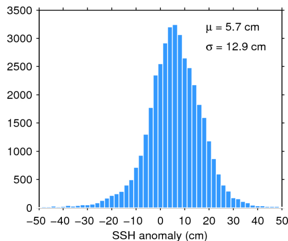
Figure 11. Histogram of science-valid SSH anomaly over oceans and lakes for 19/09/2019. The mean ( \mu ) and standard deviation ( \sigma ) are also shown. Note that values outside [-50 50] cm are excluded from the histogram for the sake of readability but not from the computation of \mu and \sigma .
