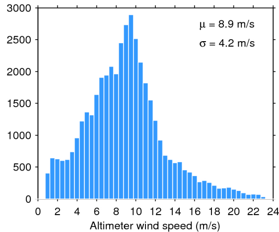
Figure 33. Histogram of flag-valid wind over oceans and lakes for 19/09/2019. The mean ( \mu ) and standard deviation ( \sigma ) are also shown. Note that values larger than 24 m/s are excluded from the histogram for the sake of readability but not from the computation of \mu and \sigma .
