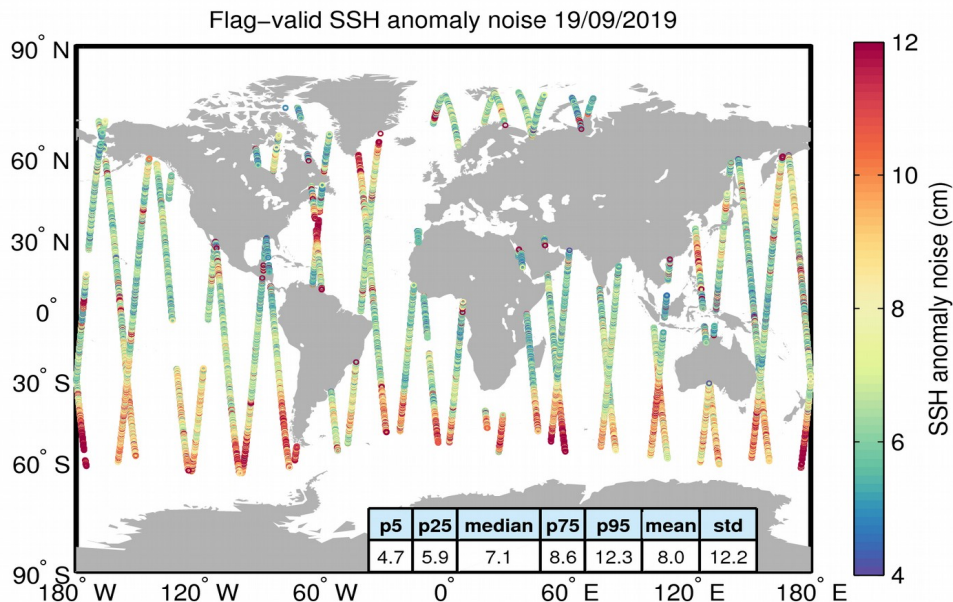
Figure 8. Geographical distribution of flag-valid 20-Hz SSH anomaly measurement noise over oceans and lakes for 19/09/2019. The statistical values shown in the table refer to the SSH anomaly noise and are calculated over all measurements shown in the figure.
