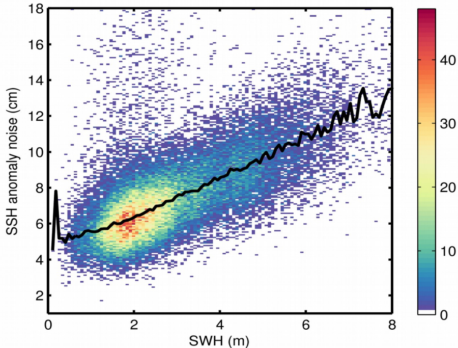
Figure 9. 2D histogram showing flag-valid SSH anomaly noise as a function of SWH for 19/09/2019. The black line denotes the median SSH anomaly noise as a function of SWH.
