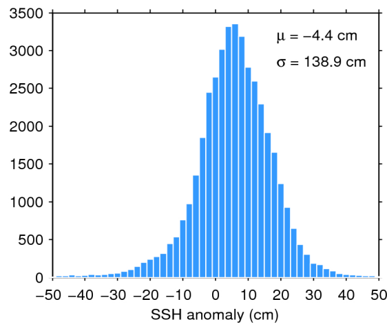
Figure 7. Histogram of flag-valid SSH anomaly over oceans and lakes for 19/09/2019. The mean ( \mu ) and standard deviation ( \sigma ) are also shown. Note that values outside [-50\ 50] cm are excluded from the histogram for the sake of readability but not from the computation of \mu and \sigma .
