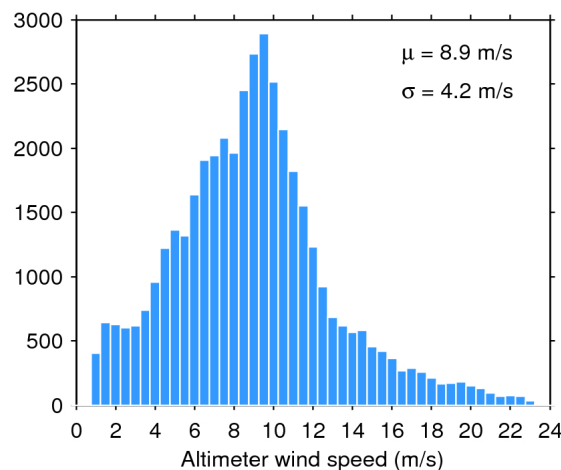
Figure 35. Histogram of science-valid wind over oceans and lakes for 19/09/2019. The mean ( \mu ) and standard deviation ( \sigma ) are also shown. Note that values larger than 24 m/s are excluded from the histogram for the sake of readability but not from the computation of \mu and \sigma .
