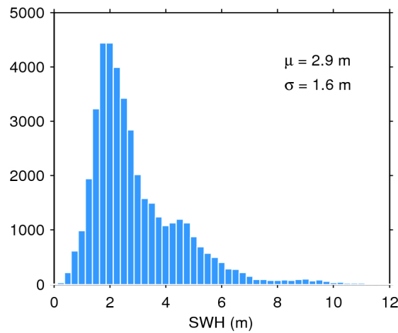
Figure 17. Histogram of flag-valid SWH over oceans and lakes for 19/09/2019. The mean ( \mu ) and standard deviation ( \sigma ) are also shown. Note that values larger than 12 m are excluded from the histogram for the sake of readability but not from the computation of \mu and \sigma .
