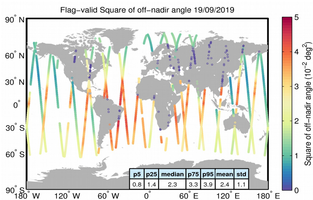
Figure 37. Geographical distribution of flag-valid mispointing data over oceans and lakes for 19/09/2019. The statistical values shown in the table refer to the mispointing in 10^{-2} \text{ deg}^2 and are calculated over all measurements shown in the figure.
