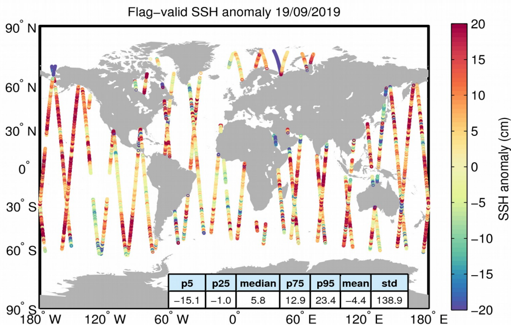
Figure 5. Geographical distribution of flag-valid 1-Hz SSH anomaly data over oceans and lakes for 19/09/2019. The statistical values shown in the table refer to the SSH anomaly in cm and are calculated over all measurements shown in the figure.
