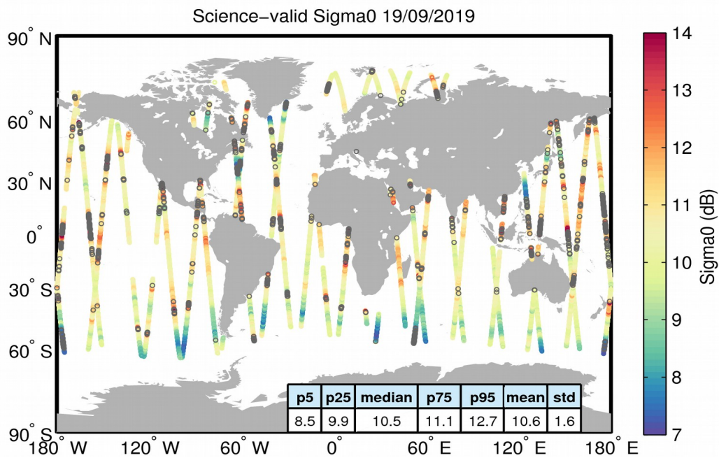
Figure 27. Geographical distribution of science-valid sigma0 data over oceans and lakes for 19/09/2019. The statistical values shown in the table refer to the sigma0 in dB and are calculated over all measurements shown in the figure. Gray circles denote records that have been rejected based on the editing criteria described in Table 4.
