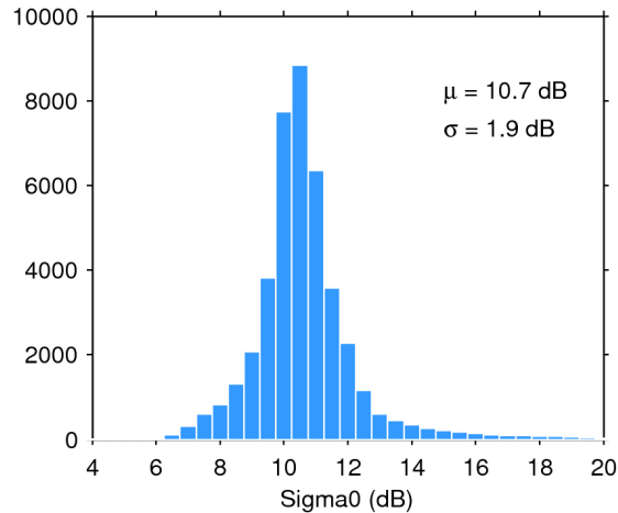
Figure 25. Histogram of flag-valid sigma0 over oceans and lakes for 19/09/2019. The mean ( \mu ) and standard deviation ( \sigma ) are also shown. Note that values outside [4 20] dB are excluded from the histogram for the sake of readability but not from the computation of \mu and \sigma .
