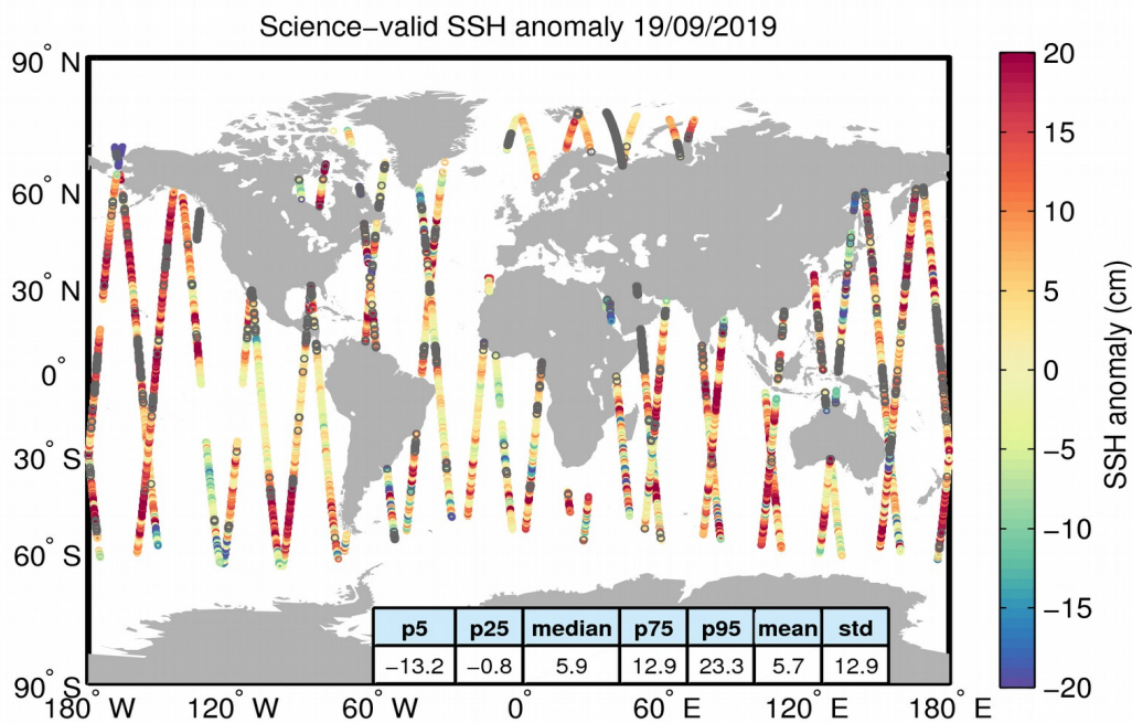
Figure 10. Geographical distribution of science-valid SSH anomaly data over oceans and lakes for 19/09/2019. The statistical values shown in the table refer to the SSH anomaly in cm and are calculated over all measurements shown in the figure. Gray circles denote records that have been rejected based on the editing criteria described in Table 2.
