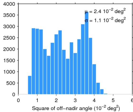
Figure 39. Histogram of flag-valid mispointing over oceans and lakes for 19/09/2019. The mean ( \mu ) and standard deviation ( \sigma ) are also shown. Note that values larger than 6 \cdot 10^{-2} \text{ deg}^2 are excluded from the histogram for the sake of readability but not from the computation of \mu and \sigma .
