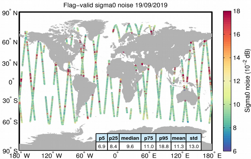
Figure 26. Geographical distribution of flag-valid 20-Hz sigma0 measurement noise over oceans and lakes for 19/09/2019. The statistical values shown in the table refer to the sigma0 noise and are calculated over all measurements shown in the figure.
