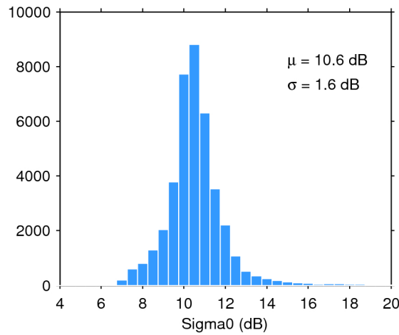
Figure 28. Histogram of science-valid sigma0 over oceans and lakes for 19/09/2019. The mean ( \mu ) and standard deviation ( \sigma ) are also shown. Note that values outside [4 20] dB are excluded from the histogram for the sake of readability but not from the computation of \mu and \sigma .
