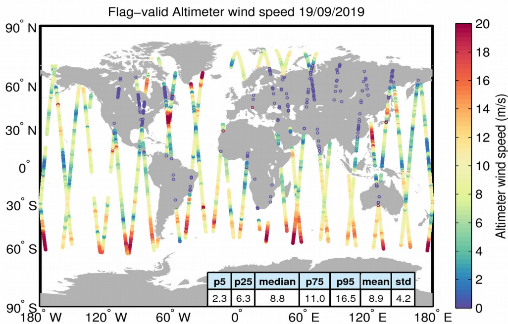
Figure 31. Geographical distribution of flag-valid wind data over oceans and lakes for 19/09/2019. The statistical values shown in the table refer to the wind in m/s and are calculated over all measurements shown in the figure.
