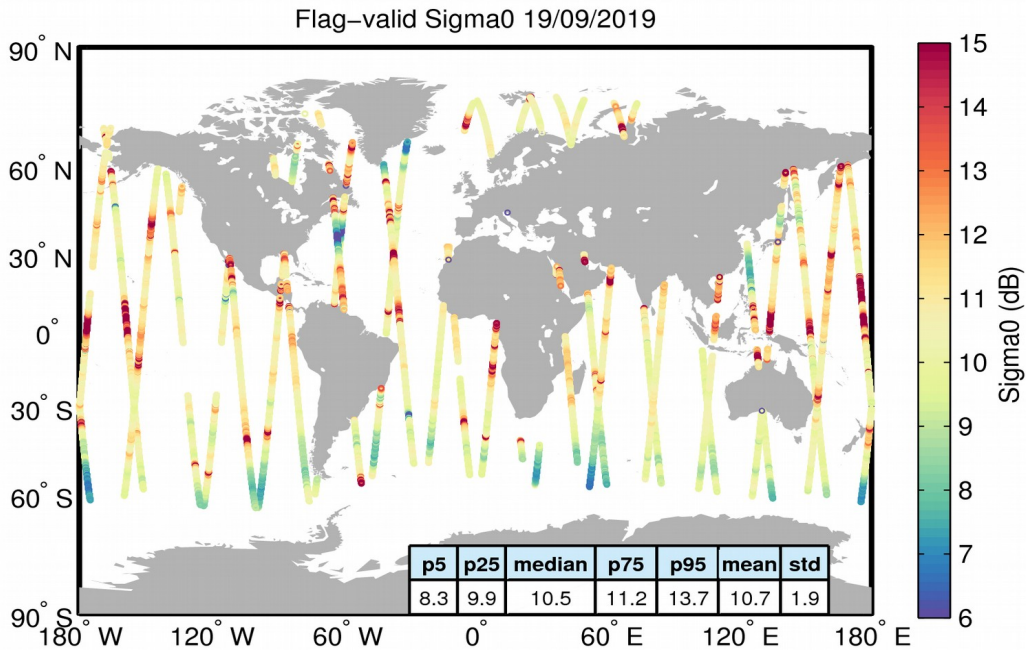
Figure 23. Geographical distribution of flag-valid sigma0 data over oceans and lakes for 19/09/2019. The statistical values shown in the table refer to the sigma0 in dB and are calculated over all measurements shown in the figure.
