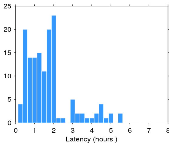
Figure 2. Histogram of the data latency for 19/09/2019. The y-axis denotes the number of files that are made available with a delay of x-hours with respect to the mean time of the records stored in the file.
