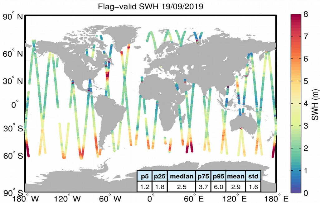
Figure 15. Geographical distribution of flag-valid SWH data over oceans and lakes for 19/09/2019. The statistical values shown in the table refer to the SWH in m and are calculated over all measurements shown in the figure.
