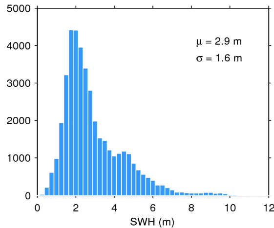
Figure 20. Histogram of science-valid SWH over oceans and lakes for 19/09/2019. The mean ( \mu ) and standard deviation ( \sigma ) are also shown. Note that values larger than 12 m are excluded from the histogram for the sake of readability but not from the computation of \mu and \sigma .
