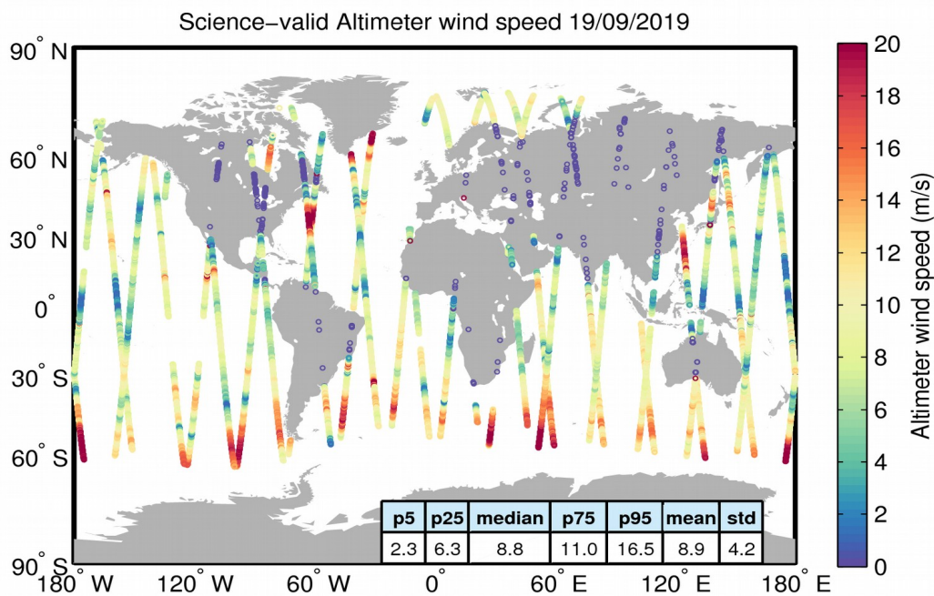
Figure 34. Geographical distribution of science-valid wind data over oceans and lakes for 19/09/2019. The statistical values shown in the table refer to the wind in m/s and are calculated over all measurements shown in the figure. Gray circles denote records that have been rejected based on the editing criteria described in Table 5.
