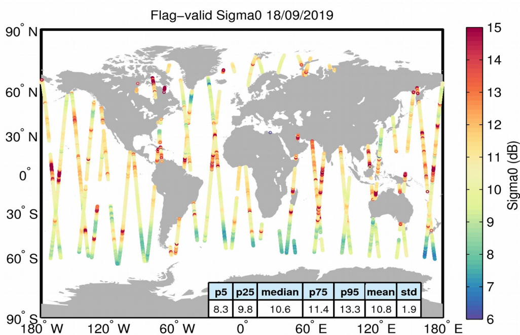
Figure 23. Geographical distribution of flag-valid sigma0 data over oceans and lakes for 18/09/2019. The statistical values shown in the table refer to the sigma0 in dB and are calculated over all measurements shown in the figure.
