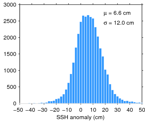
Figure 11. Histogram of science-valid SSH anomaly over oceans and lakes for 18/09/2019. The mean ( \mu ) and standard deviation ( \sigma ) are also shown. Note that values outside [-50 50] cm are excluded from the histogram for the sake of readability but not from the computation of \mu and \sigma .
