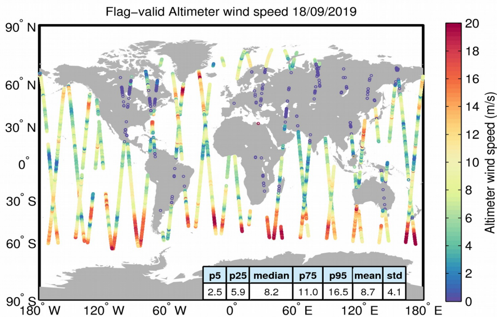
Figure 31. Geographical distribution of flag-valid wind data over oceans and lakes for 18/09/2019. The statistical values shown in the table refer to the wind in m/s and are calculated over all measurements shown in the figure.
