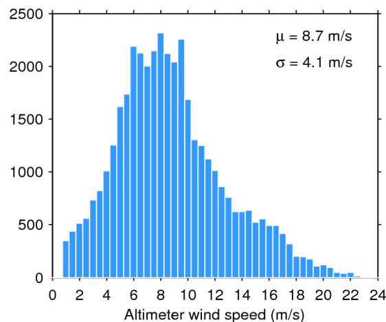
Figure 35. Histogram of science-valid wind over oceans and lakes for 18/09/2019. The mean ( \mu ) and standard deviation ( \sigma ) are also shown. Note that values larger than 24 m/s are excluded from the histogram for the sake of readability but not from the computation of \mu and \sigma .
