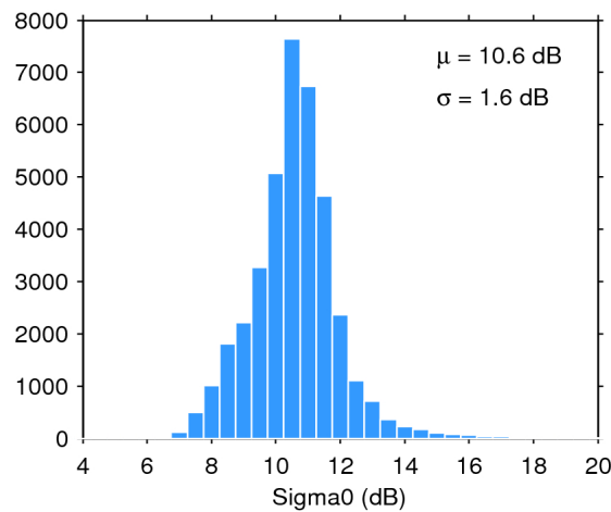
Figure 28. Histogram of science-valid sigma0 over oceans and lakes for 18/09/2019. The mean ( \mu ) and standard deviation ( \sigma ) are also shown. Note that values outside [4 20] dB are excluded from the histogram for the sake of readability but not from the computation of \mu and \sigma .
