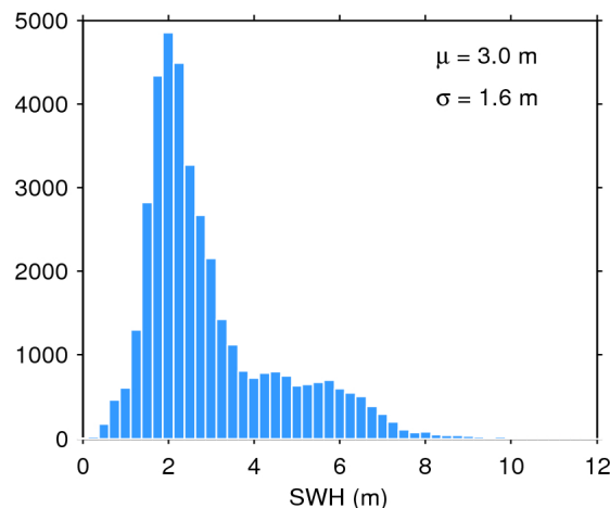
Figure 20. Histogram of science-valid SWH over oceans and lakes for 18/09/2019. The mean ( \mu ) and standard deviation ( \sigma ) are also shown. Note that values larger than 12 m are excluded from the histogram for the sake of readability but not from the computation of \mu and \sigma .
