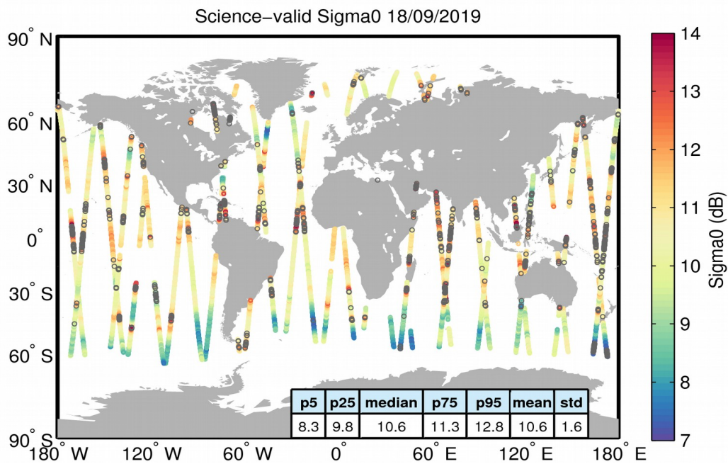
Figure 27. Geographical distribution of science-valid sigma0 data over oceans and lakes for 18/09/2019. The statistical values shown in the table refer to the sigma0 in dB and are calculated over all measurements shown in the figure. Gray circles denote records that have been rejected based on the editing criteria described in Table 4.
