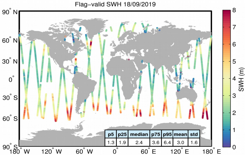
Figure 15. Geographical distribution of flag-valid SWH data over oceans and lakes for 18/09/2019. The statistical values shown in the table refer to the SWH in m and are calculated over all measurements shown in the figure.
