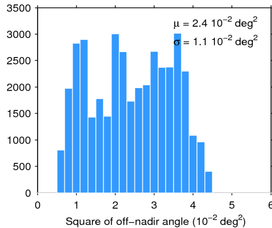
Figure 39. Histogram of flag-valid mispointing over oceans and lakes for 18/09/2019. The mean ( \mu ) and standard deviation ( \sigma ) are also shown. Note that values larger than 6 \cdot 10^{-2} \text{ deg}^2 are excluded from the histogram for the sake of readability but not from the computation of \mu and \sigma .
