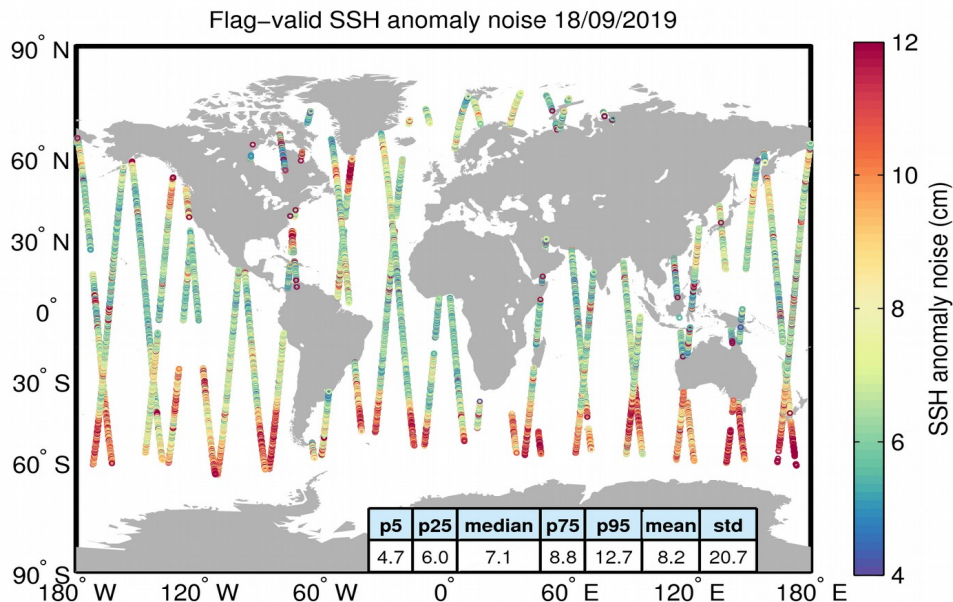
Figure 8. Geographical distribution of flag-valid 20-Hz SSH anomaly measurement noise over oceans and lakes for 18/09/2019. The statistical values shown in the table refer to the SSH anomaly noise and are calculated over all measurements shown in the figure.
