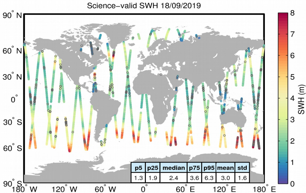
Figure 19. Geographical distribution of science-valid SWH data over oceans and lakes for 18/09/2019. The statistical values shown in the table refer to the SWH in m and are calculated over all measurements shown in the figure. Gray circles denote records that have been rejected based on the editing criteria described in Table 3.
