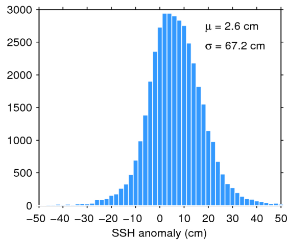
Figure 7. Histogram of flag-valid SSH anomaly over oceans and lakes for 18/09/2019. The mean ( \mu ) and standard deviation ( \sigma ) are also shown. Note that values outside [-50\ 50] cm are excluded from the histogram for the sake of readability but not from the computation of \mu and \sigma .
