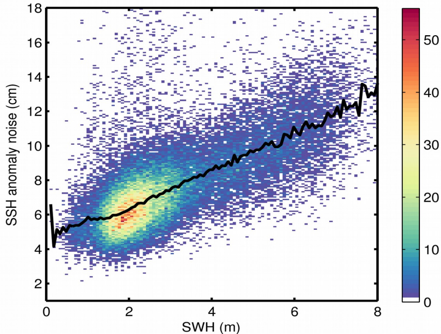
Figure 9. 2D histogram showing flag-valid SSH anomaly noise as a function of SWH for 18/09/2019. The black line denotes the median SSH anomaly noise as a function of SWH.
