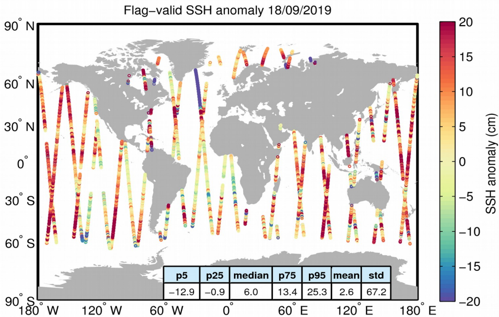
Figure 5. Geographical distribution of flag-valid 1-Hz SSH anomaly data over oceans and lakes for 18/09/2019. The statistical values shown in the table refer to the SSH anomaly in cm and are calculated over all measurements shown in the figure.
