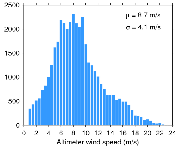
Figure 33. Histogram of flag-valid wind over oceans and lakes for 18/09/2019. The mean ( \mu ) and standard deviation ( \sigma ) are also shown. Note that values larger than 24 m/s are excluded from the histogram for the sake of readability but not from the computation of \mu and \sigma .
