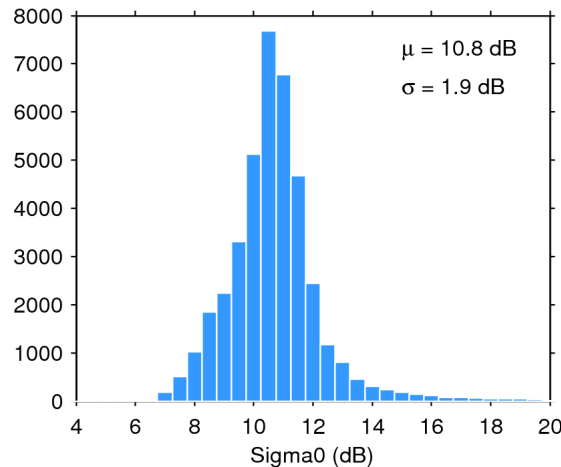
Figure 25. Histogram of flag-valid sigma0 over oceans and lakes for 18/09/2019. The mean ( \mu ) and standard deviation ( \sigma ) are also shown. Note that values outside [4 20] dB are excluded from the histogram for the sake of readability but not from the computation of \mu and \sigma .
