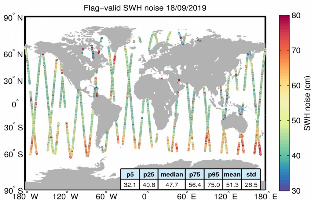
Figure 18. Geographical distribution of flag-valid 20-Hz SWH measurement noise over oceans and lakes for 18/09/2019. The statistical values shown in the figure refer to the SWH noise and are calculated over all measurements shown in the figure.
