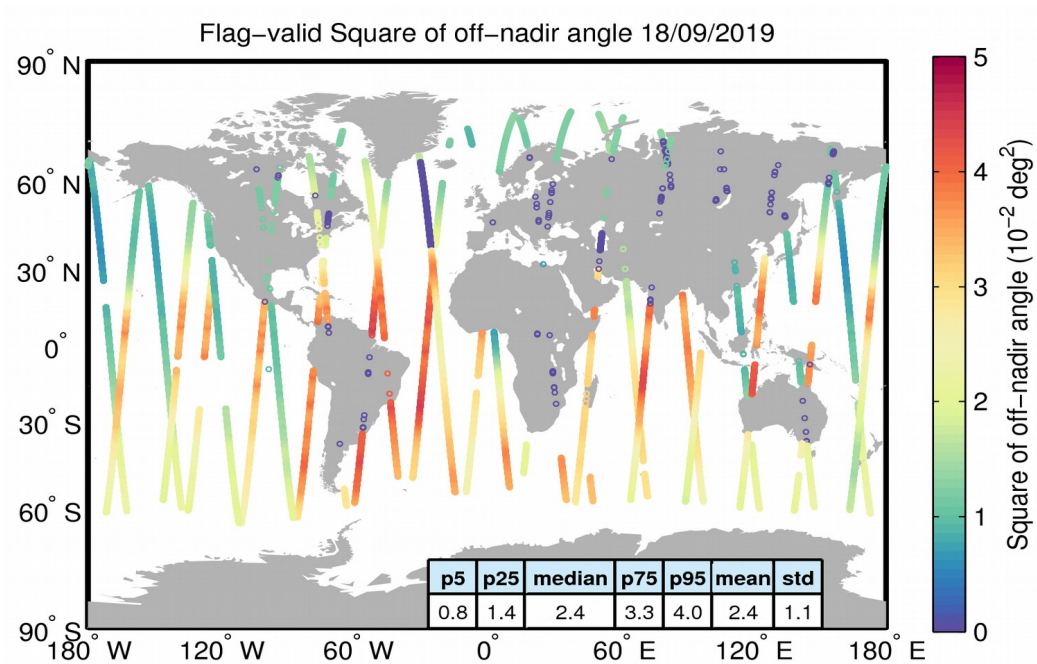
Figure 37. Geographical distribution of flag-valid mispointing data over oceans and lakes for 18/09/2019. The statistical values shown in the table refer to the mispointing in 10^{-2} \text{ deg}^2 and are calculated over all measurements shown in the figure.
