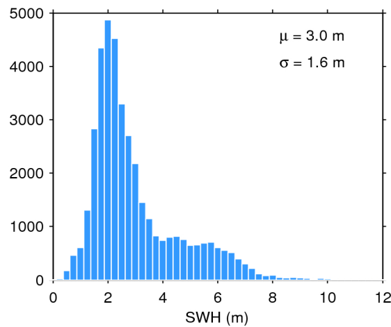
Figure 17. Histogram of flag-valid SWH over oceans and lakes for 18/09/2019. The mean ( \mu ) and standard deviation ( \sigma ) are also shown. Note that values larger than 12 m are excluded from the histogram for the sake of readability but not from the computation of \mu and \sigma .
