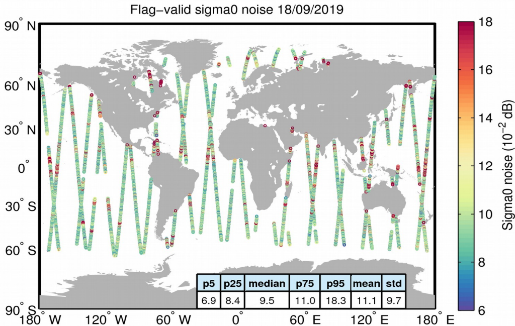
Figure 26. Geographical distribution of flag-valid 20-Hz sigma0 measurement noise over oceans and lakes for 18/09/2019. The statistical values shown in the table refer to the sigma0 noise and are calculated over all measurements shown in the figure.
