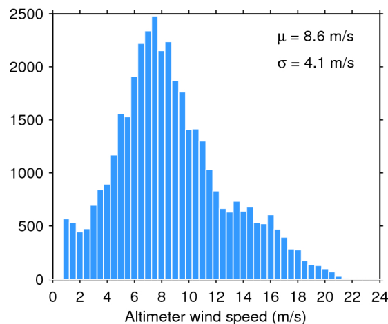
Figure 35. Histogram of science-valid wind over oceans and lakes for 17/09/2019. The mean ( \mu ) and standard deviation ( \sigma ) are also shown. Note that values larger than 24 m/s are excluded from the histogram for the sake of readability but not from the computation of \mu and \sigma .
