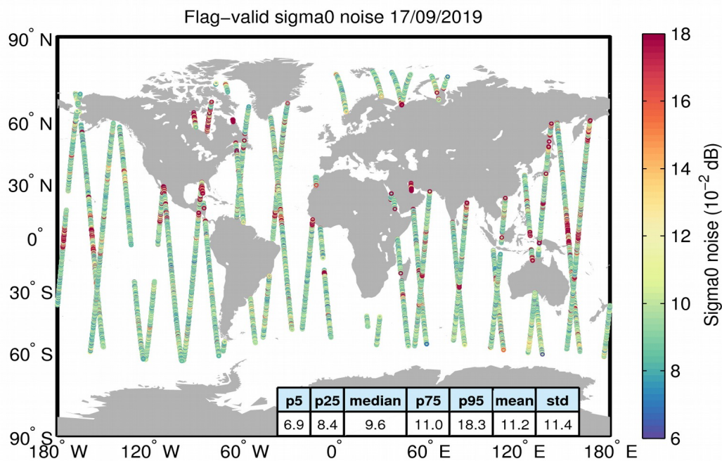
Figure 26. Geographical distribution of flag-valid 20-Hz sigma0 measurement noise over oceans and lakes for 17/09/2019. The statistical values shown in the table refer to the sigma0 noise and are calculated over all measurements shown in the figure.
