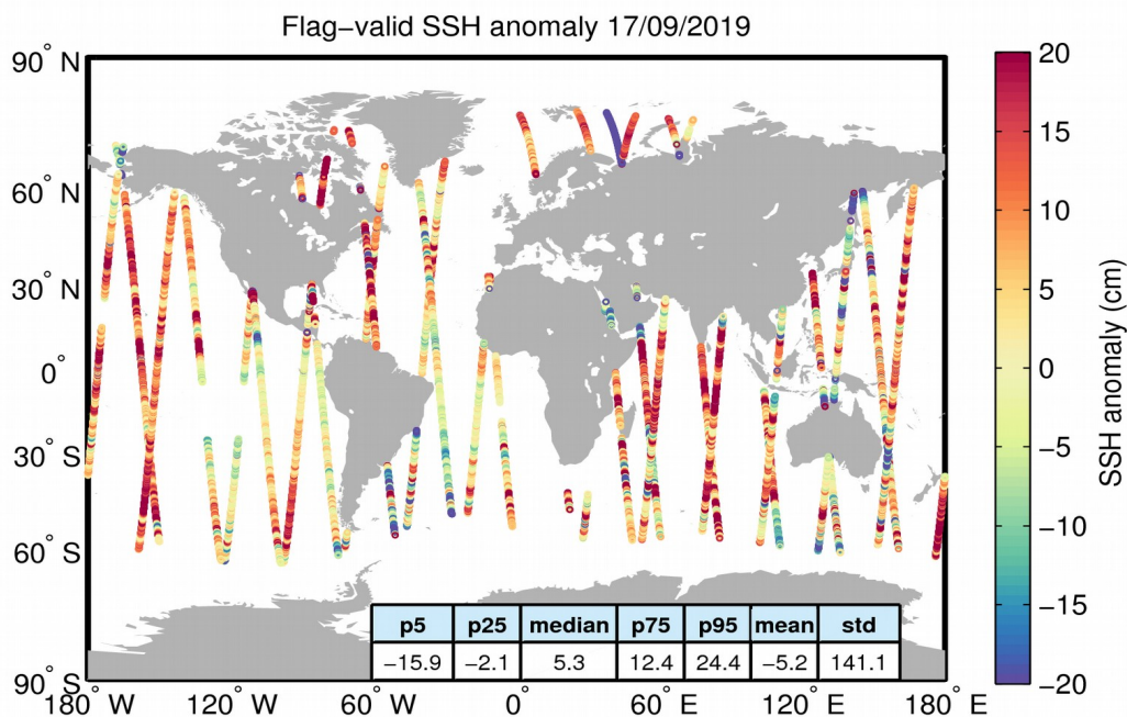
Figure 5. Geographical distribution of flag-valid 1-Hz SSH anomaly data over oceans and lakes for 17/09/2019. The statistical values shown in the table refer to the SSH anomaly in cm and are calculated over all measurements shown in the figure.
