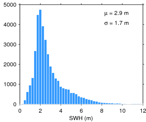
Figure 17. Histogram of flag-valid SWH over oceans and lakes for 17/09/2019. The mean ( \mu ) and standard deviation ( \sigma ) are also shown. Note that values larger than 12 m are excluded from the histogram for the sake of readability but not from the computation of \mu and \sigma .
