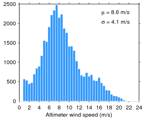
Figure 33. Histogram of flag-valid wind over oceans and lakes for 17/09/2019. The mean ( \mu ) and standard deviation ( \sigma ) are also shown. Note that values larger than 24 m/s are excluded from the histogram for the sake of readability but not from the computation of \mu and \sigma .
