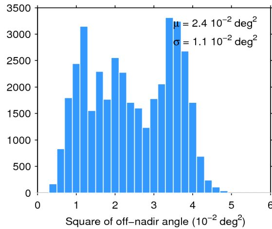
Figure 39. Histogram of flag-valid mispointing over oceans and lakes for 17/09/2019. The mean ( \mu ) and standard deviation ( \sigma ) are also shown. Note that values larger than 6 \cdot 10^{-2} \text{ deg}^2 are excluded from the histogram for the sake of readability but not from the computation of \mu and \sigma .
