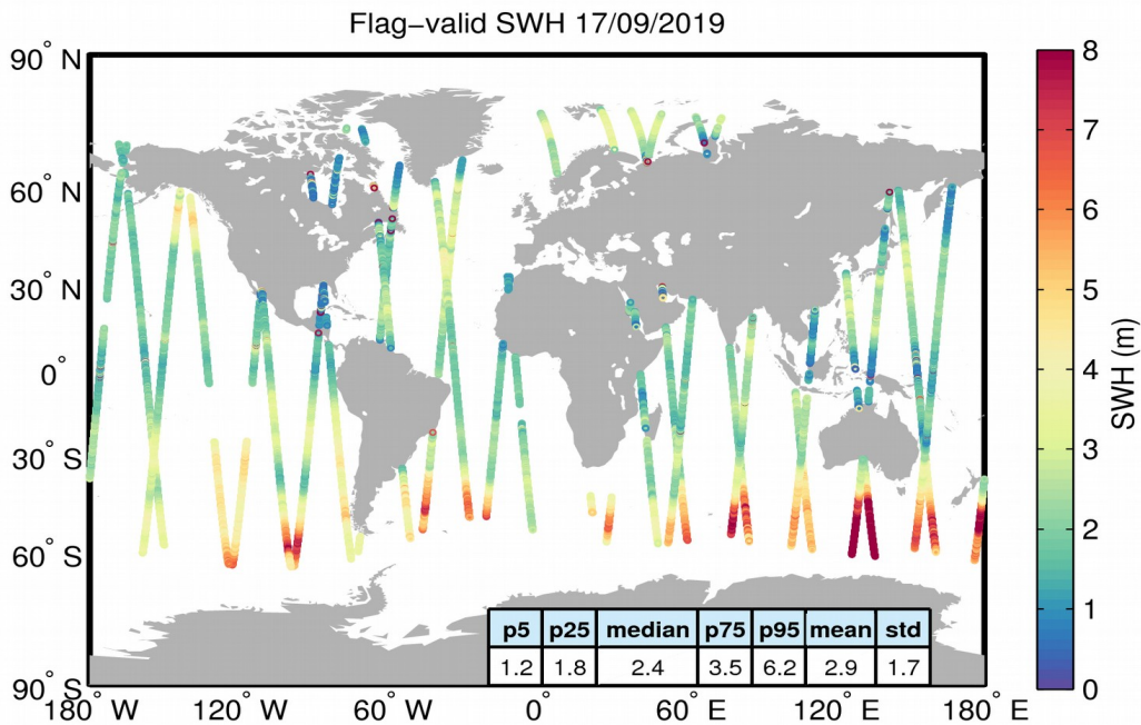
Figure 15. Geographical distribution of flag-valid SWH data over oceans and lakes for 17/09/2019. The statistical values shown in the table refer to the SWH in m and are calculated over all measurements shown in the figure.
