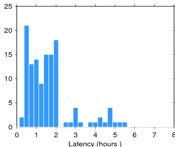
Figure 2. Histogram of the data latency for 17/09/2019. The y-axis denotes the number of files that are made available with a delay of x-hours with respect to the mean time of the records stored in the file.
