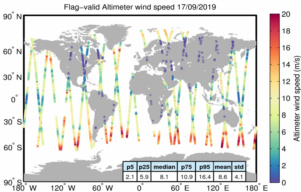
Figure 31. Geographical distribution of flag-valid wind data over oceans and lakes for 17/09/2019. The statistical values shown in the table refer to the wind in m/s and are calculated over all measurements shown in the figure.
