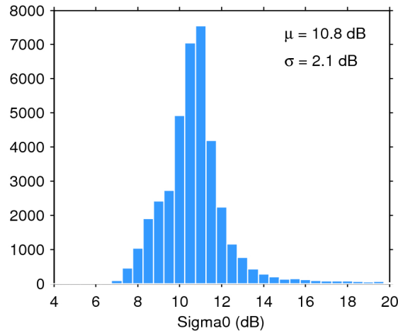
Figure 25. Histogram of flag-valid sigma0 over oceans and lakes for 17/09/2019. The mean ( \mu ) and standard deviation ( \sigma ) are also shown. Note that values outside [4 20] dB are excluded from the histogram for the sake of readability but not from the computation of \mu and \sigma .
