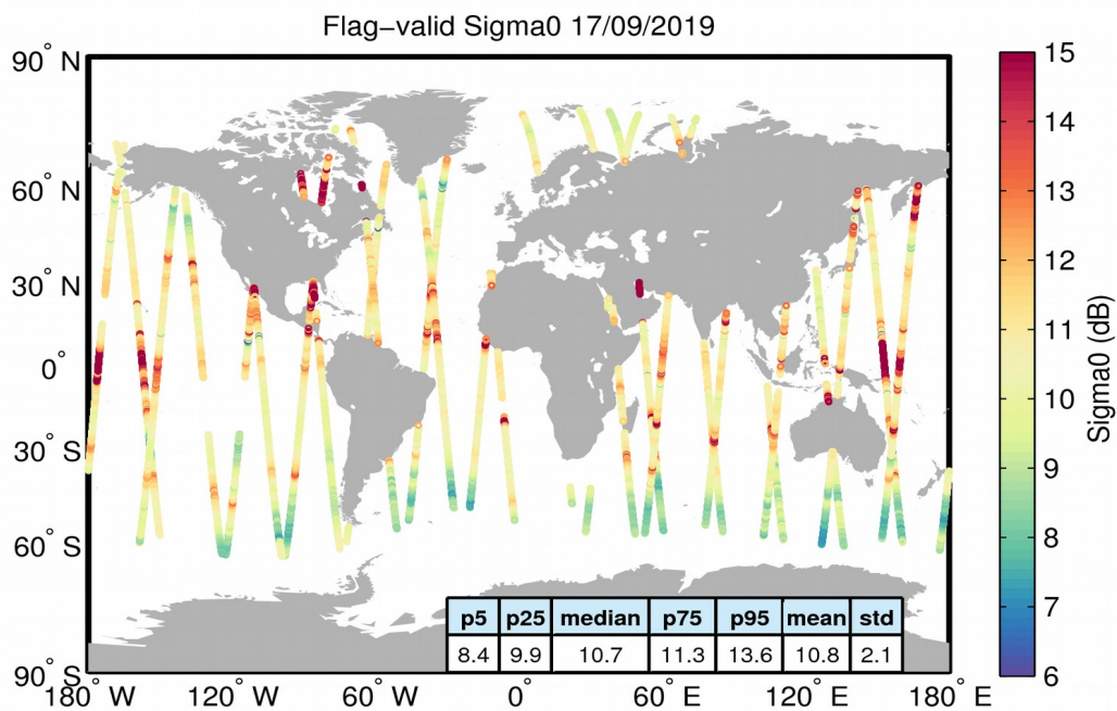
Figure 23. Geographical distribution of flag-valid sigma0 data over oceans and lakes for 17/09/2019. The statistical values shown in the table refer to the sigma0 in dB and are calculated over all measurements shown in the figure.
