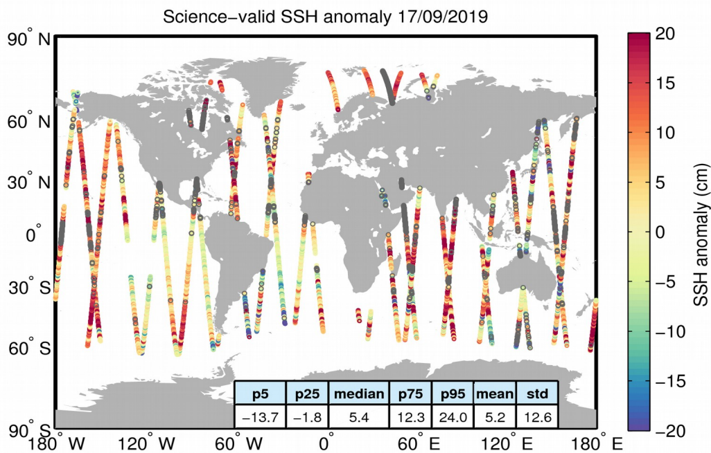
Figure 10. Geographical distribution of science-valid SSH anomaly data over oceans and lakes for 17/09/2019. The statistical values shown in the table refer to the SSH anomaly in cm and are calculated over all measurements shown in the figure. Gray circles denote records that have been rejected based on the editing criteria described in Table 2.
