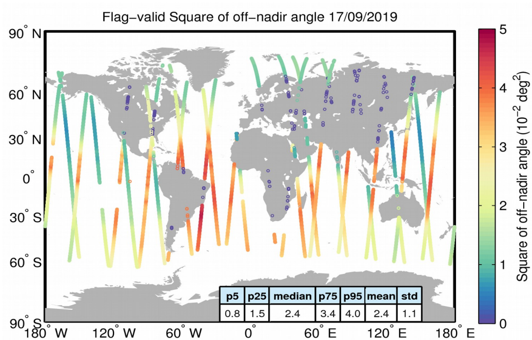
Figure 37. Geographical distribution of flag-valid mispointing data over oceans and lakes for 17/09/2019. The statistical values shown in the table refer to the mispointing in 10^{-2} \text{ deg}^2 and are calculated over all measurements shown in the figure.
