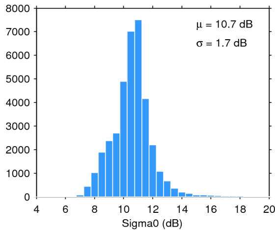
Figure 28. Histogram of science-valid sigma0 over oceans and lakes for 17/09/2019. The mean ( \mu ) and standard deviation ( \sigma ) are also shown. Note that values outside [4 20] dB are excluded from the histogram for the sake of readability but not from the computation of \mu and \sigma .
