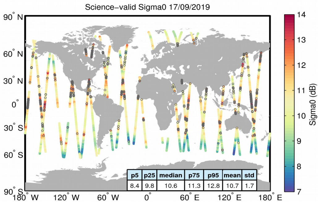
Figure 27. Geographical distribution of science-valid sigma0 data over oceans and lakes for 17/09/2019. The statistical values shown in the table refer to the sigma0 in dB and are calculated over all measurements shown in the figure. Gray circles denote records that have been rejected based on the editing criteria described in Table 4.
