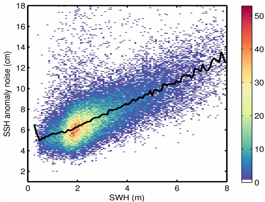
Figure 9. 2D histogram showing flag-valid SSH anomaly noise as a function of SWH for 17/09/2019. The black line denotes the median SSH anomaly noise as a function of SWH.
