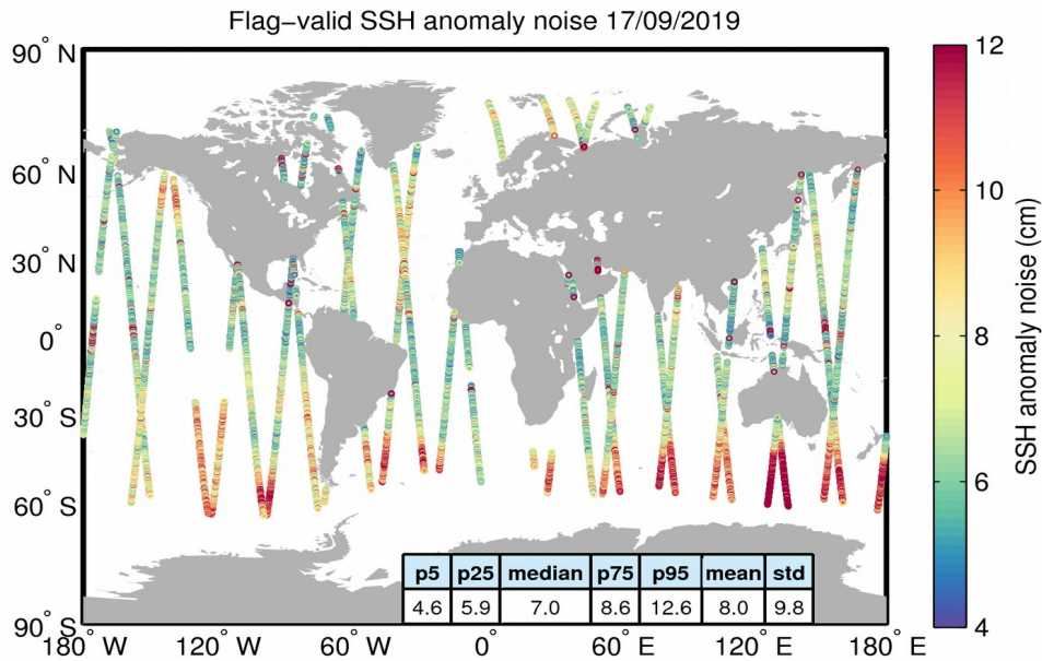
Figure 8. Geographical distribution of flag-valid 20-Hz SSH anomaly measurement noise over oceans and lakes for 17/09/2019. The statistical values shown in the table refer to the SSH anomaly noise and are calculated over all measurements shown in the figure.
