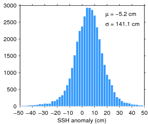
Figure 7. Histogram of flag-valid SSH anomaly over oceans and lakes for 17/09/2019. The mean ( \mu ) and standard deviation ( \sigma ) are also shown. Note that values outside [-50 50] cm are excluded from the histogram for the sake of readability but not from the computation of \mu and \sigma .
