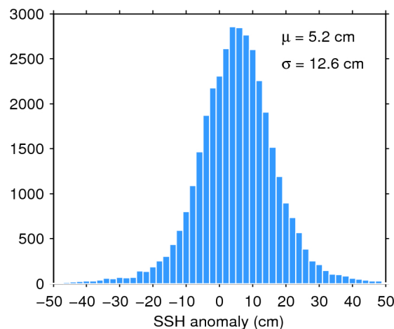
Figure 11. Histogram of science-valid SSH anomaly over oceans and lakes for 17/09/2019. The mean ( \mu ) and standard deviation ( \sigma ) are also shown. Note that values outside [-50 50] cm are excluded from the histogram for the sake of readability but not from the computation of \mu and \sigma .
