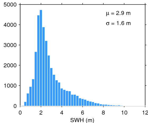
Figure 20. Histogram of science-valid SWH over oceans and lakes for 17/09/2019. The mean ( \mu ) and standard deviation ( \sigma ) are also shown. Note that values larger than 12 m are excluded from the histogram for the sake of readability but not from the computation of \mu and \sigma .
