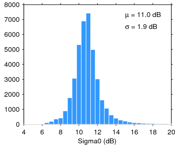
Figure 25. Histogram of flag-valid sigma0 over oceans and lakes for 16/09/2019. The mean ( \mu ) and standard deviation ( \sigma ) are also shown. Note that values outside [4 20] dB are excluded from the histogram for the sake of readability but not from the computation of \mu and \sigma .
