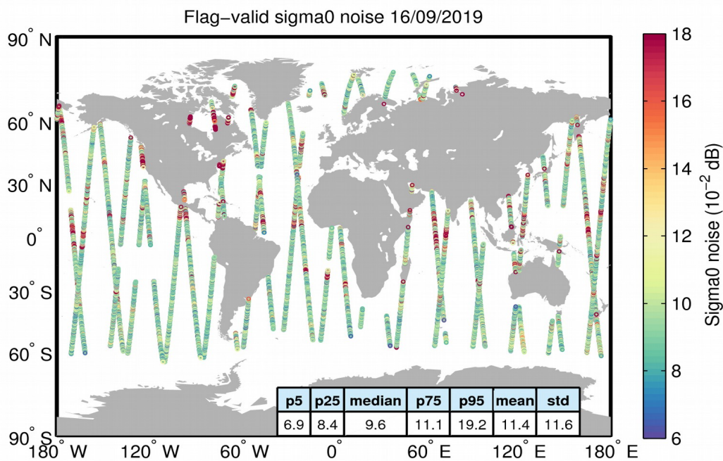
Figure 26. Geographical distribution of flag-valid 20-Hz sigma0 measurement noise over oceans and lakes for 16/09/2019. The statistical values shown in the table refer to the sigma0 noise and are calculated over all measurements shown in the figure.
