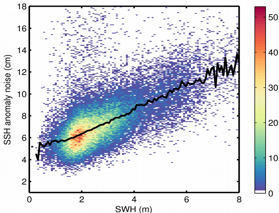
Figure 9. 2D histogram showing flag-valid SSH anomaly noise as a function of SWH for 16/09/2019. The black line denotes the median SSH anomaly noise as a function of SWH.
