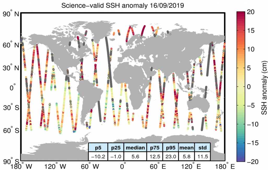
Figure 10. Geographical distribution of science-valid SSH anomaly data over oceans and lakes for 16/09/2019. The statistical values shown in the table refer to the SSH anomaly in cm and are calculated over all measurements shown in the figure. Gray circles denote records that have been rejected based on the editing criteria described in Table 2.
