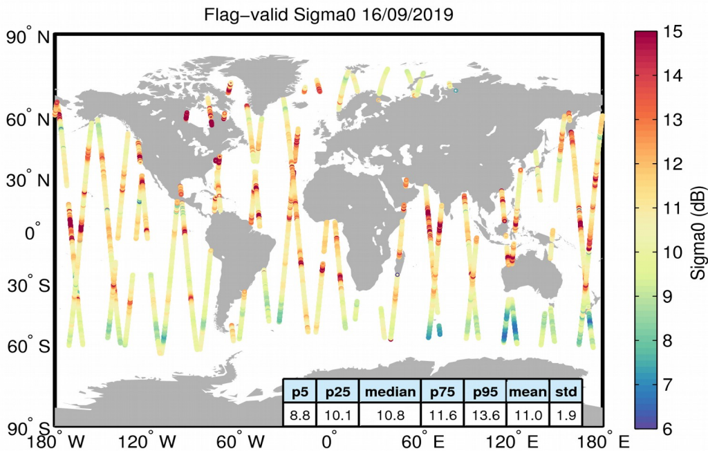
Figure 23. Geographical distribution of flag-valid sigma0 data over oceans and lakes for 16/09/2019. The statistical values shown in the table refer to the sigma0 in dB and are calculated over all measurements shown in the figure.
