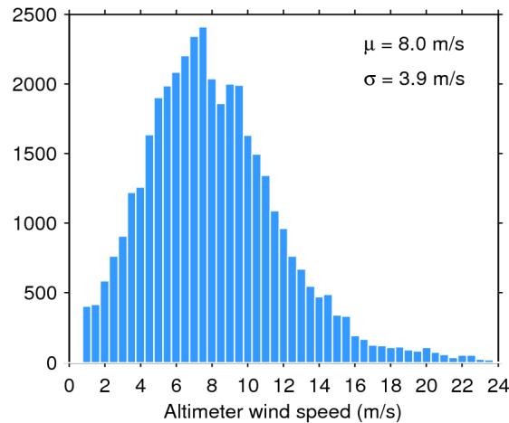
Figure 33. Histogram of flag-valid wind over oceans and lakes for 16/09/2019. The mean ( \mu ) and standard deviation ( \sigma ) are also shown. Note that values larger than 24 m/s are excluded from the histogram for the sake of readability but not from the computation of \mu and \sigma .
