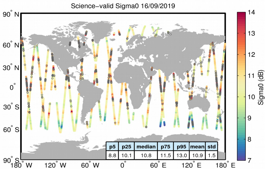
Figure 27. Geographical distribution of science-valid sigma0 data over oceans and lakes for 16/09/2019. The statistical values shown in the table refer to the sigma0 in dB and are calculated over all measurements shown in the figure. Gray circles denote records that have been rejected based on the editing criteria described in Table 4.
