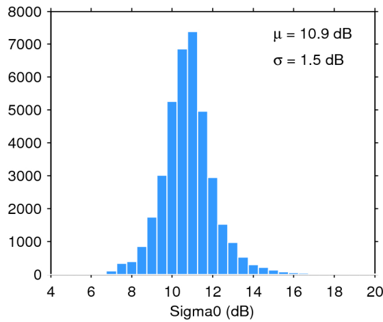
Figure 28. Histogram of science-valid sigma0 over oceans and lakes for 16/09/2019. The mean ( \mu ) and standard deviation ( \sigma ) are also shown. Note that values outside [4 20] dB are excluded from the histogram for the sake of readability but not from the computation of \mu and \sigma .
