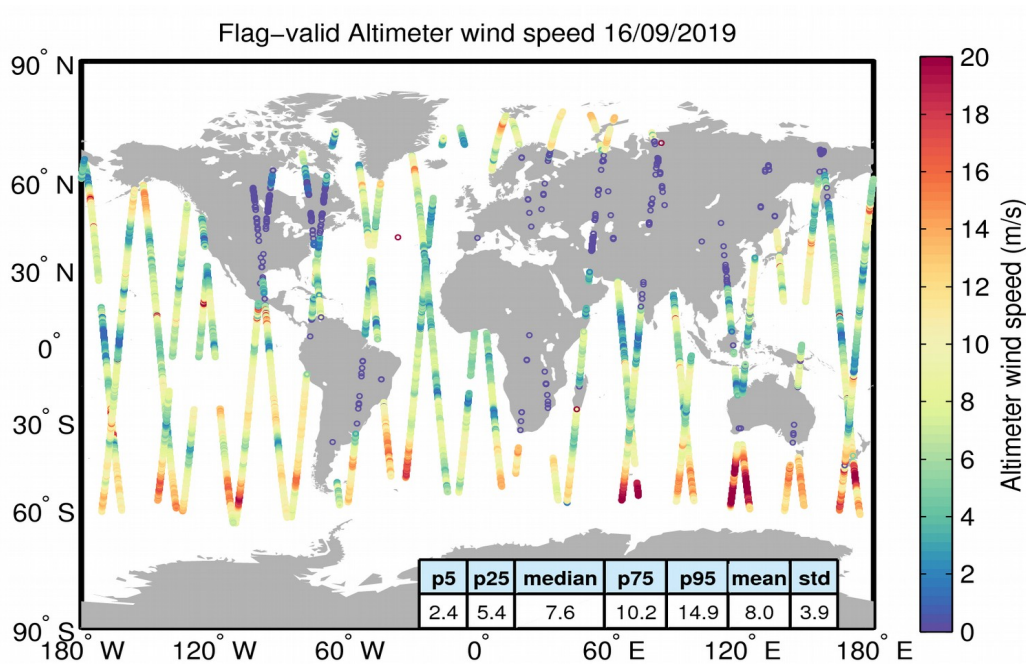
Figure 31. Geographical distribution of flag-valid wind data over oceans and lakes for 16/09/2019. The statistical values shown in the table refer to the wind in m/s and are calculated over all measurements shown in the figure.
