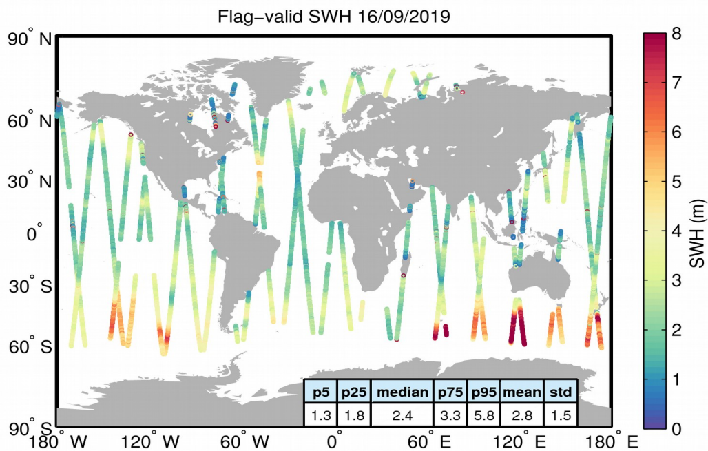
Figure 15. Geographical distribution of flag-valid SWH data over oceans and lakes for 16/09/2019. The statistical values shown in the table refer to the SWH in m and are calculated over all measurements shown in the figure.
