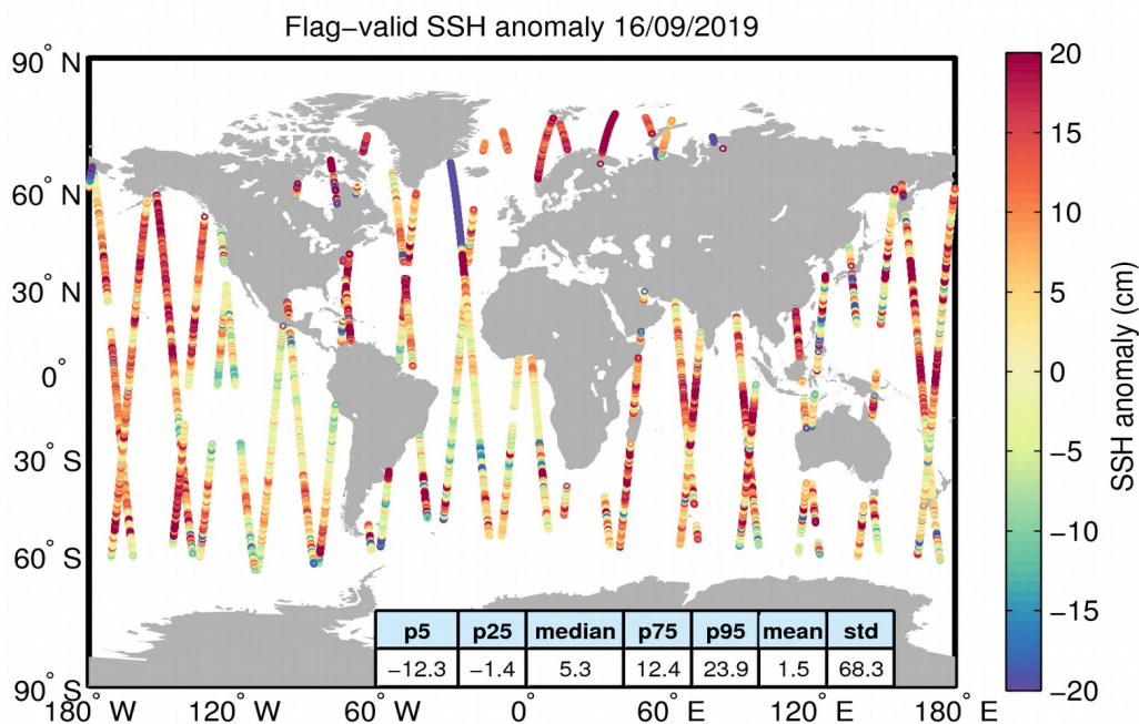
Figure 5. Geographical distribution of flag-valid 1-Hz SSH anomaly data over oceans and lakes for 16/09/2019. The statistical values shown in the table refer to the SSH anomaly in cm and are calculated over all measurements shown in the figure.
