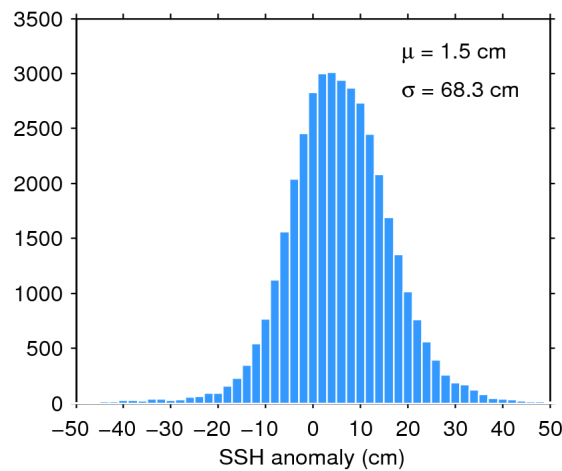
Figure 7. Histogram of flag-valid SSH anomaly over oceans and lakes for 16/09/2019. The mean ( \mu ) and standard deviation ( \sigma ) are also shown. Note that values outside [-50\ 50] cm are excluded from the histogram for the sake of readability but not from the computation of \mu and \sigma .
