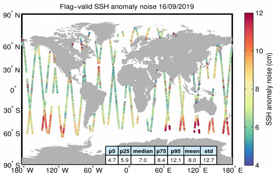
Figure 8. Geographical distribution of flag-valid 20-Hz SSH anomaly measurement noise over oceans and lakes for 16/09/2019. The statistical values shown in the table refer to the SSH anomaly noise and are calculated over all measurements shown in the figure.
