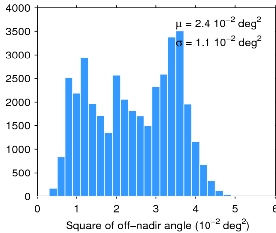
Figure 39. Histogram of flag-valid mispointing over oceans and lakes for 16/09/2019. The mean ( \mu ) and standard deviation ( \sigma ) are also shown. Note that values larger than 6 \cdot 10^{-2} \text{ deg}^2 are excluded from the histogram for the sake of readability but not from the computation of \mu and \sigma .
