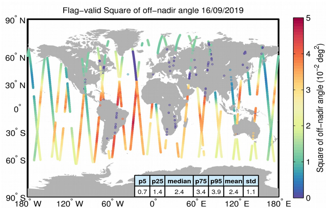
Figure 37. Geographical distribution of flag-valid mispointing data over oceans and lakes for 16/09/2019. The statistical values shown in the table refer to the mispointing in 10^{-2} \text{ deg}^2 and are calculated over all measurements shown in the figure.
