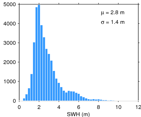
Figure 20. Histogram of science-valid SWH over oceans and lakes for 16/09/2019. The mean ( \mu ) and standard deviation ( \sigma ) are also shown. Note that values larger than 12 m are excluded from the histogram for the sake of readability but not from the computation of \mu and \sigma .
