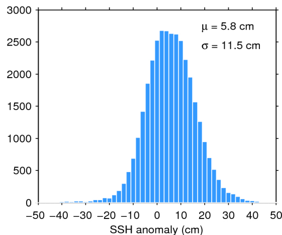
Figure 11. Histogram of science-valid SSH anomaly over oceans and lakes for 16/09/2019. The mean ( \mu ) and standard deviation ( \sigma ) are also shown. Note that values outside [-50 50] cm are excluded from the histogram for the sake of readability but not from the computation of \mu and \sigma .
