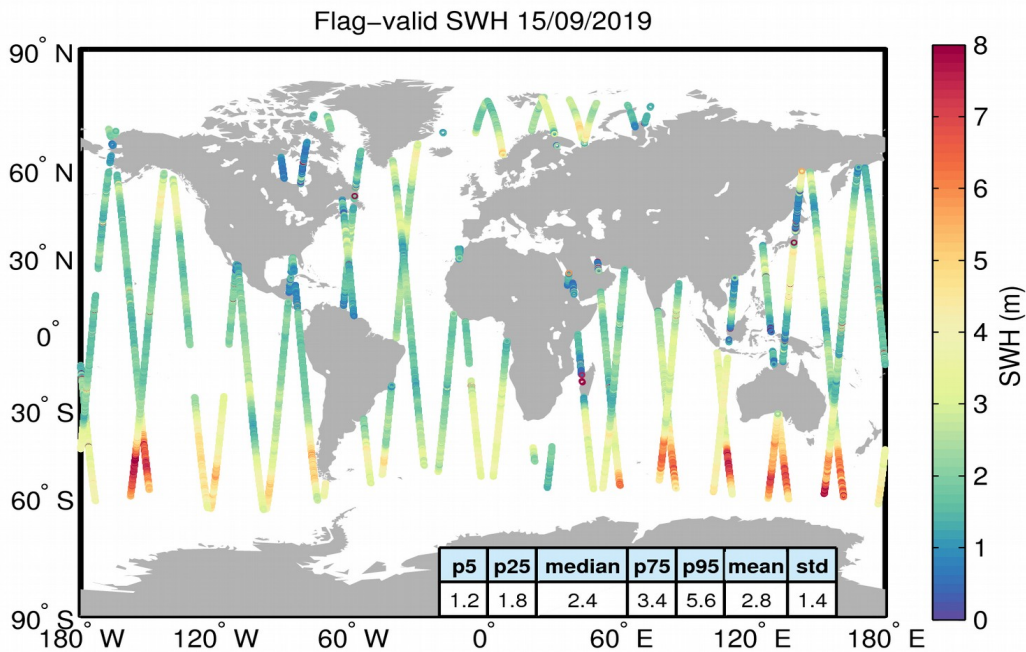
Figure 15. Geographical distribution of flag-valid SWH data over oceans and lakes for 15/09/2019. The statistical values shown in the table refer to the SWH in m and are calculated over all measurements shown in the figure.
