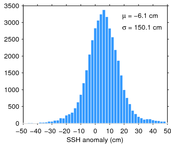
Figure 7. Histogram of flag-valid SSH anomaly over oceans and lakes for 15/09/2019. The mean ( \mu ) and standard deviation ( \sigma ) are also shown. Note that values outside [-50\ 50] cm are excluded from the histogram for the sake of readability but not from the computation of \mu and \sigma .
