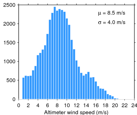
Figure 35. Histogram of science-valid wind over oceans and lakes for 15/09/2019. The mean ( \mu ) and standard deviation ( \sigma ) are also shown. Note that values larger than 24 m/s are excluded from the histogram for the sake of readability but not from the computation of \mu and \sigma .
