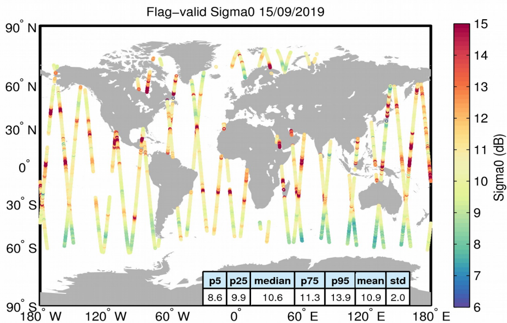
Figure 23. Geographical distribution of flag-valid sigma0 data over oceans and lakes for 15/09/2019. The statistical values shown in the table refer to the sigma0 in dB and are calculated over all measurements shown in the figure.
