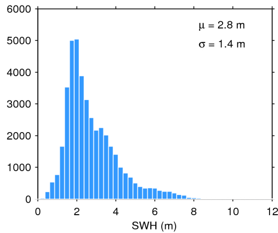
Figure 17. Histogram of flag-valid SWH over oceans and lakes for 15/09/2019. The mean ( \mu ) and standard deviation ( \sigma ) are also shown. Note that values larger than 12 m are excluded from the histogram for the sake of readability but not from the computation of \mu and \sigma .
