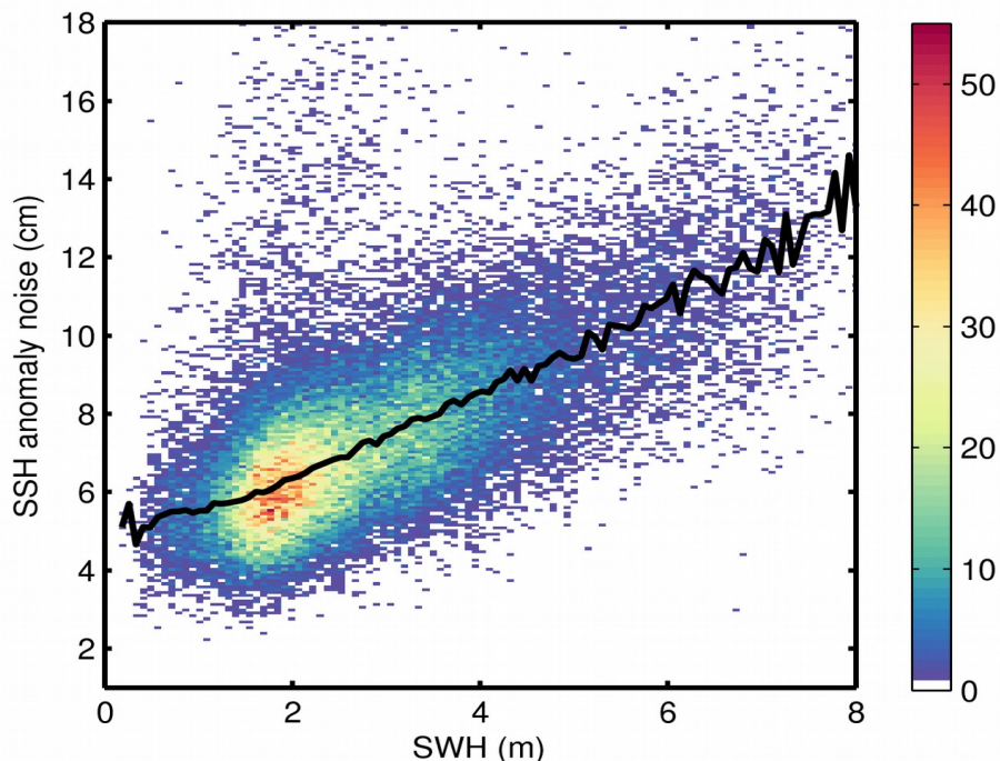
Figure 9. 2D histogram showing flag-valid SSH anomaly noise as a function of SWH for 15/09/2019. The black line denotes the median SSH anomaly noise as a function of SWH.
