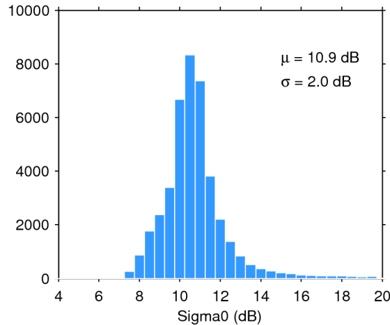
Figure 25. Histogram of flag-valid sigma0 over oceans and lakes for 15/09/2019. The mean ( \mu ) and standard deviation ( \sigma ) are also shown. Note that values outside [4 20] dB are excluded from the histogram for the sake of readability but not from the computation of \mu and \sigma .
