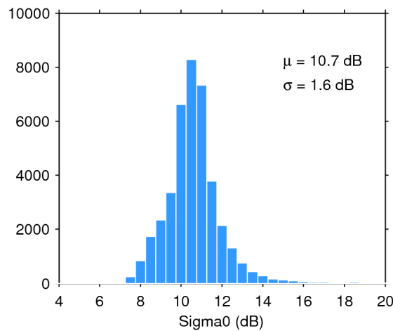
Figure 28. Histogram of science-valid sigma0 over oceans and lakes for 15/09/2019. The mean ( \mu ) and standard deviation ( \sigma ) are also shown. Note that values outside [4 20] dB are excluded from the histogram for the sake of readability but not from the computation of \mu and \sigma .
