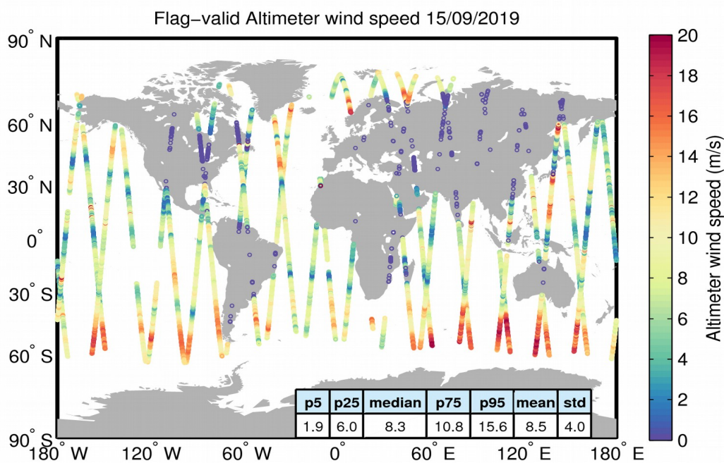
Figure 31. Geographical distribution of flag-valid wind data over oceans and lakes for 15/09/2019. The statistical values shown in the table refer to the wind in m/s and are calculated over all measurements shown in the figure.
