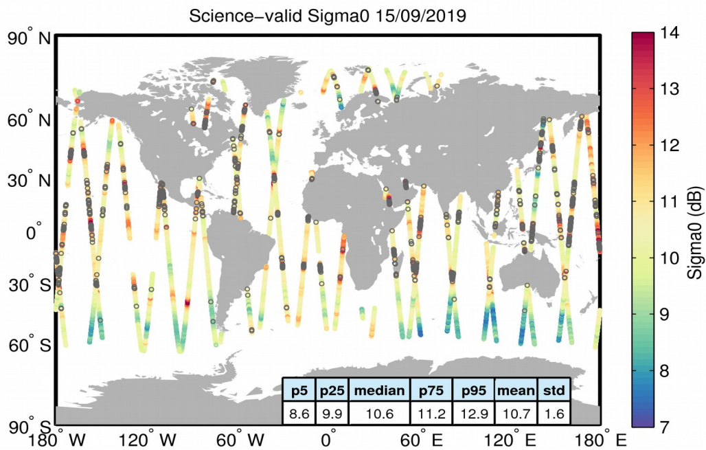
Figure 27. Geographical distribution of science-valid sigma0 data over oceans and lakes for 15/09/2019. The statistical values shown in the table refer to the sigma0 in dB and are calculated over all measurements shown in the figure. Gray circles denote records that have been rejected based on the editing criteria described in Table 4.
