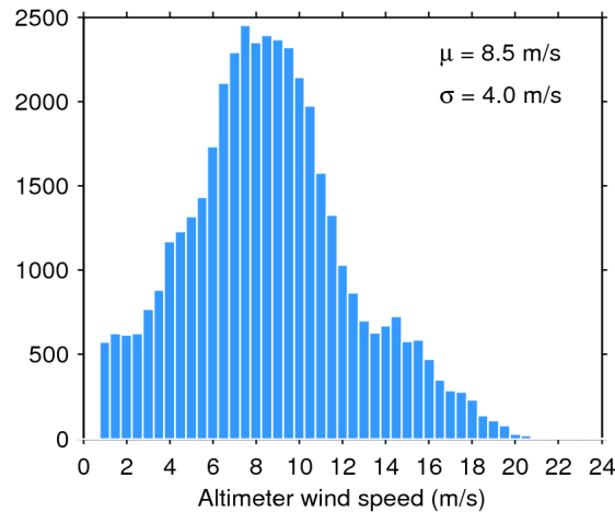
Figure 33. Histogram of flag-valid wind over oceans and lakes for 15/09/2019. The mean ( \mu ) and standard deviation ( \sigma ) are also shown. Note that values larger than 24 m/s are excluded from the histogram for the sake of readability but not from the computation of \mu and \sigma .
