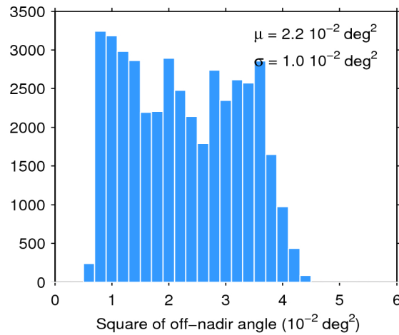
Figure 39. Histogram of flag-valid mispointing over oceans and lakes for 15/09/2019. The mean ( \mu ) and standard deviation ( \sigma ) are also shown. Note that values larger than 6 \cdot 10^{-2} \text{ deg}^2 are excluded from the histogram for the sake of readability but not from the computation of \mu and \sigma .
