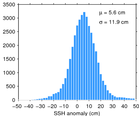
Figure 11. Histogram of science-valid SSH anomaly over oceans and lakes for 15/09/2019. The mean ( \mu ) and standard deviation ( \sigma ) are also shown. Note that values outside [-50 50] cm are excluded from the histogram for the sake of readability but not from the computation of \mu and \sigma .
