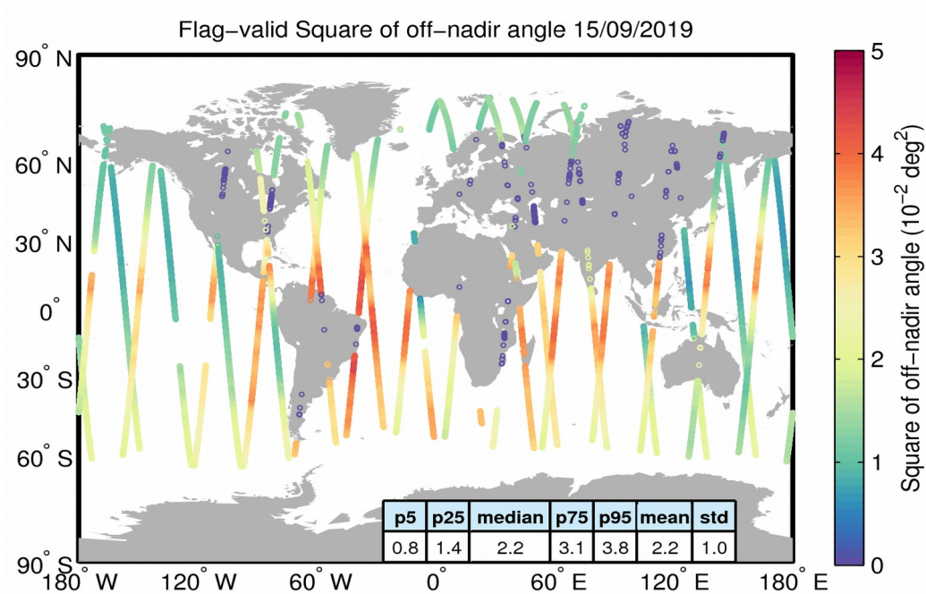
Figure 37. Geographical distribution of flag-valid mispointing data over oceans and lakes for 15/09/2019. The statistical values shown in the table refer to the mispointing in 10^{-2} \text{ deg}^2 and are calculated over all measurements shown in the figure.
