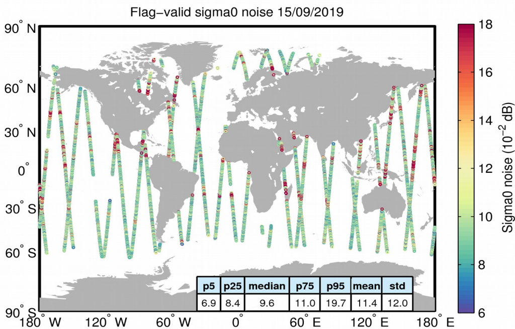
Figure 26. Geographical distribution of flag-valid 20-Hz sigma0 measurement noise over oceans and lakes for 15/09/2019. The statistical values shown in the table refer to the sigma0 noise and are calculated over all measurements shown in the figure.
