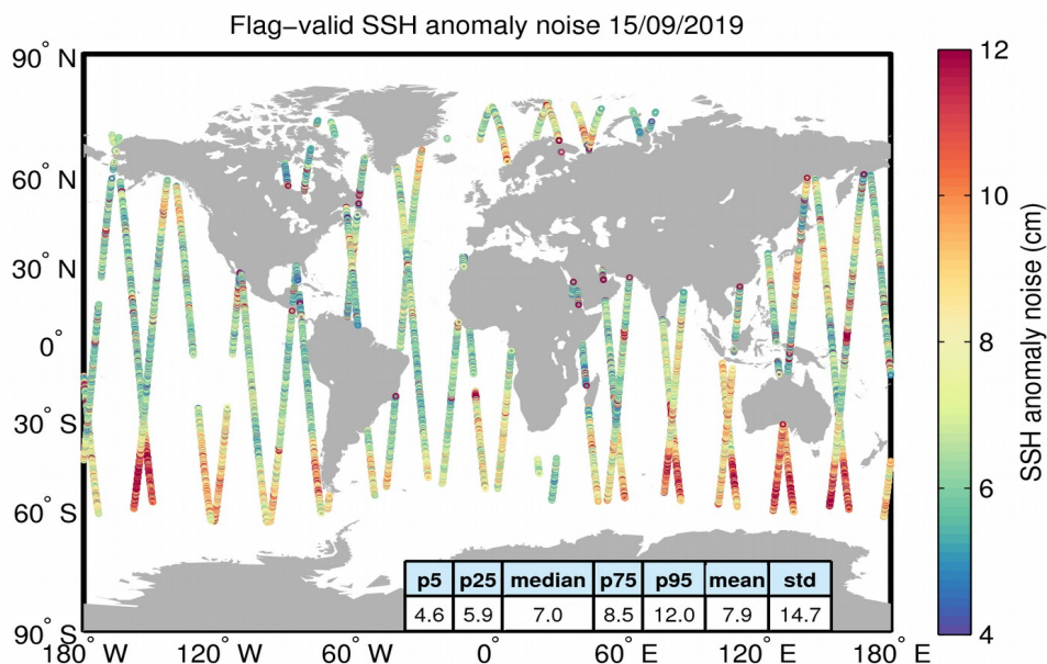
Figure 8. Geographical distribution of flag-valid 20-Hz SSH anomaly measurement noise over oceans and lakes for 15/09/2019. The statistical values shown in the table refer to the SSH anomaly noise and are calculated over all measurements shown in the figure.
