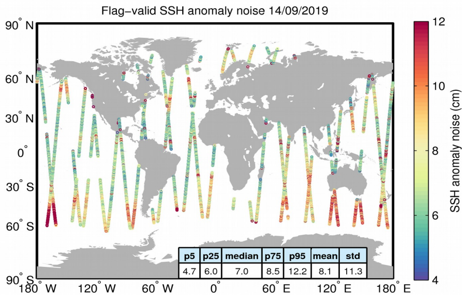
Figure 8. Geographical distribution of flag-valid 20-Hz SSH anomaly measurement noise over oceans and lakes for 14/09/2019. The statistical values shown in the table refer to the SSH anomaly noise and are calculated over all measurements shown in the figure.
