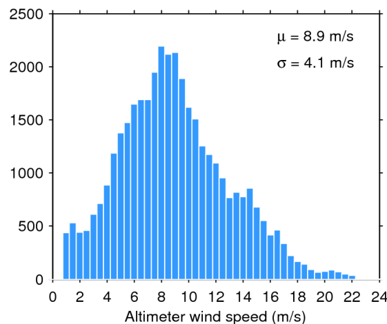
Figure 35. Histogram of science-valid wind over oceans and lakes for 14/09/2019. The mean ( \mu ) and standard deviation ( \sigma ) are also shown. Note that values larger than 24 m/s are excluded from the histogram for the sake of readability but not from the computation of \mu and \sigma .
