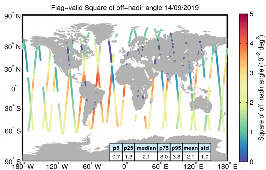
Figure 37. Geographical distribution of flag-valid mispointing data over oceans and lakes for 14/09/2019. The statistical values shown in the table refer to the mispointing in 10^{-2} \text{ deg}^2 and are calculated over all measurements shown in the figure.
