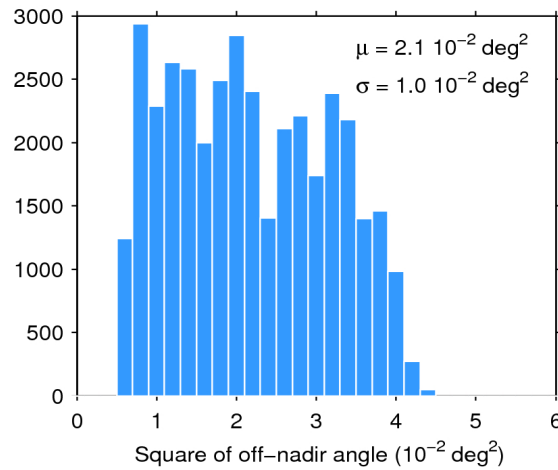
Figure 39. Histogram of flag-valid mispointing over oceans and lakes for 14/09/2019. The mean ( \mu ) and standard deviation ( \sigma ) are also shown. Note that values larger than 6 \cdot 10^{-2} \text{ deg}^2 are excluded from the histogram for the sake of readability but not from the computation of \mu and \sigma .
