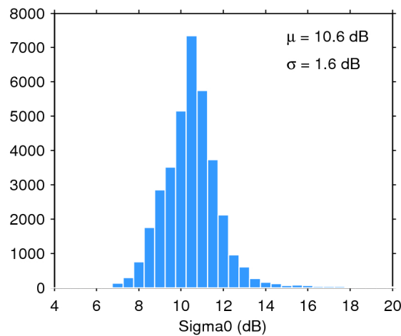
Figure 28. Histogram of science-valid sigma0 over oceans and lakes for 14/09/2019. The mean ( \mu ) and standard deviation ( \sigma ) are also shown. Note that values outside [4 20] dB are excluded from the histogram for the sake of readability but not from the computation of \mu and \sigma .
