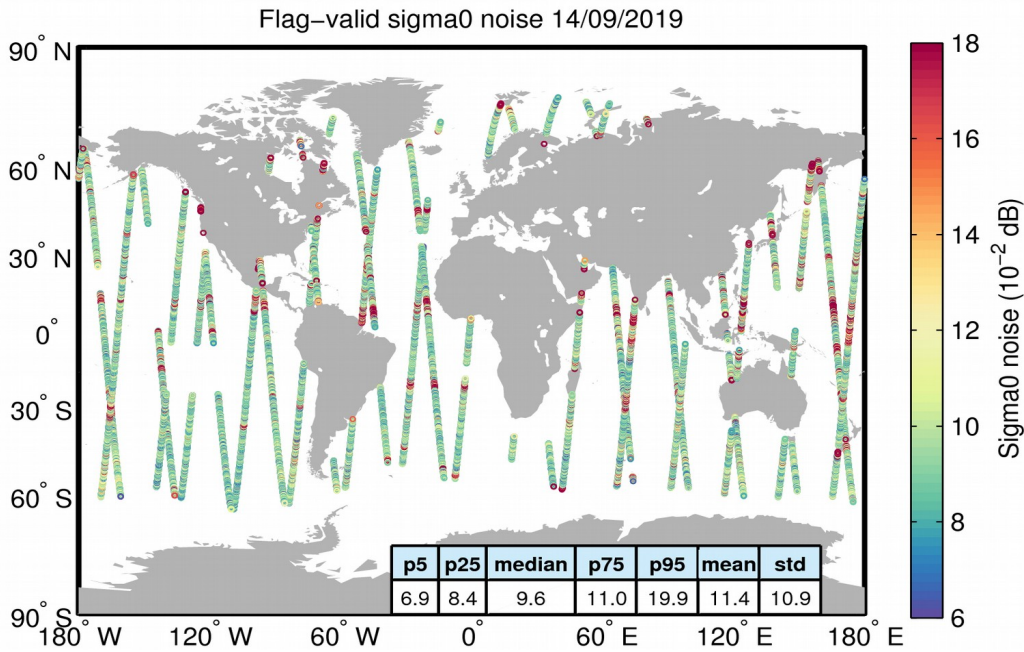
Figure 26. Geographical distribution of flag-valid 20-Hz sigma0 measurement noise over oceans and lakes for 14/09/2019. The statistical values shown in the table refer to the sigma0 noise and are calculated over all measurements shown in the figure.
