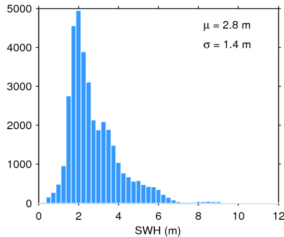
Figure 20. Histogram of science-valid SWH over oceans and lakes for 14/09/2019. The mean ( \mu ) and standard deviation ( \sigma ) are also shown. Note that values larger than 12 m are excluded from the histogram for the sake of readability but not from the computation of \mu and \sigma .
