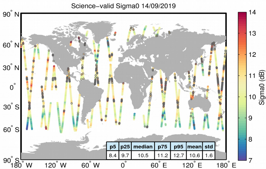
Figure 27. Geographical distribution of science-valid sigma0 data over oceans and lakes for 14/09/2019. The statistical values shown in the table refer to the sigma0 in dB and are calculated over all measurements shown in the figure. Gray circles denote records that have been rejected based on the editing criteria described in Table 4.
