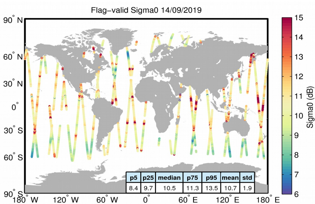
Figure 23. Geographical distribution of flag-valid sigma0 data over oceans and lakes for 14/09/2019. The statistical values shown in the table refer to the sigma0 in dB and are calculated over all measurements shown in the figure.
