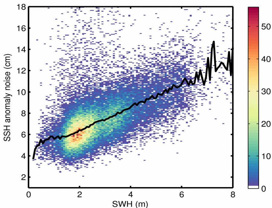
Figure 9. 2D histogram showing flag-valid SSH anomaly noise as a function of SWH for 14/09/2019. The black line denotes the median SSH anomaly noise as a function of SWH.
