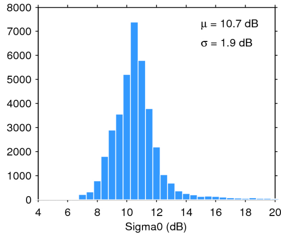
Figure 25. Histogram of flag-valid sigma0 over oceans and lakes for 14/09/2019. The mean ( \mu ) and standard deviation ( \sigma ) are also shown. Note that values outside [4 20] dB are excluded from the histogram for the sake of readability but not from the computation of \mu and \sigma .
