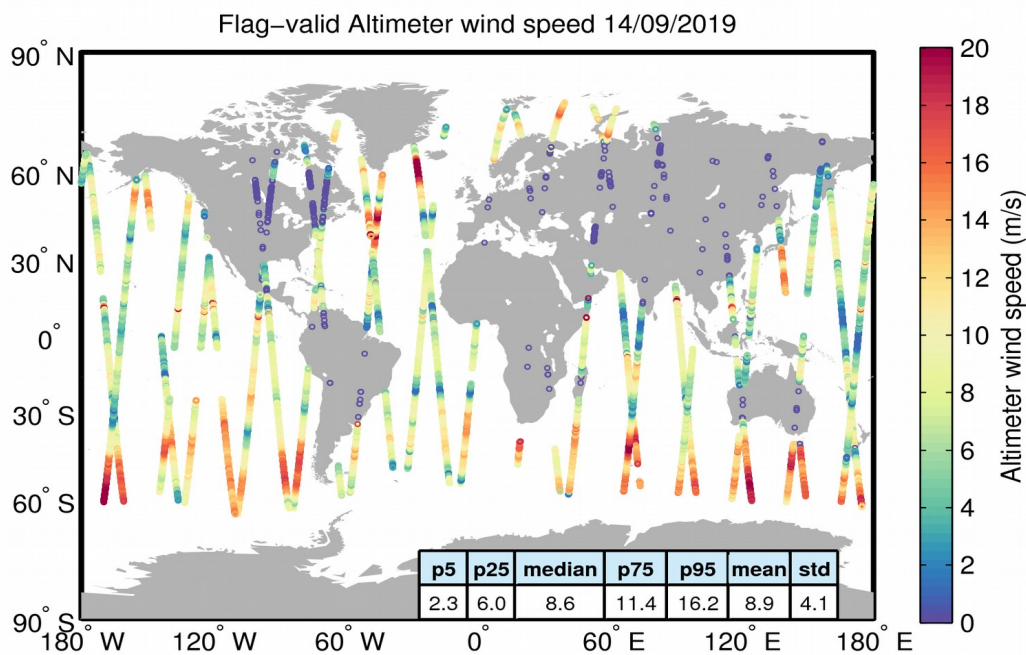
Figure 31. Geographical distribution of flag-valid wind data over oceans and lakes for 14/09/2019. The statistical values shown in the table refer to the wind in m/s and are calculated over all measurements shown in the figure.
