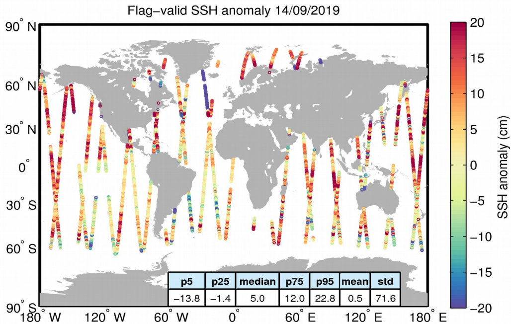
Figure 5. Geographical distribution of flag-valid 1-Hz SSH anomaly data over oceans and lakes for 14/09/2019. The statistical values shown in the table refer to the SSH anomaly in cm and are calculated over all measurements shown in the figure.
