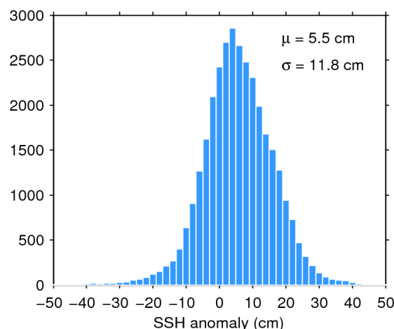
Figure 11. Histogram of science-valid SSH anomaly over oceans and lakes for 14/09/2019. The mean ( \mu ) and standard deviation ( \sigma ) are also shown. Note that values outside [-50 50] cm are excluded from the histogram for the sake of readability but not from the computation of \mu and \sigma .
