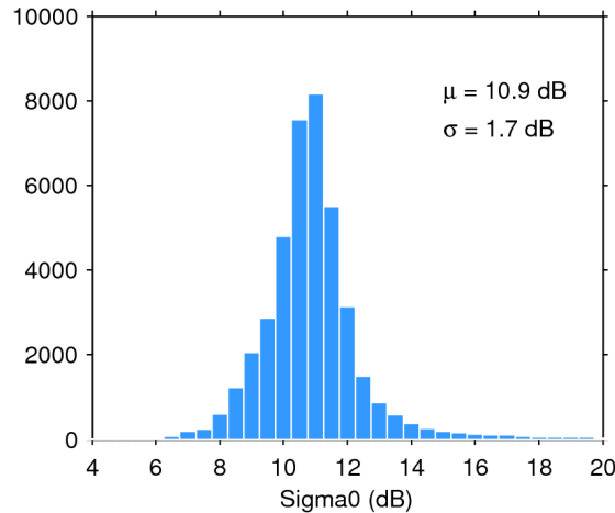
Figure 25. Histogram of flag-valid sigma0 over oceans and lakes for 13/09/2019. The mean ( \mu ) and standard deviation ( \sigma ) are also shown. Note that values outside [4 20] dB are excluded from the histogram for the sake of readability but not from the computation of \mu and \sigma .
