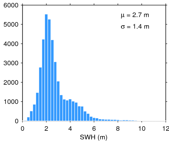
Figure 20. Histogram of science-valid SWH over oceans and lakes for 13/09/2019. The mean ( \mu ) and standard deviation ( \sigma ) are also shown. Note that values larger than 12 m are excluded from the histogram for the sake of readability but not from the computation of \mu and \sigma .
