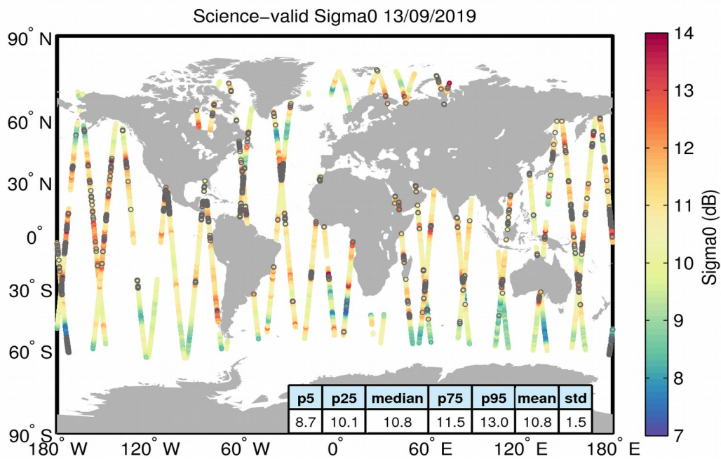
Figure 27. Geographical distribution of science-valid sigma0 data over oceans and lakes for 13/09/2019. The statistical values shown in the table refer to the sigma0 in dB and are calculated over all measurements shown in the figure. Gray circles denote records that have been rejected based on the editing criteria described in Table 4.
