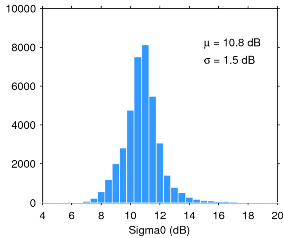
Figure 28. Histogram of science-valid sigma0 over oceans and lakes for 13/09/2019. The mean ( \mu ) and standard deviation ( \sigma ) are also shown. Note that values outside [4 20] dB are excluded from the histogram for the sake of readability but not from the computation of \mu and \sigma .
