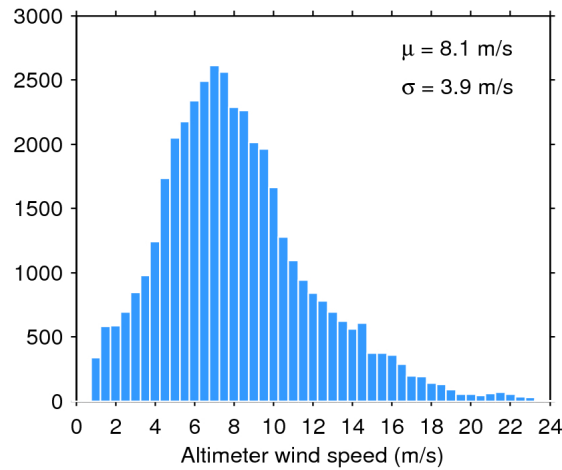
Figure 33. Histogram of flag-valid wind over oceans and lakes for 13/09/2019. The mean ( \mu ) and standard deviation ( \sigma ) are also shown. Note that values larger than 24 m/s are excluded from the histogram for the sake of readability but not from the computation of \mu and \sigma .
