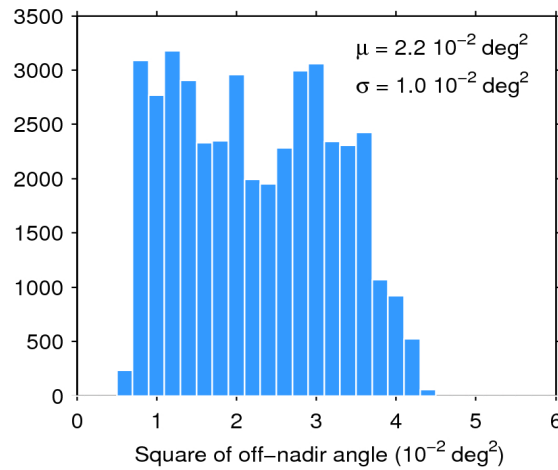
Figure 39. Histogram of flag-valid mispointing over oceans and lakes for 13/09/2019. The mean ( \mu ) and standard deviation ( \sigma ) are also shown. Note that values larger than 6 \cdot 10^{-2} \text{ deg}^2 are excluded from the histogram for the sake of readability but not from the computation of \mu and \sigma .
