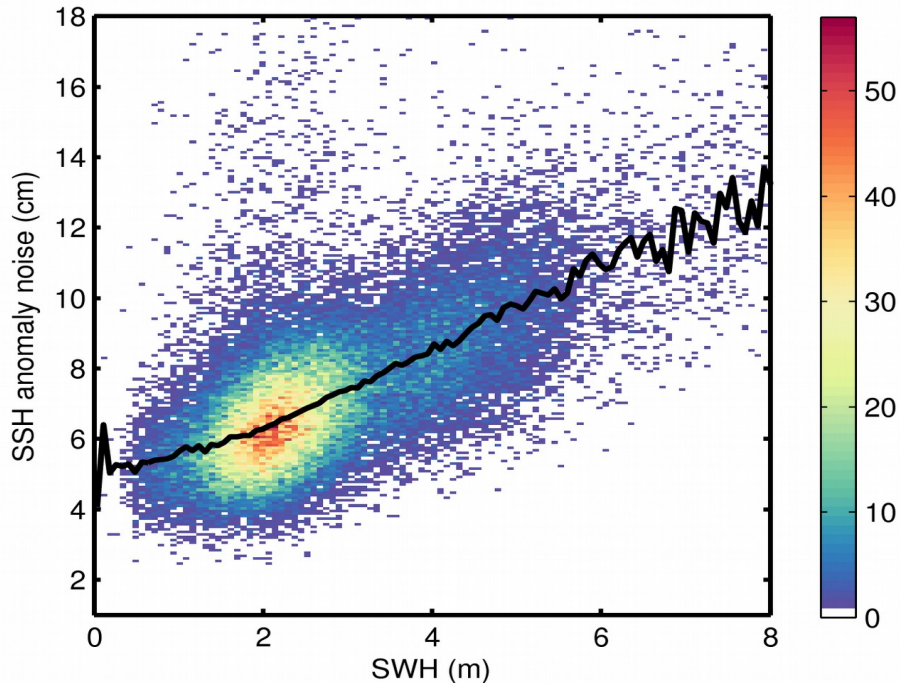
Figure 9. 2D histogram showing flag-valid SSH anomaly noise as a function of SWH for 13/09/2019. The black line denotes the median SSH anomaly noise as a function of SWH.
