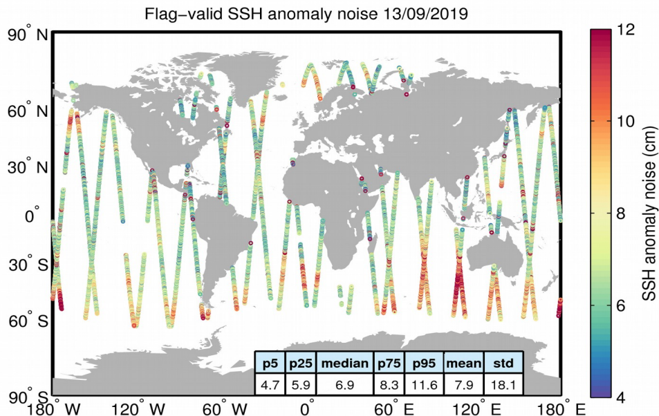
Figure 8. Geographical distribution of flag-valid 20-Hz SSH anomaly measurement noise over oceans and lakes for 13/09/2019. The statistical values shown in the table refer to the SSH anomaly noise and are calculated over all measurements shown in the figure.
