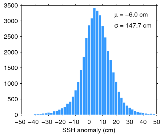
Figure 7. Histogram of flag-valid SSH anomaly over oceans and lakes for 13/09/2019. The mean ( \mu ) and standard deviation ( \sigma ) are also shown. Note that values outside [-50 50] cm are excluded from the histogram for the sake of readability but not from the computation of \mu and \sigma .
