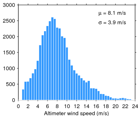
Figure 35. Histogram of science-valid wind over oceans and lakes for 13/09/2019. The mean ( \mu ) and standard deviation ( \sigma ) are also shown. Note that values larger than 24 m/s are excluded from the histogram for the sake of readability but not from the computation of \mu and \sigma .
