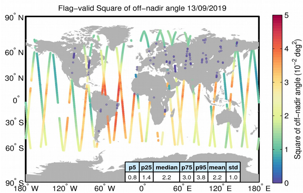
Figure 37. Geographical distribution of flag-valid mispointing data over oceans and lakes for 13/09/2019. The statistical values shown in the table refer to the mispointing in 10^{-2} \text{ deg}^2 and are calculated over all measurements shown in the figure.
