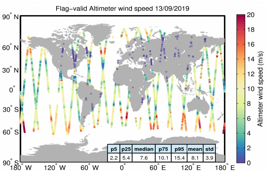
Figure 31. Geographical distribution of flag-valid wind data over oceans and lakes for 13/09/2019. The statistical values shown in the table refer to the wind in m/s and are calculated over all measurements shown in the figure.
