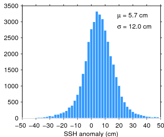
Figure 11. Histogram of science-valid SSH anomaly over oceans and lakes for 13/09/2019. The mean ( \mu ) and standard deviation ( \sigma ) are also shown. Note that values outside [-50 50] cm are excluded from the histogram for the sake of readability but not from the computation of \mu and \sigma .
