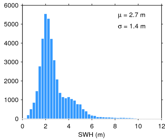
Figure 17. Histogram of flag-valid SWH over oceans and lakes for 13/09/2019. The mean ( \mu ) and standard deviation ( \sigma ) are also shown. Note that values larger than 12 m are excluded from the histogram for the sake of readability but not from the computation of \mu and \sigma .
