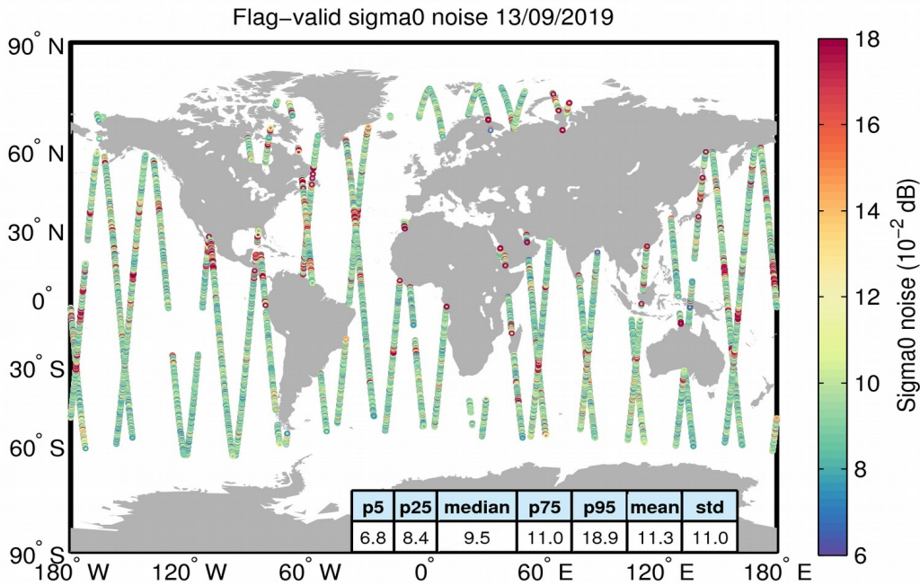
Figure 26. Geographical distribution of flag-valid 20-Hz sigma0 measurement noise over oceans and lakes for 13/09/2019. The statistical values shown in the table refer to the sigma0 noise and are calculated over all measurements shown in the figure.
