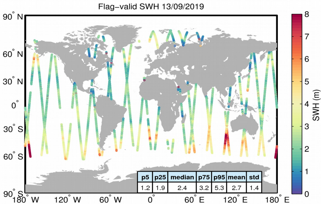
Figure 15. Geographical distribution of flag-valid SWH data over oceans and lakes for 13/09/2019. The statistical values shown in the table refer to the SWH in m and are calculated over all measurements shown in the figure.
