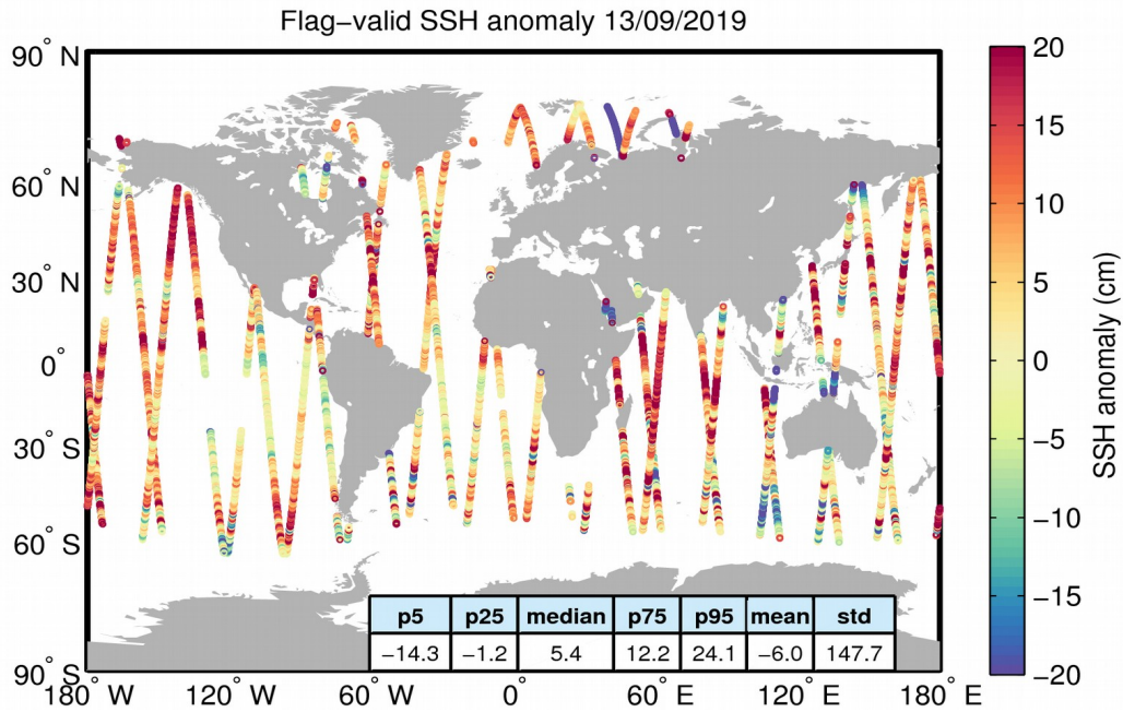
Figure 5. Geographical distribution of flag-valid 1-Hz SSH anomaly data over oceans and lakes for 13/09/2019. The statistical values shown in the table refer to the SSH anomaly in cm and are calculated over all measurements shown in the figure.
