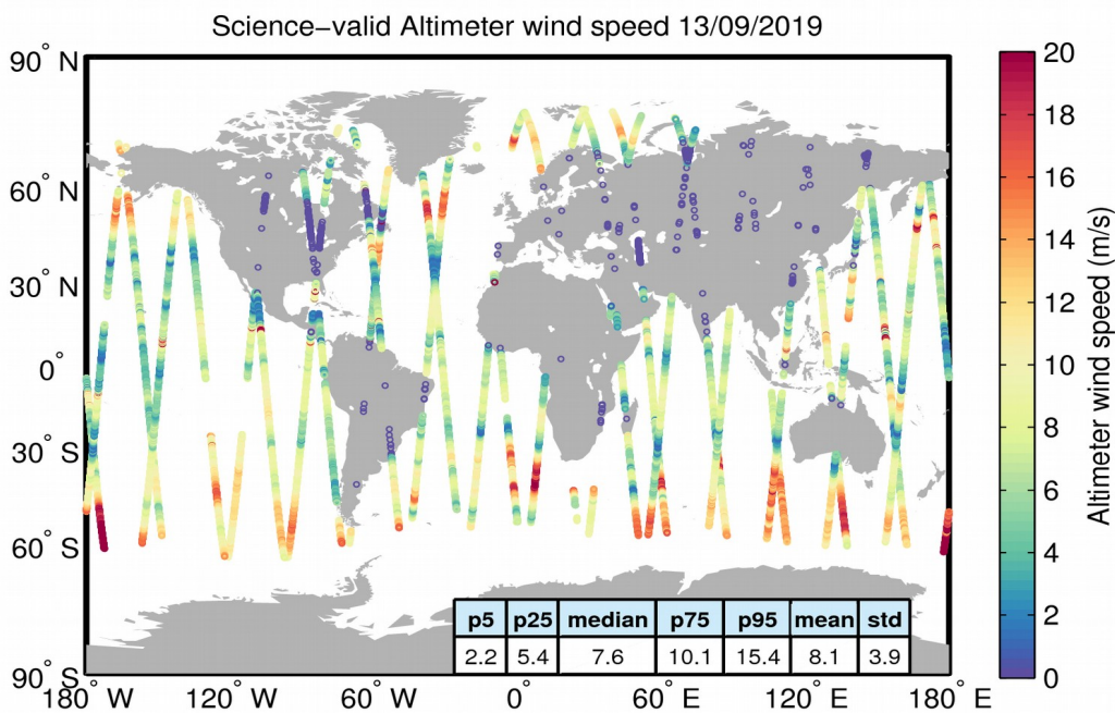
Figure 34. Geographical distribution of science-valid wind data over oceans and lakes for 13/09/2019. The statistical values shown in the table refer to the wind in m/s and are calculated over all measurements shown in the figure. Gray circles denote records that have been rejected based on the editing criteria described in Table 5.
