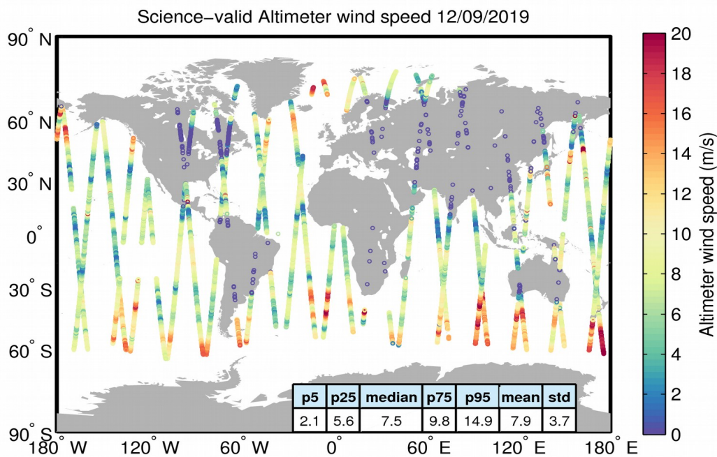
Figure 34. Geographical distribution of science-valid wind data over oceans and lakes for 12/09/2019. The statistical values shown in the table refer to the wind in m/s and are calculated over all measurements shown in the figure. Gray circles denote records that have been rejected based on the editing criteria described in Table 5.
