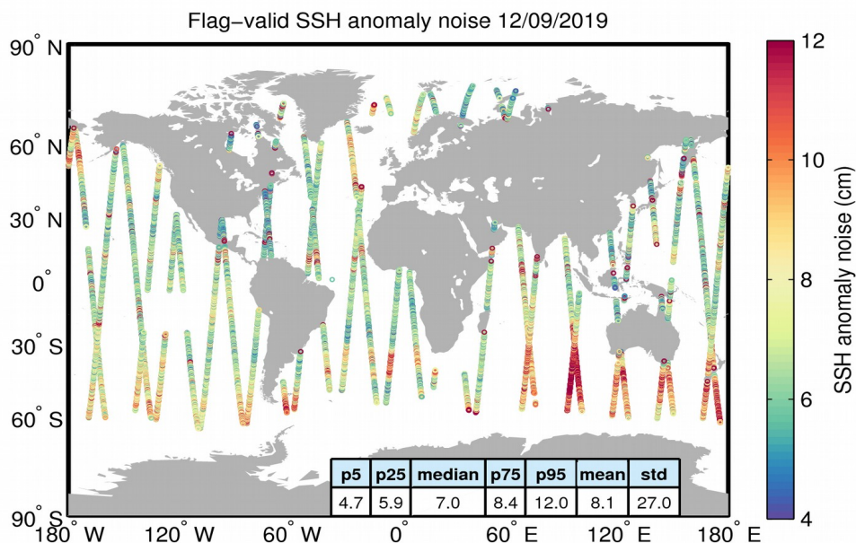
Figure 8. Geographical distribution of flag-valid 20-Hz SSH anomaly measurement noise over oceans and lakes for 12/09/2019. The statistical values shown in the table refer to the SSH anomaly noise and are calculated over all measurements shown in the figure.
