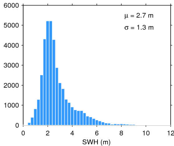
Figure 20. Histogram of science-valid SWH over oceans and lakes for 12/09/2019. The mean ( \mu ) and standard deviation ( \sigma ) are also shown. Note that values larger than 12 m are excluded from the histogram for the sake of readability but not from the computation of \mu and \sigma .
