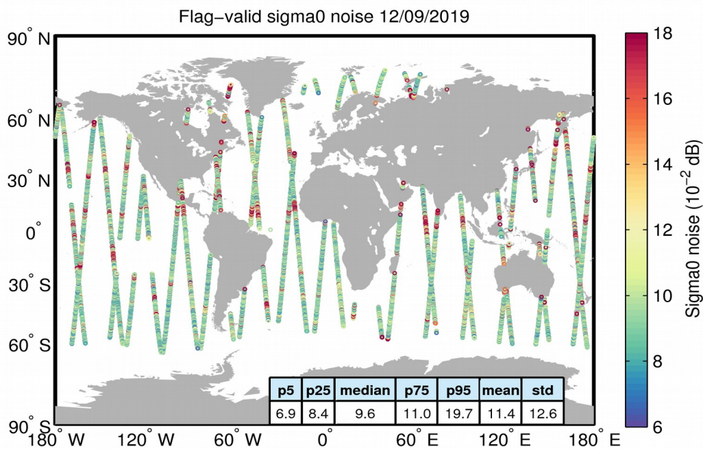
Figure 26. Geographical distribution of flag-valid 20-Hz sigma0 measurement noise over oceans and lakes for 12/09/2019. The statistical values shown in the table refer to the sigma0 noise and are calculated over all measurements shown in the figure.
