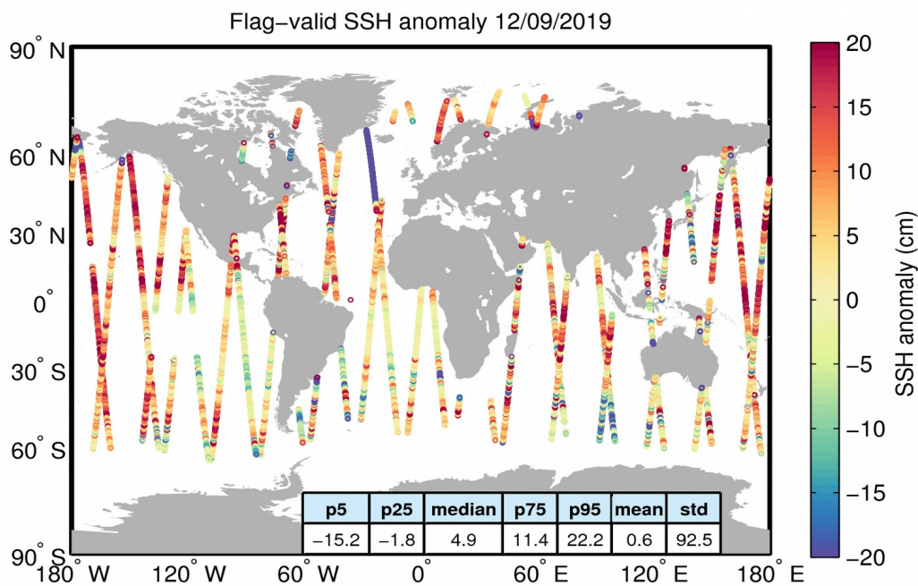
Figure 5. Geographical distribution of flag-valid 1-Hz SSH anomaly data over oceans and lakes for 12/09/2019. The statistical values shown in the table refer to the SSH anomaly in cm and are calculated over all measurements shown in the figure.
