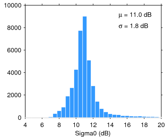
Figure 25. Histogram of flag-valid sigma0 over oceans and lakes for 12/09/2019. The mean ( \mu ) and standard deviation ( \sigma ) are also shown. Note that values outside [4 20] dB are excluded from the histogram for the sake of readability but not from the computation of \mu and \sigma .
