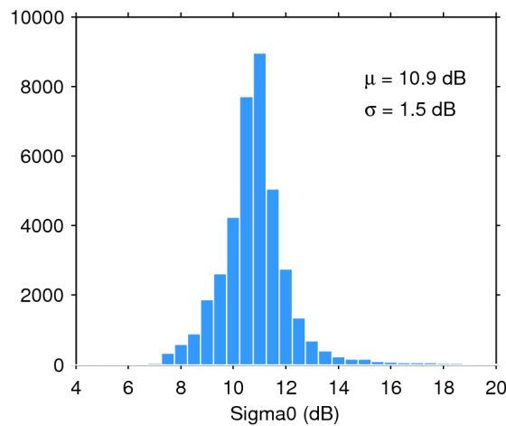
Figure 28. Histogram of science-valid sigma0 over oceans and lakes for 12/09/2019. The mean ( \mu ) and standard deviation ( \sigma ) are also shown. Note that values outside [4 20] dB are excluded from the histogram for the sake of readability but not from the computation of \mu and \sigma .
