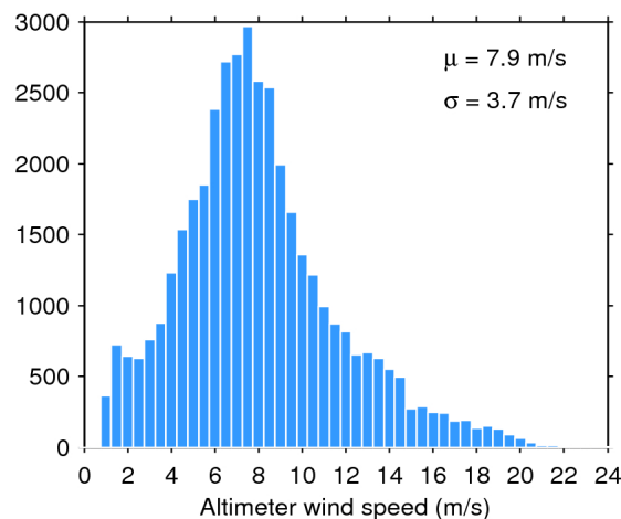
Figure 35. Histogram of science-valid wind over oceans and lakes for 12/09/2019. The mean ( \mu ) and standard deviation ( \sigma ) are also shown. Note that values larger than 24 m/s are excluded from the histogram for the sake of readability but not from the computation of \mu and \sigma .
