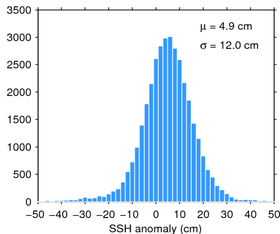
Figure 11. Histogram of science-valid SSH anomaly over oceans and lakes for 12/09/2019. The mean ( \mu ) and standard deviation ( \sigma ) are also shown. Note that values outside [-50 50] cm are excluded from the histogram for the sake of readability but not from the computation of \mu and \sigma .
