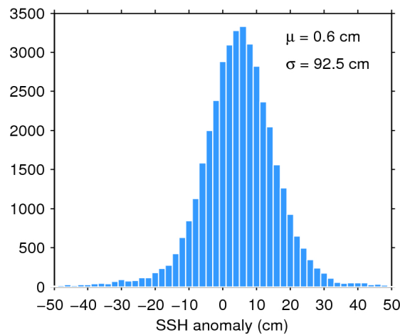
Figure 7. Histogram of flag-valid SSH anomaly over oceans and lakes for 12/09/2019. The mean ( \mu ) and standard deviation ( \sigma ) are also shown. Note that values outside [-50\ 50] cm are excluded from the histogram for the sake of readability but not from the computation of \mu and \sigma .
