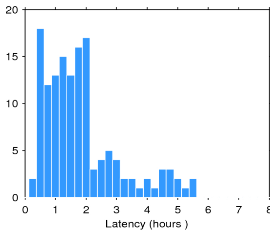
Figure 2. Histogram of the data latency for 12/09/2019. The y-axis denotes the number of files that are made available with a delay of x-hours with respect to the mean time of the records stored in the file.
