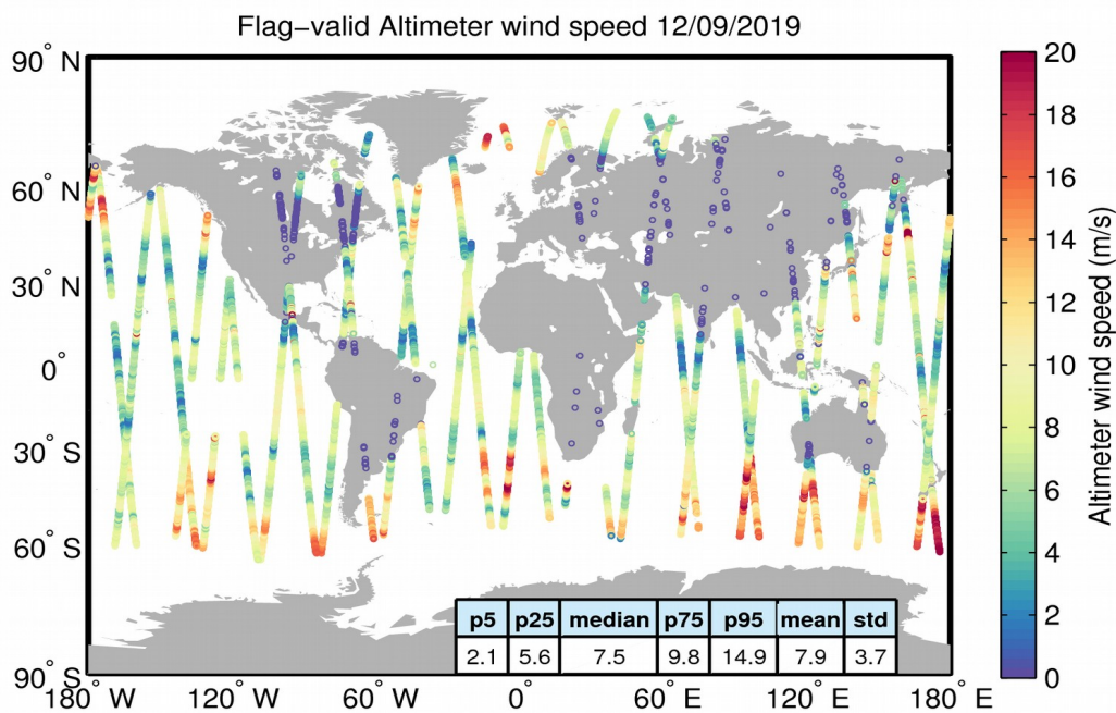
Figure 31. Geographical distribution of flag-valid wind data over oceans and lakes for 12/09/2019. The statistical values shown in the table refer to the wind in m/s and are calculated over all measurements shown in the figure.
