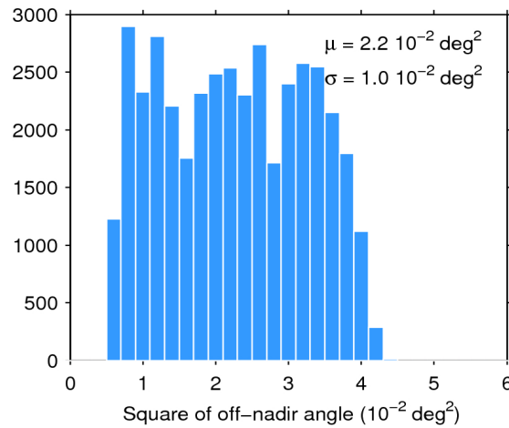
Figure 39. Histogram of flag-valid mispointing over oceans and lakes for 12/09/2019. The mean ( \mu ) and standard deviation ( \sigma ) are also shown. Note that values larger than 6 \cdot 10^{-2} \text{ deg}^2 are excluded from the histogram for the sake of readability but not from the computation of \mu and \sigma .
