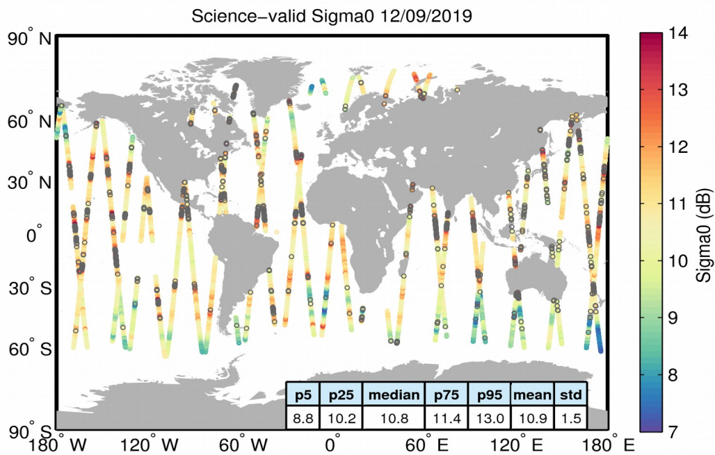
Figure 27. Geographical distribution of science-valid sigma0 data over oceans and lakes for 12/09/2019. The statistical values shown in the table refer to the sigma0 in dB and are calculated over all measurements shown in the figure. Gray circles denote records that have been rejected based on the editing criteria described in Table 4.
