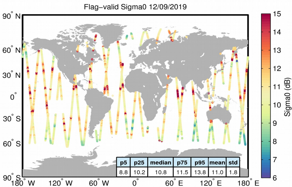
Figure 23. Geographical distribution of flag-valid sigma0 data over oceans and lakes for 12/09/2019. The statistical values shown in the table refer to the sigma0 in dB and are calculated over all measurements shown in the figure.
