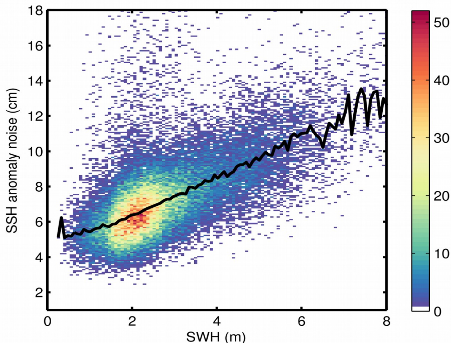
Figure 9. 2D histogram showing flag-valid SSH anomaly noise as a function of SWH for 12/09/2019. The black line denotes the median SSH anomaly noise as a function of SWH.
