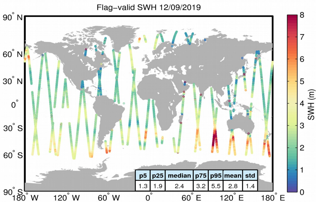
Figure 15. Geographical distribution of flag-valid SWH data over oceans and lakes for 12/09/2019. The statistical values shown in the table refer to the SWH in m and are calculated over all measurements shown in the figure.
