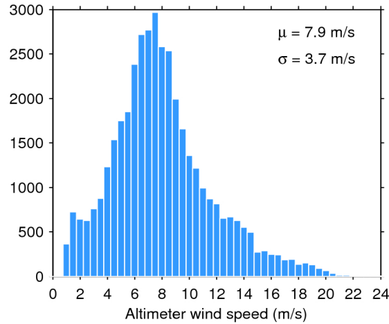
Figure 33. Histogram of flag-valid wind over oceans and lakes for 12/09/2019. The mean ( \mu ) and standard deviation ( \sigma ) are also shown. Note that values larger than 24 m/s are excluded from the histogram for the sake of readability but not from the computation of \mu and \sigma .
