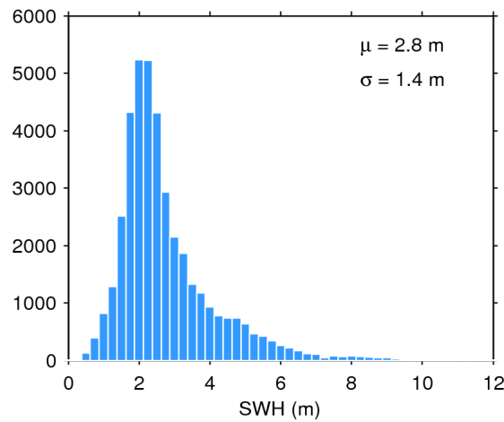
Figure 17. Histogram of flag-valid SWH over oceans and lakes for 12/09/2019. The mean ( \mu ) and standard deviation ( \sigma ) are also shown. Note that values larger than 12 m are excluded from the histogram for the sake of readability but not from the computation of \mu and \sigma .
