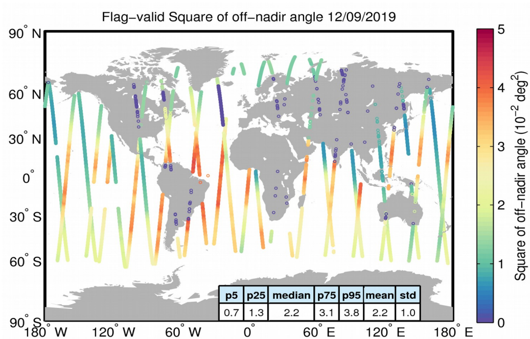
Figure 37. Geographical distribution of flag-valid mispointing data over oceans and lakes for 12/09/2019. The statistical values shown in the table refer to the mispointing in 10^{-2} \text{ deg}^2 and are calculated over all measurements shown in the figure.
