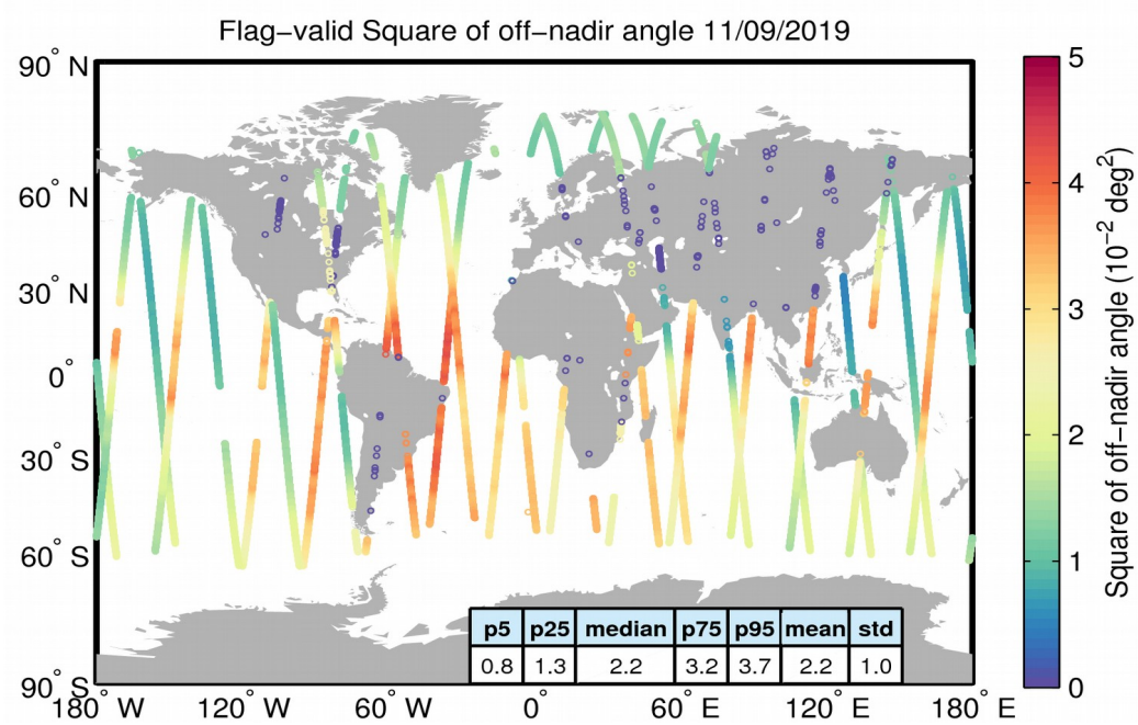
Figure 37. Geographical distribution of flag-valid mispointing data over oceans and lakes for 11/09/2019. The statistical values shown in the table refer to the mispointing in 10^{-2} \text{ deg}^2 and are calculated over all measurements shown in the figure.
