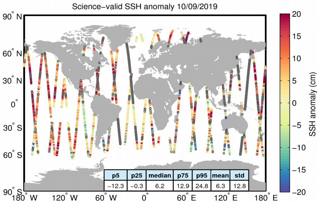
Figure 10. Geographical distribution of science-valid SSH anomaly data over oceans and lakes for 10/09/2019. The statistical values shown in the table refer to the SSH anomaly in cm and are calculated over all measurements shown in the figure. Gray circles denote records that have been rejected based on the editing criteria described in Table 2.
