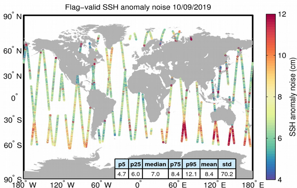
Figure 8. Geographical distribution of flag-valid 20-Hz SSH anomaly measurement noise over oceans and lakes for 10/09/2019. The statistical values shown in the table refer to the SSH anomaly noise and are calculated over all measurements shown in the figure.
