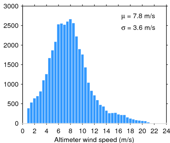
Figure 35. Histogram of science-valid wind over oceans and lakes for 10/09/2019. The mean ( \mu ) and standard deviation ( \sigma ) are also shown. Note that values larger than 24 m/s are excluded from the histogram for the sake of readability but not from the computation of \mu and \sigma .
