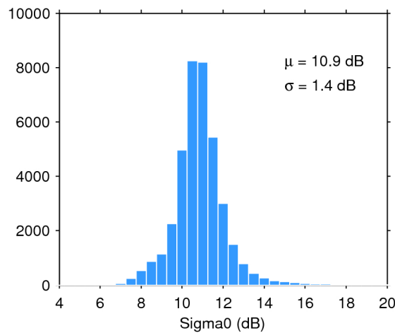
Figure 28. Histogram of science-valid sigma0 over oceans and lakes for 10/09/2019. The mean ( \mu ) and standard deviation ( \sigma ) are also shown. Note that values outside [4 20] dB are excluded from the histogram for the sake of readability but not from the computation of \mu and \sigma .
