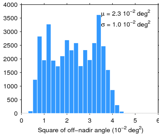
Figure 39. Histogram of flag-valid mispointing over oceans and lakes for 10/09/2019. The mean ( \mu ) and standard deviation ( \sigma ) are also shown. Note that values larger than 6 \cdot 10^{-2} \text{ deg}^2 are excluded from the histogram for the sake of readability but not from the computation of \mu and \sigma .
