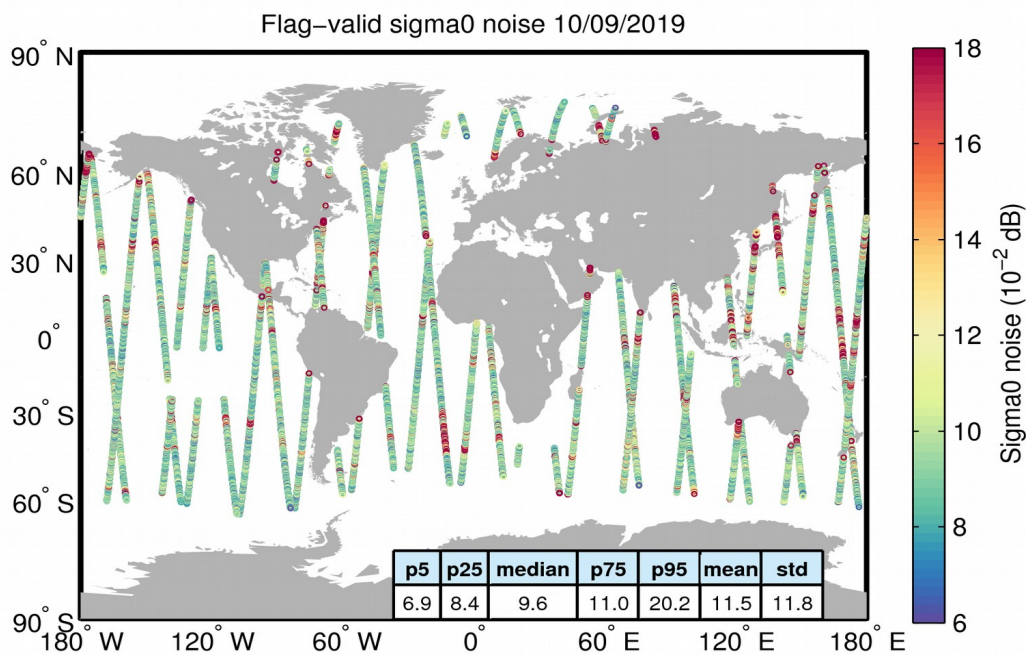
Figure 26. Geographical distribution of flag-valid 20-Hz sigma0 measurement noise over oceans and lakes for 10/09/2019. The statistical values shown in the table refer to the sigma0 noise and are calculated over all measurements shown in the figure.
