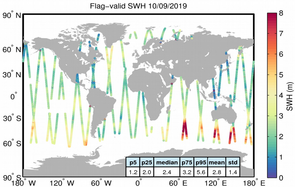
Figure 15. Geographical distribution of flag-valid SWH data over oceans and lakes for 10/09/2019. The statistical values shown in the table refer to the SWH in m and are calculated over all measurements shown in the figure.
