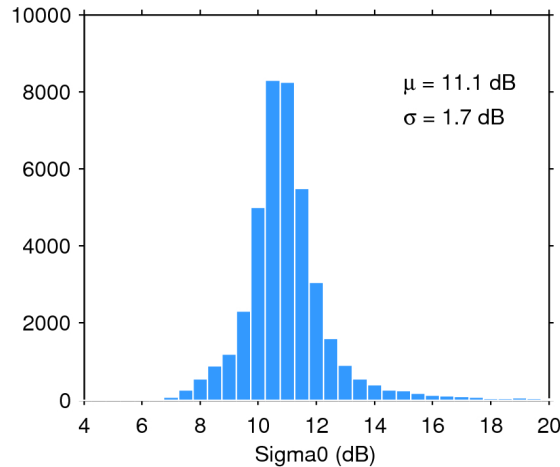
Figure 25. Histogram of flag-valid sigma0 over oceans and lakes for 10/09/2019. The mean ( \mu ) and standard deviation ( \sigma ) are also shown. Note that values outside [4 20] dB are excluded from the histogram for the sake of readability but not from the computation of \mu and \sigma .
