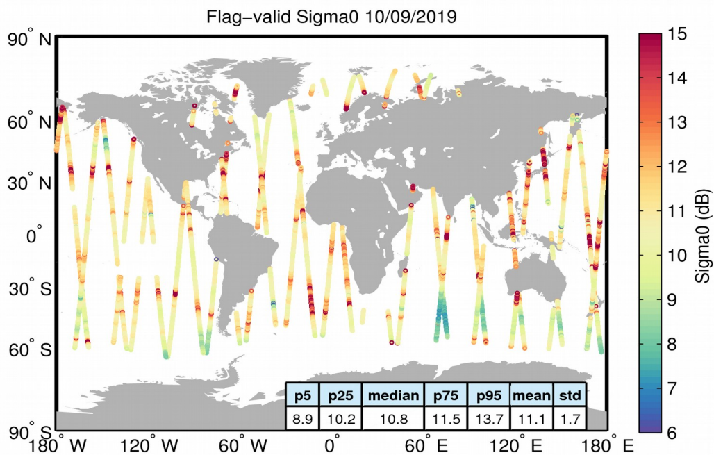
Figure 23. Geographical distribution of flag-valid sigma0 data over oceans and lakes for 10/09/2019. The statistical values shown in the table refer to the sigma0 in dB and are calculated over all measurements shown in the figure.
