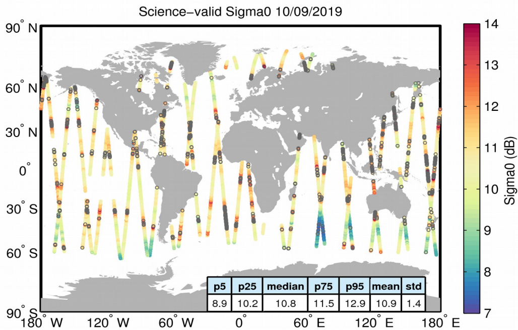
Figure 27. Geographical distribution of science-valid sigma0 data over oceans and lakes for 10/09/2019. The statistical values shown in the table refer to the sigma0 in dB and are calculated over all measurements shown in the figure. Gray circles denote records that have been rejected based on the editing criteria described in Table 4.
