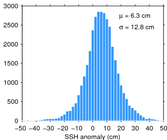
Figure 11. Histogram of science-valid SSH anomaly over oceans and lakes for 10/09/2019. The mean ( \mu ) and standard deviation ( \sigma ) are also shown. Note that values outside [-50 50] cm are excluded from the histogram for the sake of readability but not from the computation of \mu and \sigma .
