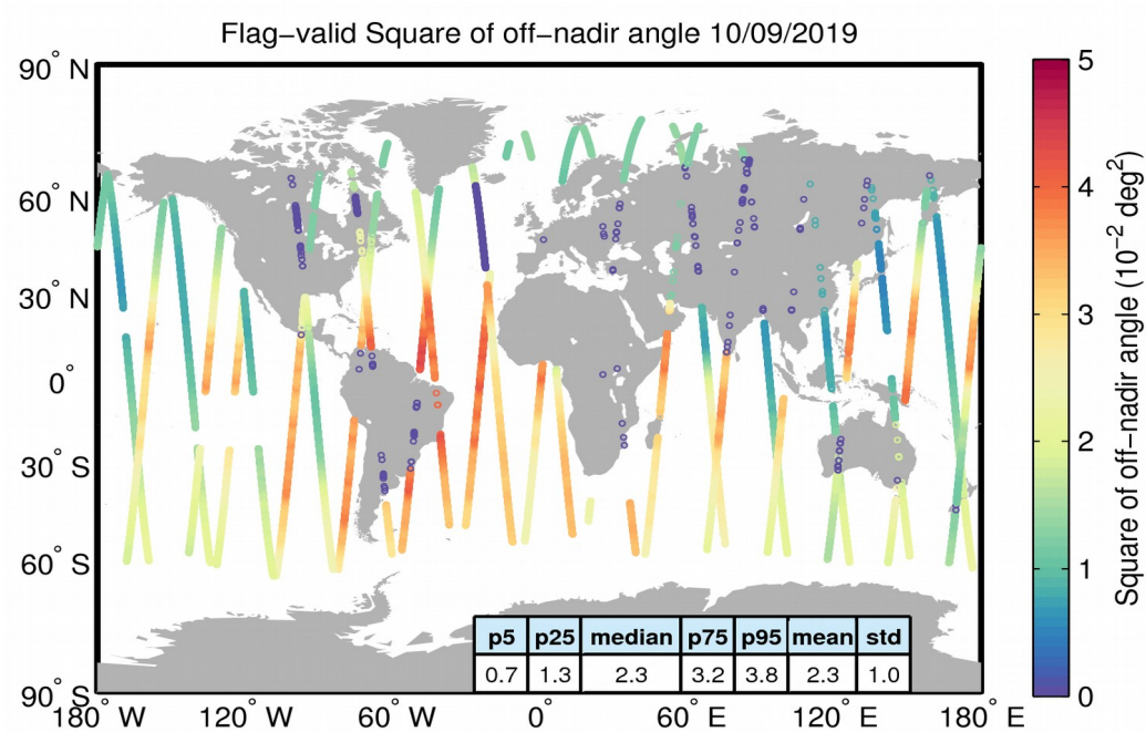
Figure 37. Geographical distribution of flag-valid mispointing data over oceans and lakes for 10/09/2019. The statistical values shown in the table refer to the mispointing in 10^{-2} \text{ deg}^2 and are calculated over all measurements shown in the figure.
