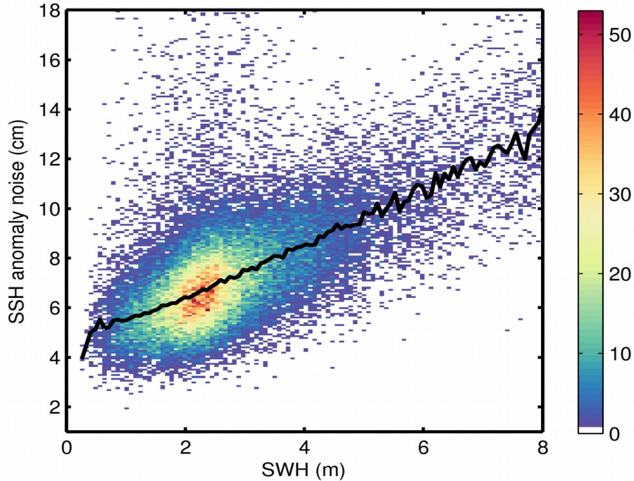
Figure 9. 2D histogram showing flag-valid SSH anomaly noise as a function of SWH for 10/09/2019. The black line denotes the median SSH anomaly noise as a function of SWH.
