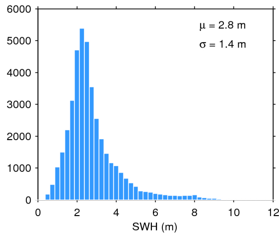
Figure 17. Histogram of flag-valid SWH over oceans and lakes for 10/09/2019. The mean ( \mu ) and standard deviation ( \sigma ) are also shown. Note that values larger than 12 m are excluded from the histogram for the sake of readability but not from the computation of \mu and \sigma .
