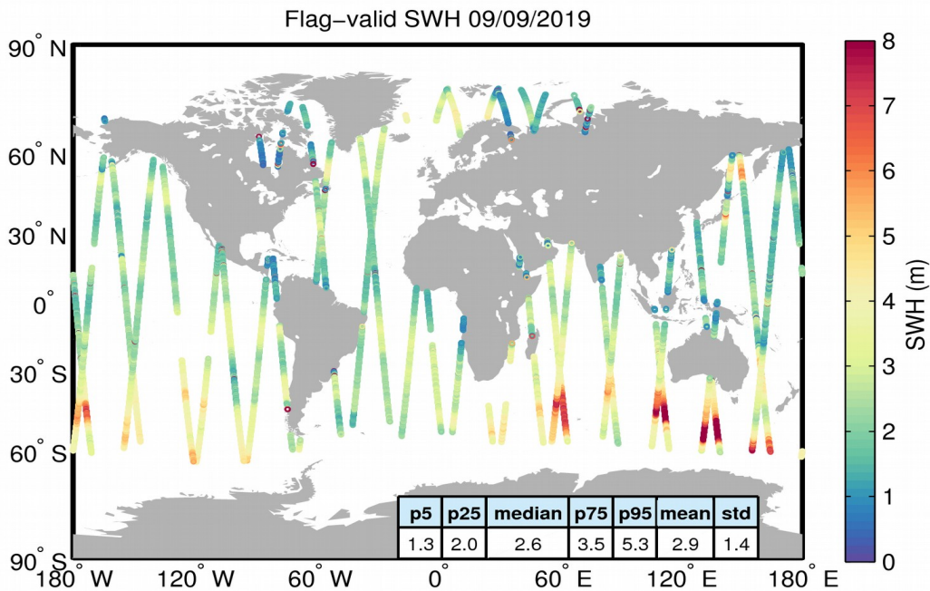
Figure 15. Geographical distribution of flag-valid SWH data over oceans and lakes for 09/09/2019. The statistical values shown in the table refer to the SWH in m and are calculated over all measurements shown in the figure.
