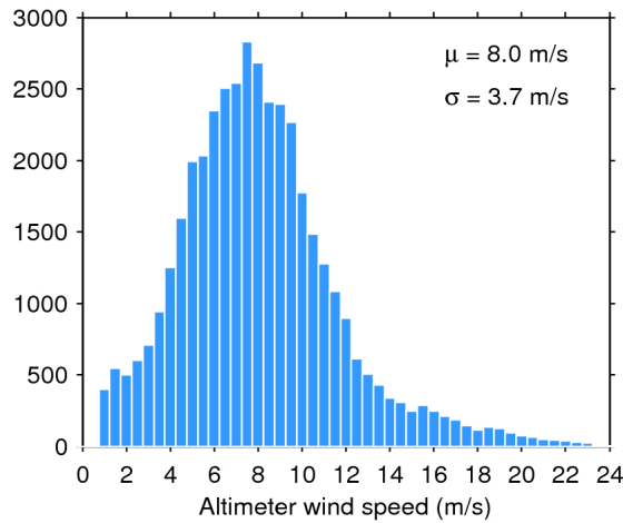
Figure 33. Histogram of flag-valid wind over oceans and lakes for 09/09/2019. The mean ( \mu ) and standard deviation ( \sigma ) are also shown. Note that values larger than 24 m/s are excluded from the histogram for the sake of readability but not from the computation of \mu and \sigma .
