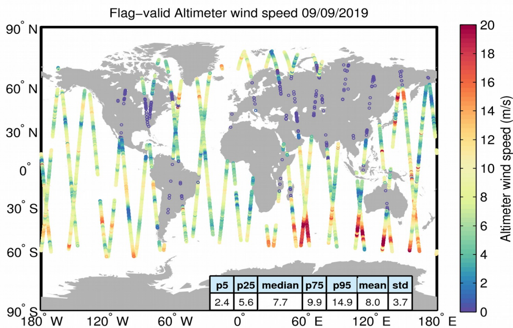
Figure 31. Geographical distribution of flag-valid wind data over oceans and lakes for 09/09/2019. The statistical values shown in the table refer to the wind in m/s and are calculated over all measurements shown in the figure.
