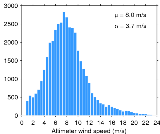
Figure 35. Histogram of science-valid wind over oceans and lakes for 09/09/2019. The mean ( \mu ) and standard deviation ( \sigma ) are also shown. Note that values larger than 24 m/s are excluded from the histogram for the sake of readability but not from the computation of \mu and \sigma .
