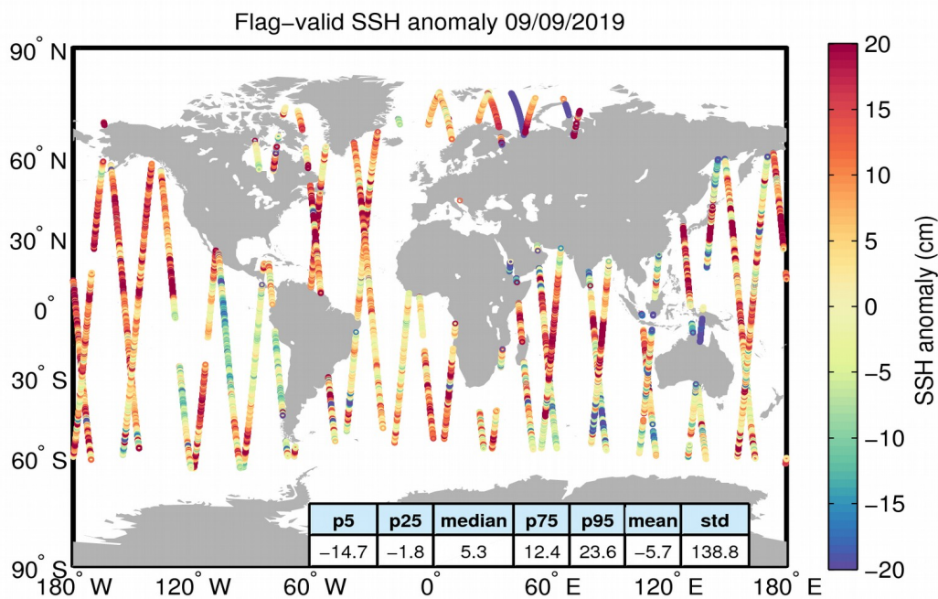
Figure 5. Geographical distribution of flag-valid 1-Hz SSH anomaly data over oceans and lakes for 09/09/2019. The statistical values shown in the table refer to the SSH anomaly in cm and are calculated over all measurements shown in the figure.
