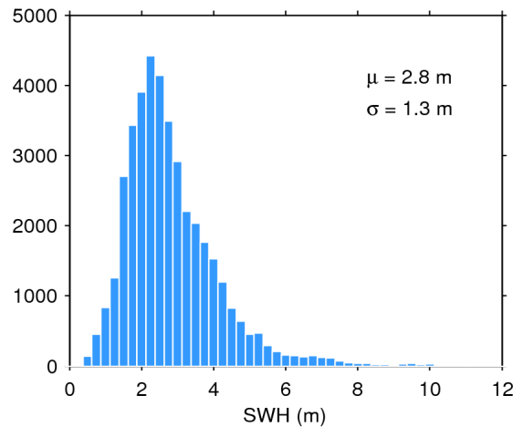
Figure 20. Histogram of science-valid SWH over oceans and lakes for 09/09/2019. The mean ( \mu ) and standard deviation ( \sigma ) are also shown. Note that values larger than 12 m are excluded from the histogram for the sake of readability but not from the computation of \mu and \sigma .
