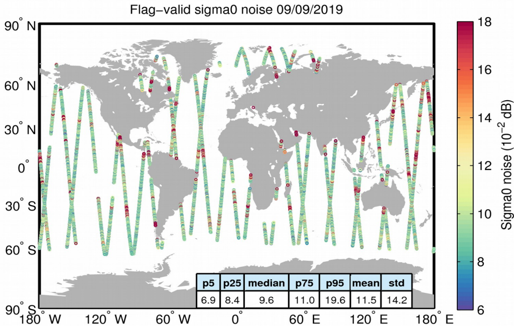
Figure 26. Geographical distribution of flag-valid 20-Hz sigma0 measurement noise over oceans and lakes for 09/09/2019. The statistical values shown in the table refer to the sigma0 noise and are calculated over all measurements shown in the figure.
