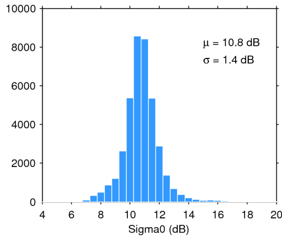
Figure 28. Histogram of science-valid sigma0 over oceans and lakes for 09/09/2019. The mean ( \mu ) and standard deviation ( \sigma ) are also shown. Note that values outside [4 20] dB are excluded from the histogram for the sake of readability but not from the computation of \mu and \sigma .
