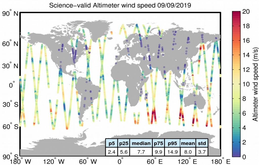
Figure 34. Geographical distribution of science-valid wind data over oceans and lakes for 09/09/2019. The statistical values shown in the table refer to the wind in m/s and are calculated over all measurements shown in the figure. Gray circles denote records that have been rejected based on the editing criteria described in Table 5.
