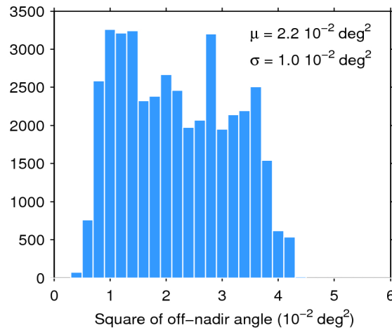
Figure 39. Histogram of flag-valid mispointing over oceans and lakes for 09/09/2019. The mean ( \mu ) and standard deviation ( \sigma ) are also shown. Note that values larger than 6 \cdot 10^{-2} \text{ deg}^2 are excluded from the histogram for the sake of readability but not from the computation of \mu and \sigma .
