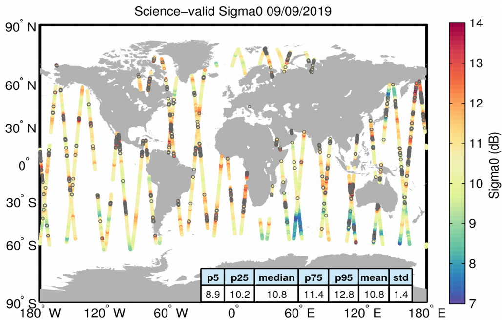
Figure 27. Geographical distribution of science-valid sigma0 data over oceans and lakes for 09/09/2019. The statistical values shown in the table refer to the sigma0 in dB and are calculated over all measurements shown in the figure. Gray circles denote records that have been rejected based on the editing criteria described in Table 4.
