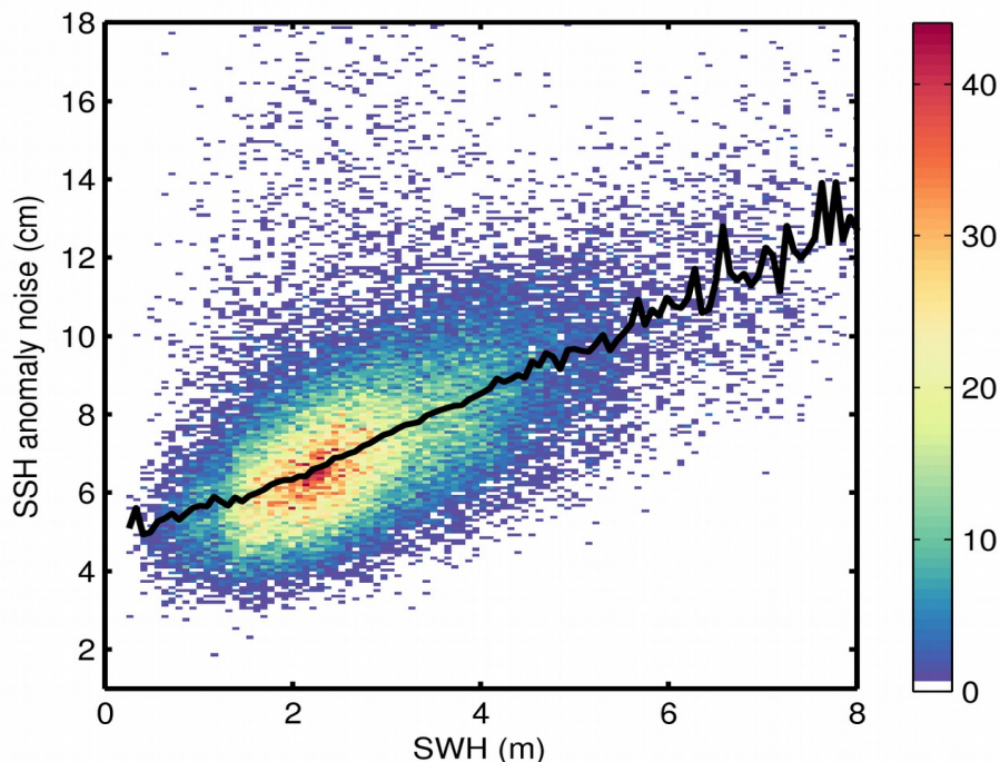
Figure 9. 2D histogram showing flag-valid SSH anomaly noise as a function of SWH for 09/09/2019. The black line denotes the median SSH anomaly noise as a function of SWH.
