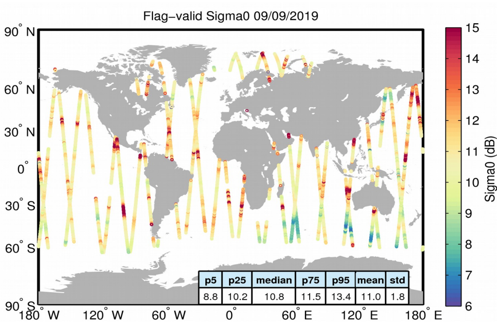
Figure 23. Geographical distribution of flag-valid sigma0 data over oceans and lakes for 09/09/2019. The statistical values shown in the table refer to the sigma0 in dB and are calculated over all measurements shown in the figure.
