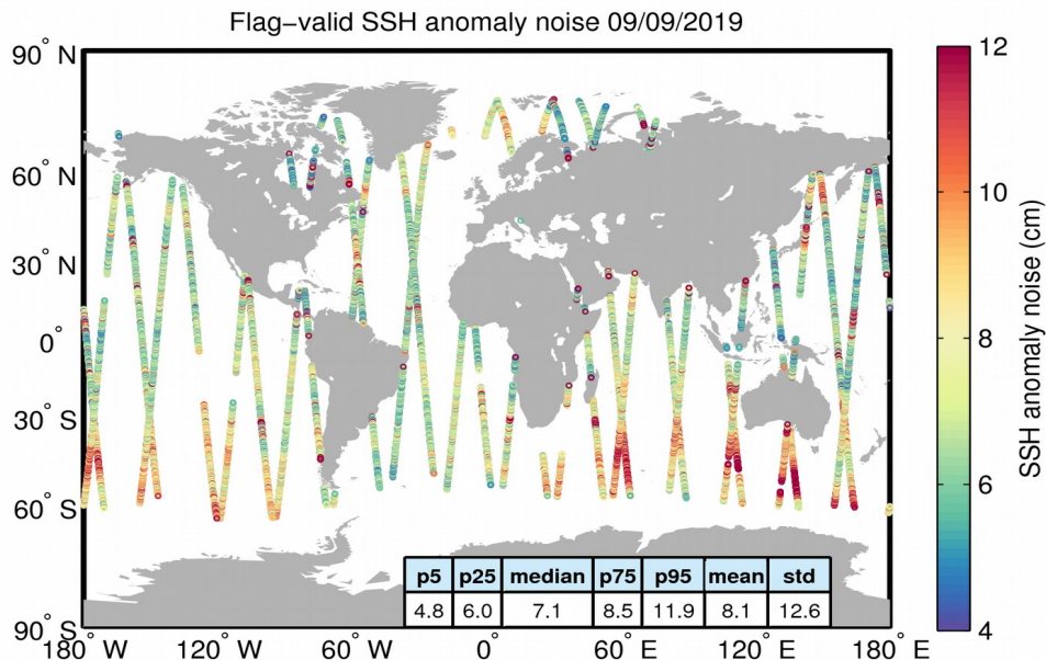
Figure 8. Geographical distribution of flag-valid 20-Hz SSH anomaly measurement noise over oceans and lakes for 09/09/2019. The statistical values shown in the table refer to the SSH anomaly noise and are calculated over all measurements shown in the figure.
