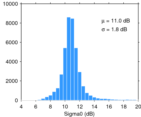
Figure 25. Histogram of flag-valid sigma0 over oceans and lakes for 09/09/2019. The mean ( \mu ) and standard deviation ( \sigma ) are also shown. Note that values outside [4 20] dB are excluded from the histogram for the sake of readability but not from the computation of \mu and \sigma .
