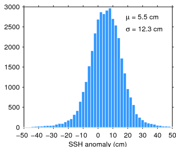
Figure 11. Histogram of science-valid SSH anomaly over oceans and lakes for 09/09/2019. The mean ( \mu ) and standard deviation ( \sigma ) are also shown. Note that values outside [-50 50] cm are excluded from the histogram for the sake of readability but not from the computation of \mu and \sigma .
