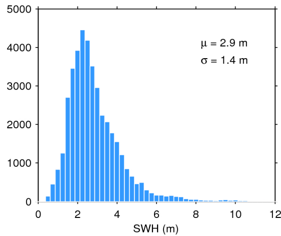
Figure 17. Histogram of flag-valid SWH over oceans and lakes for 09/09/2019. The mean ( \mu ) and standard deviation ( \sigma ) are also shown. Note that values larger than 12 m are excluded from the histogram for the sake of readability but not from the computation of \mu and \sigma .
