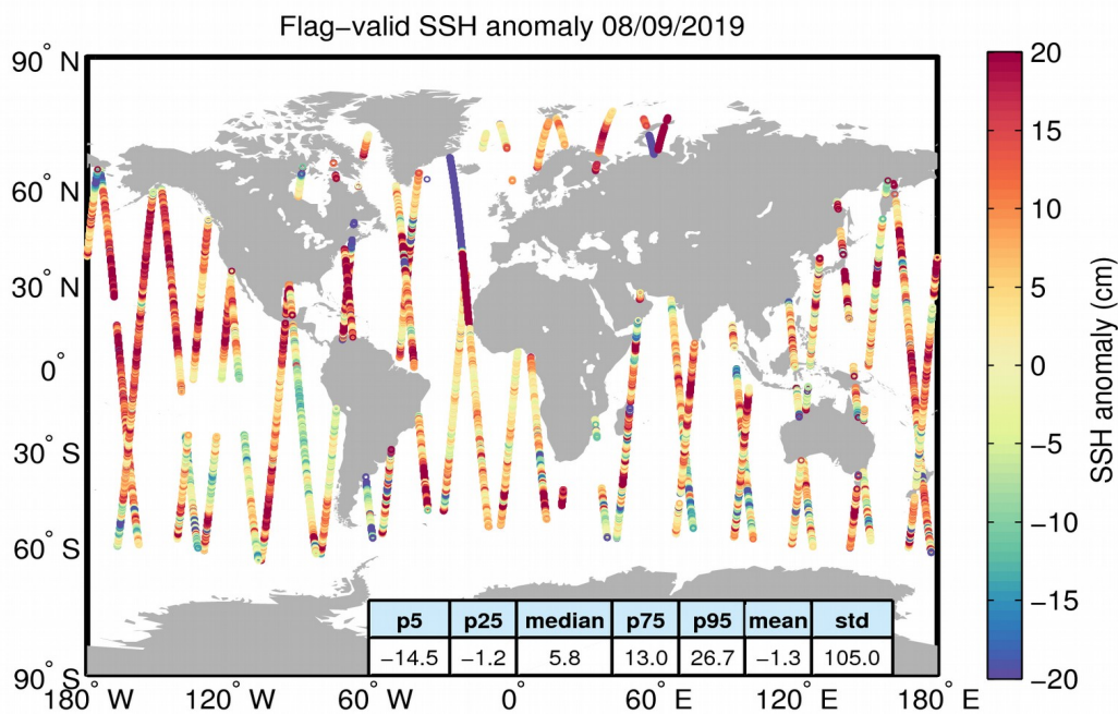
Figure 5. Geographical distribution of flag-valid 1-Hz SSH anomaly data over oceans and lakes for 08/09/2019. The statistical values shown in the table refer to the SSH anomaly in cm and are calculated over all measurements shown in the figure.
