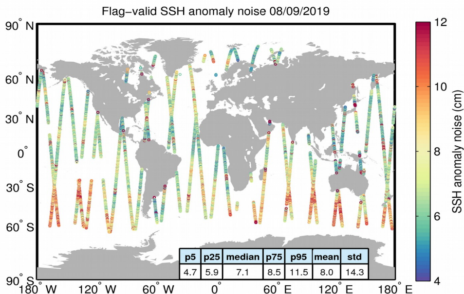
Figure 8. Geographical distribution of flag-valid 20-Hz SSH anomaly measurement noise over oceans and lakes for 08/09/2019. The statistical values shown in the table refer to the SSH anomaly noise and are calculated over all measurements shown in the figure.
