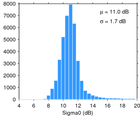
Figure 25. Histogram of flag-valid sigma0 over oceans and lakes for 08/09/2019. The mean ( \mu ) and standard deviation ( \sigma ) are also shown. Note that values outside [4 20] dB are excluded from the histogram for the sake of readability but not from the computation of \mu and \sigma .
