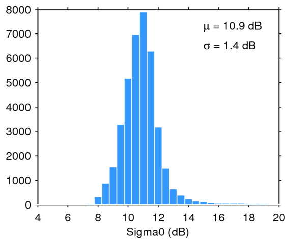
Figure 28. Histogram of science-valid sigma0 over oceans and lakes for 08/09/2019. The mean ( \mu ) and standard deviation ( \sigma ) are also shown. Note that values outside [4 20] dB are excluded from the histogram for the sake of readability but not from the computation of \mu and \sigma .
