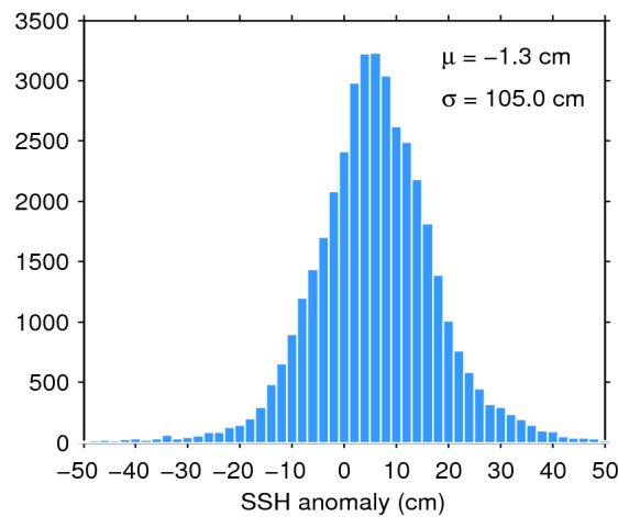
Figure 7. Histogram of flag-valid SSH anomaly over oceans and lakes for 08/09/2019. The mean ( \mu ) and standard deviation ( \sigma ) are also shown. Note that values outside [-50\ 50] cm are excluded from the histogram for the sake of readability but not from the computation of \mu and \sigma .
