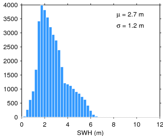
Figure 20. Histogram of science-valid SWH over oceans and lakes for 08/09/2019. The mean ( \mu ) and standard deviation ( \sigma ) are also shown. Note that values larger than 12 m are excluded from the histogram for the sake of readability but not from the computation of \mu and \sigma .
