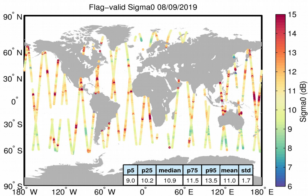
Figure 23. Geographical distribution of flag-valid sigma0 data over oceans and lakes for 08/09/2019. The statistical values shown in the table refer to the sigma0 in dB and are calculated over all measurements shown in the figure.
