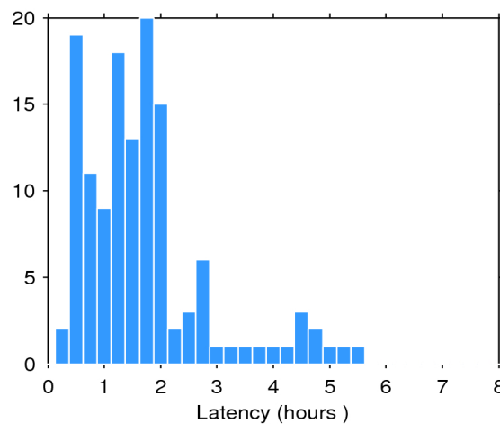
Figure 2. Histogram of the data latency for 08/09/2019. The y-axis denotes the number of files that are made available with a delay of x-hours with respect to the mean time of the records stored in the file.
