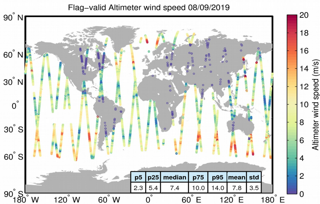
Figure 31. Geographical distribution of flag-valid wind data over oceans and lakes for 08/09/2019. The statistical values shown in the table refer to the wind in m/s and are calculated over all measurements shown in the figure.
