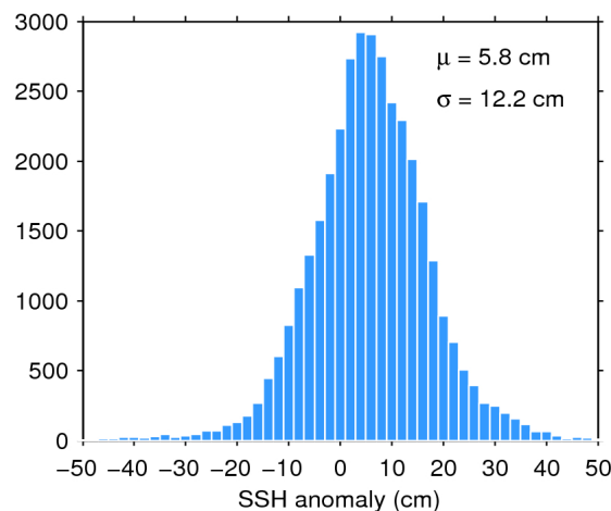
Figure 11. Histogram of science-valid SSH anomaly over oceans and lakes for 08/09/2019. The mean ( \mu ) and standard deviation ( \sigma ) are also shown. Note that values outside [-50 50] cm are excluded from the histogram for the sake of readability but not from the computation of \mu and \sigma .
