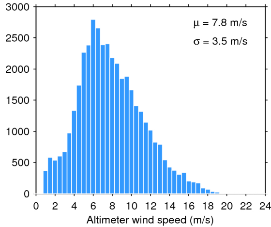
Figure 33. Histogram of flag-valid wind over oceans and lakes for 08/09/2019. The mean ( \mu ) and standard deviation ( \sigma ) are also shown. Note that values larger than 24 m/s are excluded from the histogram for the sake of readability but not from the computation of \mu and \sigma .
