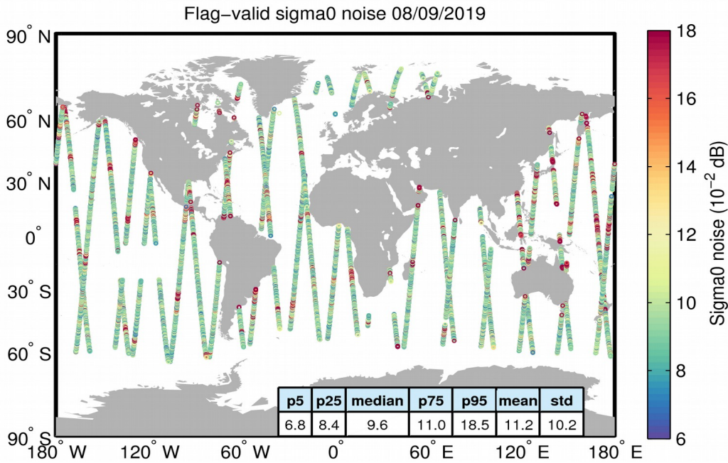
Figure 26. Geographical distribution of flag-valid 20-Hz sigma0 measurement noise over oceans and lakes for 08/09/2019. The statistical values shown in the table refer to the sigma0 noise and are calculated over all measurements shown in the figure.
