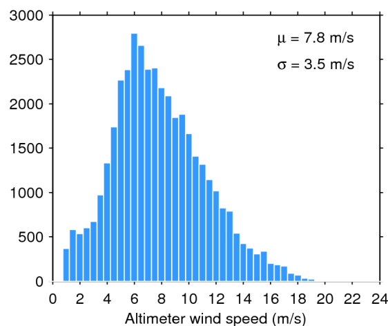
Figure 35. Histogram of science-valid wind over oceans and lakes for 08/09/2019. The mean ( \mu ) and standard deviation ( \sigma ) are also shown. Note that values larger than 24 m/s are excluded from the histogram for the sake of readability but not from the computation of \mu and \sigma .
