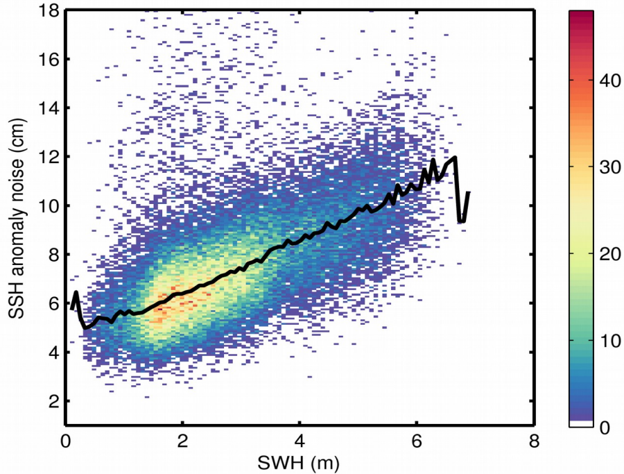
Figure 9. 2D histogram showing flag-valid SSH anomaly noise as a function of SWH for 08/09/2019. The black line denotes the median SSH anomaly noise as a function of SWH.
