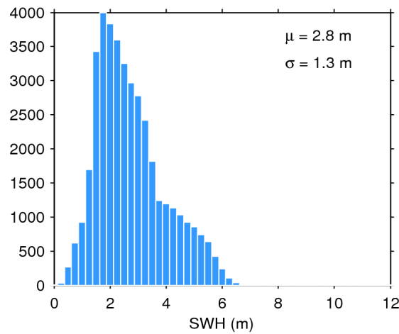
Figure 17. Histogram of flag-valid SWH over oceans and lakes for 08/09/2019. The mean ( \mu ) and standard deviation ( \sigma ) are also shown. Note that values larger than 12 m are excluded from the histogram for the sake of readability but not from the computation of \mu and \sigma .
