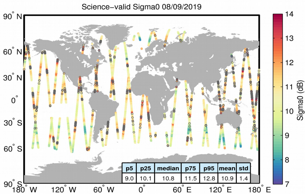
Figure 27. Geographical distribution of science-valid sigma0 data over oceans and lakes for 08/09/2019. The statistical values shown in the table refer to the sigma0 in dB and are calculated over all measurements shown in the figure. Gray circles denote records that have been rejected based on the editing criteria described in Table 4.
