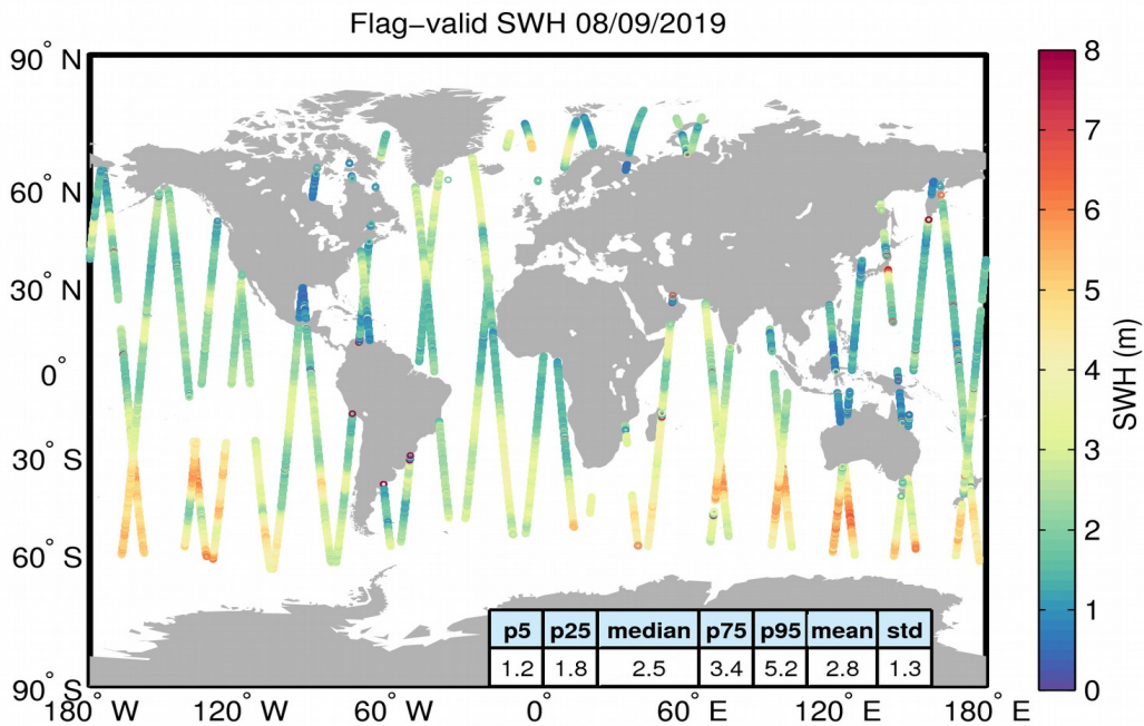
Figure 15. Geographical distribution of flag-valid SWH data over oceans and lakes for 08/09/2019. The statistical values shown in the table refer to the SWH in m and are calculated over all measurements shown in the figure.
