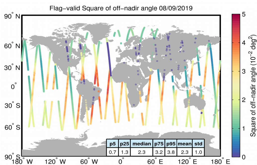
Figure 37. Geographical distribution of flag-valid mispointing data over oceans and lakes for 08/09/2019. The statistical values shown in the table refer to the mispointing in 10^{-2} \text{ deg}^2 and are calculated over all measurements shown in the figure.
