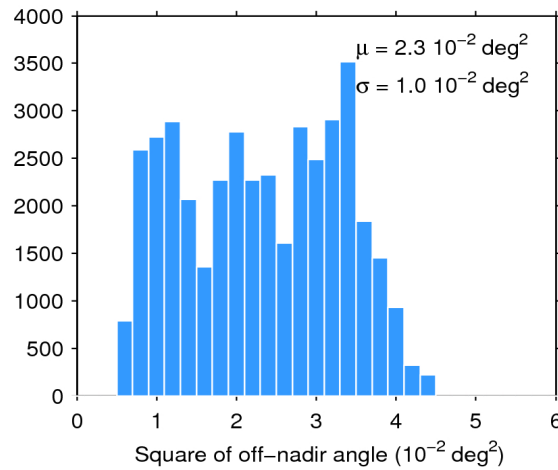
Figure 39. Histogram of flag-valid mispointing over oceans and lakes for 08/09/2019. The mean ( \mu ) and standard deviation ( \sigma ) are also shown. Note that values larger than 6 \cdot 10^{-2} \text{ deg}^2 are excluded from the histogram for the sake of readability but not from the computation of \mu and \sigma .
