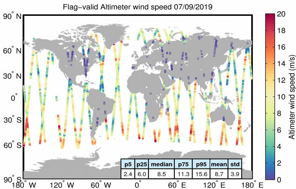
Figure 31. Geographical distribution of flag-valid wind data over oceans and lakes for 07/09/2019. The statistical values shown in the table refer to the wind in m/s and are calculated over all measurements shown in the figure.
