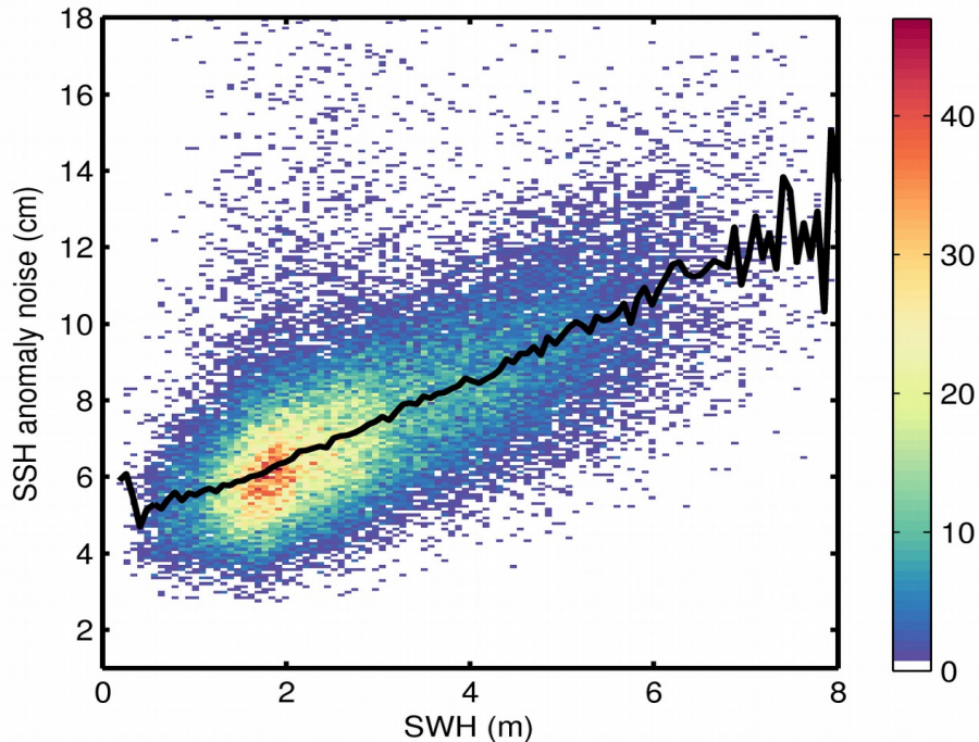
Figure 9. 2D histogram showing flag-valid SSH anomaly noise as a function of SWH for 07/09/2019. The black line denotes the median SSH anomaly noise as a function of SWH.
