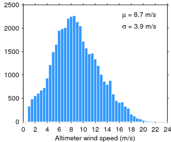
Figure 33. Histogram of flag-valid wind over oceans and lakes for 07/09/2019. The mean ( \mu ) and standard deviation ( \sigma ) are also shown. Note that values larger than 24 m/s are excluded from the histogram for the sake of readability but not from the computation of \mu and \sigma .
