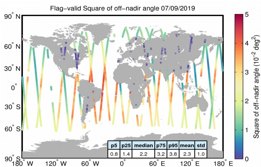
Figure 37. Geographical distribution of flag-valid mispointing data over oceans and lakes for 07/09/2019. The statistical values shown in the table refer to the mispointing in 10^{-2} \text{ deg}^2 and are calculated over all measurements shown in the figure.
