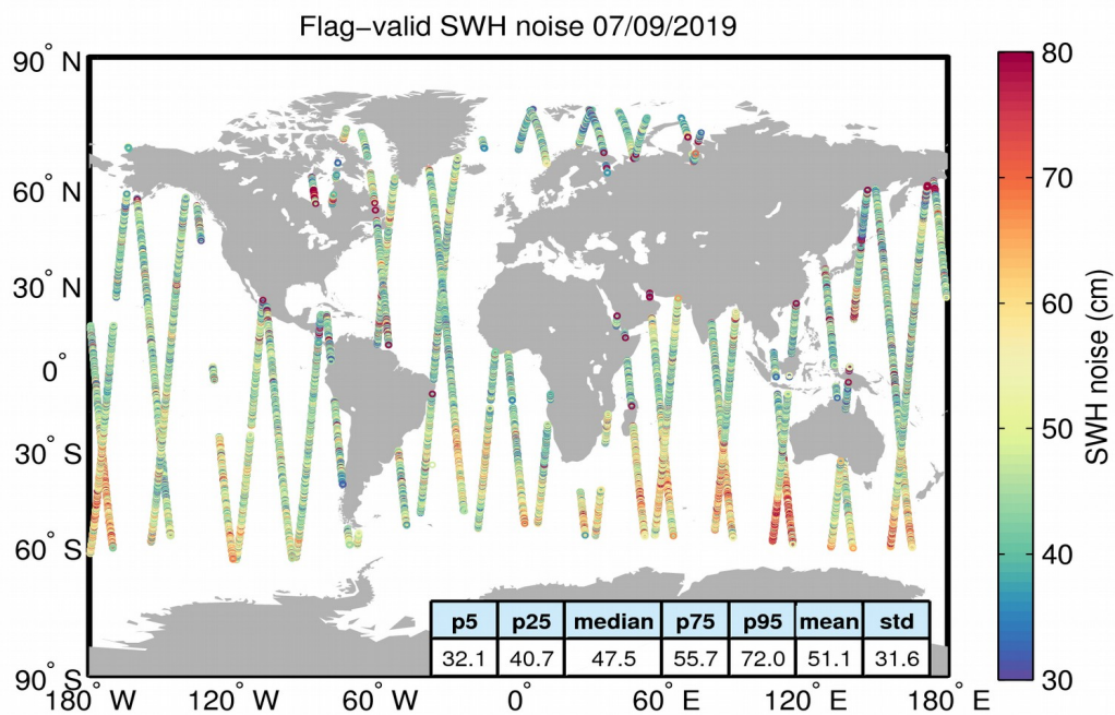
Figure 18. Geographical distribution of flag-valid 20-Hz SWH measurement noise over oceans and lakes for 07/09/2019. The statistical values shown in the table refer to the SWH noise and are calculated over all measurements shown in the figure.
