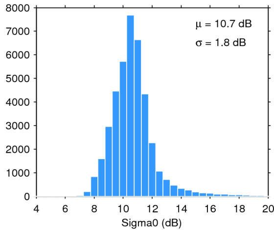
Figure 25. Histogram of flag-valid sigma0 over oceans and lakes for 07/09/2019. The mean ( \mu ) and standard deviation ( \sigma ) are also shown. Note that values outside [4 20] dB are excluded from the histogram for the sake of readability but not from the computation of \mu and \sigma .
