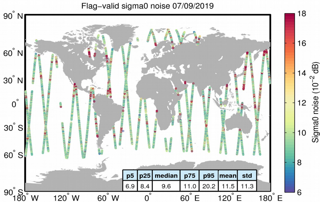
Figure 26. Geographical distribution of flag-valid 20-Hz sigma0 measurement noise over oceans and lakes for 07/09/2019. The statistical values shown in the table refer to the sigma0 noise and are calculated over all measurements shown in the figure.
