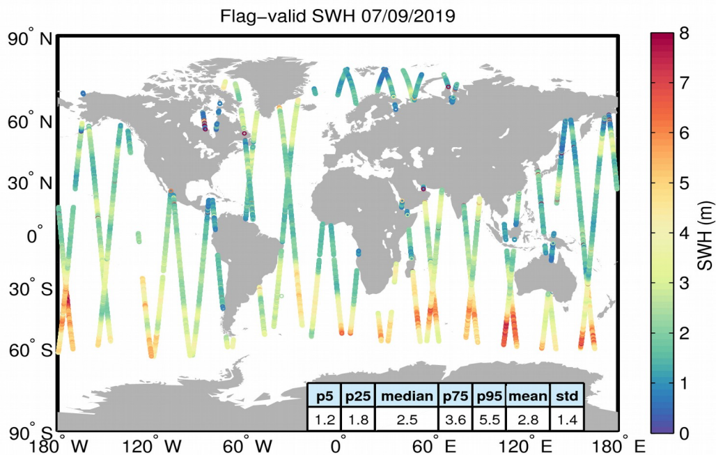
Figure 15. Geographical distribution of flag-valid SWH data over oceans and lakes for 07/09/2019. The statistical values shown in the table refer to the SWH in m and are calculated over all measurements shown in the figure.
