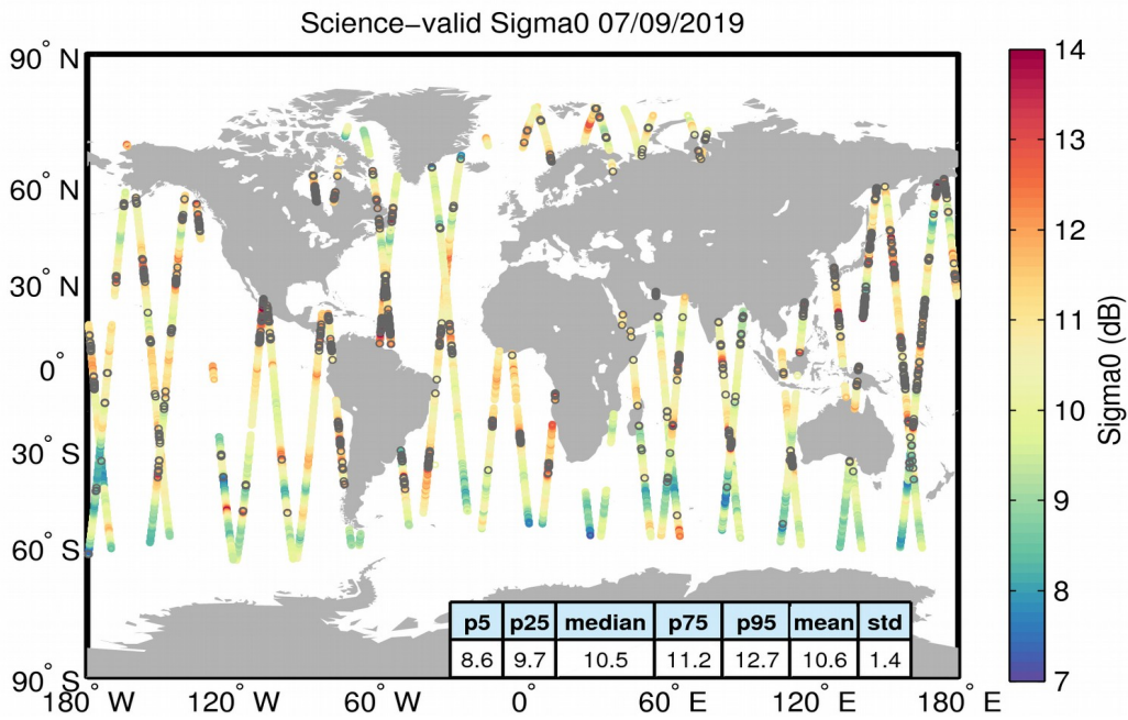
Figure 27. Geographical distribution of science-valid sigma0 data over oceans and lakes for 07/09/2019. The statistical values shown in the table refer to the sigma0 in dB and are calculated over all measurements shown in the figure. Gray circles denote records that have been rejected based on the editing criteria described in Table 4.
