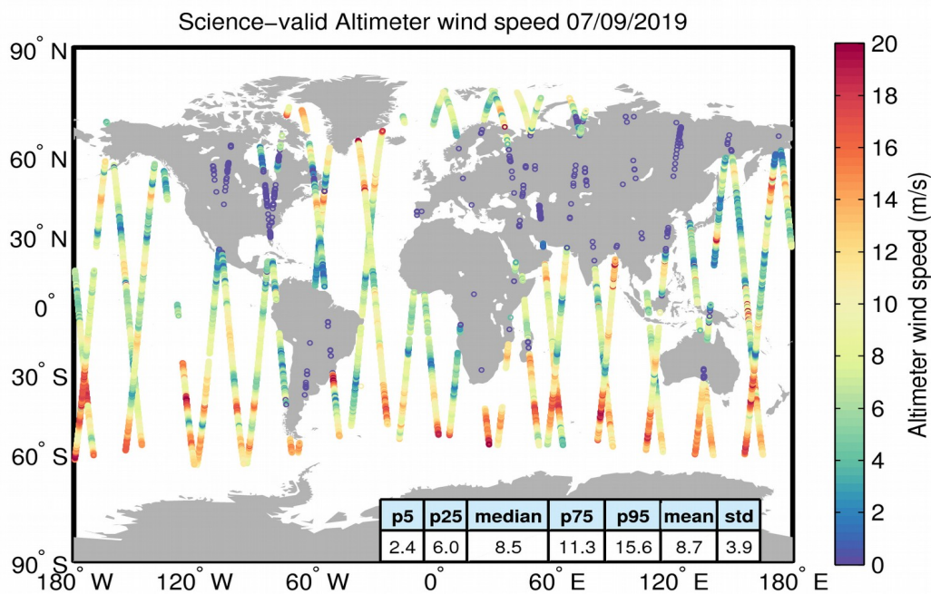
Figure 34. Geographical distribution of science-valid wind data over oceans and lakes for 07/09/2019. The statistical values shown in the table refer to the wind in m/s and are calculated over all measurements shown in the figure. Gray circles denote records that have been rejected based on the editing criteria described in Table 5.
