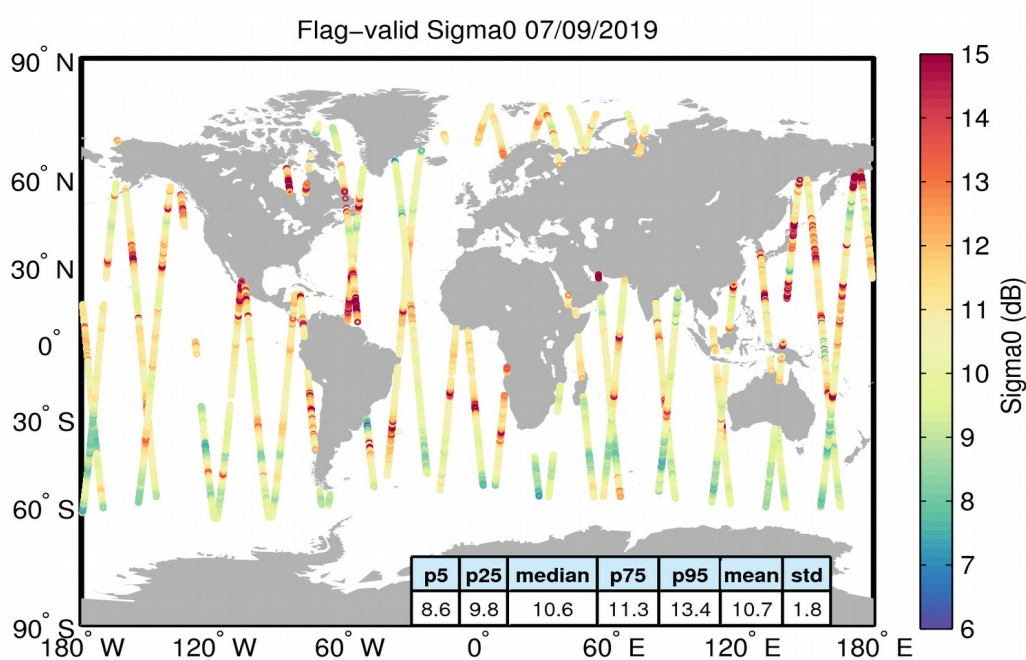
Figure 23. Geographical distribution of flag-valid sigma0 data over oceans and lakes for 07/09/2019. The statistical values shown in the table refer to the sigma0 in dB and are calculated over all measurements shown in the figure.
