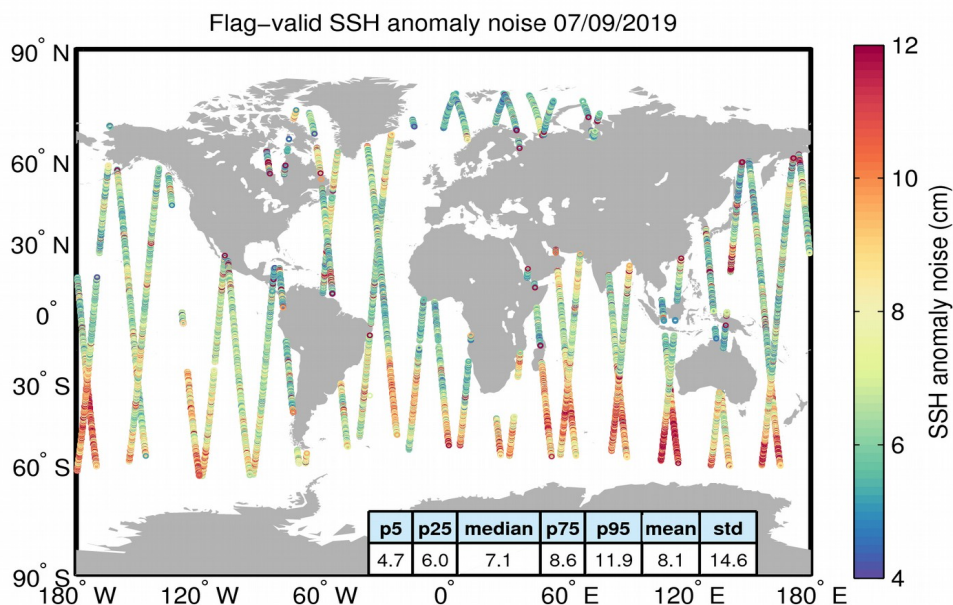
Figure 8. Geographical distribution of flag-valid 20-Hz SSH anomaly measurement noise over oceans and lakes for 07/09/2019. The statistical values shown in the table refer to the SSH anomaly noise and are calculated over all measurements shown in the figure.
