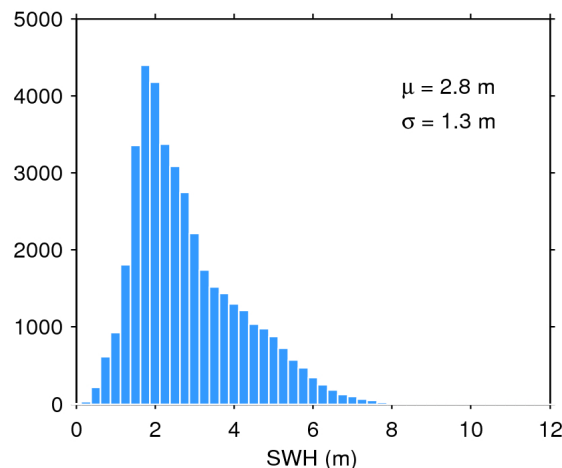
Figure 20. Histogram of science-valid SWH over oceans and lakes for 07/09/2019. The mean ( \mu ) and standard deviation ( \sigma ) are also shown. Note that values larger than 12 m are excluded from the histogram for the sake of readability but not from the computation of \mu and \sigma .
