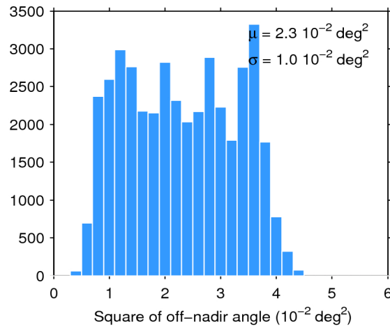
Figure 39. Histogram of flag-valid mispointing over oceans and lakes for 07/09/2019. The mean ( \mu ) and standard deviation ( \sigma ) are also shown. Note that values larger than 6 \cdot 10^{-2} \text{ deg}^2 are excluded from the histogram for the sake of readability but not from the computation of \mu and \sigma .
