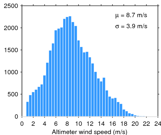
Figure 35. Histogram of science-valid wind over oceans and lakes for 07/09/2019. The mean ( \mu ) and standard deviation ( \sigma ) are also shown. Note that values larger than 24 m/s are excluded from the histogram for the sake of readability but not from the computation of \mu and \sigma .
