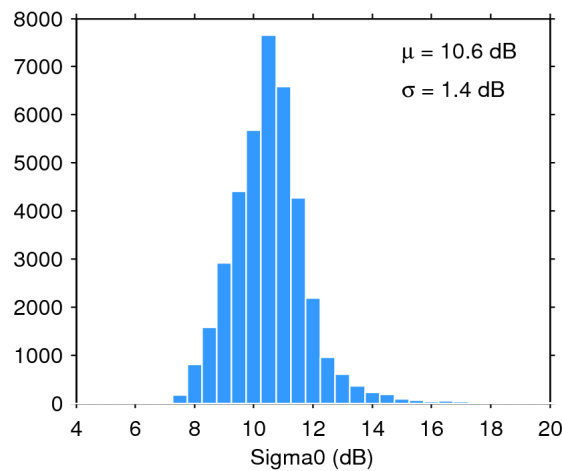
Figure 28. Histogram of science-valid sigma0 over oceans and lakes for 07/09/2019. The mean ( \mu ) and standard deviation ( \sigma ) are also shown. Note that values outside [4 20] dB are excluded from the histogram for the sake of readability but not from the computation of \mu and \sigma .
