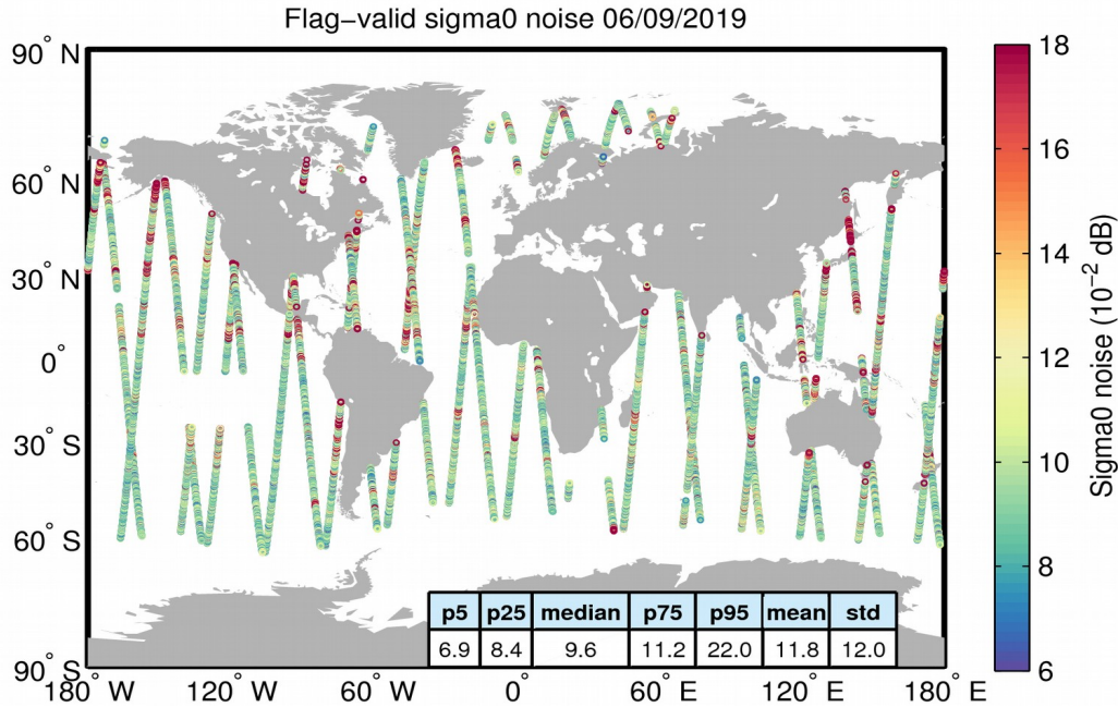
Figure 26. Geographical distribution of flag-valid 20-Hz sigma0 measurement noise over oceans and lakes for 06/09/2019. The statistical values shown in the table refer to the sigma0 noise and are calculated over all measurements shown in the figure.
