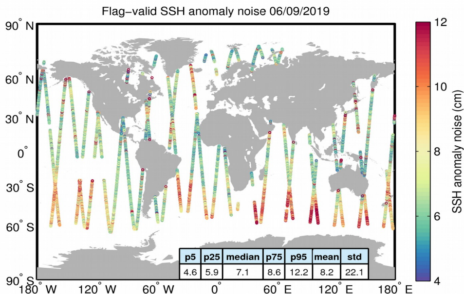
Figure 8. Geographical distribution of flag-valid 20-Hz SSH anomaly measurement noise over oceans and lakes for 06/09/2019. The statistical values shown in the table refer to the SSH anomaly noise and are calculated over all measurements shown in the figure.
