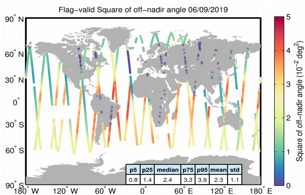
Figure 37. Geographical distribution of flag-valid mispointing data over oceans and lakes for 06/09/2019. The statistical values shown in the table refer to the mispointing in 10^{-2} \text{ deg}^2 and are calculated over all measurements shown in the figure.
