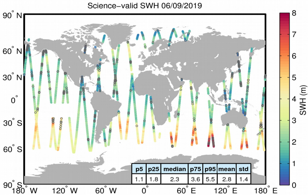
Figure 19. Geographical distribution of science-valid SWH data over oceans and lakes for 06/09/2019. The statistical values shown in the table refer to the SWH in m and are calculated over all measurements shown in the figure. Gray circles denote records that have been rejected based on the editing criteria described in Table 3.
