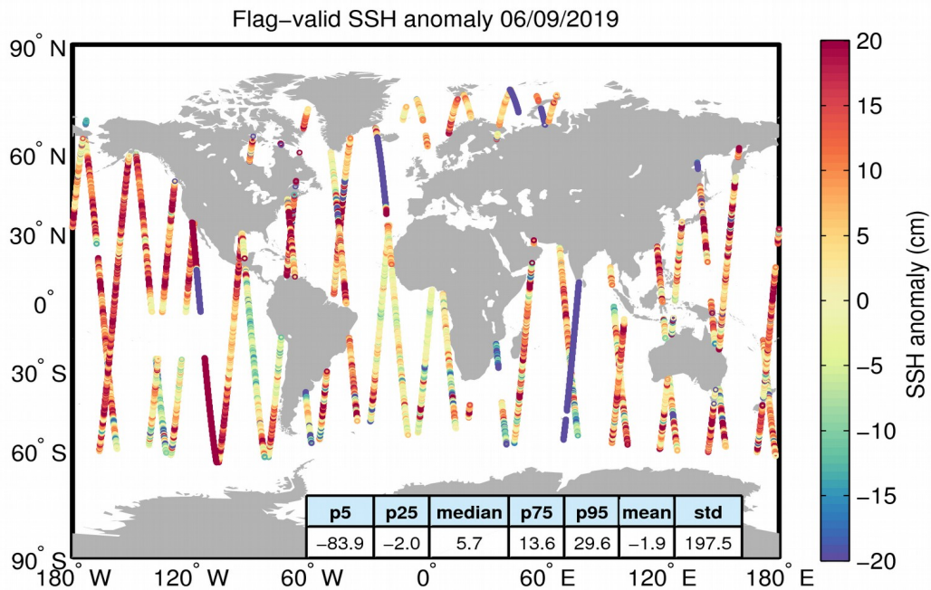
Figure 5. Geographical distribution of flag-valid 1-Hz SSH anomaly data over oceans and lakes for 06/09/2019. The statistical values shown in the table refer to the SSH anomaly in cm and are calculated over all measurements shown in the figure.
