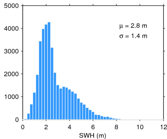
Figure 17. Histogram of flag-valid SWH over oceans and lakes for 06/09/2019. The mean ( \mu ) and standard deviation ( \sigma ) are also shown. Note that values larger than 12 m are excluded from the histogram for the sake of readability but not from the computation of \mu and \sigma .
