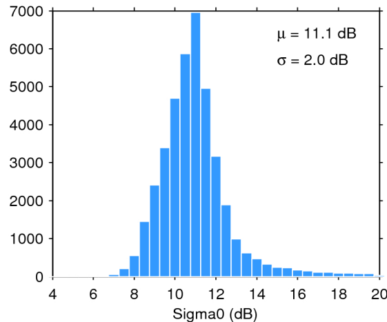
Figure 25. Histogram of flag-valid sigma0 over oceans and lakes for 06/09/2019. The mean ( \mu ) and standard deviation ( \sigma ) are also shown. Note that values outside [4 20] dB are excluded from the histogram for the sake of readability but not from the computation of \mu and \sigma .
