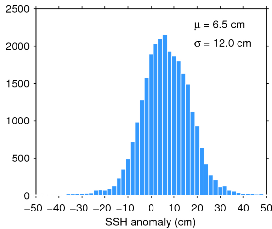
Figure 11. Histogram of science-valid SSH anomaly over oceans and lakes for 06/09/2019. The mean ( \mu ) and standard deviation ( \sigma ) are also shown. Note that values outside [-50 50] cm are excluded from the histogram for the sake of readability but not from the computation of \mu and \sigma .
