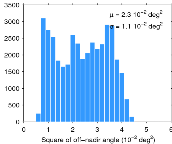
Figure 39. Histogram of flag-valid mispointing over oceans and lakes for 06/09/2019. The mean ( \mu ) and standard deviation ( \sigma ) are also shown. Note that values larger than 6 \cdot 10^{-2} \text{ deg}^2 are excluded from the histogram for the sake of readability but not from the computation of \mu and \sigma .
