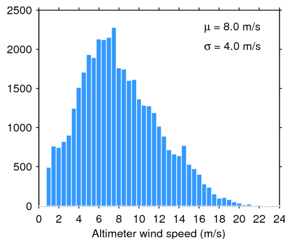
Figure 35. Histogram of science-valid wind over oceans and lakes for 06/09/2019. The mean ( \mu ) and standard deviation ( \sigma ) are also shown. Note that values larger than 24 m/s are excluded from the histogram for the sake of readability but not from the computation of \mu and \sigma .
