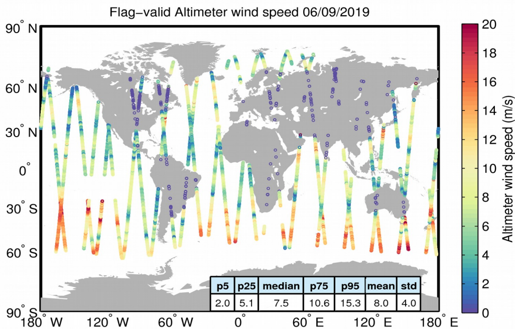
Figure 31. Geographical distribution of flag-valid wind data over oceans and lakes for 06/09/2019. The statistical values shown in the table refer to the wind in m/s and are calculated over all measurements shown in the figure.
