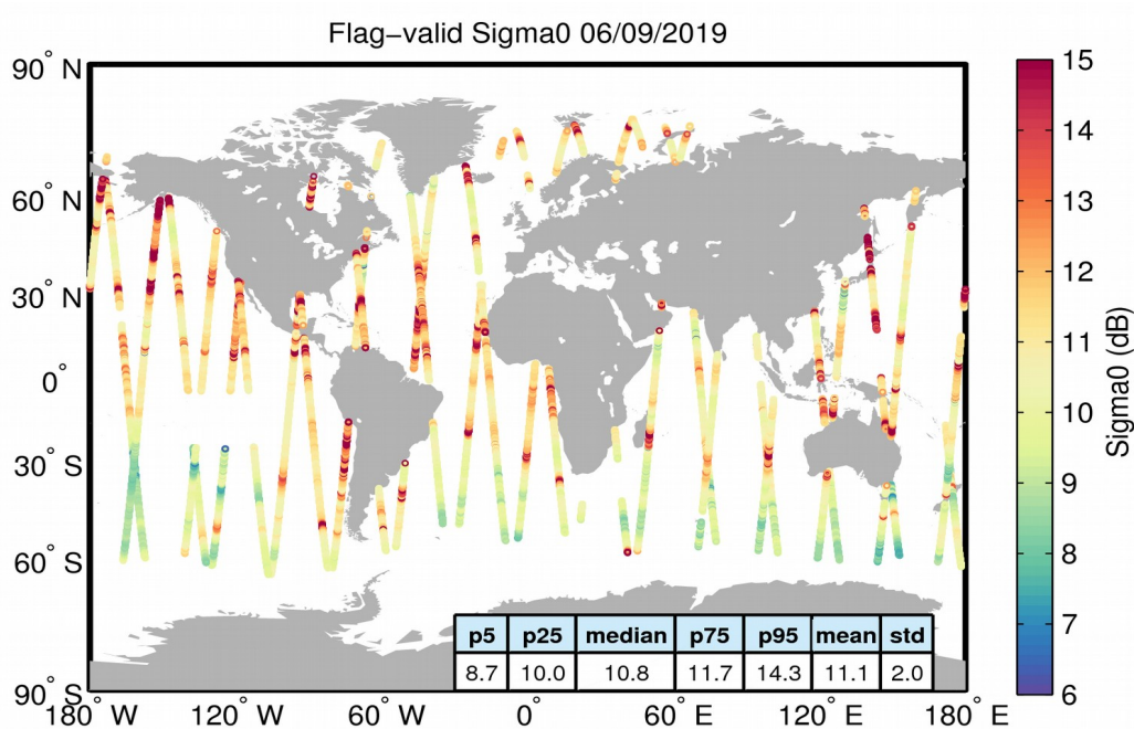
Figure 23. Geographical distribution of flag-valid sigma0 data over oceans and lakes for 06/09/2019. The statistical values shown in the table refer to the sigma0 in dB and are calculated over all measurements shown in the figure.
