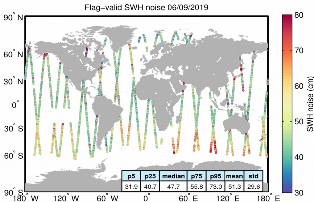
Figure 18. Geographical distribution of flag-valid 20-Hz SWH measurement noise over oceans and lakes for 06/09/2019. The statistical values shown in the figure refer to the SWH noise and are calculated over all measurements shown in the figure.
