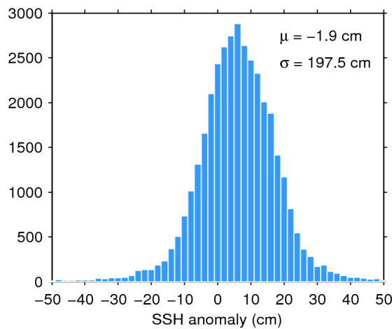
Figure 7. Histogram of flag-valid SSH anomaly over oceans and lakes for 06/09/2019. The mean ( \mu ) and standard deviation ( \sigma ) are also shown. Note that values outside [-50\ 50] cm are excluded from the histogram for the sake of readability but not from the computation of \mu and \sigma .
