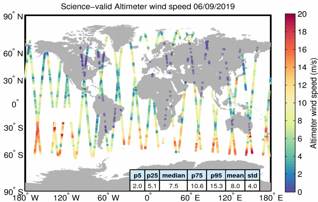
Figure 34. Geographical distribution of science-valid wind data over oceans and lakes for 06/09/2019. The statistical values shown in the table refer to the wind in m/s and are calculated over all measurements shown in the figure. Gray circles denote records that have been rejected based on the editing criteria described in Table 5.
