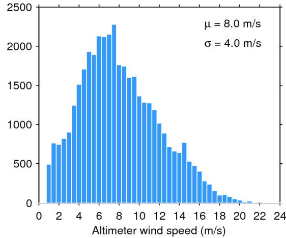
Figure 33. Histogram of flag-valid wind over oceans and lakes for 06/09/2019. The mean ( \mu ) and standard deviation ( \sigma ) are also shown. Note that values larger than 24 m/s are excluded from the histogram for the sake of readability but not from the computation of \mu and \sigma .
