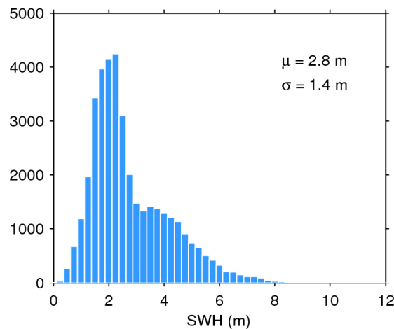
Figure 20. Histogram of science-valid SWH over oceans and lakes for 06/09/2019. The mean ( \mu ) and standard deviation ( \sigma ) are also shown. Note that values larger than 12 m are excluded from the histogram for the sake of readability but not from the computation of \mu and \sigma .
