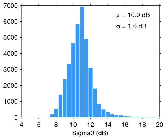
Figure 28. Histogram of science-valid sigma0 over oceans and lakes for 06/09/2019. The mean ( \mu ) and standard deviation ( \sigma ) are also shown. Note that values outside [4 20] dB are excluded from the histogram for the sake of readability but not from the computation of \mu and \sigma .
