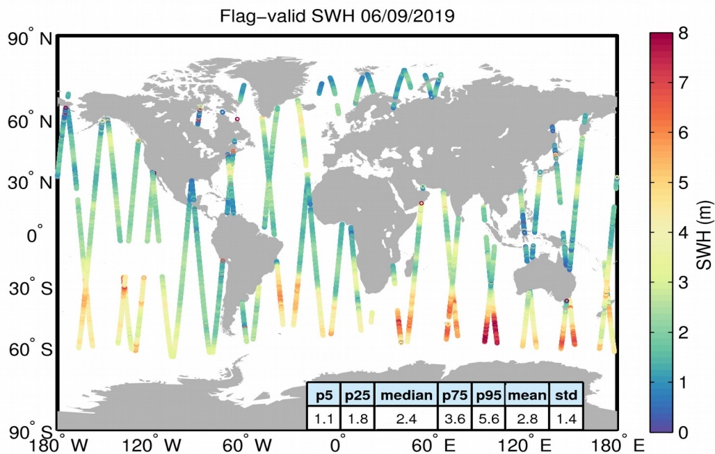
Figure 15. Geographical distribution of flag-valid SWH data over oceans and lakes for 06/09/2019. The statistical values shown in the table refer to the SWH in m and are calculated over all measurements shown in the figure.
