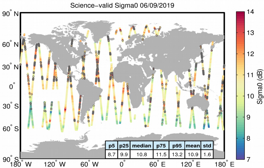
Figure 27. Geographical distribution of science-valid sigma0 data over oceans and lakes for 06/09/2019. The statistical values shown in the table refer to the sigma0 in dB and are calculated over all measurements shown in the figure. Gray circles denote records that have been rejected based on the editing criteria described in Table 4.
