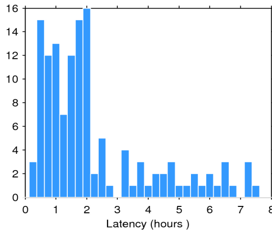
Figure 2. Histogram of the data latency for 06/09/2019. The y-axis denotes the number of files that are made available with a delay of x-hours with respect to the mean time of the records stored in the file.
