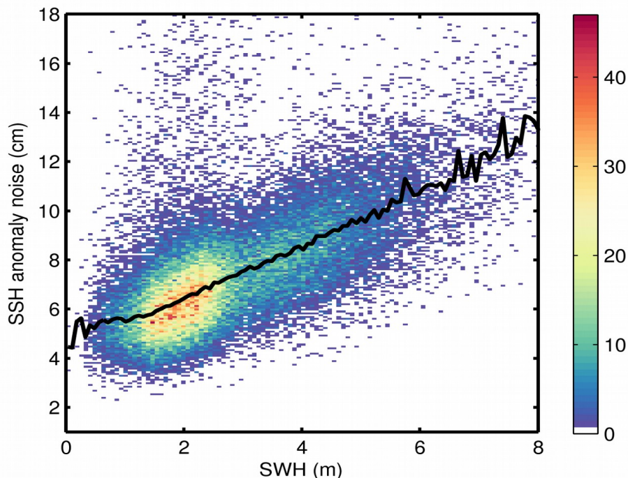
Figure 9. 2D histogram showing flag-valid SSH anomaly noise as a function of SWH for 06/09/2019. The black line denotes the median SSH anomaly noise as a function of SWH.
