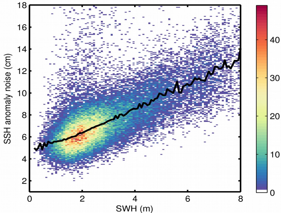
Figure 9. 2D histogram showing flag-valid SSH anomaly noise as a function of SWH for 05/09/2019. The black line denotes the median SSH anomaly noise as a function of SWH.
