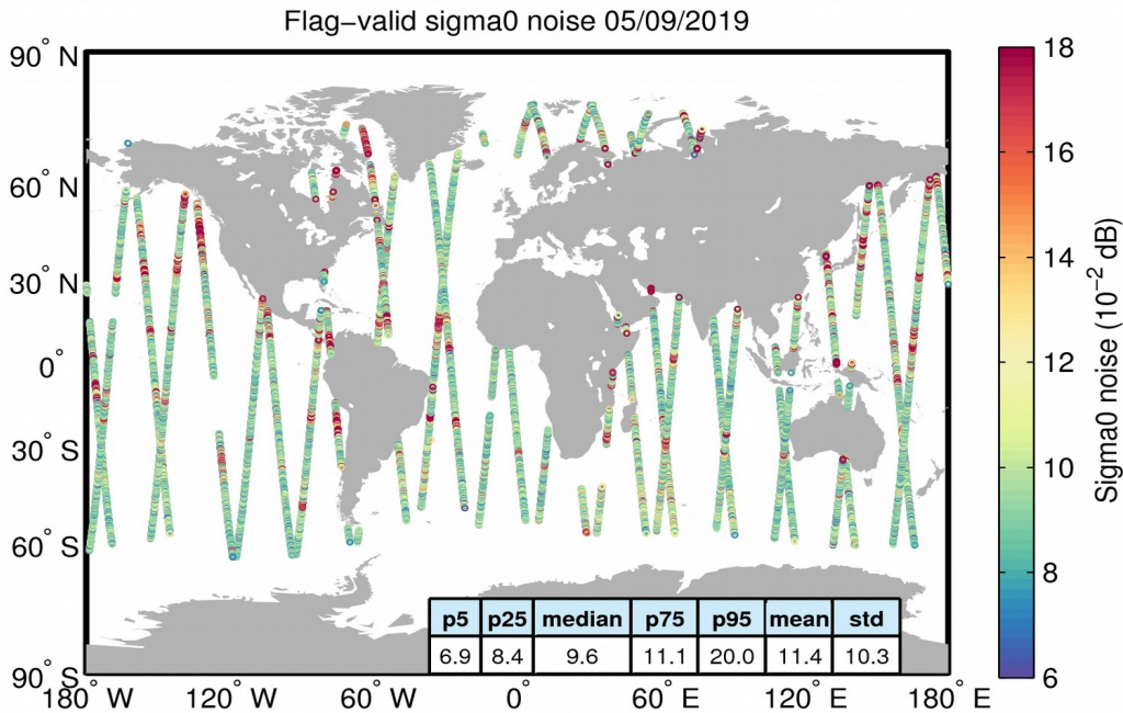
Figure 26. Geographical distribution of flag-valid 20-Hz sigma0 measurement noise over oceans and lakes for 05/09/2019. The statistical values shown in the table refer to the sigma0 noise and are calculated over all measurements shown in the figure.
