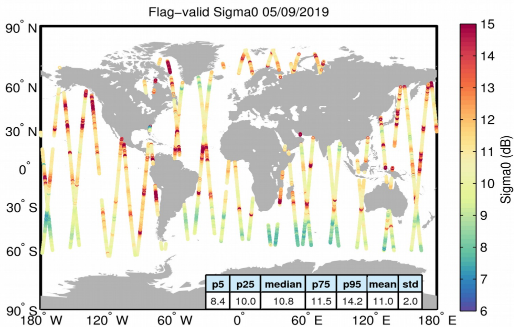
Figure 23. Geographical distribution of flag-valid sigma0 data over oceans and lakes for 05/09/2019. The statistical values shown in the table refer to the sigma0 in dB and are calculated over all measurements shown in the figure.
