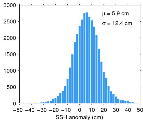
Figure 11. Histogram of science-valid SSH anomaly over oceans and lakes for 05/09/2019. The mean ( \mu ) and standard deviation ( \sigma ) are also shown. Note that values outside [-50 50] cm are excluded from the histogram for the sake of readability but not from the computation of \mu and \sigma .
