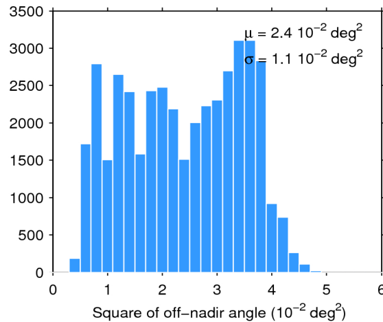
Figure 39. Histogram of flag-valid mispointing over oceans and lakes for 05/09/2019. The mean ( \mu ) and standard deviation ( \sigma ) are also shown. Note that values larger than 6 \cdot 10^{-2} \text{ deg}^2 are excluded from the histogram for the sake of readability but not from the computation of \mu and \sigma .
