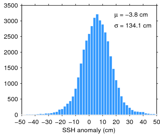
Figure 7. Histogram of flag-valid SSH anomaly over oceans and lakes for 05/09/2019. The mean ( \mu ) and standard deviation ( \sigma ) are also shown. Note that values outside [-50\ 50] cm are excluded from the histogram for the sake of readability but not from the computation of \mu and \sigma .
