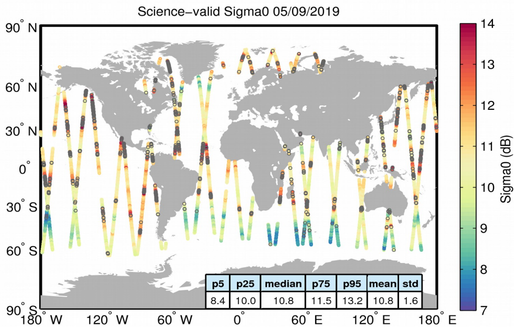
Figure 27. Geographical distribution of science-valid sigma0 data over oceans and lakes for 05/09/2019. The statistical values shown in the table refer to the sigma0 in dB and are calculated over all measurements shown in the figure. Gray circles denote records that have been rejected based on the editing criteria described in Table 4.
