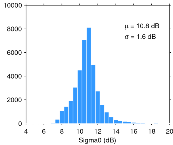
Figure 28. Histogram of science-valid sigma0 over oceans and lakes for 05/09/2019. The mean ( \mu ) and standard deviation ( \sigma ) are also shown. Note that values outside [4 20] dB are excluded from the histogram for the sake of readability but not from the computation of \mu and \sigma .
