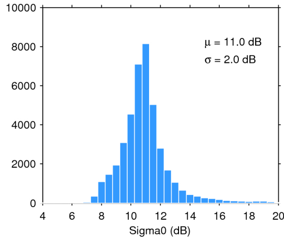
Figure 25. Histogram of flag-valid sigma0 over oceans and lakes for 05/09/2019. The mean ( \mu ) and standard deviation ( \sigma ) are also shown. Note that values outside [4 20] dB are excluded from the histogram for the sake of readability but not from the computation of \mu and \sigma .
