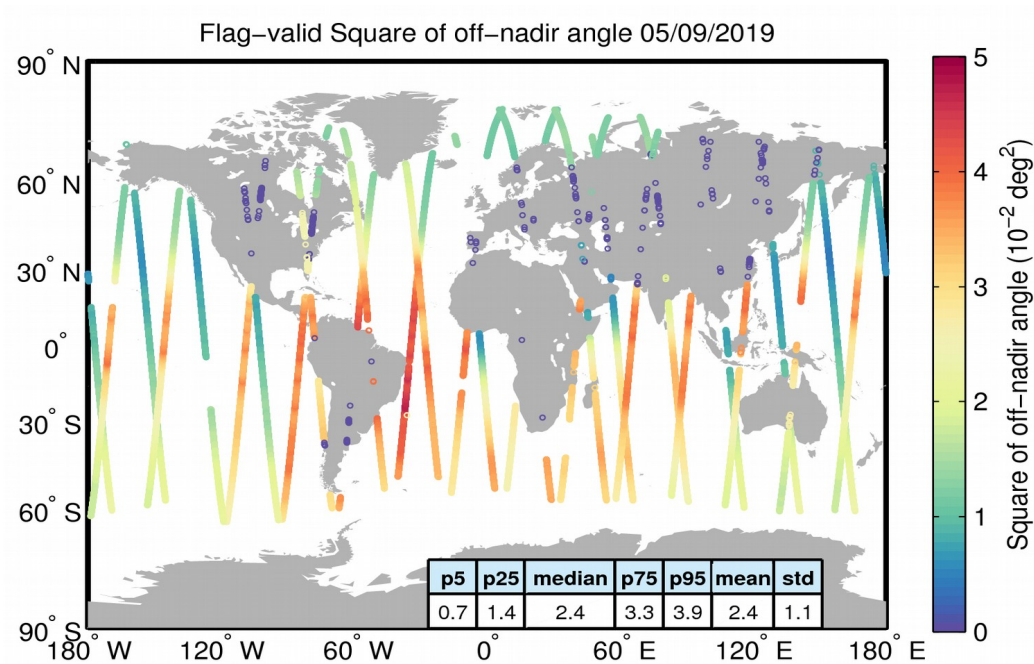
Figure 37. Geographical distribution of flag-valid mispointing data over oceans and lakes for 05/09/2019. The statistical values shown in the table refer to the mispointing in 10^{-2} \text{ deg}^2 and are calculated over all measurements shown in the figure.
