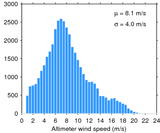
Figure 33. Histogram of flag-valid wind over oceans and lakes for 05/09/2019. The mean ( \mu ) and standard deviation ( \sigma ) are also shown. Note that values larger than 24 m/s are excluded from the histogram for the sake of readability but not from the computation of \mu and \sigma .
