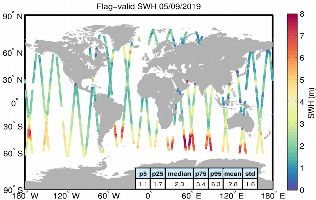
Figure 15. Geographical distribution of flag-valid SWH data over oceans and lakes for 05/09/2019. The statistical values shown in the table refer to the SWH in m and are calculated over all measurements shown in the figure.
