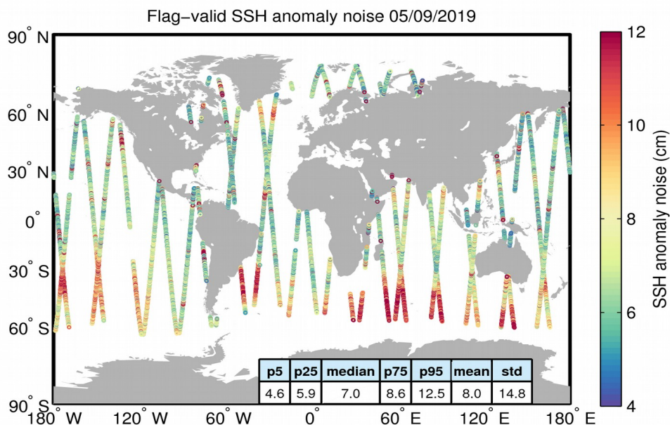
Figure 8. Geographical distribution of flag-valid 20-Hz SSH anomaly measurement noise over oceans and lakes for 05/09/2019. The statistical values shown in the table refer to the SSH anomaly noise and are calculated over all measurements shown in the figure.
