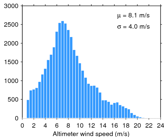
Figure 35. Histogram of science-valid wind over oceans and lakes for 05/09/2019. The mean ( \mu ) and standard deviation ( \sigma ) are also shown. Note that values larger than 24 m/s are excluded from the histogram for the sake of readability but not from the computation of \mu and \sigma .
