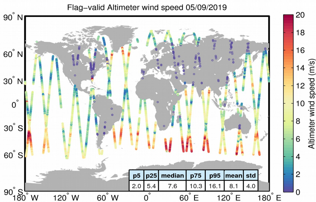
Figure 31. Geographical distribution of flag-valid wind data over oceans and lakes for 05/09/2019. The statistical values shown in the table refer to the wind in m/s and are calculated over all measurements shown in the figure.
