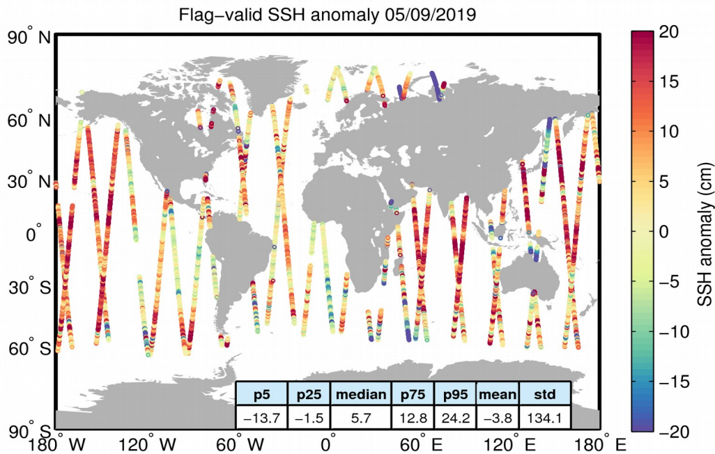
Figure 5. Geographical distribution of flag-valid 1-Hz SSH anomaly data over oceans and lakes for 05/09/2019. The statistical values shown in the table refer to the SSH anomaly in cm and are calculated over all measurements shown in the figure.
