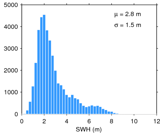
Figure 20. Histogram of science-valid SWH over oceans and lakes for 05/09/2019. The mean ( \mu ) and standard deviation ( \sigma ) are also shown. Note that values larger than 12 m are excluded from the histogram for the sake of readability but not from the computation of \mu and \sigma .
