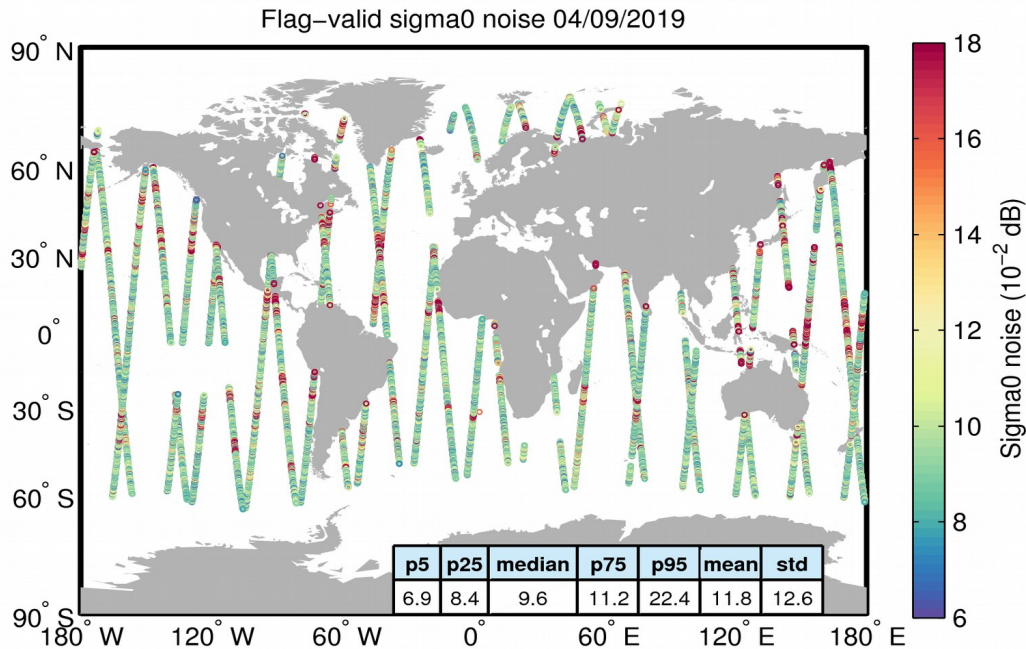
Figure 26. Geographical distribution of flag-valid 20-Hz sigma0 measurement noise over oceans and lakes for 04/09/2019. The statistical values shown in the table refer to the sigma0 noise and are calculated over all measurements shown in the figure.
