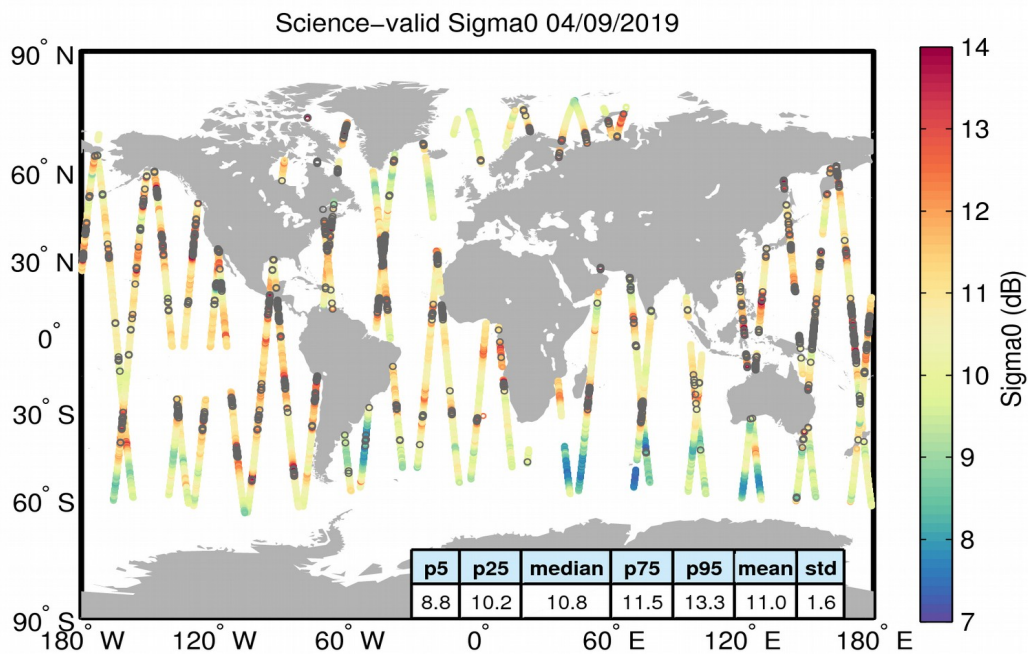
Figure 27. Geographical distribution of science-valid sigma0 data over oceans and lakes for 04/09/2019. The statistical values shown in the table refer to the sigma0 in dB and are calculated over all measurements shown in the figure. Gray circles denote records that have been rejected based on the editing criteria described in Table 4.
