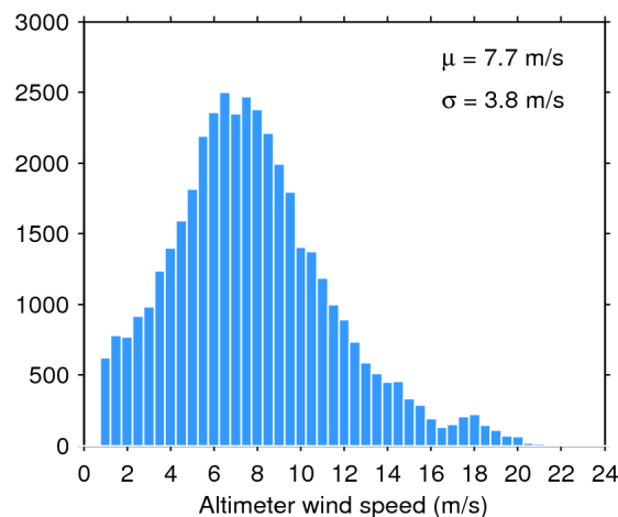
Figure 35. Histogram of science-valid wind over oceans and lakes for 04/09/2019. The mean ( \mu ) and standard deviation ( \sigma ) are also shown. Note that values larger than 24 m/s are excluded from the histogram for the sake of readability but not from the computation of \mu and \sigma .
