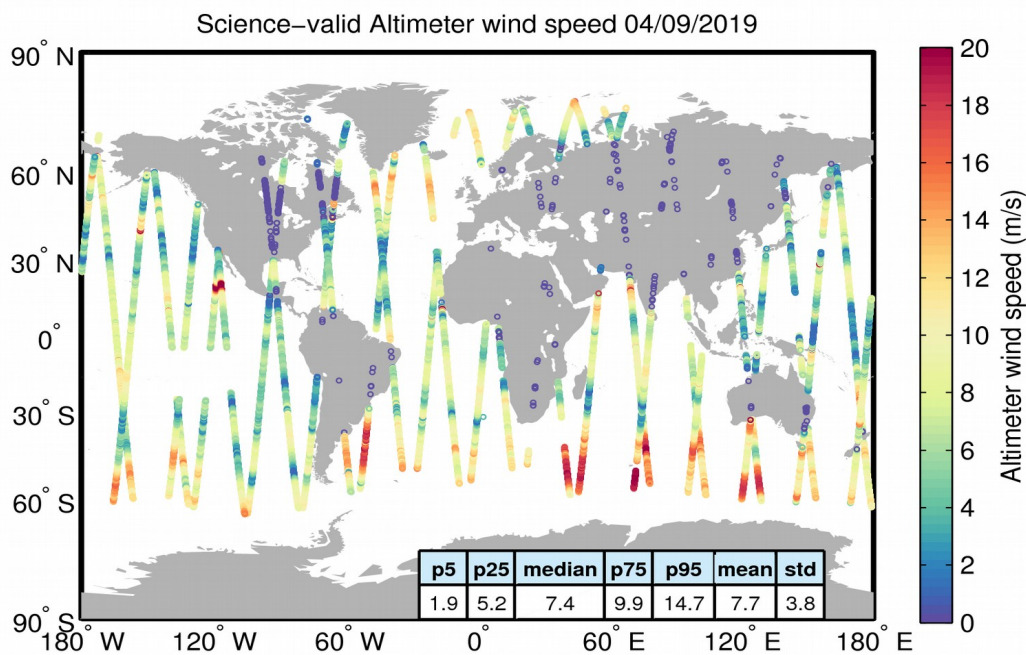
Figure 34. Geographical distribution of science-valid wind data over oceans and lakes for 04/09/2019. The statistical values shown in the table refer to the wind in m/s and are calculated over all measurements shown in the figure. Gray circles denote records that have been rejected based on the editing criteria described in Table 5.
