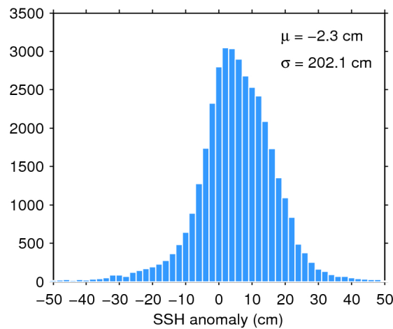
Figure 7. Histogram of flag-valid SSH anomaly over oceans and lakes for 04/09/2019. The mean ( \mu ) and standard deviation ( \sigma ) are also shown. Note that values outside [-50 50] cm are excluded from the histogram for the sake of readability but not from the computation of \mu and \sigma .
