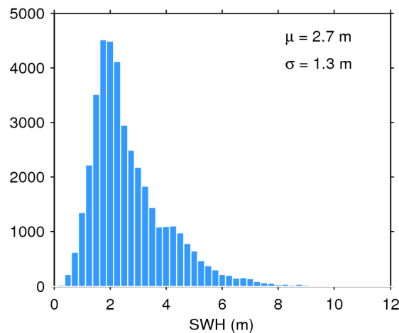
Figure 20. Histogram of science-valid SWH over oceans and lakes for 04/09/2019. The mean ( \mu ) and standard deviation ( \sigma ) are also shown. Note that values larger than 12 m are excluded from the histogram for the sake of readability but not from the computation of \mu and \sigma .
