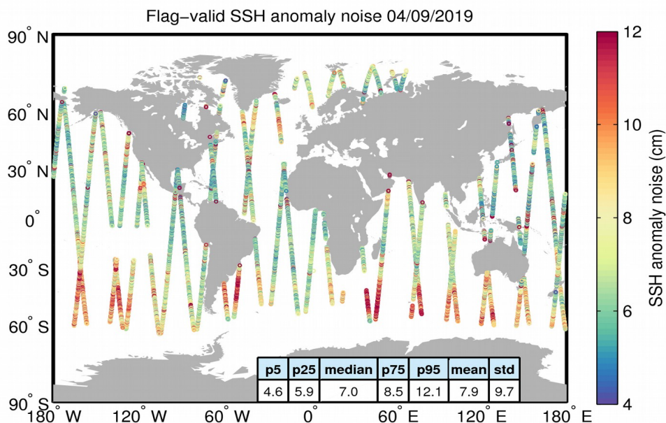
Figure 8. Geographical distribution of flag-valid 20-Hz SSH anomaly measurement noise over oceans and lakes for 04/09/2019. The statistical values shown in the table refer to the SSH anomaly noise and are calculated over all measurements shown in the figure.
