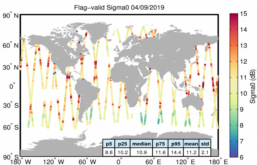
Figure 23. Geographical distribution of flag-valid sigma0 data over oceans and lakes for 04/09/2019. The statistical values shown in the table refer to the sigma0 in dB and are calculated over all measurements shown in the figure.
