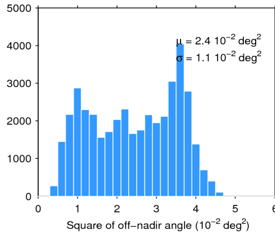
Figure 39. Histogram of flag-valid mispointing over oceans and lakes for 04/09/2019. The mean ( \mu ) and standard deviation ( \sigma ) are also shown. Note that values larger than 6 \cdot 10^{-2} \text{ deg}^2 are excluded from the histogram for the sake of readability but not from the computation of \mu and \sigma .
