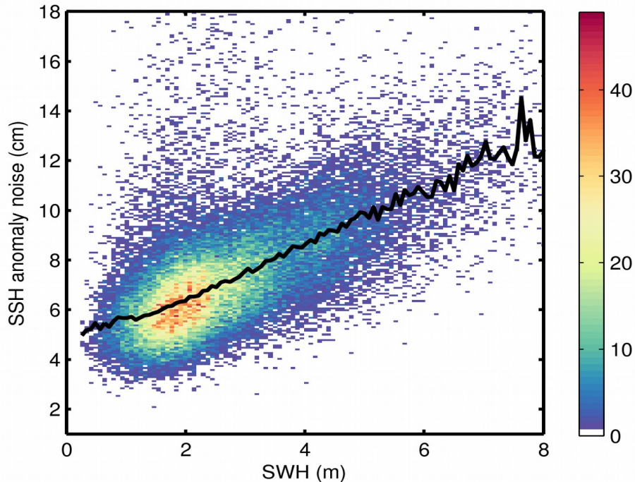
Figure 9. 2D histogram showing flag-valid SSH anomaly noise as a function of SWH for 04/09/2019. The black line denotes the median SSH anomaly noise as a function of SWH.
