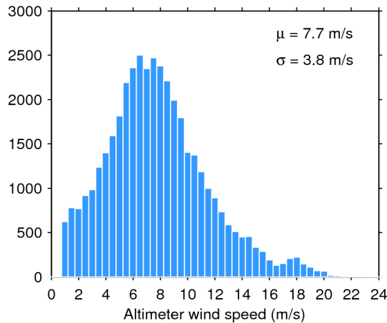
Figure 33. Histogram of flag-valid wind over oceans and lakes for 04/09/2019. The mean ( \mu ) and standard deviation ( \sigma ) are also shown. Note that values larger than 24 m/s are excluded from the histogram for the sake of readability but not from the computation of \mu and \sigma .
