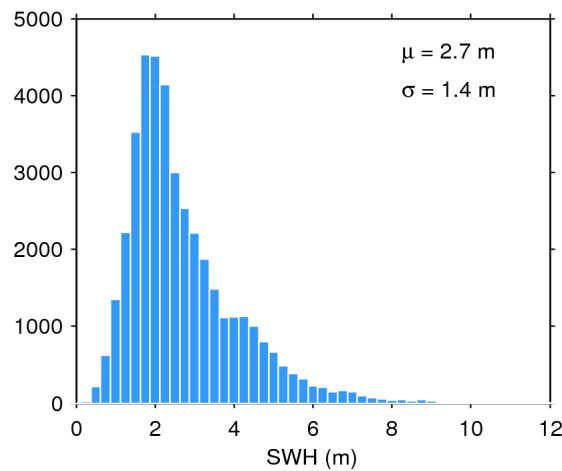
Figure 17. Histogram of flag-valid SWH over oceans and lakes for 04/09/2019. The mean ( \mu ) and standard deviation ( \sigma ) are also shown. Note that values larger than 12 m are excluded from the histogram for the sake of readability but not from the computation of \mu and \sigma .
