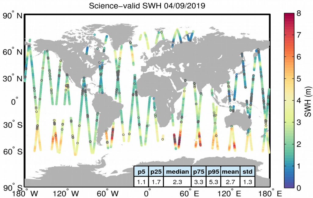
Figure 19. Geographical distribution of science-valid SWH data over oceans and lakes for 04/09/2019. The statistical values shown in the table refer to the SWH in m and are calculated over all measurements shown in the figure. Gray circles denote records that have been rejected based on the editing criteria described in Table 3.
