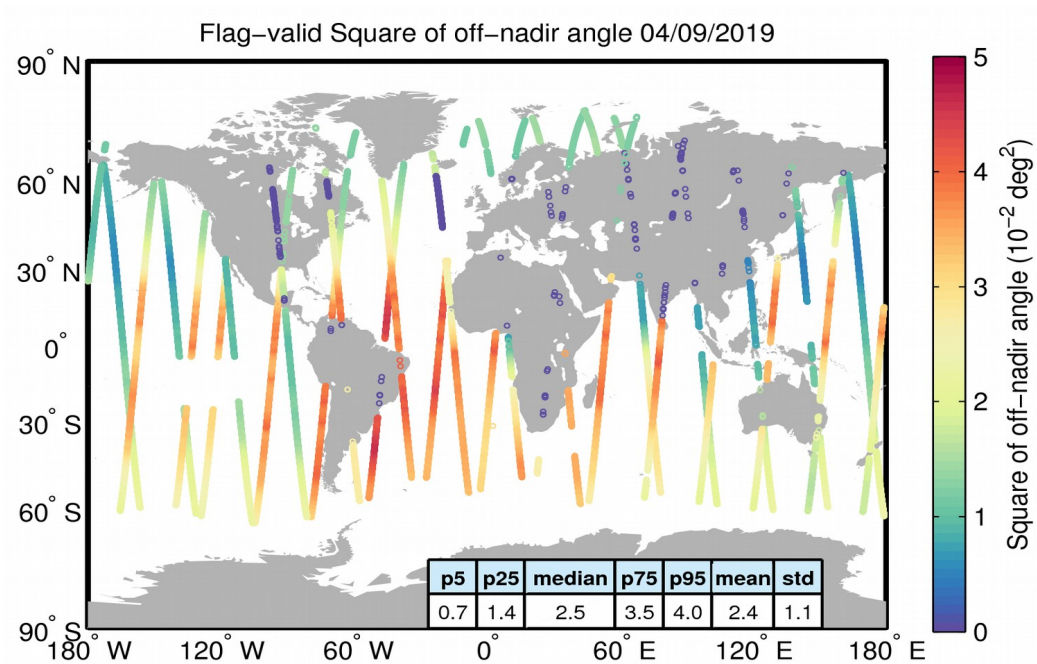
Figure 37. Geographical distribution of flag-valid mispointing data over oceans and lakes for 04/09/2019. The statistical values shown in the table refer to the mispointing in 10^{-2} \text{ deg}^2 and are calculated over all measurements shown in the figure.
