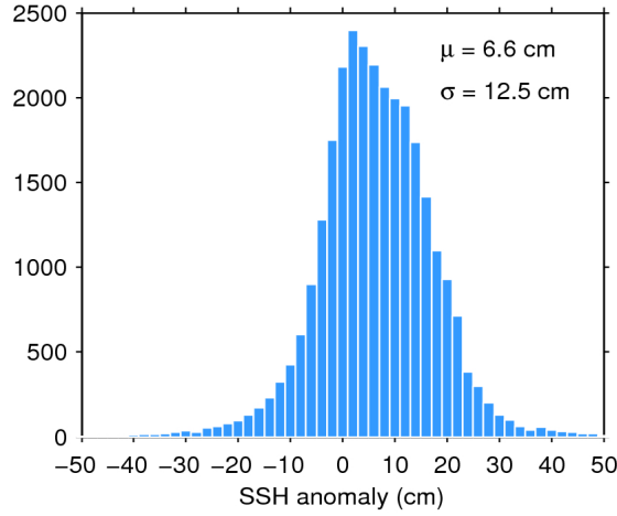
Figure 11. Histogram of science-valid SSH anomaly over oceans and lakes for 04/09/2019. The mean ( \mu ) and standard deviation ( \sigma ) are also shown. Note that values outside [-50 50] cm are excluded from the histogram for the sake of readability but not from the computation of \mu and \sigma .
