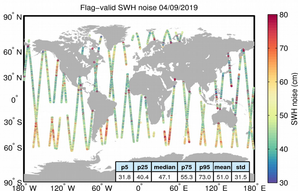
Figure 18. Geographical distribution of flag-valid 20-Hz SWH measurement noise over oceans and lakes for 04/09/2019. The statistical values shown in the figure refer to the SWH noise and are calculated over all measurements shown in the figure.
