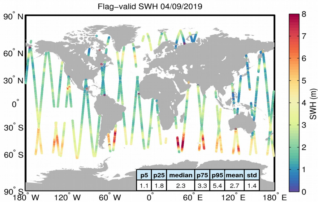
Figure 15. Geographical distribution of flag-valid SWH data over oceans and lakes for 04/09/2019. The statistical values shown in the table refer to the SWH in m and are calculated over all measurements shown in the figure.
