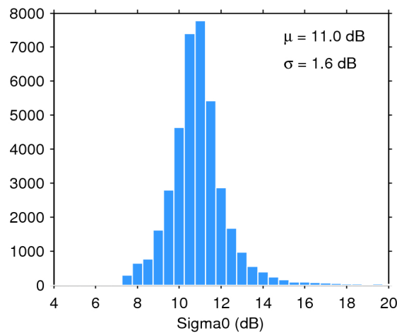
Figure 28. Histogram of science-valid sigma0 over oceans and lakes for 04/09/2019. The mean ( \mu ) and standard deviation ( \sigma ) are also shown. Note that values outside [4 20] dB are excluded from the histogram for the sake of readability but not from the computation of \mu and \sigma .
