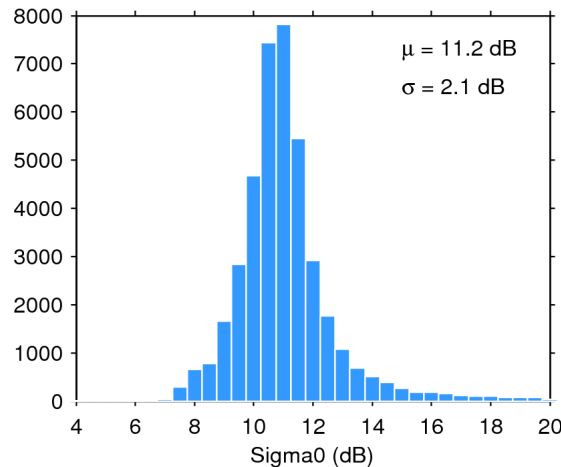
Figure 25. Histogram of flag-valid sigma0 over oceans and lakes for 04/09/2019. The mean ( \mu ) and standard deviation ( \sigma ) are also shown. Note that values outside [4 20] dB are excluded from the histogram for the sake of readability but not from the computation of \mu and \sigma .
