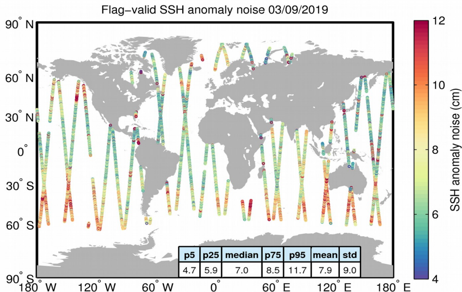
Figure 8. Geographical distribution of flag-valid 20-Hz SSH anomaly measurement noise over oceans and lakes for 03/09/2019. The statistical values shown in the table refer to the SSH anomaly noise and are calculated over all measurements shown in the figure.
