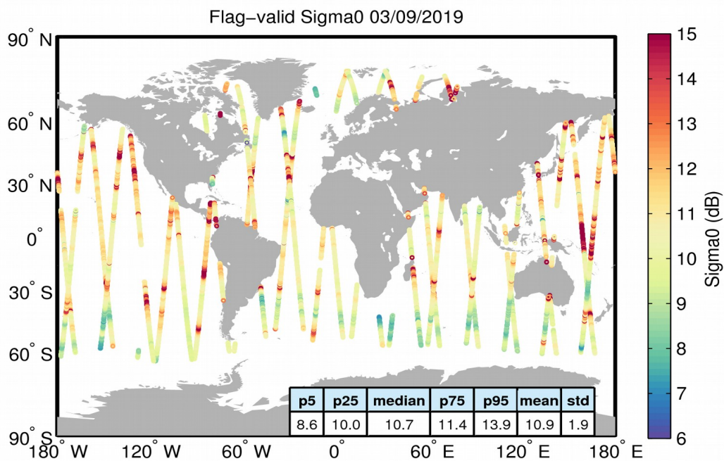
Figure 23. Geographical distribution of flag-valid sigma0 data over oceans and lakes for 03/09/2019. The statistical values shown in the table refer to the sigma0 in dB and are calculated over all measurements shown in the figure.
