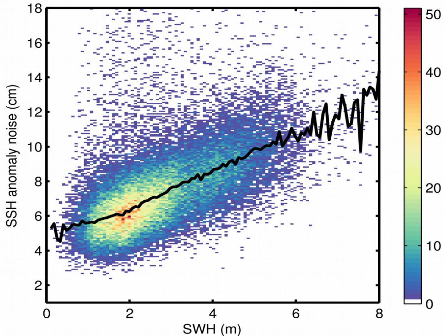
Figure 9. 2D histogram showing flag-valid SSH anomaly noise as a function of SWH for 03/09/2019. The black line denotes the median SSH anomaly noise as a function of SWH.
