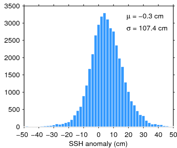
Figure 7. Histogram of flag-valid SSH anomaly over oceans and lakes for 03/09/2019. The mean ( \mu ) and standard deviation ( \sigma ) are also shown. Note that values outside [-50\ 50] cm are excluded from the histogram for the sake of readability but not from the computation of \mu and \sigma .
