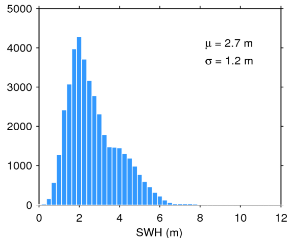
Figure 20. Histogram of science-valid SWH over oceans and lakes for 03/09/2019. The mean ( \mu ) and standard deviation ( \sigma ) are also shown. Note that values larger than 12 m are excluded from the histogram for the sake of readability but not from the computation of \mu and \sigma .
