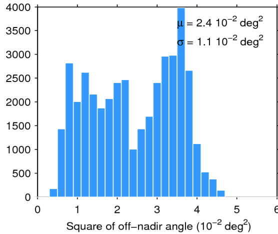
Figure 39. Histogram of flag-valid mispointing over oceans and lakes for 03/09/2019. The mean ( \mu ) and standard deviation ( \sigma ) are also shown. Note that values larger than 6 \cdot 10^{-2} \text{ deg}^2 are excluded from the histogram for the sake of readability but not from the computation of \mu and \sigma .
