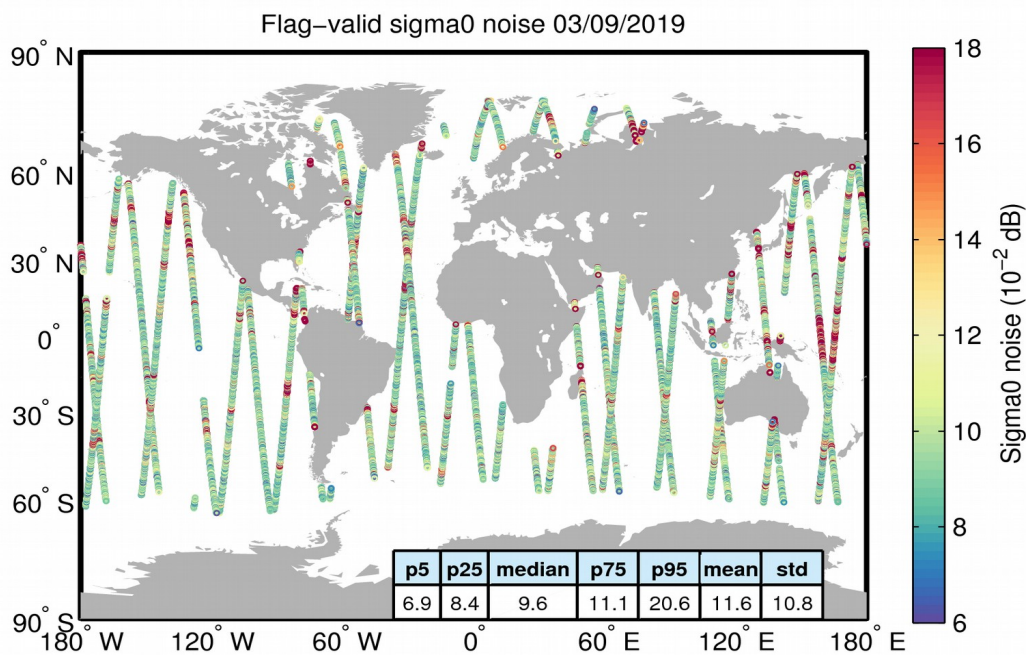
Figure 26. Geographical distribution of flag-valid 20-Hz sigma0 measurement noise over oceans and lakes for 03/09/2019. The statistical values shown in the table refer to the sigma0 noise and are calculated over all measurements shown in the figure.
