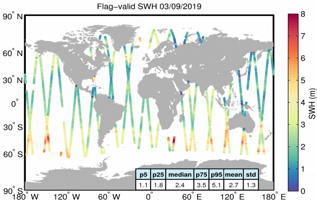
Figure 15. Geographical distribution of flag-valid SWH data over oceans and lakes for 03/09/2019. The statistical values shown in the table refer to the SWH in m and are calculated over all measurements shown in the figure.
