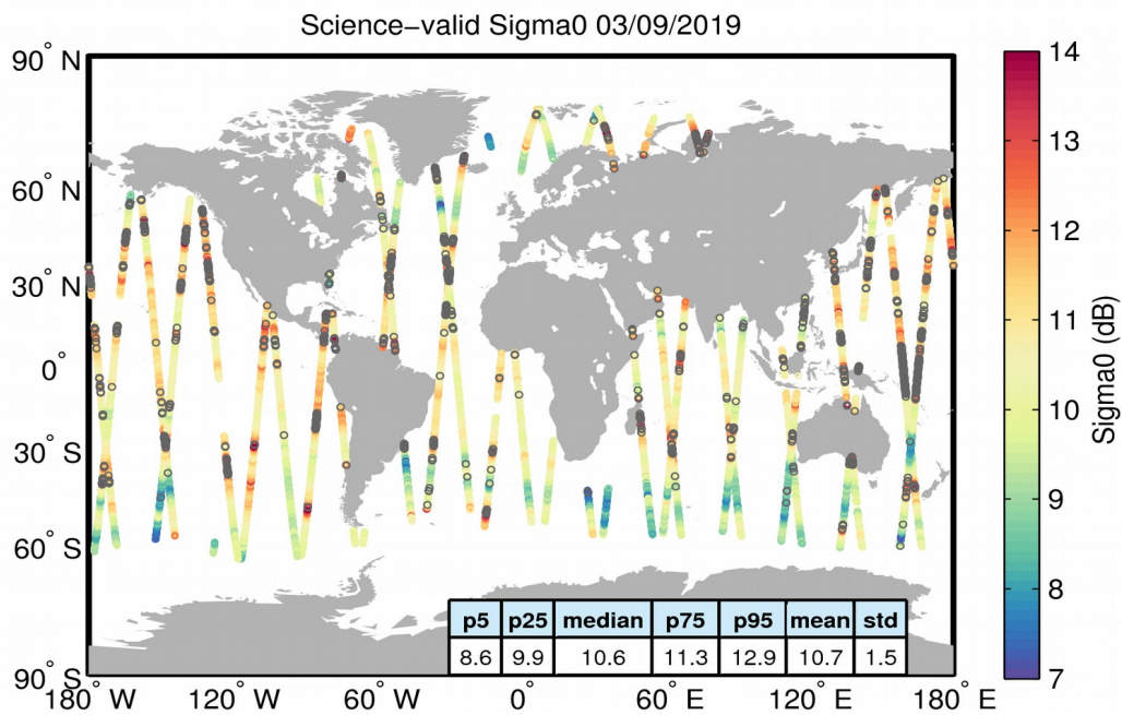
Figure 27. Geographical distribution of science-valid sigma0 data over oceans and lakes for 03/09/2019. The statistical values shown in the table refer to the sigma0 in dB and are calculated over all measurements shown in the figure. Gray circles denote records that have been rejected based on the editing criteria described in Table 4.
