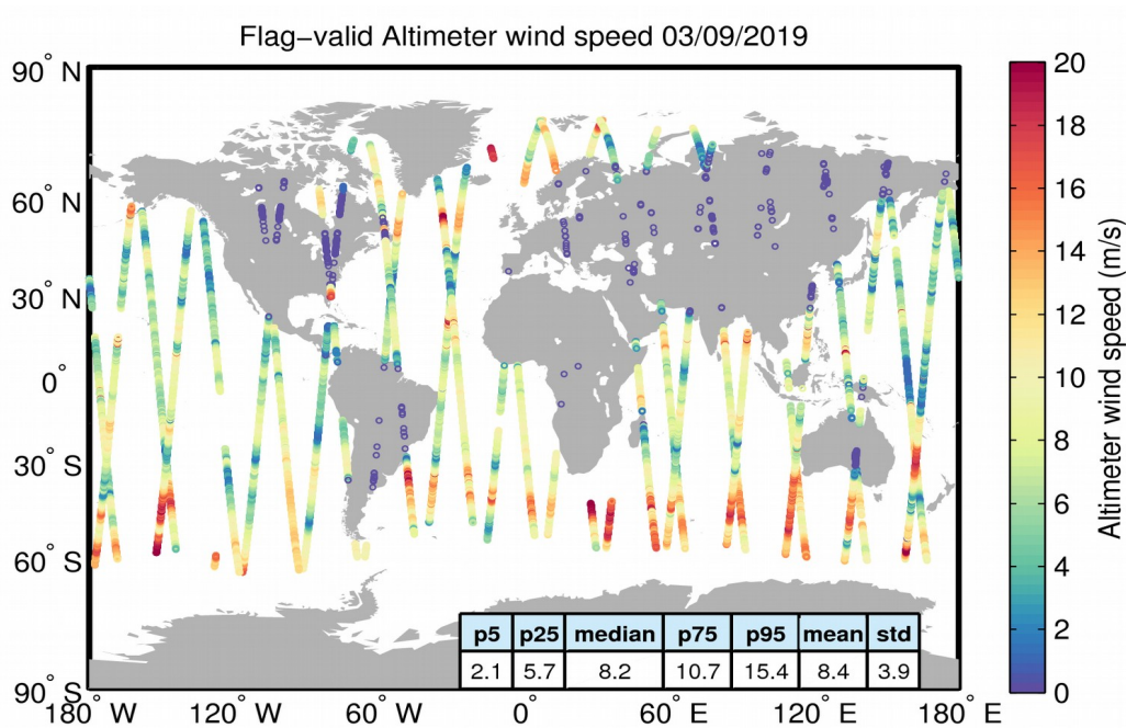
Figure 31. Geographical distribution of flag-valid wind data over oceans and lakes for 03/09/2019. The statistical values shown in the table refer to the wind in m/s and are calculated over all measurements shown in the figure.
