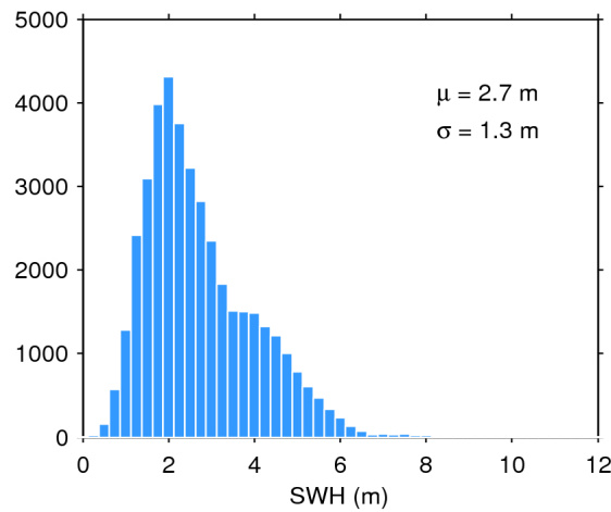
Figure 17. Histogram of flag-valid SWH over oceans and lakes for 03/09/2019. The mean ( \mu ) and standard deviation ( \sigma ) are also shown. Note that values larger than 12 m are excluded from the histogram for the sake of readability but not from the computation of \mu and \sigma .
