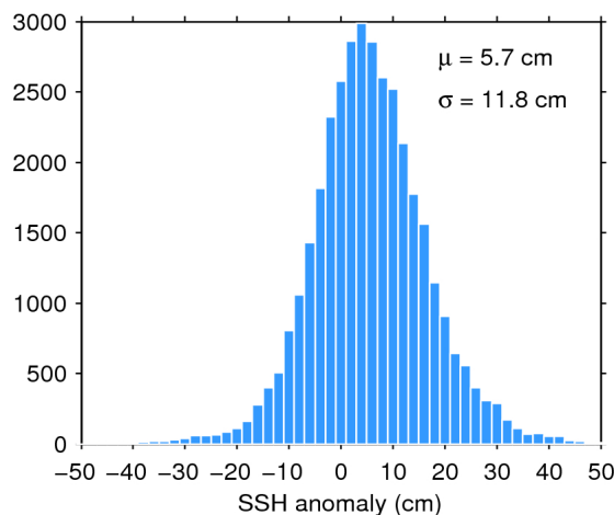
Figure 11. Histogram of science-valid SSH anomaly over oceans and lakes for 03/09/2019. The mean ( \mu ) and standard deviation ( \sigma ) are also shown. Note that values outside [-50 50] cm are excluded from the histogram for the sake of readability but not from the computation of \mu and \sigma .
