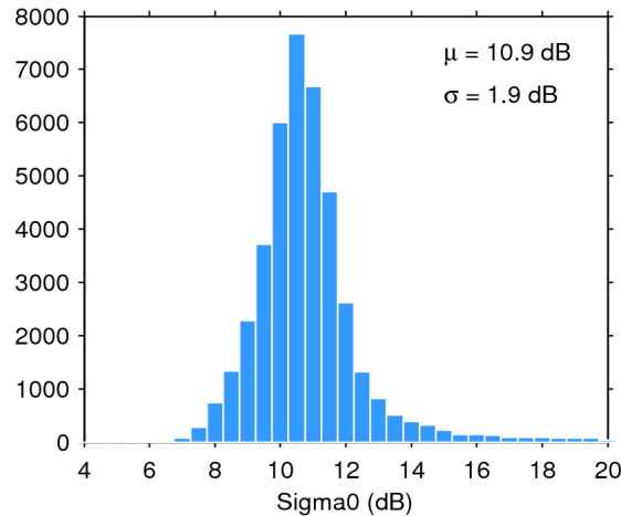
Figure 25. Histogram of flag-valid sigma0 over oceans and lakes for 03/09/2019. The mean ( \mu ) and standard deviation ( \sigma ) are also shown. Note that values outside [4 20] dB are excluded from the histogram for the sake of readability but not from the computation of \mu and \sigma .
