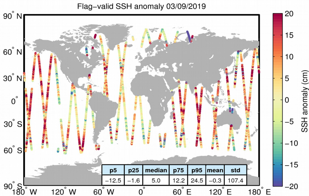
Figure 5. Geographical distribution of flag-valid 1-Hz SSH anomaly data over oceans and lakes for 03/09/2019. The statistical values shown in the table refer to the SSH anomaly in cm and are calculated over all measurements shown in the figure.
