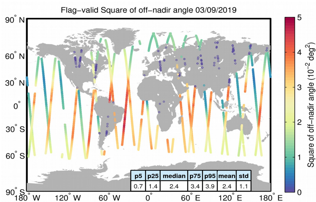
Figure 37. Geographical distribution of flag-valid mispointing data over oceans and lakes for 03/09/2019. The statistical values shown in the table refer to the mispointing in 10^{-2} deg 2 and are calculated over all measurements shown in the figure.
