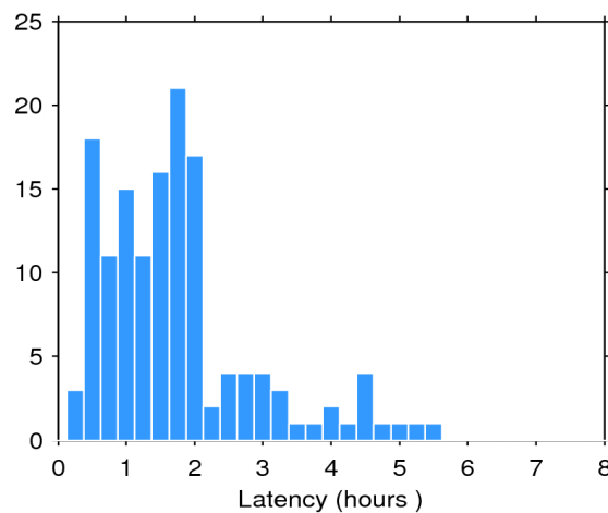
Figure 2. Histogram of the data latency for 03/09/2019. The y-axis denotes the number of files that are made available with a delay of x-hours with respect to the mean time of the records stored in the file.
