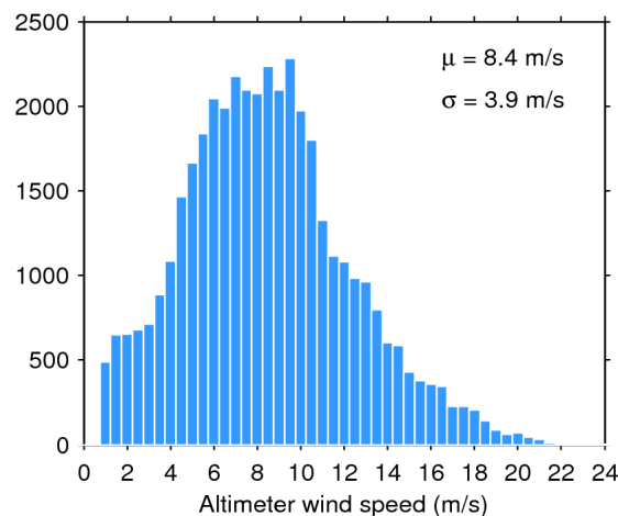
Figure 35. Histogram of science-valid wind over oceans and lakes for 03/09/2019. The mean ( \mu ) and standard deviation ( \sigma ) are also shown. Note that values larger than 24 m/s are excluded from the histogram for the sake of readability but not from the computation of \mu and \sigma .
