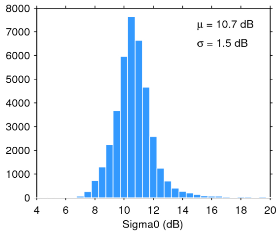
Figure 28. Histogram of science-valid sigma0 over oceans and lakes for 03/09/2019. The mean ( \mu ) and standard deviation ( \sigma ) are also shown. Note that values outside [4 20] dB are excluded from the histogram for the sake of readability but not from the computation of \mu and \sigma .
