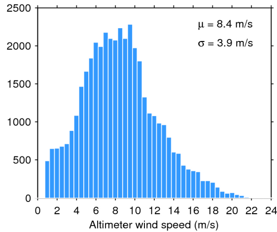
Figure 33. Histogram of flag-valid wind over oceans and lakes for 03/09/2019. The mean ( \mu ) and standard deviation ( \sigma ) are also shown. Note that values larger than 24 m/s are excluded from the histogram for the sake of readability but not from the computation of \mu and \sigma .
