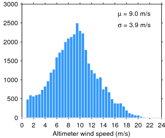
Figure 33. Histogram of flag-valid wind over oceans and lakes for 02/09/2019. The mean ( \mu ) and standard deviation ( \sigma ) are also shown. Note that values larger than 24 m/s are excluded from the histogram for the sake of readability but not from the computation of \mu and \sigma .
