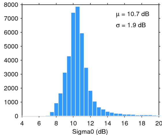
Figure 25. Histogram of flag-valid sigma0 over oceans and lakes for 02/09/2019. The mean ( \mu ) and standard deviation ( \sigma ) are also shown. Note that values outside [4 20] dB are excluded from the histogram for the sake of readability but not from the computation of \mu and \sigma .
