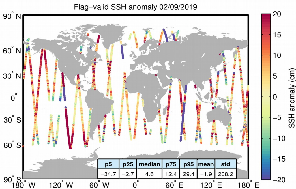
Figure 5. Geographical distribution of flag-valid 1-Hz SSH anomaly data over oceans and lakes for 02/09/2019. The statistical values shown in the table refer to the SSH anomaly in cm and are calculated over all measurements shown in the figure.
