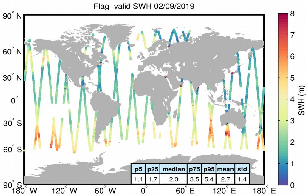
Figure 15. Geographical distribution of flag-valid SWH data over oceans and lakes for 02/09/2019. The statistical values shown in the table refer to the SWH in m and are calculated over all measurements shown in the figure.
