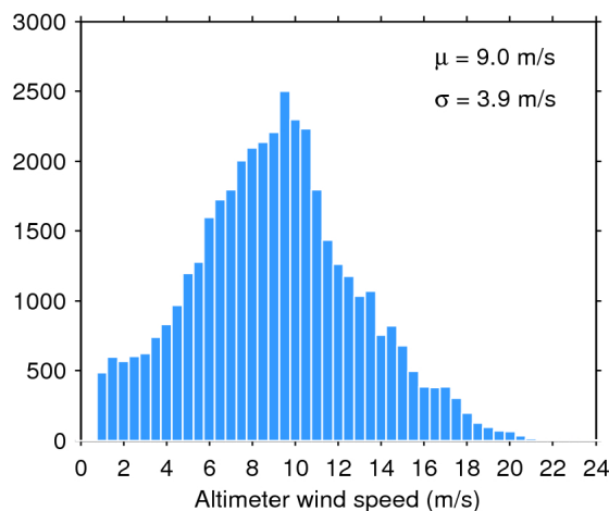
Figure 35. Histogram of science-valid wind over oceans and lakes for 02/09/2019. The mean ( \mu ) and standard deviation ( \sigma ) are also shown. Note that values larger than 24 m/s are excluded from the histogram for the sake of readability but not from the computation of \mu and \sigma .
