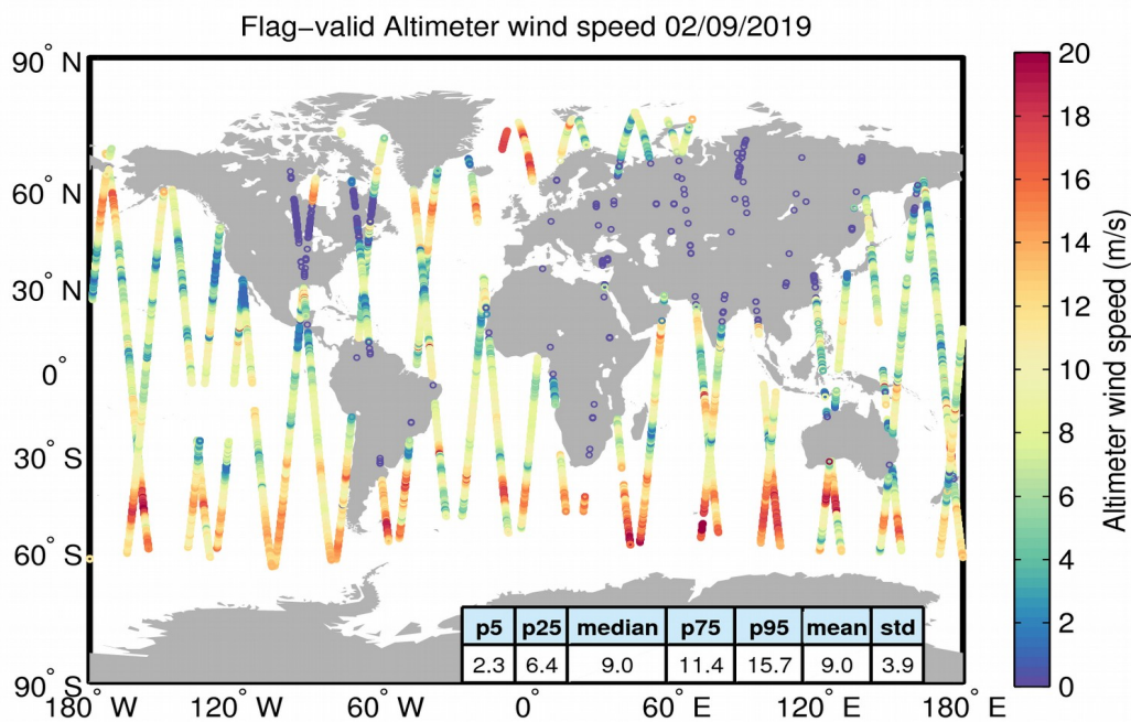
Figure 31. Geographical distribution of flag-valid wind data over oceans and lakes for 02/09/2019. The statistical values shown in the figure refer to the wind in m/s and are calculated over all measurements shown in the figure.
