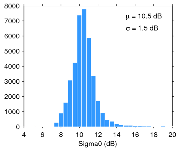
Figure 28. Histogram of science-valid sigma0 over oceans and lakes for 02/09/2019. The mean ( \mu ) and standard deviation ( \sigma ) are also shown. Note that values outside [4 20] dB are excluded from the histogram for the sake of readability but not from the computation of \mu and \sigma .
