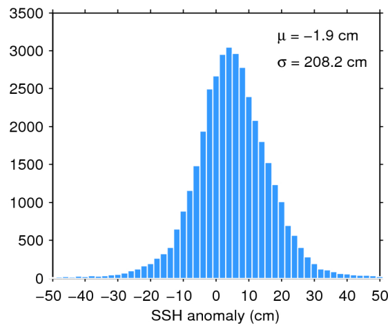
Figure 7. Histogram of flag-valid SSH anomaly over oceans and lakes for 02/09/2019. The mean ( \mu ) and standard deviation ( \sigma ) are also shown. Note that values outside [-50\ 50] cm are excluded from the histogram for the sake of readability but not from the computation of \mu and \sigma .
