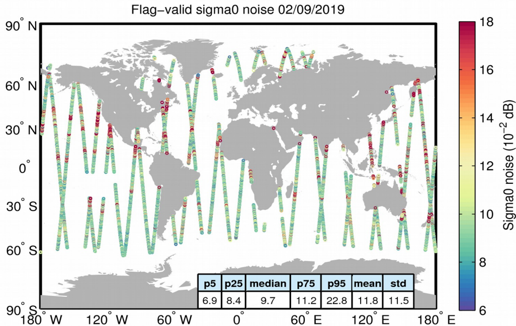
Figure 26. Geographical distribution of flag-valid 20-Hz sigma0 measurement noise over oceans and lakes for 02/09/2019. The statistical values shown in the table refer to the sigma0 noise and are calculated over all measurements shown in the figure.
