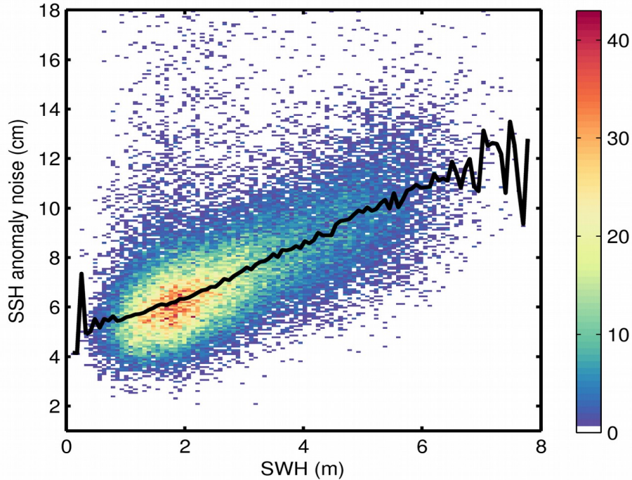
Figure 9. 2D histogram showing flag-valid SSH anomaly noise as a function of SWH for 02/09/2019. The black line denotes the median SSH anomaly noise as a function of SWH.
