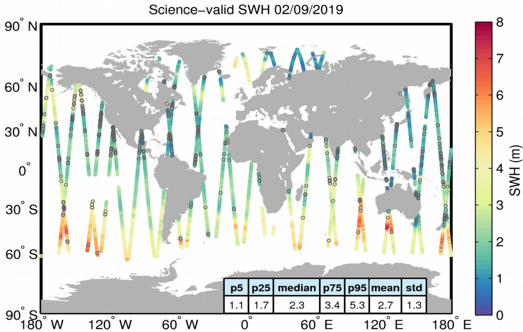
Figure 19. Geographical distribution of science-valid SWH data over oceans and lakes for 02/09/2019. The statistical values shown in the table refer to the SWH in m and are calculated over all measurements shown in the figure. Gray circles denote records that have been rejected based on the editing criteria described in Table 3.
