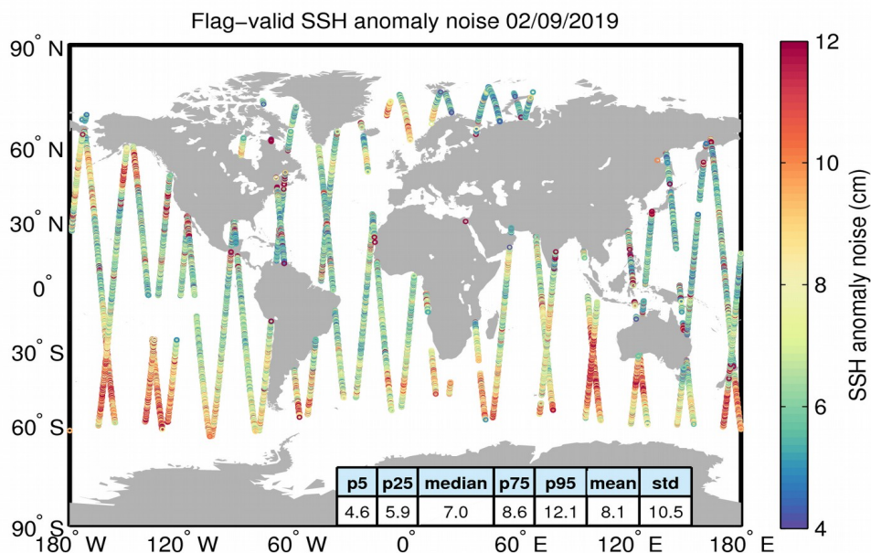
Figure 8. Geographical distribution of flag-valid 20-Hz SSH anomaly measurement noise over oceans and lakes for 02/09/2019. The statistical values shown in the table refer to the SSH anomaly noise and are calculated over all measurements shown in the figure.
