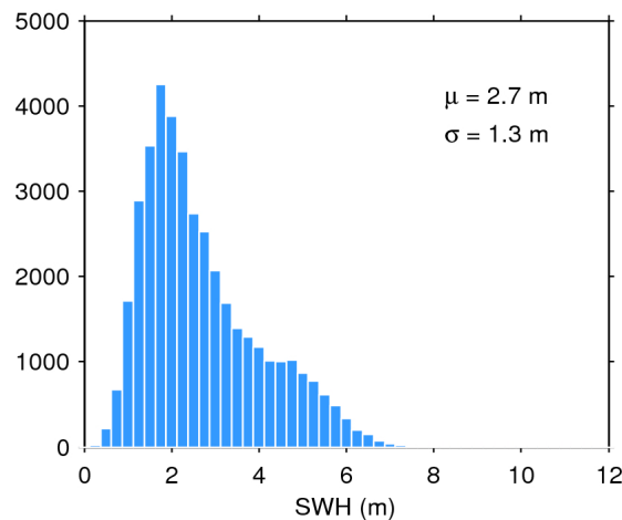
Figure 20. Histogram of science-valid SWH over oceans and lakes for 02/09/2019. The mean ( \mu ) and standard deviation ( \sigma ) are also shown. Note that values larger than 12 m are excluded from the histogram for the sake of readability but not from the computation of \mu and \sigma .
