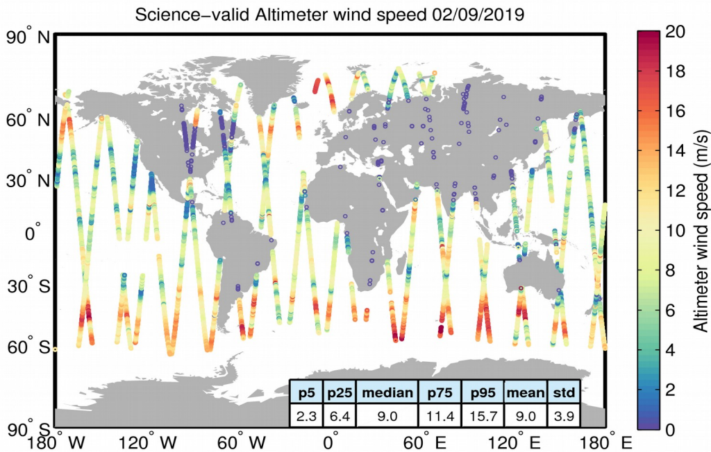
Figure 34. Geographical distribution of science-valid wind data over oceans and lakes for 02/09/2019. The statistical values shown in the table refer to the wind in m/s and are calculated over all measurements shown in the figure. Gray circles denote records that have been rejected based on the editing criteria described in Table 5.
