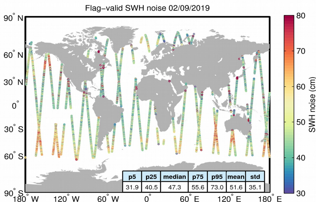
Figure 18. Geographical distribution of flag-valid 20-Hz SWH measurement noise over oceans and lakes for 02/09/2019. The statistical values shown in the figure refer to the SWH noise and are calculated over all measurements shown in the figure.
