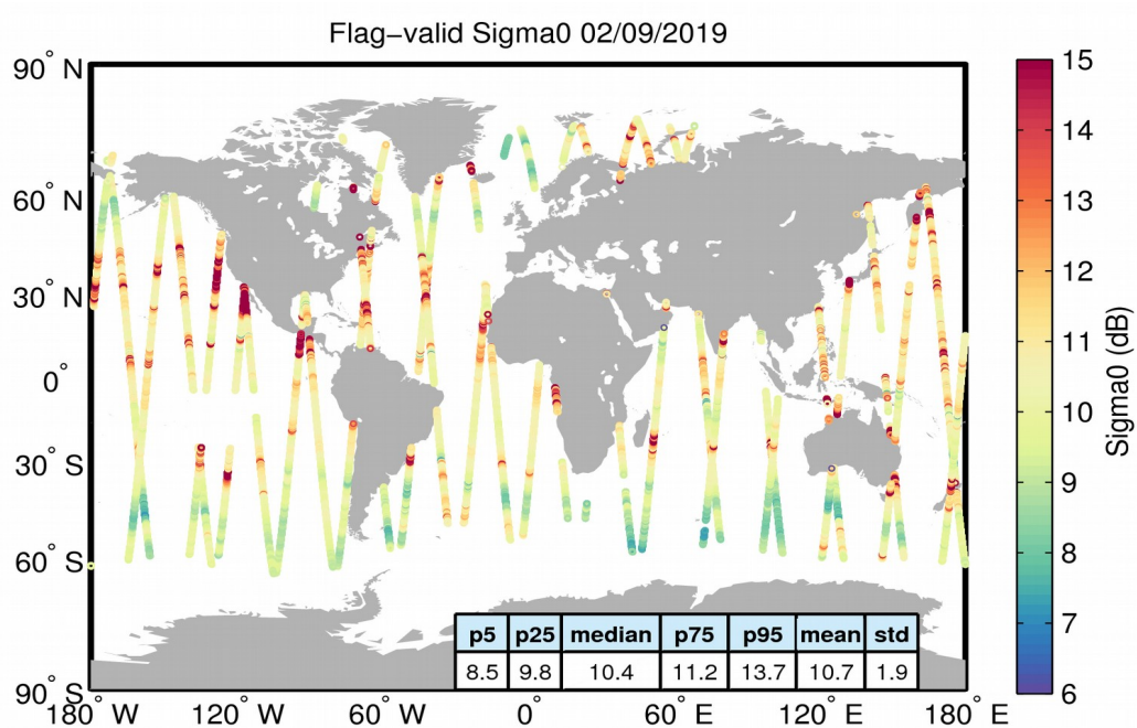
Figure 23. Geographical distribution of flag-valid sigma0 data over oceans and lakes for 02/09/2019. The statistical values shown in the table refer to the sigma0 in dB and are calculated over all measurements shown in the figure.
