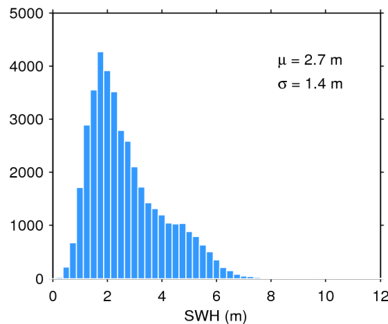
Figure 17. Histogram of flag-valid SWH over oceans and lakes for 02/09/2019. The mean ( \mu ) and standard deviation ( \sigma ) are also shown. Note that values larger than 12 m are excluded from the histogram for the sake of readability but not from the computation of \mu and \sigma .
