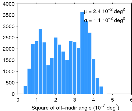
Figure 39. Histogram of flag-valid mispointing over oceans and lakes for 02/09/2019. The mean ( \mu ) and standard deviation ( \sigma ) are also shown. Note that values larger than 6 \cdot 10^{-2} \text{ deg}^2 are excluded from the histogram for the sake of readability but not from the computation of \mu and \sigma .
