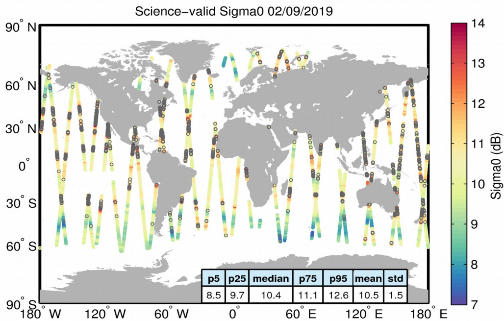
Figure 27. Geographical distribution of science-valid sigma0 data over oceans and lakes for 02/09/2019. The statistical values shown in the table refer to the sigma0 in dB and are calculated over all measurements shown in the figure. Gray circles denote records that have been rejected based on the editing criteria described in Table 4.
