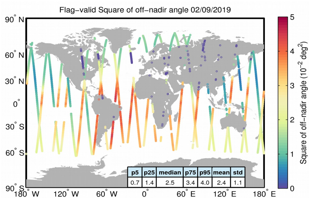
Figure 37. Geographical distribution of flag-valid mispointing data over oceans and lakes for 02/09/2019. The statistical values shown in the table refer to the mispointing in 10^{-2} deg 2 and are calculated over all measurements shown in the figure.
