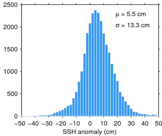
Figure 11. Histogram of science-valid SSH anomaly over oceans and lakes for 02/09/2019. The mean ( \mu ) and standard deviation ( \sigma ) are also shown. Note that values outside [-50 50] cm are excluded from the histogram for the sake of readability but not from the computation of \mu and \sigma .
