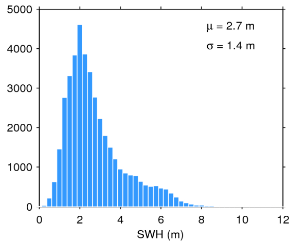
Figure 17. Histogram of flag-valid SWH over oceans and lakes for 01/09/2019. The mean ( \mu ) and standard deviation ( \sigma ) are also shown. Note that values larger than 12 m are excluded from the histogram for the sake of readability but not from the computation of \mu and \sigma .
