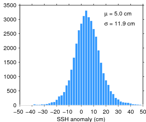
Figure 11. Histogram of science-valid SSH anomaly over oceans and lakes for 01/09/2019. The mean ( \mu ) and standard deviation ( \sigma ) are also shown. Note that values outside [-50 50] cm are excluded from the histogram for the sake of readability but not from the computation of \mu and \sigma .
