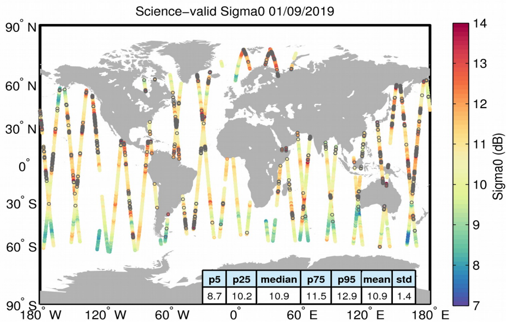
Figure 27. Geographical distribution of science-valid sigma0 data over oceans and lakes for 01/09/2019. The statistical values shown in the table refer to the sigma0 in dB and are calculated over all measurements shown in the figure. Gray circles denote records that have been rejected based on the editing criteria described in Table 4.
