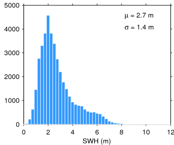
Figure 20. Histogram of science-valid SWH over oceans and lakes for 01/09/2019. The mean ( \mu ) and standard deviation ( \sigma ) are also shown. Note that values larger than 12 m are excluded from the histogram for the sake of readability but not from the computation of \mu and \sigma .
