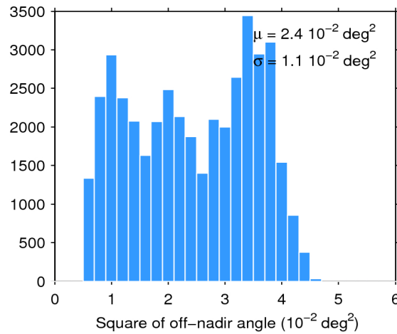
Figure 39. Histogram of flag-valid mispointing over oceans and lakes for 01/09/2019. The mean ( \mu ) and standard deviation ( \sigma ) are also shown. Note that values larger than 6 \cdot 10^{-2} \text{ deg}^2 are excluded from the histogram for the sake of readability but not from the computation of \mu and \sigma .
