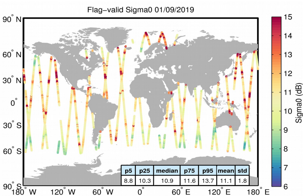
Figure 23. Geographical distribution of flag-valid sigma0 data over oceans and lakes for 01/09/2019. The statistical values shown in the table refer to the sigma0 in dB and are calculated over all measurements shown in the figure.
