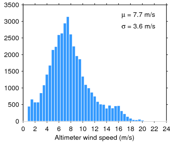
Figure 33. Histogram of flag-valid wind over oceans and lakes for 01/09/2019. The mean ( \mu ) and standard deviation ( \sigma ) are also shown. Note that values larger than 24 m/s are excluded from the histogram for the sake of readability but not from the computation of \mu and \sigma .
