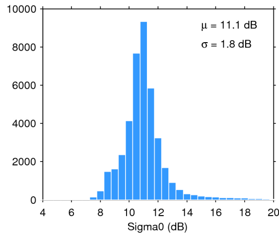
Figure 25. Histogram of flag-valid sigma0 over oceans and lakes for 01/09/2019. The mean ( \mu ) and standard deviation ( \sigma ) are also shown. Note that values outside [4 20] dB are excluded from the histogram for the sake of readability but not from the computation of \mu and \sigma .
