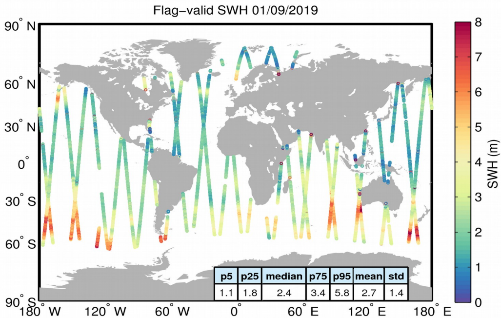
Figure 15. Geographical distribution of flag-valid SWH data over oceans and lakes for 01/09/2019. The statistical values shown in the table refer to the SWH in m and are calculated over all measurements shown in the figure.
