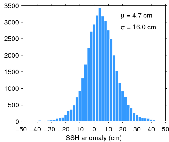
Figure 7. Histogram of flag-valid SSH anomaly over oceans and lakes for 01/09/2019. The mean ( \mu ) and standard deviation ( \sigma ) are also shown. Note that values outside [-50\ 50] cm are excluded from the histogram for the sake of readability but not from the computation of \mu and \sigma .
