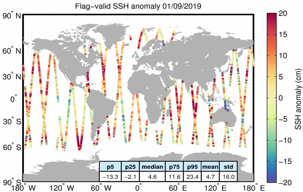
Figure 5. Geographical distribution of flag-valid 1-Hz SSH anomaly data over oceans and lakes for 01/09/2019. The statistical values shown in the table refer to the SSH anomaly in cm and are calculated over all measurements shown in the figure.
