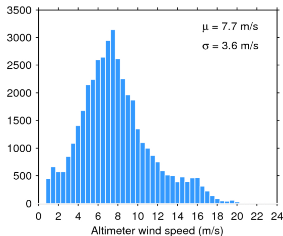
Figure 35. Histogram of science-valid wind over oceans and lakes for 01/09/2019. The mean ( \mu ) and standard deviation ( \sigma ) are also shown. Note that values larger than 24 m/s are excluded from the histogram for the sake of readability but not from the computation of \mu and \sigma .
