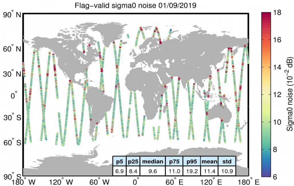
Figure 26. Geographical distribution of flag-valid 20-Hz sigma0 measurement noise over oceans and lakes for 01/09/2019. The statistical values shown in the figure refer to the sigma0 noise and are calculated over all measurements shown in the figure.
