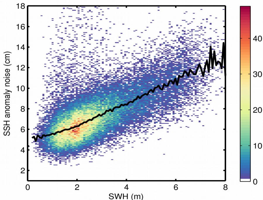
Figure 9. 2D histogram showing flag-valid SSH anomaly noise as a function of SWH for 01/09/2019. The black line denotes the median SSH anomaly noise as a function of SWH.
