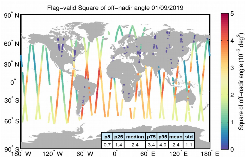
Figure 37. Geographical distribution of flag-valid mispointing data over oceans and lakes for 01/09/2019. The statistical values shown in the table refer to the mispointing in 10^{-2} \text{ deg}^2 and are calculated over all measurements shown in the figure.
