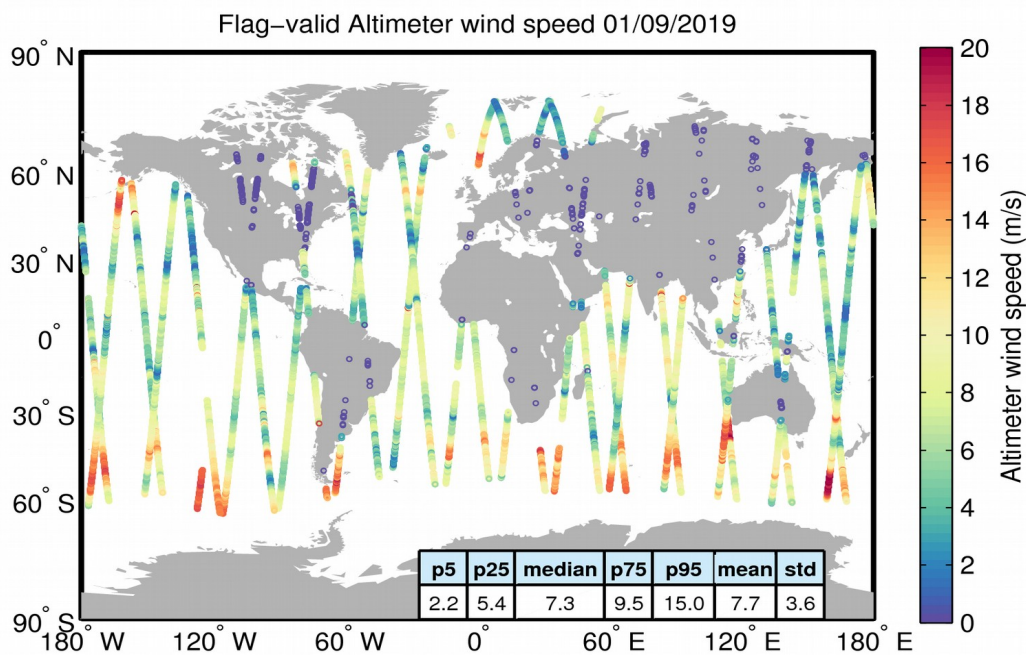
Figure 31. Geographical distribution of flag-valid wind data over oceans and lakes for 01/09/2019. The statistical values shown in the table refer to the wind in m/s and are calculated over all measurements shown in the figure.
