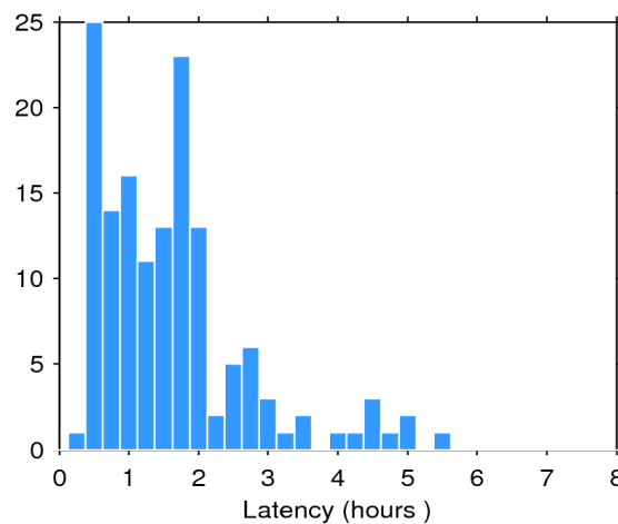
Figure 2. Histogram of the data latency for 01/09/2019. The y-axis denotes the number of files that are made available with a delay of x-hours with respect to the mean time of the records stored in the file.
