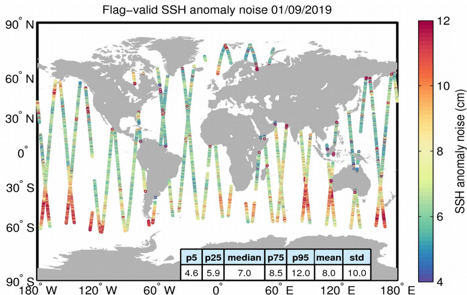
Figure 8. Geographical distribution of flag-valid 20-Hz SSH anomaly measurement noise over oceans and lakes for 01/09/2019. The statistical values shown in the table refer to the SSH anomaly noise and are calculated over all measurements shown in the figure.
