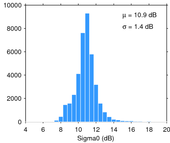
Figure 28. Histogram of science-valid sigma0 over oceans and lakes for 01/09/2019. The mean ( \mu ) and standard deviation ( \sigma ) are also shown. Note that values outside [4 20] dB are excluded from the histogram for the sake of readability but not from the computation of \mu and \sigma .
