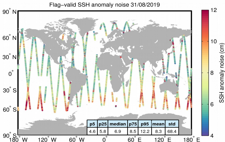
Figure 8. Geographical distribution of flag-valid 20-Hz SSH anomaly measurement noise over oceans and lakes for 31/08/2019. The statistical values shown in the table refer to the SSH anomaly noise and are calculated over all measurements shown in the figure.
