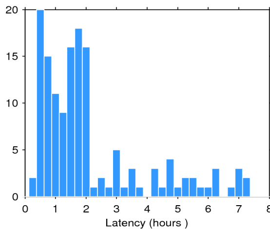
Figure 2. Histogram of the data latency for 31/08/2019. The y-axis denotes the number of files that are made available with a delay of x-hours with respect to the mean time of the records stored in the file.
