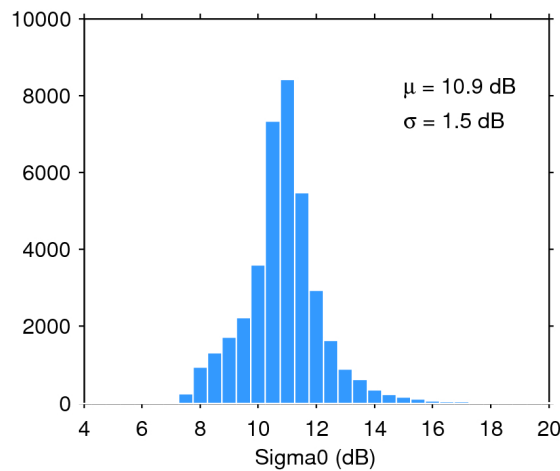
Figure 28. Histogram of science-valid sigma0 over oceans and lakes for 31/08/2019. The mean ( \mu ) and standard deviation ( \sigma ) are also shown. Note that values outside [4 20] dB are excluded from the histogram for the sake of readability but not from the computation of \mu and \sigma .
