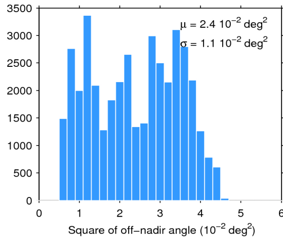
Figure 39. Histogram of flag-valid mispointing over oceans and lakes for 31/08/2019. The mean ( \mu ) and standard deviation ( \sigma ) are also shown. Note that values larger than 6 \cdot 10^{-2} \text{ deg}^2 are excluded from the histogram for the sake of readability but not from the computation of \mu and \sigma .
