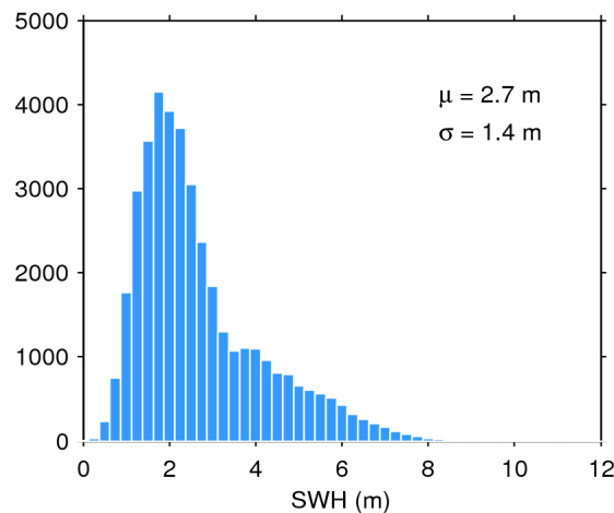
Figure 20. Histogram of science-valid SWH over oceans and lakes for 31/08/2019. The mean ( \mu ) and standard deviation ( \sigma ) are also shown. Note that values larger than 12 m are excluded from the histogram for the sake of readability but not from the computation of \mu and \sigma .
