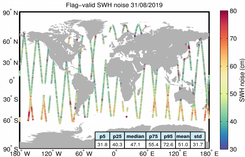
Figure 18. Geographical distribution of flag-valid 20-Hz SWH measurement noise over oceans and lakes for 31/08/2019. The statistical values shown in the table refer to the SWH noise and are calculated over all measurements shown in the figure.
