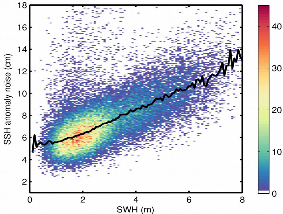
Figure 9. 2D histogram showing flag-valid SSH anomaly noise as a function of SWH for 31/08/2019. The black line denotes the median SSH anomaly noise as a function of SWH.
