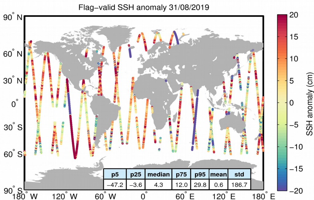
Figure 5. Geographical distribution of flag-valid 1-Hz SSH anomaly data over oceans and lakes for 31/08/2019. The statistical values shown in the table refer to the SSH anomaly in cm and are calculated over all measurements shown in the figure.
