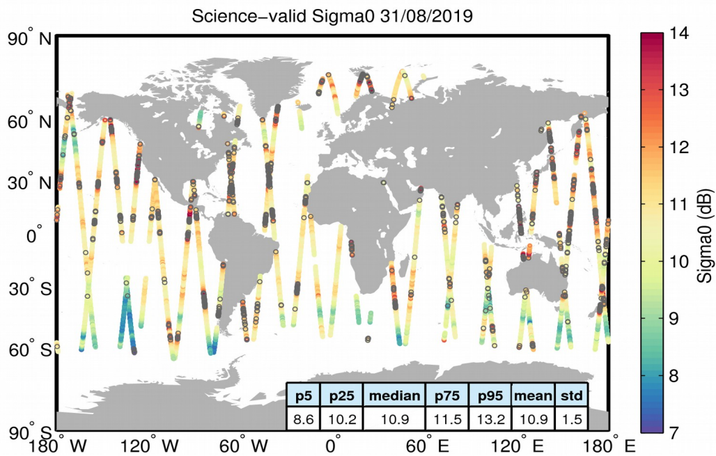
Figure 27. Geographical distribution of science-valid sigma0 data over oceans and lakes for 31/08/2019. The statistical values shown in the table refer to the sigma0 in dB and are calculated over all measurements shown in the figure. Gray circles denote records that have been rejected based on the editing criteria described in Table 4.
