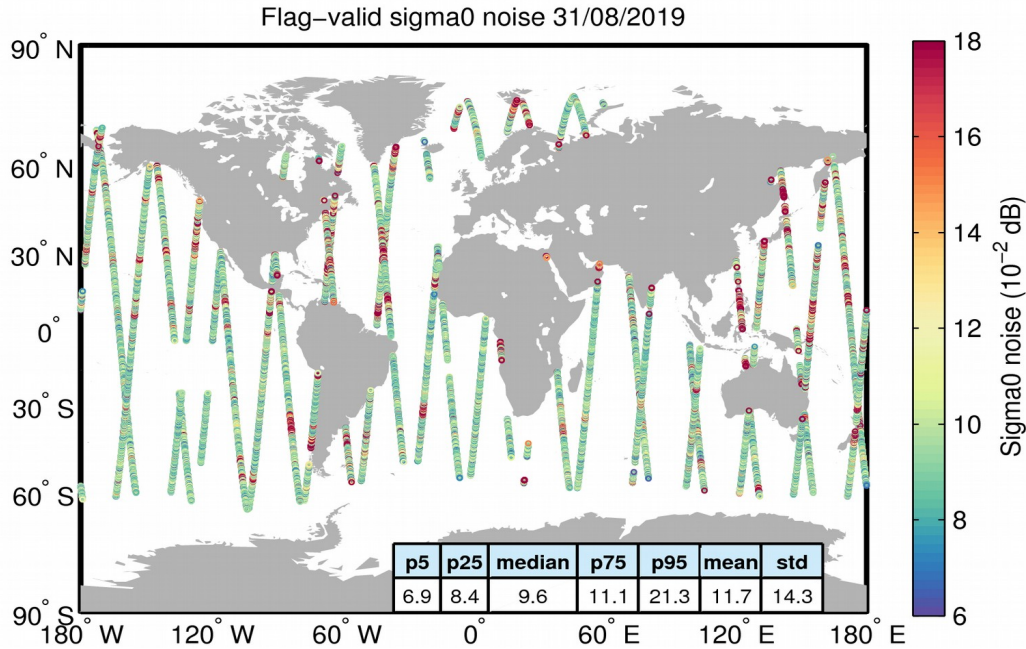
Figure 26. Geographical distribution of flag-valid 20-Hz sigma0 measurement noise over oceans and lakes for 31/08/2019. The statistical values shown in the table refer to the sigma0 noise and are calculated over all measurements shown in the figure.
