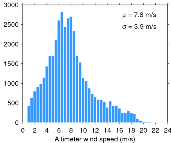
Figure 33. Histogram of flag-valid wind over oceans and lakes for 31/08/2019. The mean ( \mu ) and standard deviation ( \sigma ) are also shown. Note that values larger than 24 m/s are excluded from the histogram for the sake of readability but not from the computation of \mu and \sigma .
