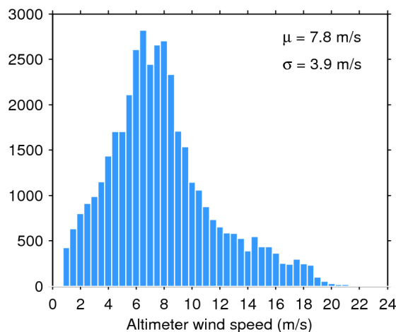
Figure 35. Histogram of science-valid wind over oceans and lakes for 31/08/2019. The mean ( \mu ) and standard deviation ( \sigma ) are also shown. Note that values larger than 24 m/s are excluded from the histogram for the sake of readability but not from the computation of \mu and \sigma .
