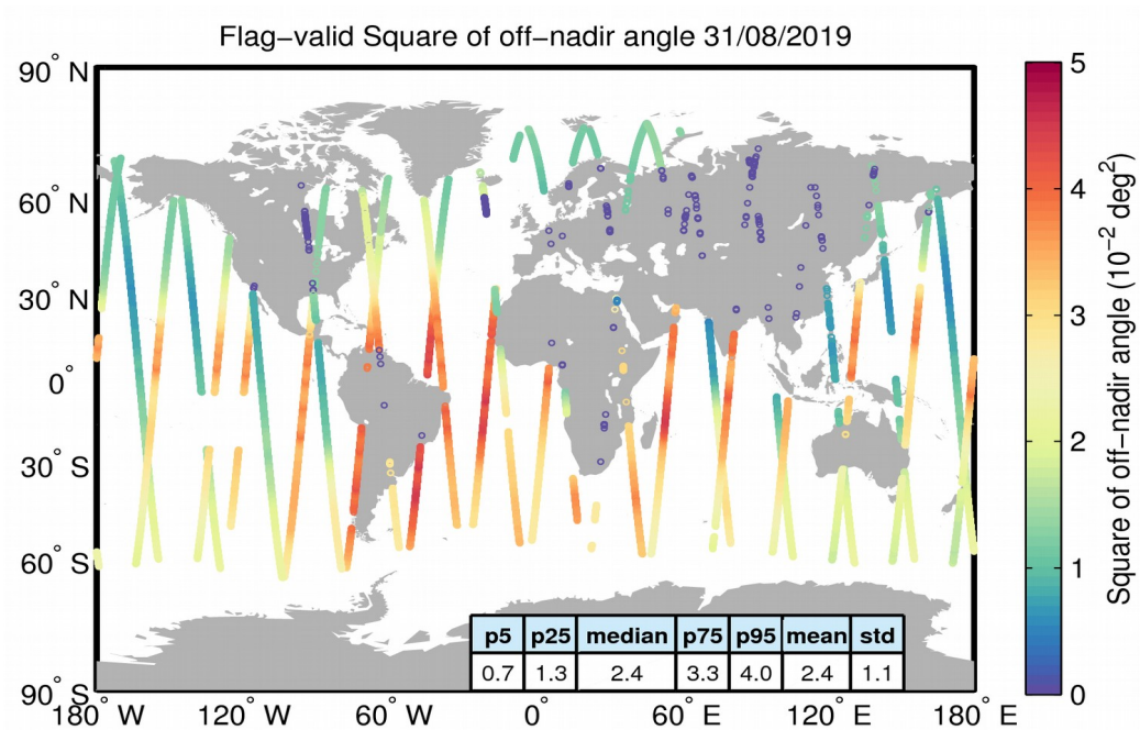
Figure 37. Geographical distribution of flag-valid mispointing data over oceans and lakes for 31/08/2019. The statistical values shown in the table refer to the mispointing in 10^{-2} deg 2 and are calculated over all measurements shown in the figure.
