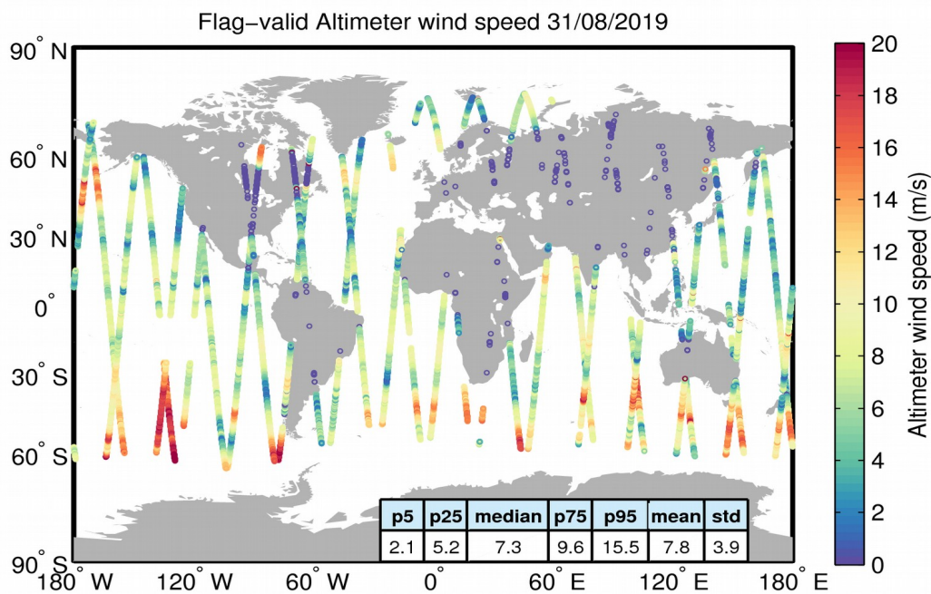
Figure 31. Geographical distribution of flag-valid wind data over oceans and lakes for 31/08/2019. The statistical values shown in the table refer to the wind in m/s and are calculated over all measurements shown in the figure.
