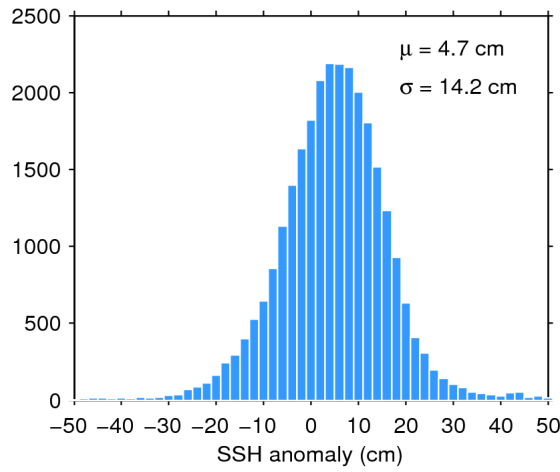
Figure 11. Histogram of science-valid SSH anomaly over oceans and lakes for 31/08/2019. The mean ( \mu ) and standard deviation ( \sigma ) are also shown. Note that values outside [-50 50] cm are excluded from the histogram for the sake of readability but not from the computation of \mu and \sigma .
