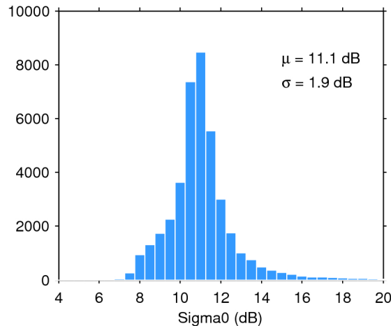
Figure 25. Histogram of flag-valid sigma0 over oceans and lakes for 31/08/2019. The mean ( \mu ) and standard deviation ( \sigma ) are also shown. Note that values outside [4 20] dB are excluded from the histogram for the sake of readability but not from the computation of \mu and \sigma .
