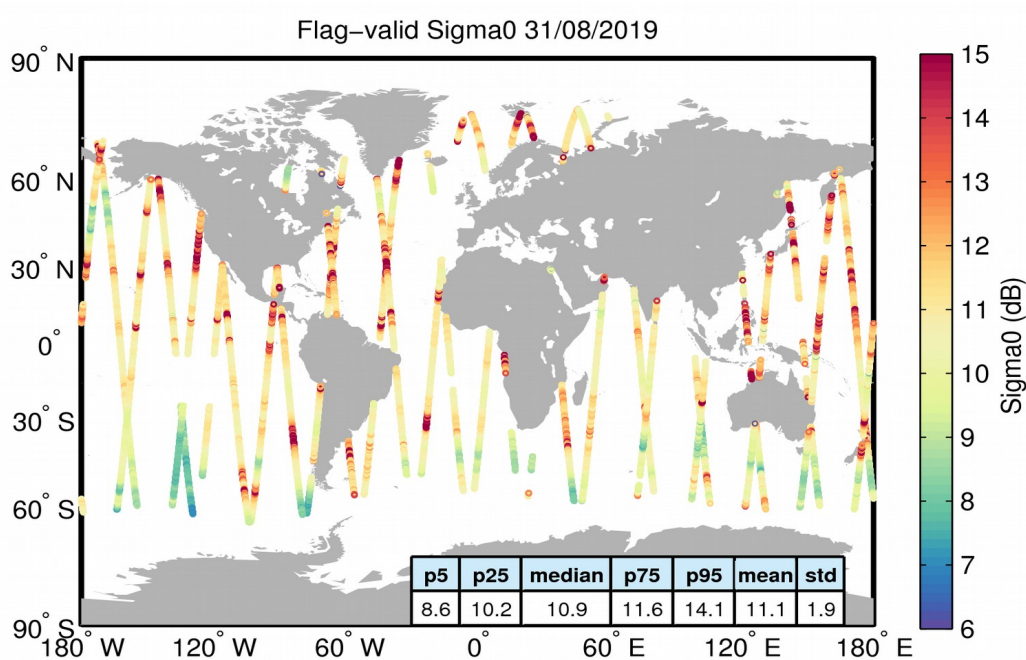
Figure 23. Geographical distribution of flag-valid sigma0 data over oceans and lakes for 31/08/2019. The statistical values shown in the table refer to the sigma0 in dB and are calculated over all measurements shown in the figure.
