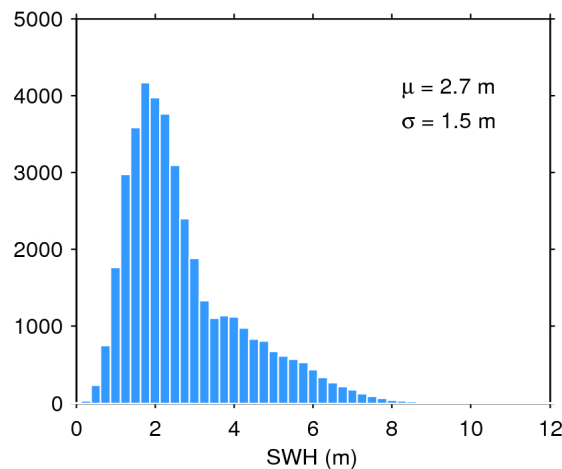
Figure 17. Histogram of flag-valid SWH over oceans and lakes for 31/08/2019. The mean ( \mu ) and standard deviation ( \sigma ) are also shown. Note that values larger than 12 m are excluded from the histogram for the sake of readability but not from the computation of \mu and \sigma .
