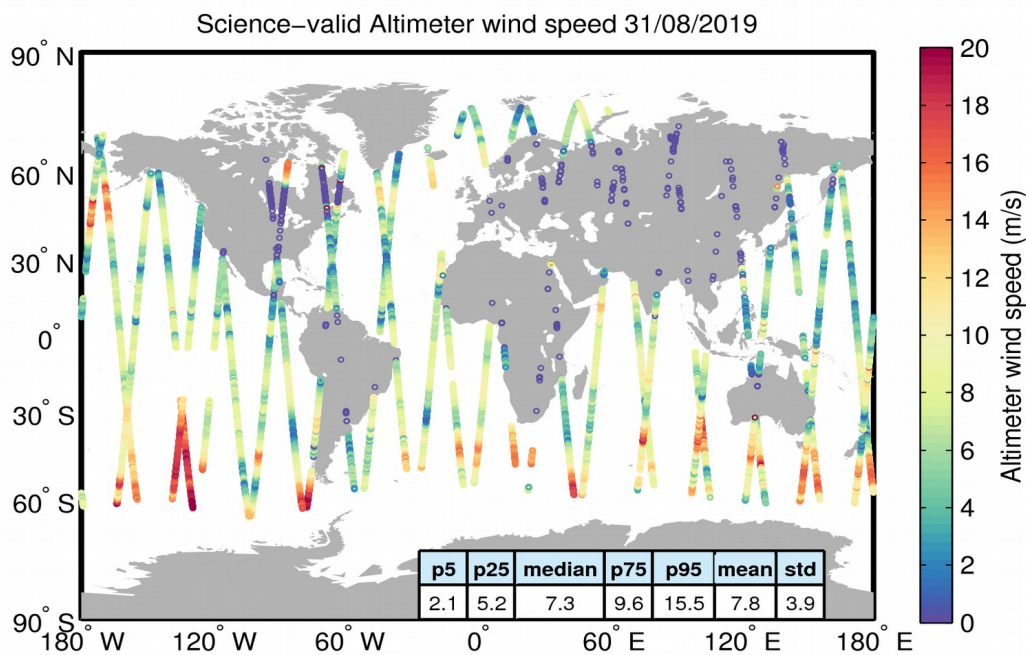
Figure 34. Geographical distribution of science-valid wind data over oceans and lakes for 31/08/2019. The statistical values shown in the table refer to the wind in m/s and are calculated over all measurements shown in the figure. Gray circles denote records that have been rejected based on the editing criteria described in Table 5.
