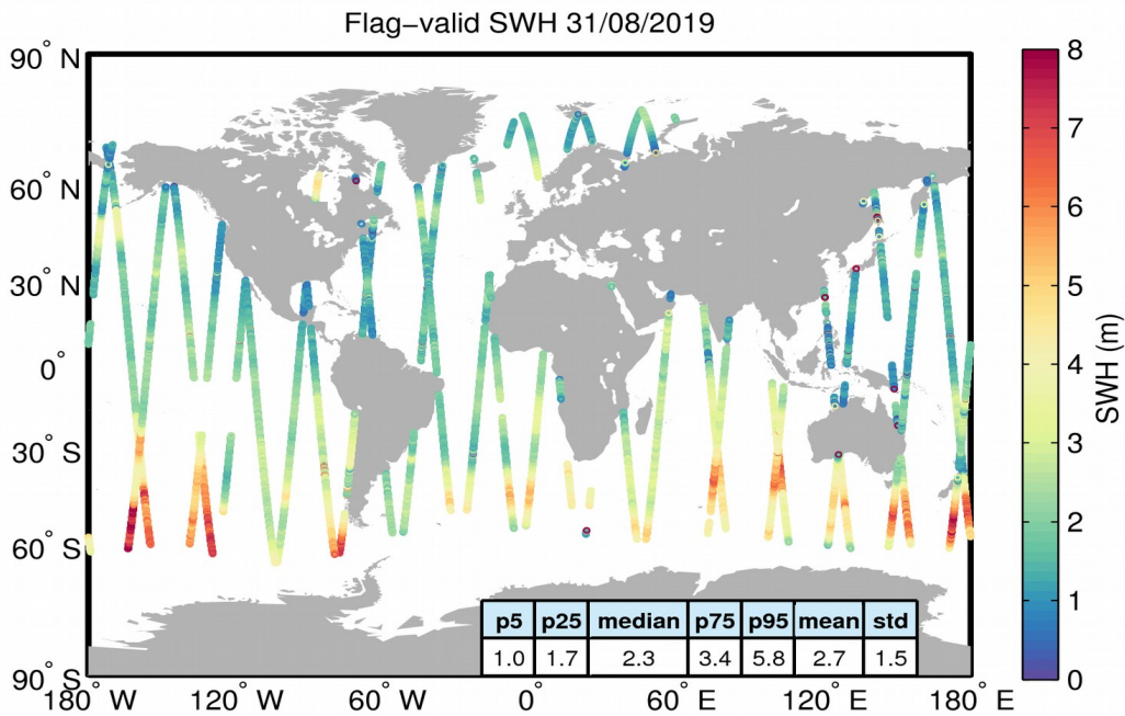
Figure 15. Geographical distribution of flag-valid SWH data over oceans and lakes for 31/08/2019. The statistical values shown in the table refer to the SWH in m and are calculated over all measurements shown in the figure.
