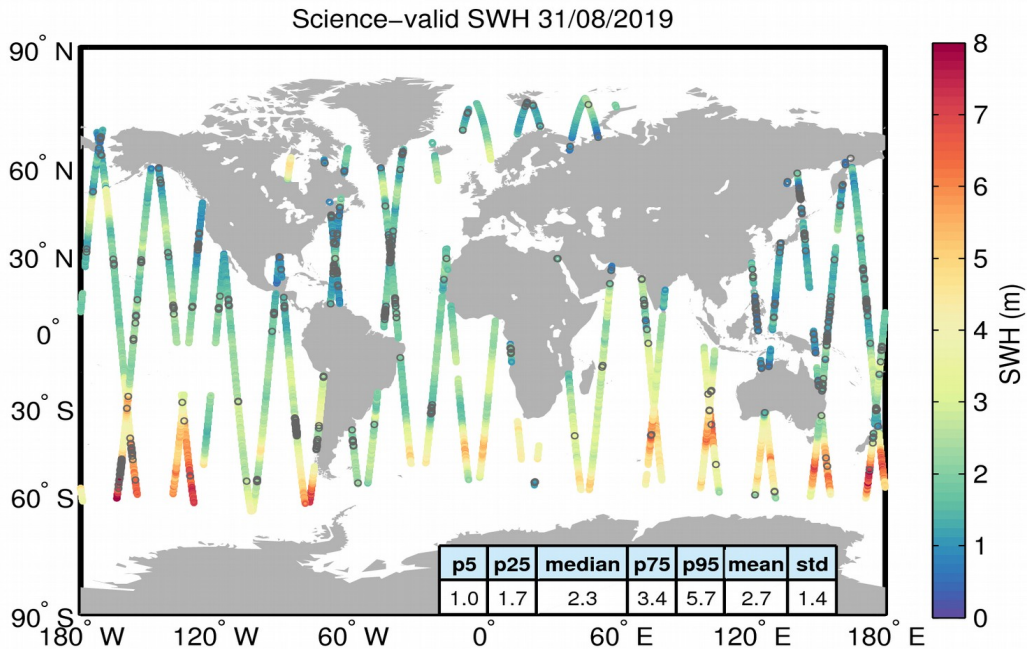
Figure 19. Geographical distribution of science-valid SWH data over oceans and lakes for 31/08/2019. The statistical values shown in the table refer to the SWH in m and are calculated over all measurements shown in the figure. Gray circles denote records that have been rejected based on the editing criteria described in Table 3.
