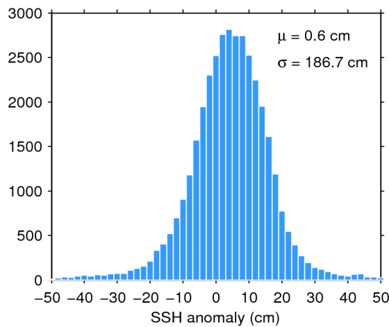
Figure 7. Histogram of flag-valid SSH anomaly over oceans and lakes for 31/08/2019. The mean ( \mu ) and standard deviation ( \sigma ) are also shown. Note that values outside [-50 50] cm are excluded from the histogram for the sake of readability but not from the computation of \mu and \sigma .
