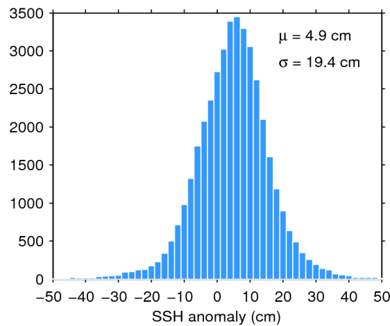
Figure 7. Histogram of flag-valid SSH anomaly over oceans and lakes for 30/08/2019. The mean ( \mu ) and standard deviation ( \sigma ) are also shown. Note that values outside [-50\ 50] cm are excluded from the histogram for the sake of readability but not from the computation of \mu and \sigma .
