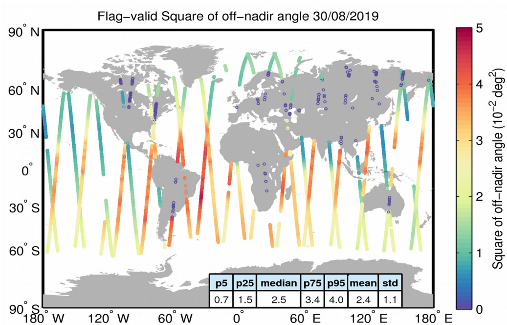
Figure 37. Geographical distribution of flag-valid mispointing data over oceans and lakes for 30/08/2019. The statistical values shown in the table refer to the mispointing in 10^{-2} \text{ deg}^2 and are calculated over all measurements shown in the figure.
