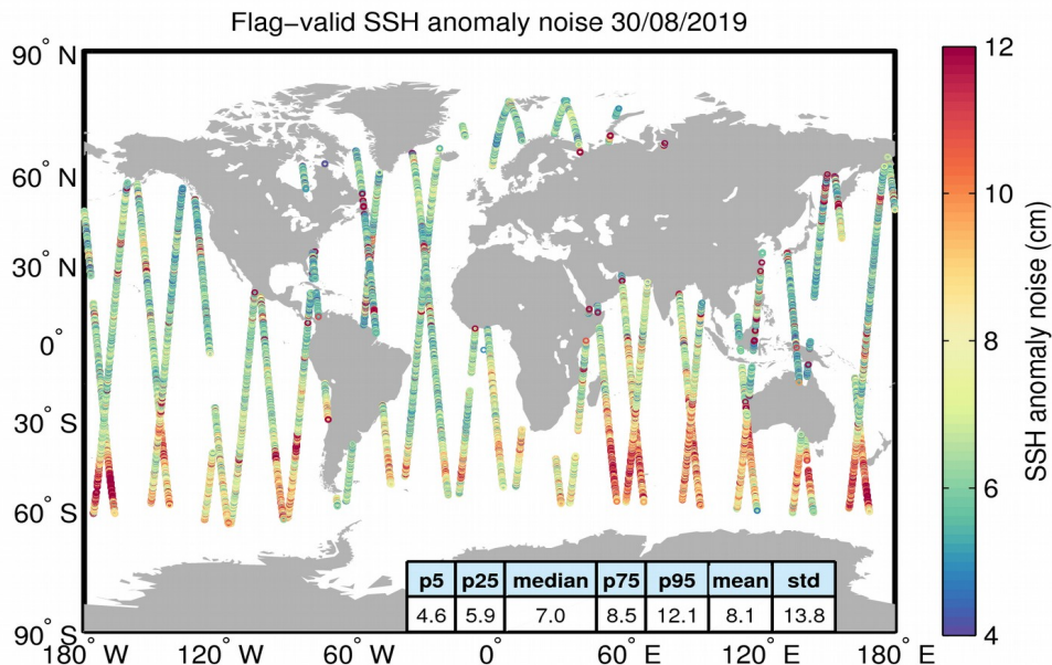
Figure 8. Geographical distribution of flag-valid 20-Hz SSH anomaly measurement noise over oceans and lakes for 30/08/2019. The statistical values shown in the table refer to the SSH anomaly noise and are calculated over all measurements shown in the figure.
