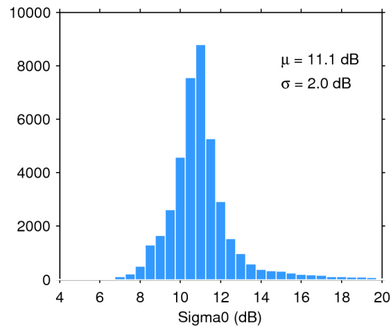
Figure 25. Histogram of flag-valid sigma0 over oceans and lakes for 30/08/2019. The mean ( \mu ) and standard deviation ( \sigma ) are also shown. Note that values outside [4 20] dB are excluded from the histogram for the sake of readability but not from the computation of \mu and \sigma .
