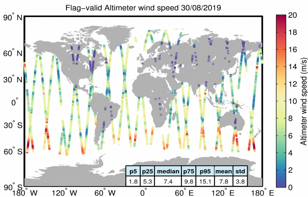
Figure 31. Geographical distribution of flag-valid wind data over oceans and lakes for 30/08/2019. The statistical values shown in the table refer to the wind in m/s and are calculated over all measurements shown in the figure.
