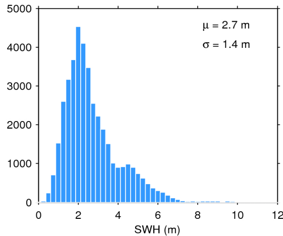
Figure 20. Histogram of science-valid SWH over oceans and lakes for 30/08/2019. The mean ( \mu ) and standard deviation ( \sigma ) are also shown. Note that values larger than 12 m are excluded from the histogram for the sake of readability but not from the computation of \mu and \sigma .
