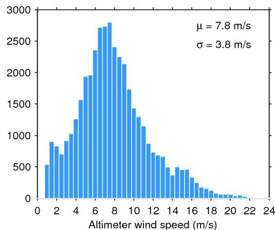
Figure 35. Histogram of science-valid wind over oceans and lakes for 30/08/2019. The mean ( \mu ) and standard deviation ( \sigma ) are also shown. Note that values larger than 24 m/s are excluded from the histogram for the sake of readability but not from the computation of \mu and \sigma .
