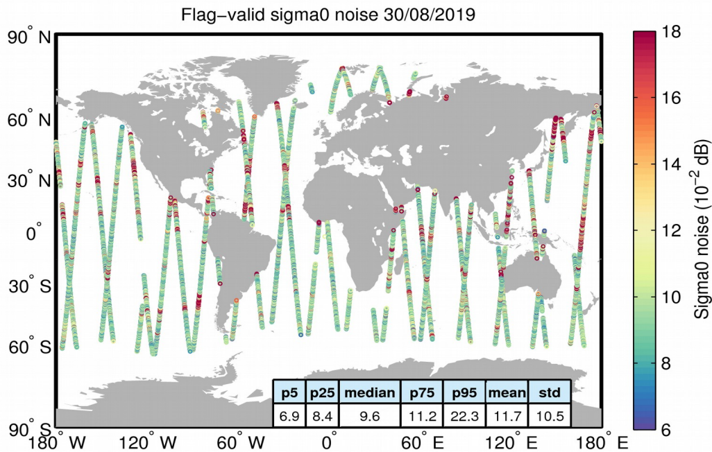
Figure 26. Geographical distribution of flag-valid 20-Hz sigma0 measurement noise over oceans and lakes for 30/08/2019. The statistical values shown in the table refer to the sigma0 noise and are calculated over all measurements shown in the figure.
