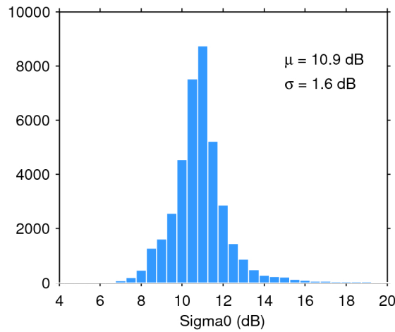
Figure 28. Histogram of science-valid sigma0 over oceans and lakes for 30/08/2019. The mean ( \mu ) and standard deviation ( \sigma ) are also shown. Note that values outside [4 20] dB are excluded from the histogram for the sake of readability but not from the computation of \mu and \sigma .
