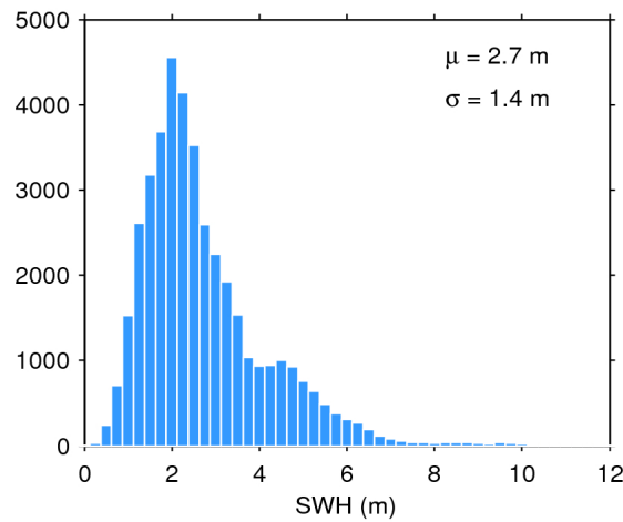
Figure 17. Histogram of flag-valid SWH over oceans and lakes for 30/08/2019. The mean ( \mu ) and standard deviation ( \sigma ) are also shown. Note that values larger than 12 m are excluded from the histogram for the sake of readability but not from the computation of \mu and \sigma .
