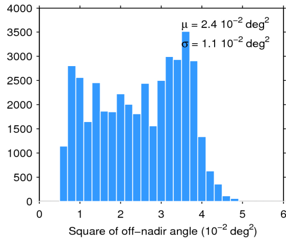
Figure 39. Histogram of flag-valid mispointing over oceans and lakes for 30/08/2019. The mean ( \mu ) and standard deviation ( \sigma ) are also shown. Note that values larger than 6 \cdot 10^{-2} \text{ deg}^2 are excluded from the histogram for the sake of readability but not from the computation of \mu and \sigma .
