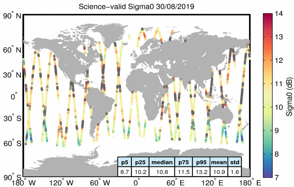
Figure 27. Geographical distribution of science-valid sigma0 data over oceans and lakes for 30/08/2019. The statistical values shown in the table refer to the sigma0 in dB and are calculated over all measurements shown in the figure. Gray circles denote records that have been rejected based on the editing criteria described in Table 4.
