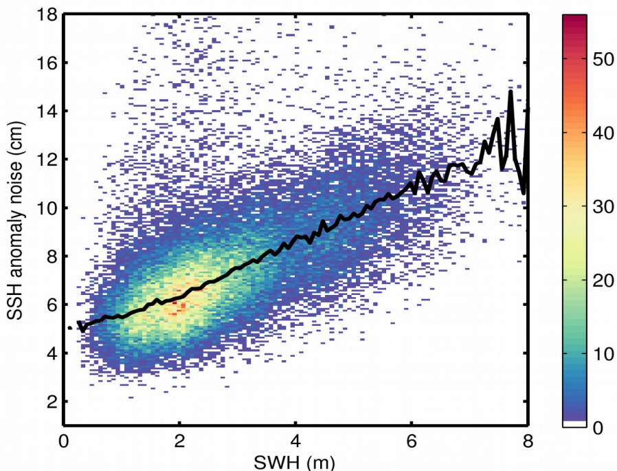
Figure 9. 2D histogram showing flag-valid SSH anomaly noise as a function of SWH for 30/08/2019. The black line denotes the median SSH anomaly noise as a function of SWH.
