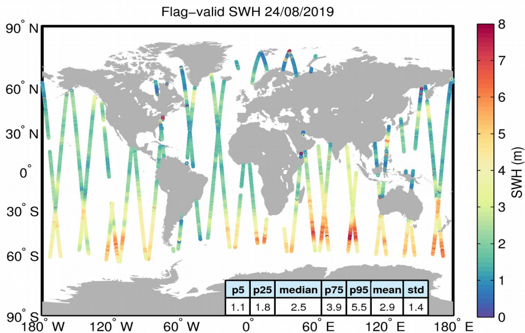
Figure 15. Geographical distribution of flag-valid SWH data over oceans and lakes for 24/08/2019. The statistical values shown in the table refer to the SWH in m and are calculated over all measurements shown in the figure.
