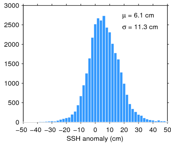
Figure 11. Histogram of science-valid SSH anomaly over oceans and lakes for 24/08/2019. The mean ( \mu ) and standard deviation ( \sigma ) are also shown. Note that values outside [-50 50] cm are excluded from the histogram for the sake of readability but not from the computation of \mu and \sigma .
