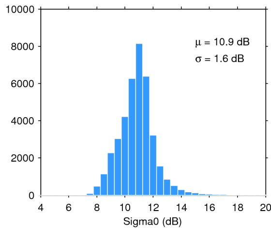
Figure 28. Histogram of science-valid sigma0 over oceans and lakes for 24/08/2019. The mean ( \mu ) and standard deviation ( \sigma ) are also shown. Note that values outside [4 20] dB are excluded from the histogram for the sake of readability but not from the computation of \mu and \sigma .
