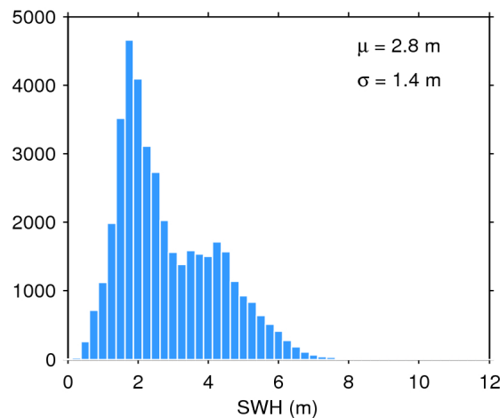
Figure 20. Histogram of science-valid SWH over oceans and lakes for 24/08/2019. The mean ( \mu ) and standard deviation ( \sigma ) are also shown. Note that values larger than 12 m are excluded from the histogram for the sake of readability but not from the computation of \mu and \sigma .
