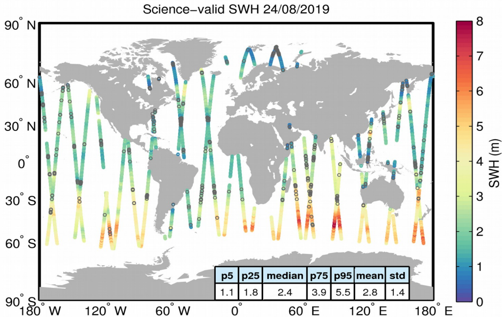
Figure 19. Geographical distribution of science-valid SWH data over oceans and lakes for 24/08/2019. The statistical values shown in the table refer to the SWH in m and are calculated over all measurements shown in the figure. Gray circles denote records that have been rejected based on the editing criteria described in Table 3.
