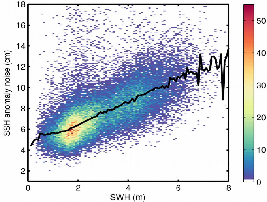
Figure 9. 2D histogram showing flag-valid SSH anomaly noise as a function of SWH for 24/08/2019. The black line denotes the median SSH anomaly noise as a function of SWH.
