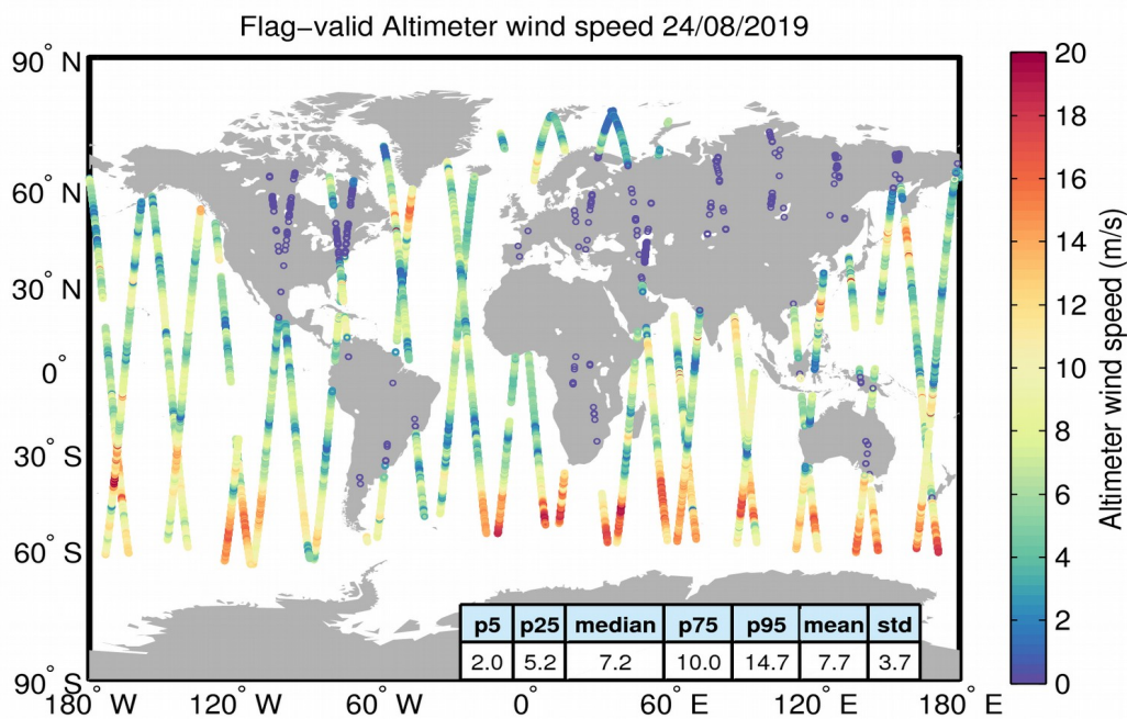
Figure 31. Geographical distribution of flag-valid wind data over oceans and lakes for 24/08/2019. The statistical values shown in the table refer to the wind in m/s and are calculated over all measurements shown in the figure.
