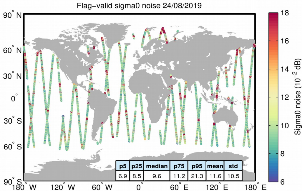
Figure 26. Geographical distribution of flag-valid 20-Hz sigma0 measurement noise over oceans and lakes for 24/08/2019. The statistical values shown in the table refer to the sigma0 noise and are calculated over all measurements shown in the figure.
