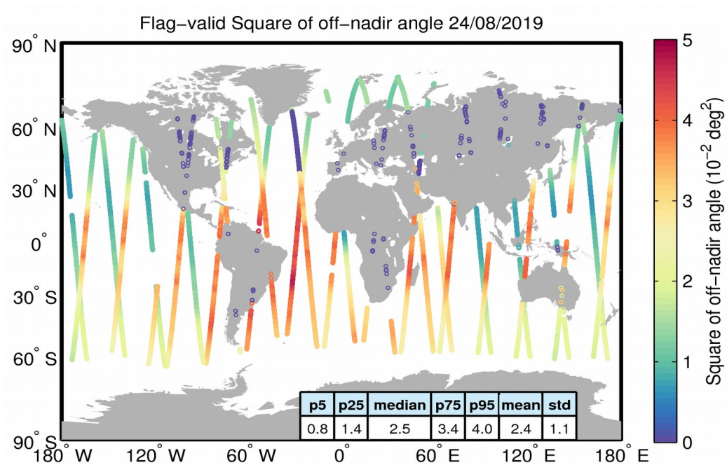
Figure 37. Geographical distribution of flag-valid mispointing data over oceans and lakes for 24/08/2019. The statistical values shown in the table refer to the mispointing in 10^{-2} \text{deg}^2 and are calculated over all measurements shown in the figure.
