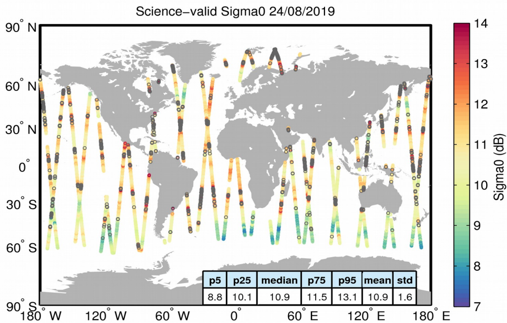
Figure 27. Geographical distribution of science-valid sigma0 data over oceans and lakes for 24/08/2019. The statistical values shown in the table refer to the sigma0 in dB and are calculated over all measurements shown in the figure. Gray circles denote records that have been rejected based on the editing criteria described in Table 4.
