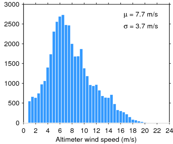
Figure 33. Histogram of flag-valid wind over oceans and lakes for 24/08/2019. The mean ( \mu ) and standard deviation ( \sigma ) are also shown. Note that values larger than 24 m/s are excluded from the histogram for the sake of readability but not from the computation of \mu and \sigma .
