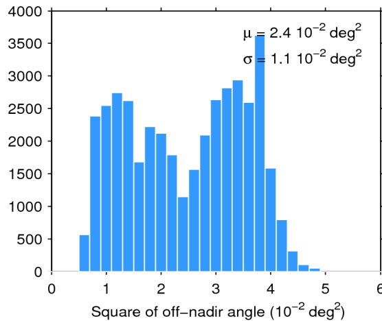
Figure 39. Histogram of flag-valid mispointing over oceans and lakes for 24/08/2019. The mean ( \mu ) and standard deviation ( \sigma ) are also shown. Note that values larger than 6 \cdot 10^{-2} \text{ deg}^2 are excluded from the histogram for the sake of readability but not from the computation of \mu and \sigma .
