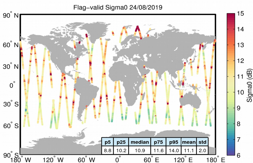
Figure 23. Geographical distribution of flag-valid sigma0 data over oceans and lakes for 24/08/2019. The statistical values shown in the table refer to the sigma0 in dB and are calculated over all measurements shown in the figure.
