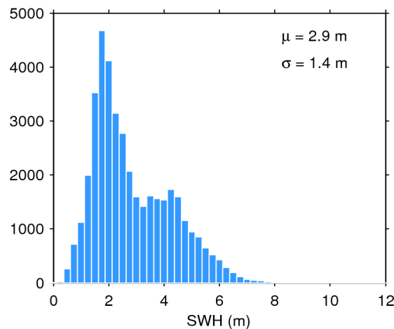
Figure 17. Histogram of flag-valid SWH over oceans and lakes for 24/08/2019. The mean ( \mu ) and standard deviation ( \sigma ) are also shown. Note that values larger than 12 m are excluded from the histogram for the sake of readability but not from the computation of \mu and \sigma .
