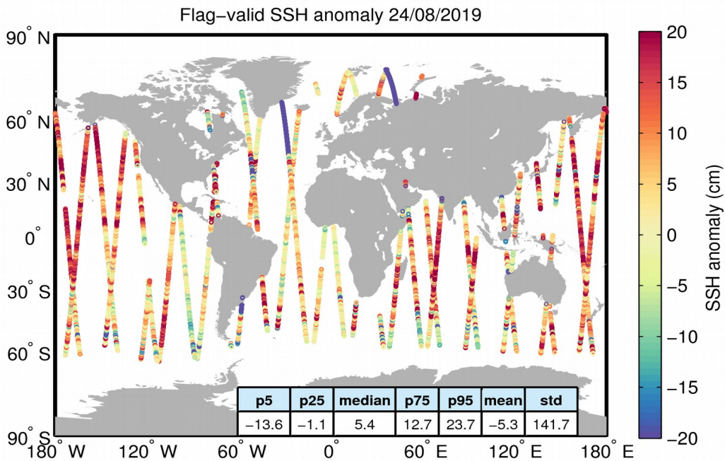
Figure 5. Geographical distribution of flag-valid 1-Hz SSH anomaly data over oceans and lakes for 24/08/2019. The statistical values shown in the table refer to the SSH anomaly in cm and are calculated over all measurements shown in the figure.
