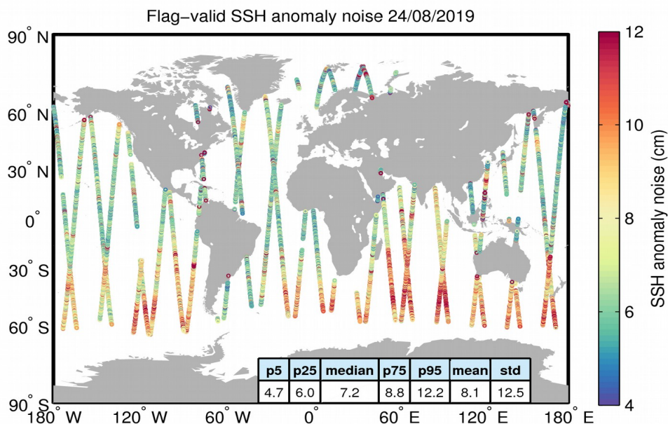
Figure 8. Geographical distribution of flag-valid 20-Hz SSH anomaly measurement noise over oceans and lakes for 24/08/2019. The statistical values shown in the table refer to the SSH anomaly noise and are calculated over all measurements shown in the figure.
