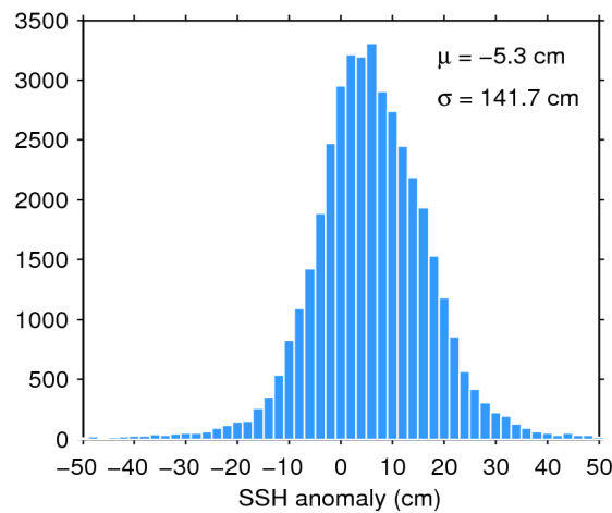
Figure 7. Histogram of flag-valid SSH anomaly over oceans and lakes for 24/08/2019. The mean ( \mu ) and standard deviation ( \sigma ) are also shown. Note that values outside [-50\ 50] cm are excluded from the histogram for the sake of readability but not from the computation of \mu and \sigma .
