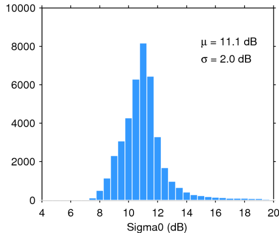
Figure 25. Histogram of flag-valid sigma0 over oceans and lakes for 24/08/2019. The mean ( \mu ) and standard deviation ( \sigma ) are also shown. Note that values outside [4 20] dB are excluded from the histogram for the sake of readability but not from the computation of \mu and \sigma .
