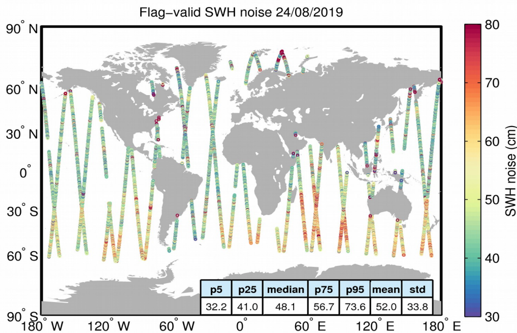
Figure 18. Geographical distribution of flag-valid 20-Hz SWH measurement noise over oceans and lakes for 24/08/2019. The statistical values shown in the figure refer to the SWH noise and are calculated over all measurements shown in the figure.
