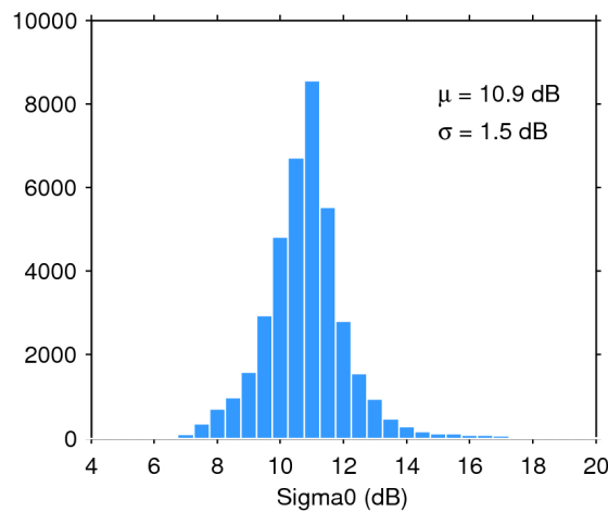
Figure 28. Histogram of science-valid sigma0 over oceans and lakes for 21/08/2019. The mean ( \mu ) and standard deviation ( \sigma ) are also shown. Note that values outside [4 20] dB are excluded from the histogram for the sake of readability but not from the computation of \mu and \sigma .
