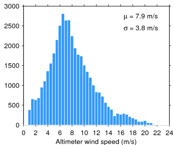
Figure 35. Histogram of science-valid wind over oceans and lakes for 21/08/2019. The mean ( \mu ) and standard deviation ( \sigma ) are also shown. Note that values larger than 24 m/s are excluded from the histogram for the sake of readability but not from the computation of \mu and \sigma .
