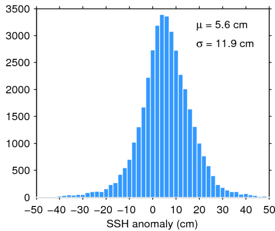
Figure 11. Histogram of science-valid SSH anomaly over oceans and lakes for 21/08/2019. The mean ( \mu ) and standard deviation ( \sigma ) are also shown. Note that values outside [-50 50] cm are excluded from the histogram for the sake of readability but not from the computation of \mu and \sigma .
