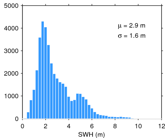
Figure 20. Histogram of science-valid SWH over oceans and lakes for 21/08/2019. The mean ( \mu ) and standard deviation ( \sigma ) are also shown. Note that values larger than 12 m are excluded from the histogram for the sake of readability but not from the computation of \mu and \sigma .
