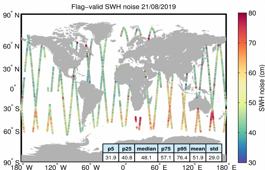
Figure 18. Geographical distribution of flag-valid 20-Hz SWH measurement noise over oceans and lakes for 21/08/2019. The statistical values shown in the table refer to the SWH noise and are calculated over all measurements shown in the figure.
