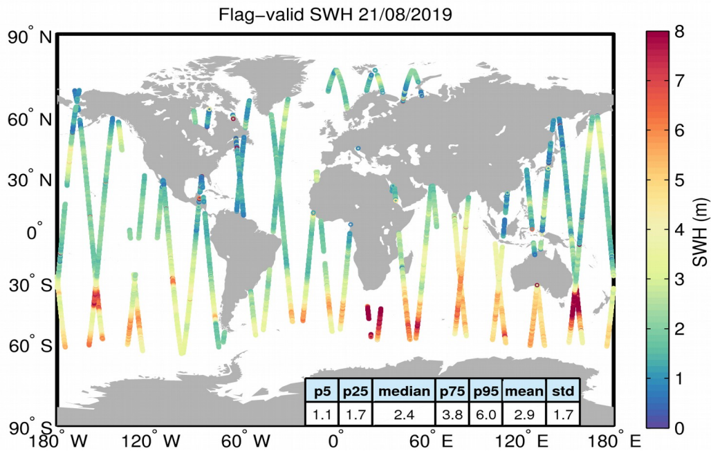
Figure 15. Geographical distribution of flag-valid SWH data over oceans and lakes for 21/08/2019. The statistical values shown in the table refer to the SWH in m and are calculated over all measurements shown in the figure.
