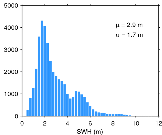
Figure 17. Histogram of flag-valid SWH over oceans and lakes for 21/08/2019. The mean ( \mu ) and standard deviation ( \sigma ) are also shown. Note that values larger than 12 m are excluded from the histogram for the sake of readability but not from the computation of \mu and \sigma .
