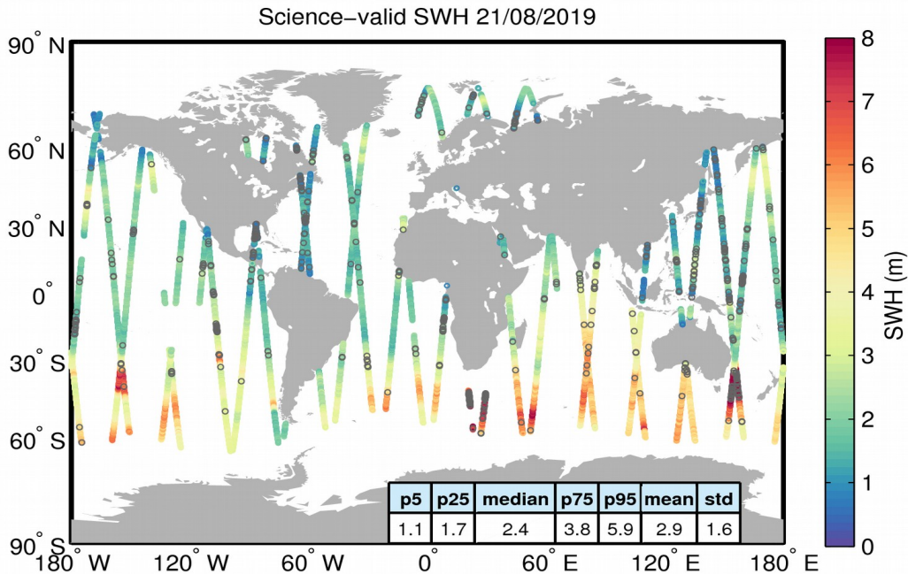
Figure 19. Geographical distribution of science-valid SWH data over oceans and lakes for 21/08/2019. The statistical values shown in the table refer to the SWH in m and are calculated over all measurements shown in the figure. Gray circles denote records that have been rejected based on the editing criteria described in Table 3.
