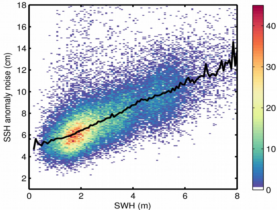
Figure 9. 2D histogram showing flag-valid SSH anomaly noise as a function of SWH for 21/08/2019. The black line denotes the median SSH anomaly noise as a function of SWH.
