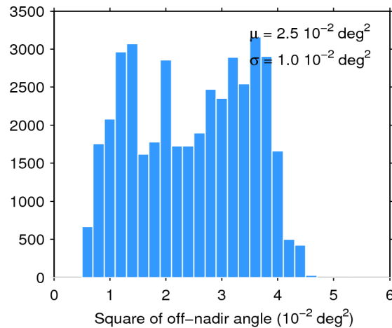
Figure 39. Histogram of flag-valid mispointing over oceans and lakes for 21/08/2019. The mean ( \mu ) and standard deviation ( \sigma ) are also shown. Note that values larger than 6 \cdot 10^{-2} \text{ deg}^2 are excluded from the histogram for the sake of readability but not from the computation of \mu and \sigma .
