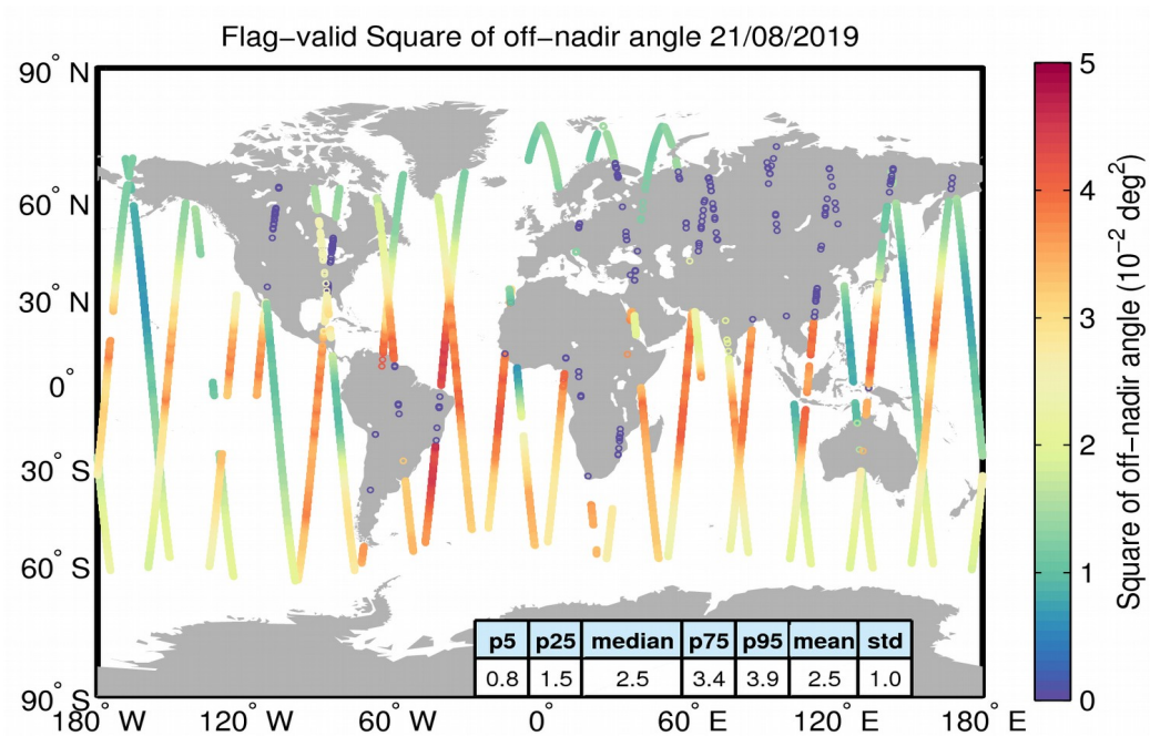
Figure 37. Geographical distribution of flag-valid mispointing data over oceans and lakes for 21/08/2019. The statistical values shown in the table refer to the mispointing in 10^{-2} \text{ deg}^2 and are calculated over all measurements shown in the figure.
