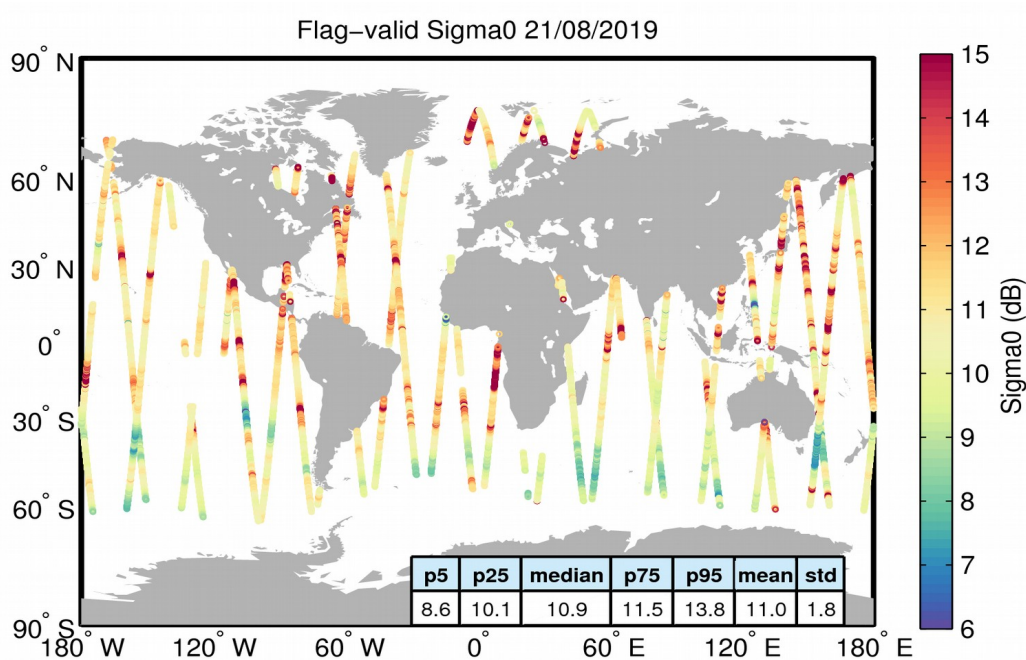
Figure 23. Geographical distribution of flag-valid sigma0 data over oceans and lakes for 21/08/2019. The statistical values shown in the table refer to the sigma0 in dB and are calculated over all measurements shown in the figure.
