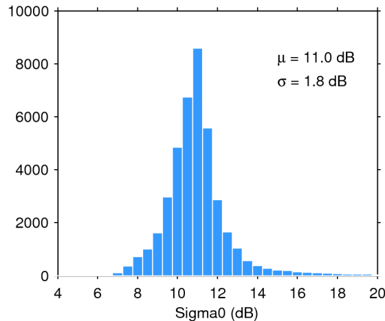
Figure 25. Histogram of flag-valid sigma0 over oceans and lakes for 21/08/2019. The mean ( \mu ) and standard deviation ( \sigma ) are also shown. Note that values outside [4 20] dB are excluded from the histogram for the sake of readability but not from the computation of \mu and \sigma .
