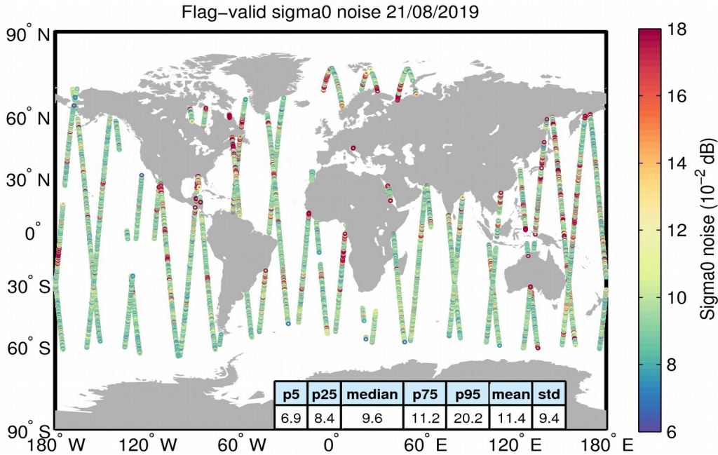
Figure 26. Geographical distribution of flag-valid 20-Hz sigma0 measurement noise over oceans and lakes for 21/08/2019. The statistical values shown in the table refer to the sigma0 noise and are calculated over all measurements shown in the figure.
