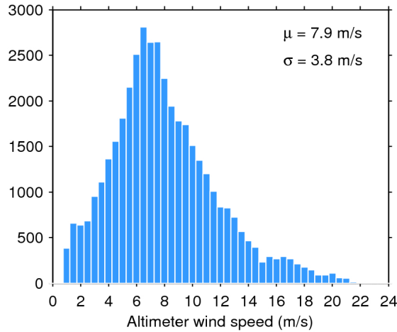
Figure 33. Histogram of flag-valid wind over oceans and lakes for 21/08/2019. The mean ( \mu ) and standard deviation ( \sigma ) are also shown. Note that values larger than 24 m/s are excluded from the histogram for the sake of readability but not from the computation of \mu and \sigma .
