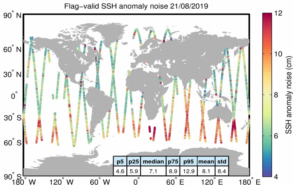
Figure 8. Geographical distribution of flag-valid 20-Hz SSH anomaly measurement noise over oceans and lakes for 21/08/2019. The statistical values shown in the table refer to the SSH anomaly noise and are calculated over all measurements shown in the figure.
