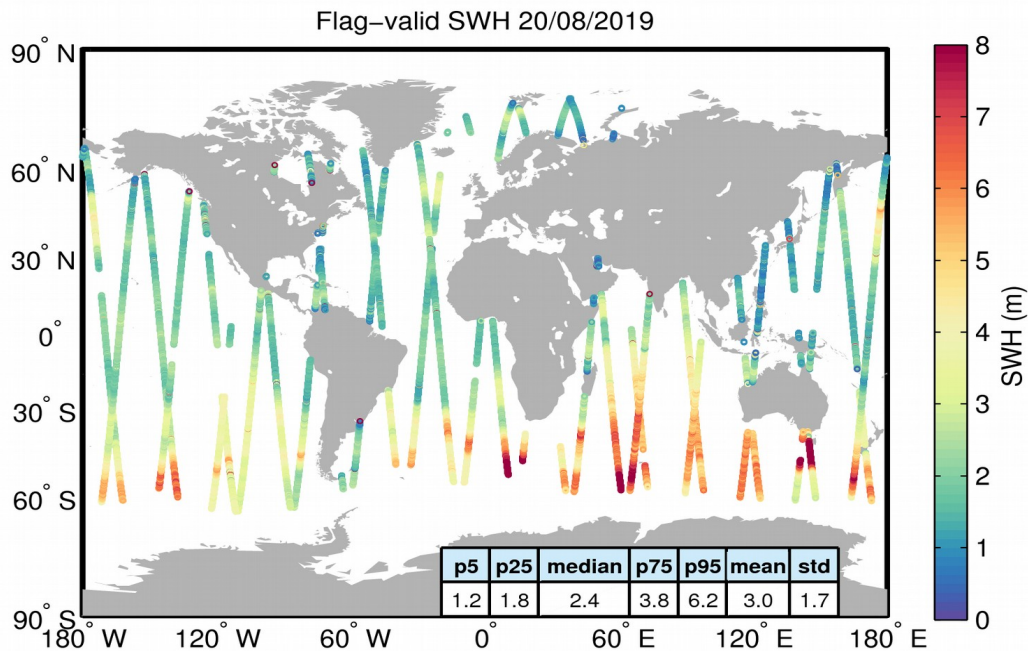
Figure 15. Geographical distribution of flag-valid SWH data over oceans and lakes for 20/08/2019. The statistical values shown in the table refer to the SWH in m and are calculated over all measurements shown in the figure.
