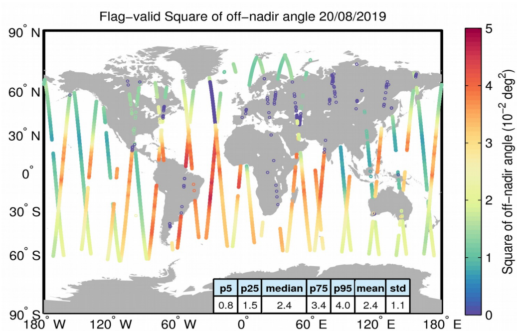
Figure 37. Geographical distribution of flag-valid mispointing data over oceans and lakes for 20/08/2019. The statistical values shown in the table refer to the mispointing in 10^{-2} \text{ deg}^2 and are calculated over all measurements shown in the figure.
