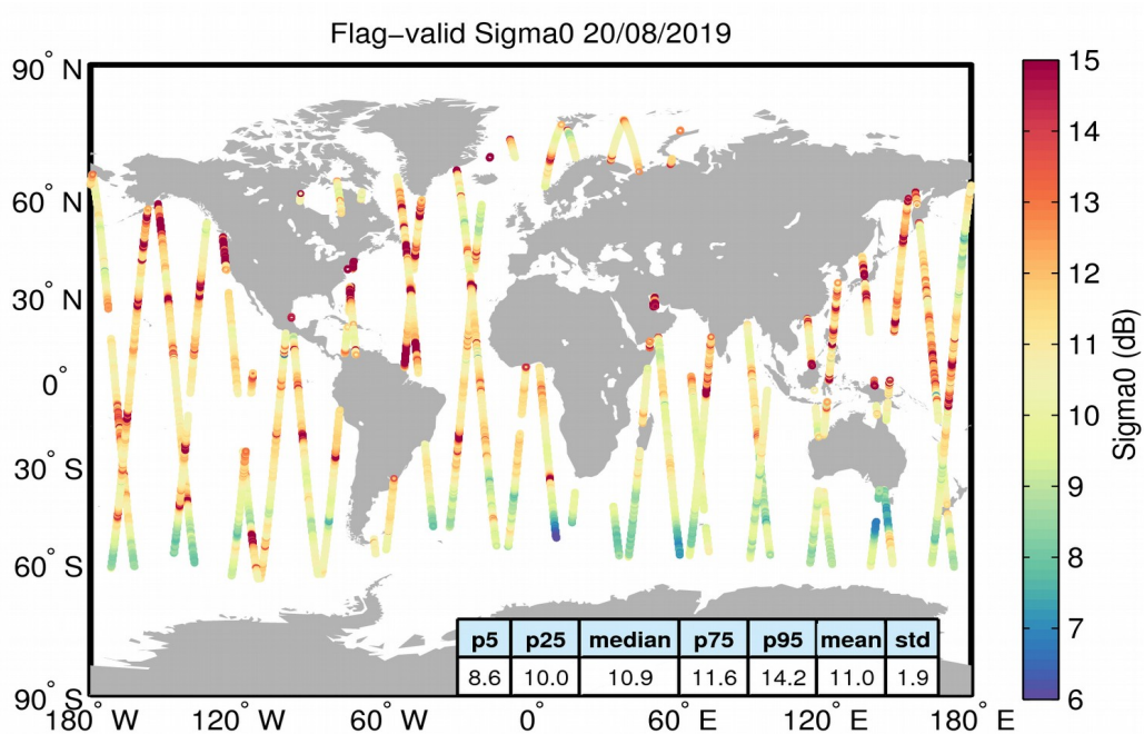
Figure 23. Geographical distribution of flag-valid sigma0 data over oceans and lakes for 20/08/2019. The statistical values shown in the table refer to the sigma0 in dB and are calculated over all measurements shown in the figure.
