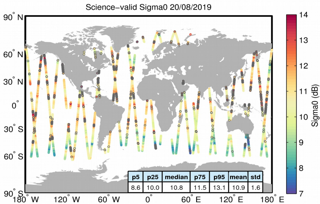
Figure 27. Geographical distribution of science-valid sigma0 data over oceans and lakes for 20/08/2019. The statistical values shown in the table refer to the sigma0 in dB and are calculated over all measurements shown in the figure. Gray circles denote records that have been rejected based on the editing criteria described in Table 4.
