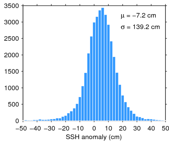
Figure 7. Histogram of flag-valid SSH anomaly over oceans and lakes for 20/08/2019. The mean ( \mu ) and standard deviation ( \sigma ) are also shown. Note that values outside [-50\ 50] cm are excluded from the histogram for the sake of readability but not from the computation of \mu and \sigma .
