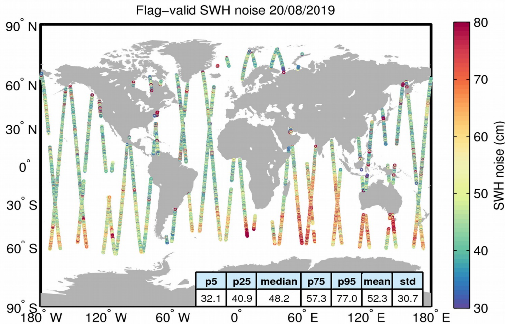
Figure 18. Geographical distribution of flag-valid 20-Hz SWH measurement noise over oceans and lakes for 20/08/2019. The statistical values shown in the table refer to the SWH noise and are calculated over all measurements shown in the figure.
