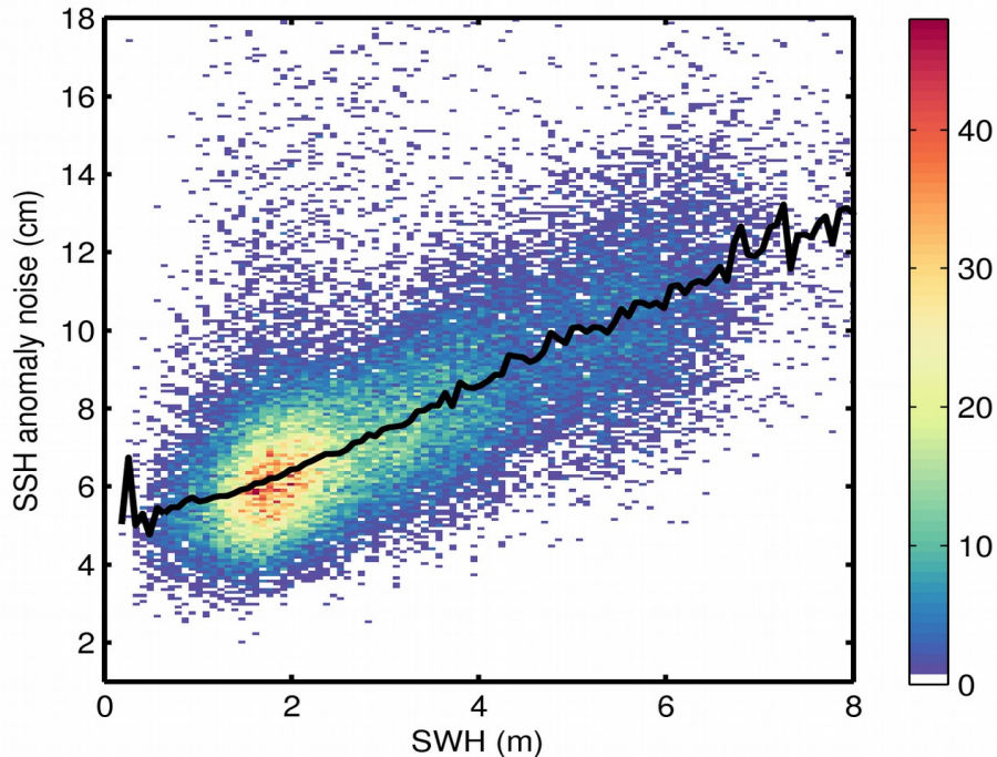
Figure 9. 2D histogram showing flag-valid SSH anomaly noise as a function of SWH for 20/08/2019. The black line denotes the median SSH anomaly noise as a function of SWH.
