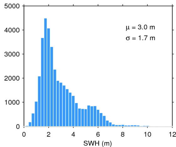
Figure 17. Histogram of flag-valid SWH over oceans and lakes for 20/08/2019. The mean ( \mu ) and standard deviation ( \sigma ) are also shown. Note that values larger than 12 m are excluded from the histogram for the sake of readability but not from the computation of \mu and \sigma .
