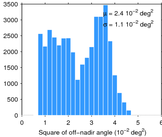
Figure 39. Histogram of flag-valid mispointing over oceans and lakes for 20/08/2019. The mean ( \mu ) and standard deviation ( \sigma ) are also shown. Note that values larger than 6 \cdot 10^{-2} \text{ deg}^2 are excluded from the histogram for the sake of readability but not from the computation of \mu and \sigma .
