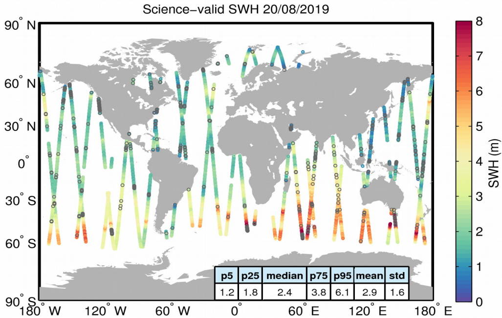
Figure 19. Geographical distribution of science-valid SWH data over oceans and lakes for 20/08/2019. The statistical values shown in the table refer to the SWH in m and are calculated over all measurements shown in the figure. Gray circles denote records that have been rejected based on the editing criteria described in Table 3.
