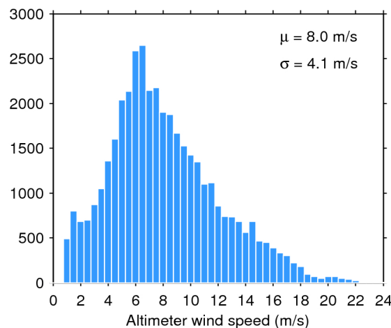
Figure 35. Histogram of science-valid wind over oceans and lakes for 20/08/2019. The mean ( \mu ) and standard deviation ( \sigma ) are also shown. Note that values larger than 24 m/s are excluded from the histogram for the sake of readability but not from the computation of \mu and \sigma .
