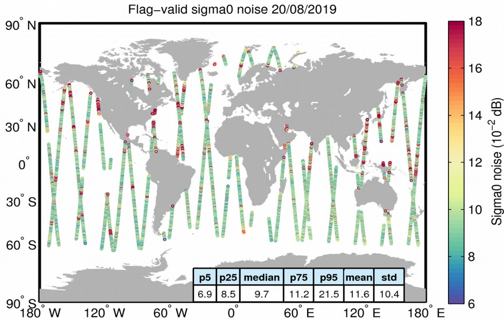
Figure 26. Geographical distribution of flag-valid 20-Hz sigma0 measurement noise over oceans and lakes for 20/08/2019. The statistical values shown in the table refer to the sigma0 noise and are calculated over all measurements shown in the figure.
