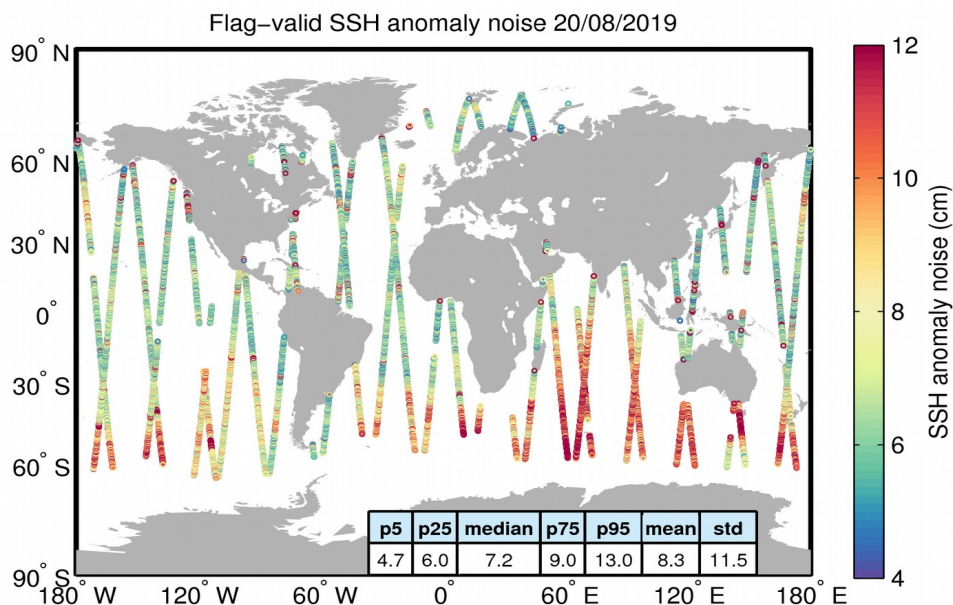
Figure 8. Geographical distribution of flag-valid 20-Hz SSH anomaly measurement noise over oceans and lakes for 20/08/2019. The statistical values shown in the table refer to the SSH anomaly noise and are calculated over all measurements shown in the figure.
