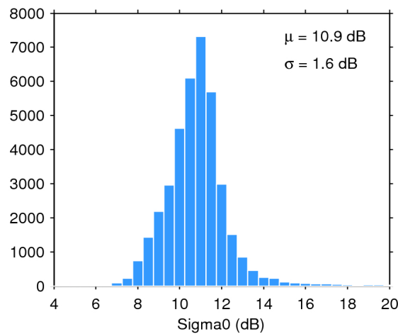
Figure 28. Histogram of science-valid sigma0 over oceans and lakes for 20/08/2019. The mean ( \mu ) and standard deviation ( \sigma ) are also shown. Note that values outside [4 20] dB are excluded from the histogram for the sake of readability but not from the computation of \mu and \sigma .
