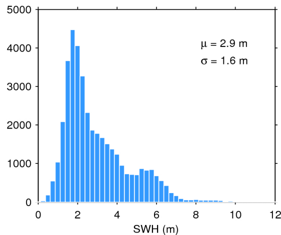
Figure 20. Histogram of science-valid SWH over oceans and lakes for 20/08/2019. The mean ( \mu ) and standard deviation ( \sigma ) are also shown. Note that values larger than 12 m are excluded from the histogram for the sake of readability but not from the computation of \mu and \sigma .
