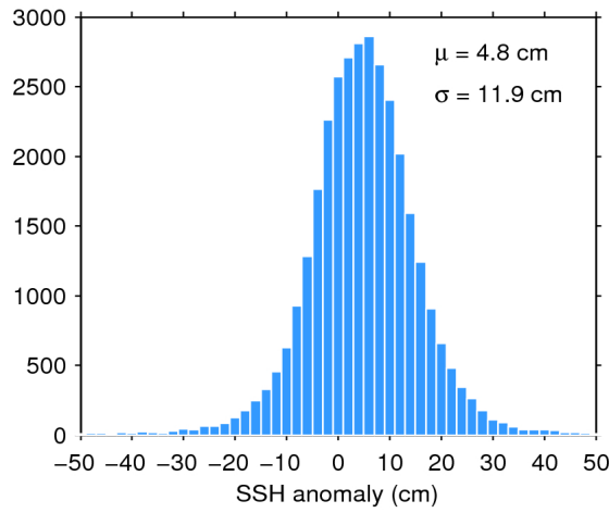
Figure 11. Histogram of science-valid SSH anomaly over oceans and lakes for 20/08/2019. The mean ( \mu ) and standard deviation ( \sigma ) are also shown. Note that values outside [-50 50] cm are excluded from the histogram for the sake of readability but not from the computation of \mu and \sigma .
