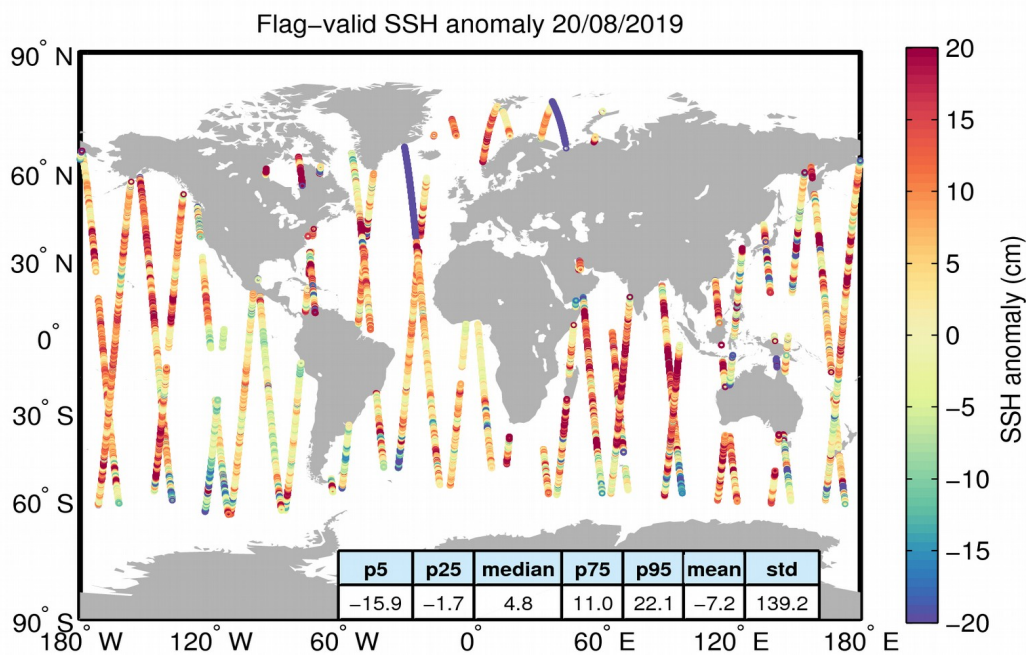
Figure 5. Geographical distribution of flag-valid 1-Hz SSH anomaly data over oceans and lakes for 20/08/2019. The statistical values shown in the table refer to the SSH anomaly in cm and are calculated over all measurements shown in the figure.
