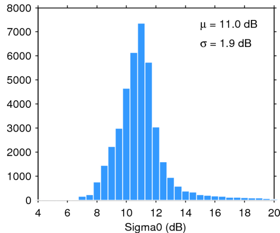
Figure 25. Histogram of flag-valid sigma0 over oceans and lakes for 20/08/2019. The mean ( \mu ) and standard deviation ( \sigma ) are also shown. Note that values outside [4 20] dB are excluded from the histogram for the sake of readability but not from the computation of \mu and \sigma .
