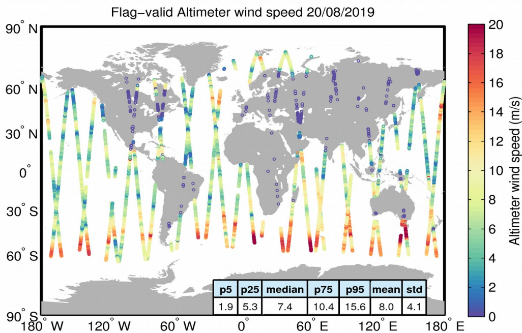
Figure 31. Geographical distribution of flag-valid wind data over oceans and lakes for 20/08/2019. The statistical values shown in the table refer to the wind in m/s and are calculated over all measurements shown in the figure.
