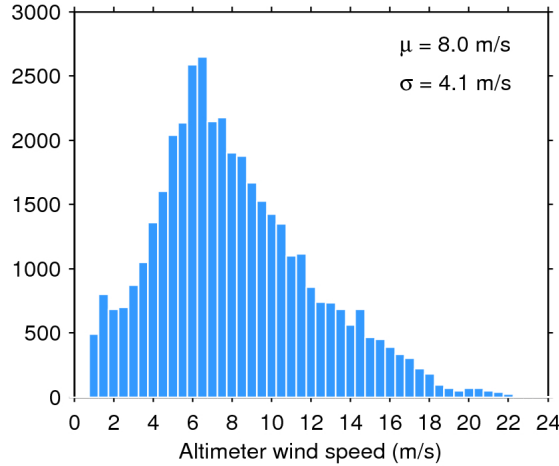
Figure 33. Histogram of flag-valid wind over oceans and lakes for 20/08/2019. The mean ( \mu ) and standard deviation ( \sigma ) are also shown. Note that values larger than 24 m/s are excluded from the histogram for the sake of readability but not from the computation of \mu and \sigma .
