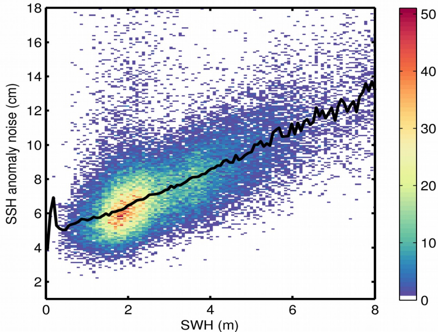
Figure 9. 2D histogram showing flag-valid SSH anomaly noise as a function of SWH for 18/08/2019. The black line denotes the median SSH anomaly noise as a function of SWH.
