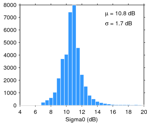
Figure 28. Histogram of science-valid sigma0 over oceans and lakes for 18/08/2019. The mean ( \mu ) and standard deviation ( \sigma ) are also shown. Note that values outside [4 20] dB are excluded from the histogram for the sake of readability but not from the computation of \mu and \sigma .
