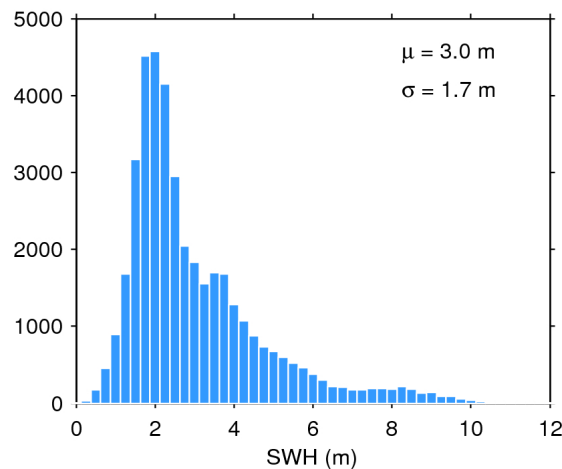
Figure 17. Histogram of flag-valid SWH over oceans and lakes for 18/08/2019. The mean ( \mu ) and standard deviation ( \sigma ) are also shown. Note that values larger than 12 m are excluded from the histogram for the sake of readability but not from the computation of \mu and \sigma .
