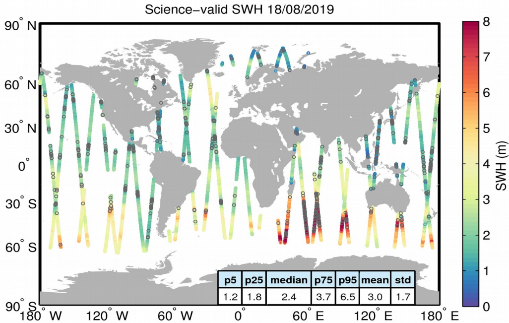
Figure 19. Geographical distribution of science-valid SWH data over oceans and lakes for 18/08/2019. The statistical values shown in the table refer to the SWH in m and are calculated over all measurements shown in the figure. Gray circles denote records that have been rejected based on the editing criteria described in Table 3.
