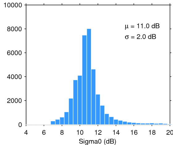
Figure 25. Histogram of flag-valid sigma0 over oceans and lakes for 18/08/2019. The mean ( \mu ) and standard deviation ( \sigma ) are also shown. Note that values outside [4 20] dB are excluded from the histogram for the sake of readability but not from the computation of \mu and \sigma .
