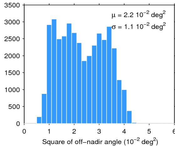
Figure 39. Histogram of flag-valid mispointing over oceans and lakes for 18/08/2019. The mean ( \mu ) and standard deviation ( \sigma ) are also shown. Note that values larger than 6 \cdot 10^{-2} \text{ deg}^2 are excluded from the histogram for the sake of readability but not from the computation of \mu and \sigma .
