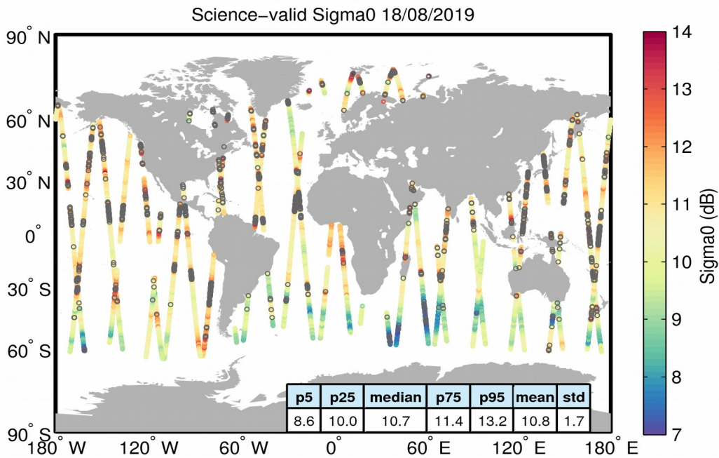
Figure 27. Geographical distribution of science-valid sigma0 data over oceans and lakes for 18/08/2019. The statistical values shown in the table refer to the sigma0 in dB and are calculated over all measurements shown in the figure. Gray circles denote records that have been rejected based on the editing criteria described in Table 4.
