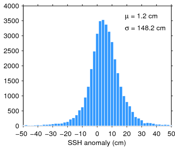
Figure 7. Histogram of flag-valid SSH anomaly over oceans and lakes for 18/08/2019. The mean ( \mu ) and standard deviation ( \sigma ) are also shown. Note that values outside [-50\ 50] cm are excluded from the histogram for the sake of readability but not from the computation of \mu and \sigma .
