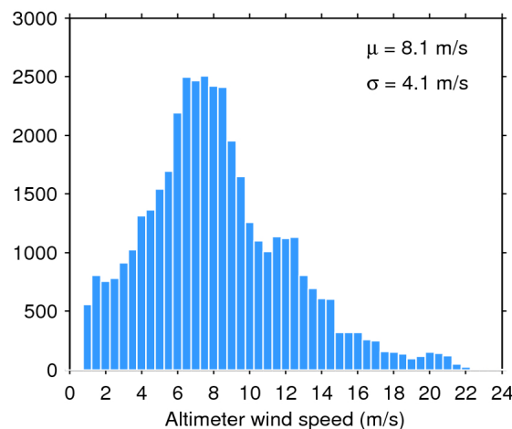
Figure 35. Histogram of science-valid wind over oceans and lakes for 18/08/2019. The mean ( \mu ) and standard deviation ( \sigma ) are also shown. Note that values larger than 24 m/s are excluded from the histogram for the sake of readability but not from the computation of \mu and \sigma .
