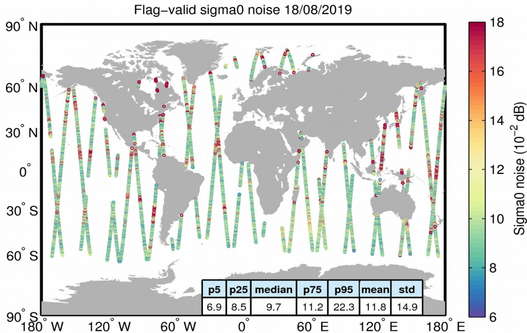
Figure 26. Geographical distribution of flag-valid 20-Hz sigma0 measurement noise over oceans and lakes for 18/08/2019. The statistical values shown in the table refer to the sigma0 noise and are calculated over all measurements shown in the figure.
