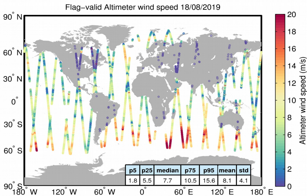
Figure 31. Geographical distribution of flag-valid wind data over oceans and lakes for 18/08/2019. The statistical values shown in the table refer to the wind in m/s and are calculated over all measurements shown in the figure.
