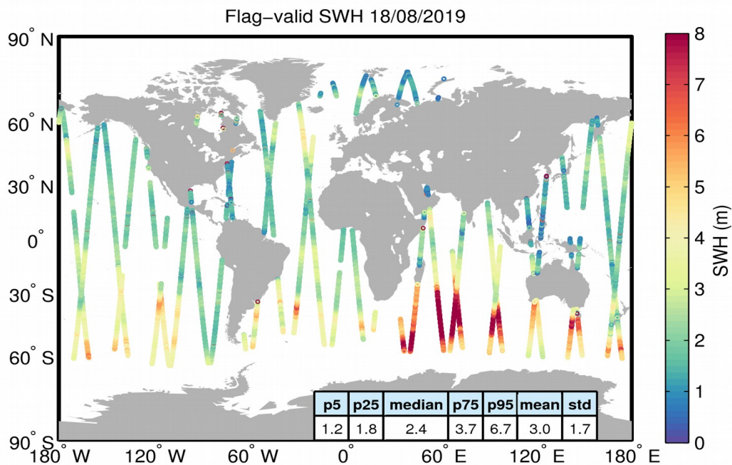
Figure 15. Geographical distribution of flag-valid SWH data over oceans and lakes for 18/08/2019. The statistical values shown in the table refer to the SWH in m and are calculated over all measurements shown in the figure.
