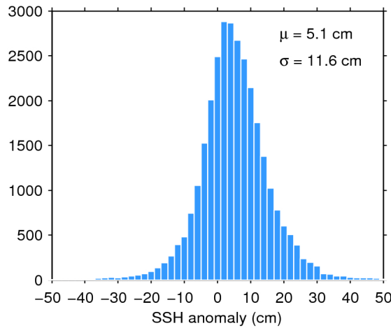
Figure 11. Histogram of science-valid SSH anomaly over oceans and lakes for 18/08/2019. The mean ( \mu ) and standard deviation ( \sigma ) are also shown. Note that values outside [-50 50] cm are excluded from the histogram for the sake of readability but not from the computation of \mu and \sigma .
