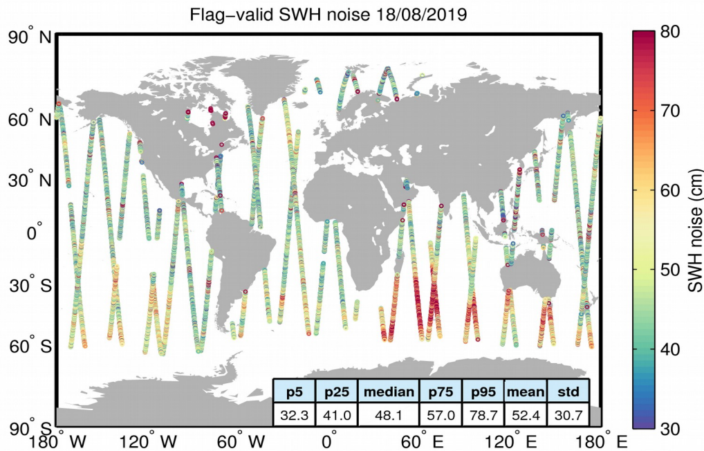
Figure 18. Geographical distribution of flag-valid 20-Hz SWH measurement noise over oceans and lakes for 18/08/2019. The statistical values shown in the table refer to the SWH noise and are calculated over all measurements shown in the figure.
