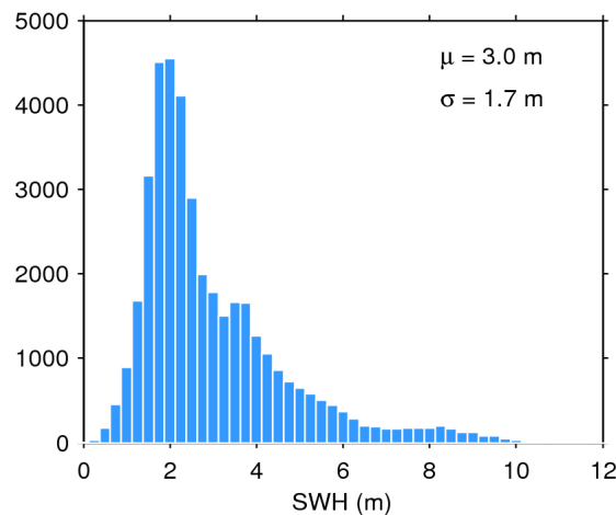
Figure 20. Histogram of science-valid SWH over oceans and lakes for 18/08/2019. The mean ( \mu ) and standard deviation ( \sigma ) are also shown. Note that values larger than 12 m are excluded from the histogram for the sake of readability but not from the computation of \mu and \sigma .
