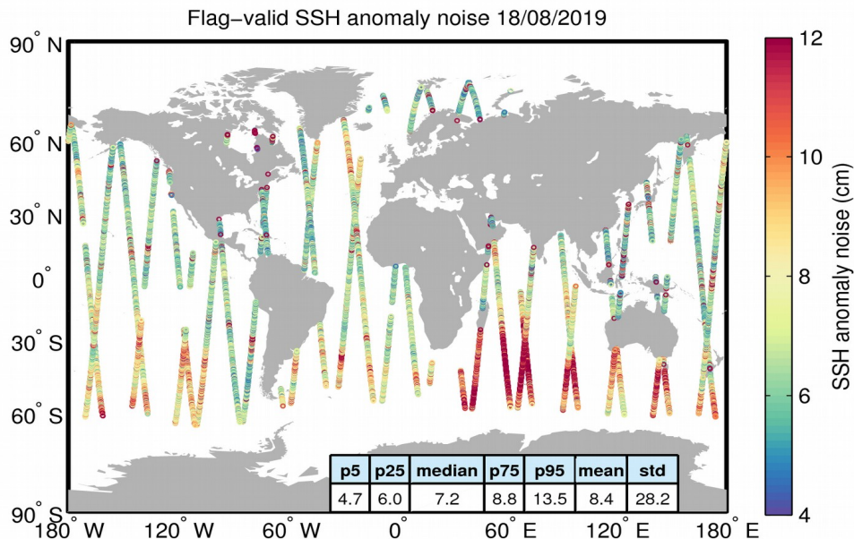
Figure 8. Geographical distribution of flag-valid 20-Hz SSH anomaly measurement noise over oceans and lakes for 18/08/2019. The statistical values shown in the table refer to the SSH anomaly noise and are calculated over all measurements shown in the figure.
