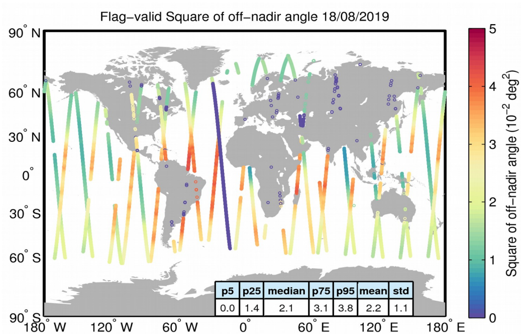
Figure 37. Geographical distribution of flag-valid mispointing data over oceans and lakes for 18/08/2019. The statistical values shown in the table refer to the mispointing in 10^{-2} \text{ deg}^2 and are calculated over all measurements shown in the figure.
