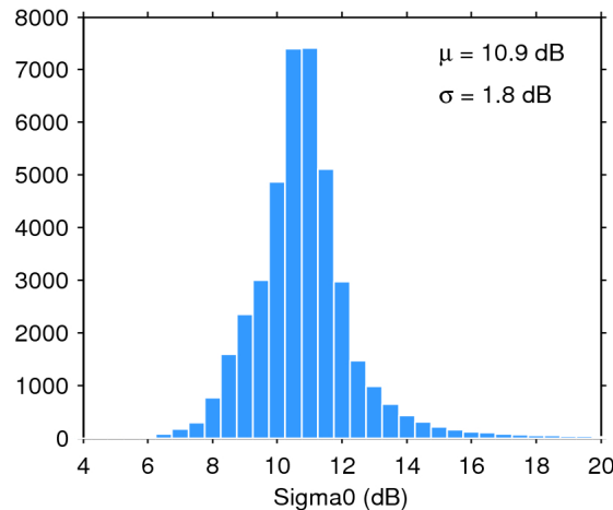
Figure 25. Histogram of flag-valid sigma0 over oceans and lakes for 16/08/2019. The mean ( \mu ) and standard deviation ( \sigma ) are also shown. Note that values outside [4 20] dB are excluded from the histogram for the sake of readability but not from the computation of \mu and \sigma .
