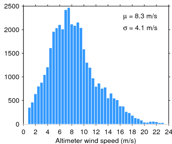
Figure 35. Histogram of science-valid wind over oceans and lakes for 16/08/2019. The mean ( \mu ) and standard deviation ( \sigma ) are also shown. Note that values larger than 24 m/s are excluded from the histogram for the sake of readability but not from the computation of \mu and \sigma .
