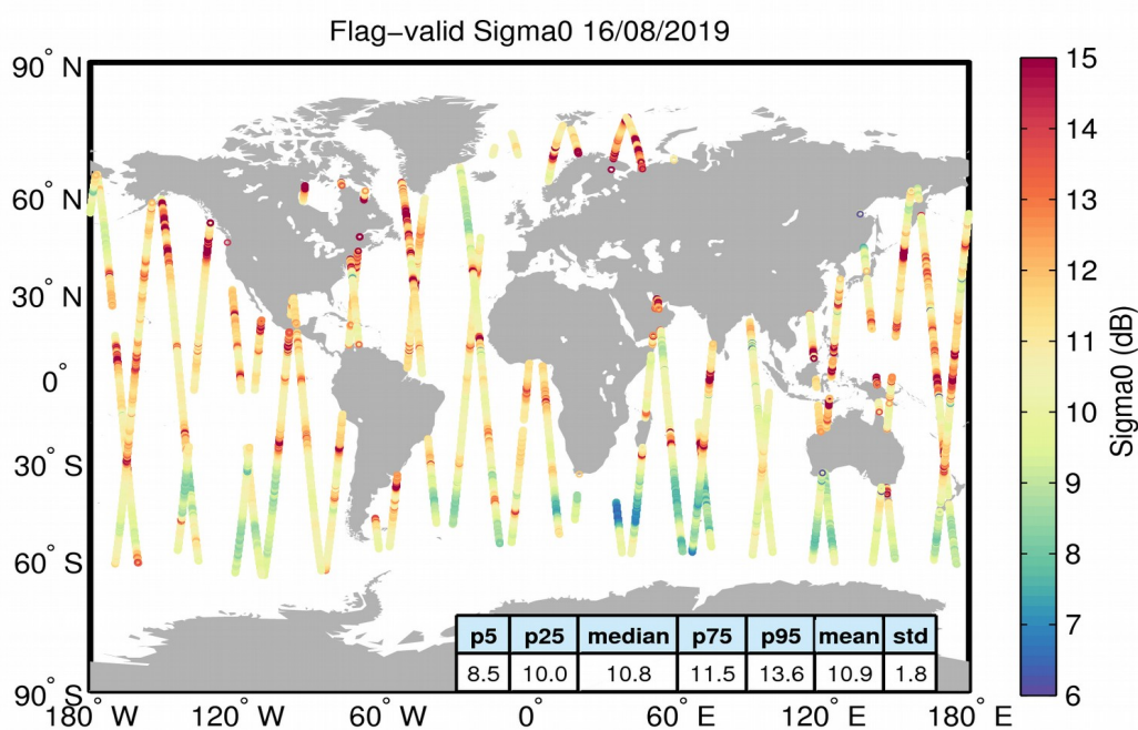
Figure 23. Geographical distribution of flag-valid sigma0 data over oceans and lakes for 16/08/2019. The statistical values shown in the table refer to the sigma0 in dB and are calculated over all measurements shown in the figure.
