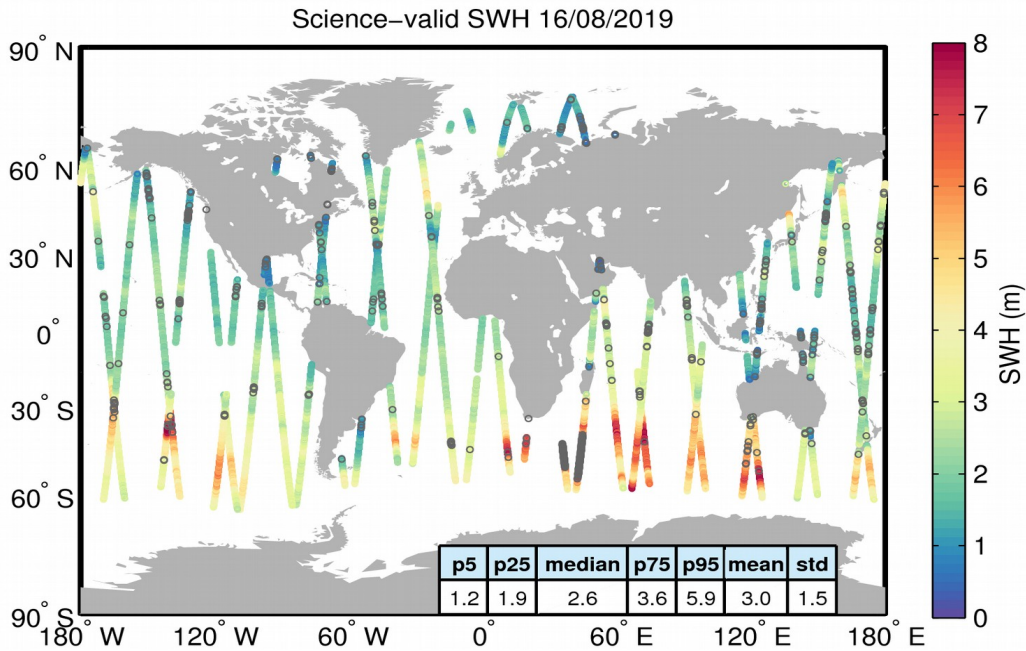
Figure 19. Geographical distribution of science-valid SWH data over oceans and lakes for 16/08/2019. The statistical values shown in the table refer to the SWH in m and are calculated over all measurements shown in the figure. Gray circles denote records that have been rejected based on the editing criteria described in Table 3.
