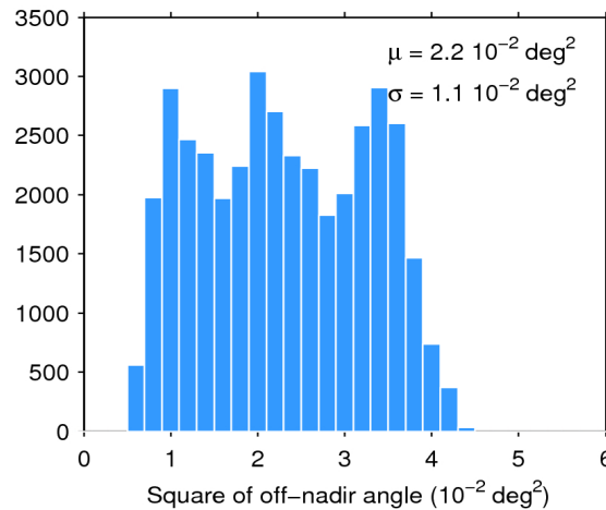
Figure 39. Histogram of flag-valid mispointing over oceans and lakes for 16/08/2019. The mean ( \mu ) and standard deviation ( \sigma ) are also shown. Note that values larger than 6 \cdot 10^{-2} \text{ deg}^2 are excluded from the histogram for the sake of readability but not from the computation of \mu and \sigma .
