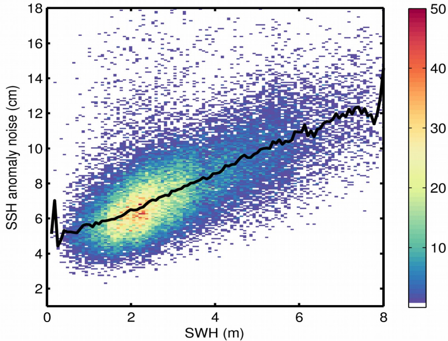
Figure 9. 2D histogram showing flag-valid SSH anomaly noise as a function of SWH for 16/08/2019. The black line denotes the median SSH anomaly noise as a function of SWH.
