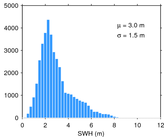
Figure 20. Histogram of science-valid SWH over oceans and lakes for 16/08/2019. The mean ( \mu ) and standard deviation ( \sigma ) are also shown. Note that values larger than 12 m are excluded from the histogram for the sake of readability but not from the computation of \mu and \sigma .
