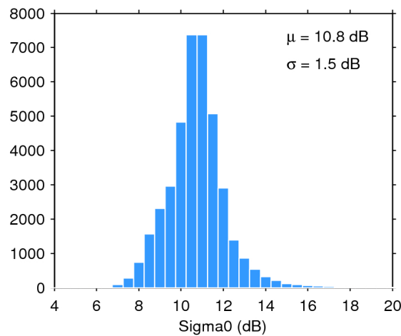
Figure 28. Histogram of science-valid sigma0 over oceans and lakes for 16/08/2019. The mean ( \mu ) and standard deviation ( \sigma ) are also shown. Note that values outside [4 20] dB are excluded from the histogram for the sake of readability but not from the computation of \mu and \sigma .
