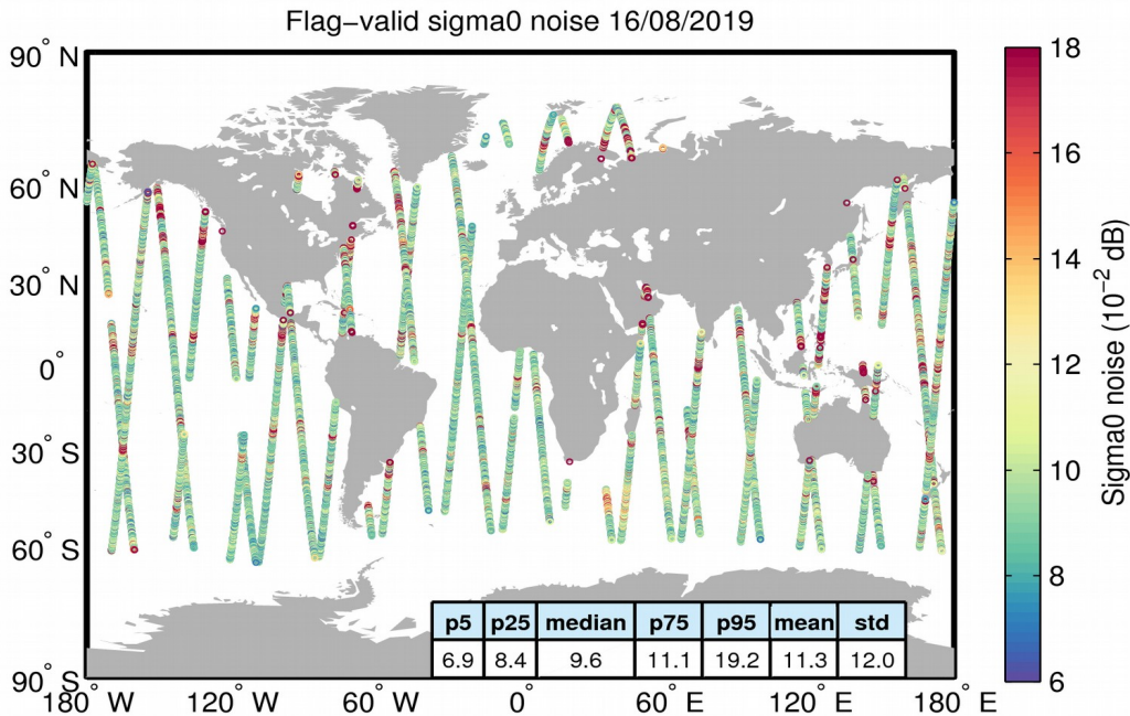
Figure 26. Geographical distribution of flag-valid 20-Hz sigma0 measurement noise over oceans and lakes for 16/08/2019. The statistical values shown in the table refer to the sigma0 noise and are calculated over all measurements shown in the figure.
