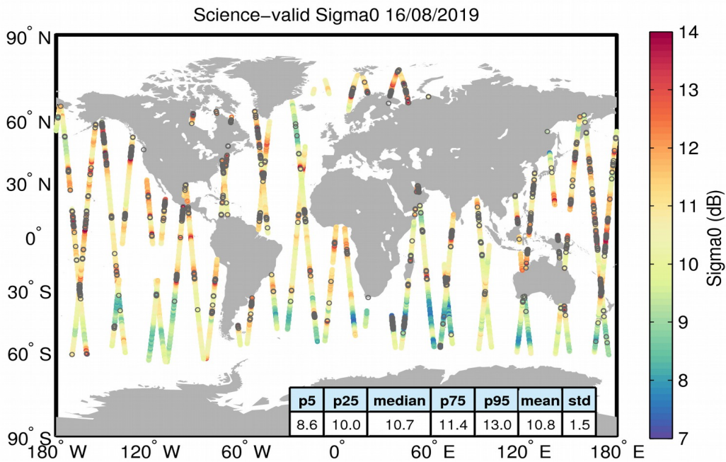
Figure 27. Geographical distribution of science-valid sigma0 data over oceans and lakes for 16/08/2019. The statistical values shown in the table refer to the sigma0 in dB and are calculated over all measurements shown in the figure. Gray circles denote records that have been rejected based on the editing criteria described in Table 4.
