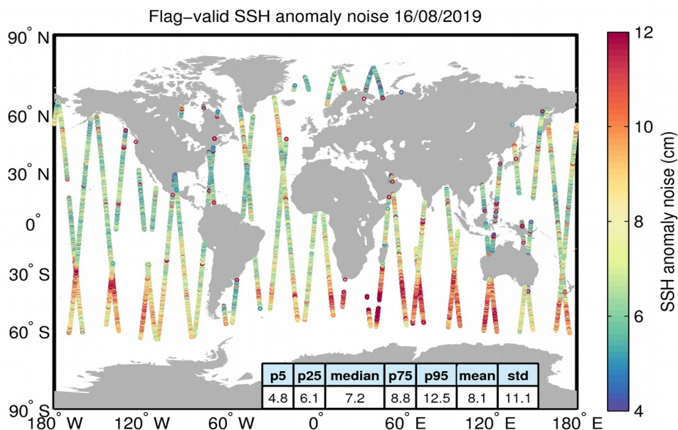
Figure 8. Geographical distribution of flag-valid 20-Hz SSH anomaly measurement noise over oceans and lakes for 16/08/2019. The statistical values shown in the table refer to the SSH anomaly noise and are calculated over all measurements shown in the figure.
