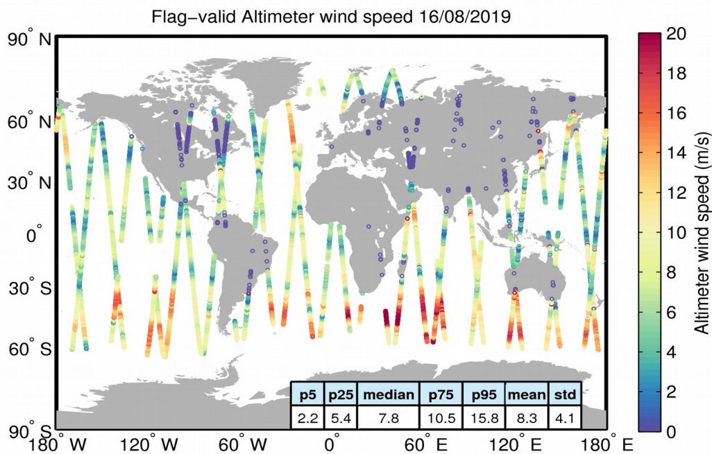
Figure 31. Geographical distribution of flag-valid wind data over oceans and lakes for 16/08/2019. The statistical values shown in the table refer to the wind in m/s and are calculated over all measurements shown in the figure.
