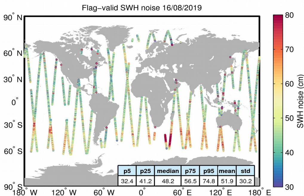
Figure 18. Geographical distribution of flag-valid 20-Hz SWH measurement noise over oceans and lakes for 16/08/2019. The statistical values shown in the figure refer to the SWH noise and are calculated over all measurements shown in the figure.
