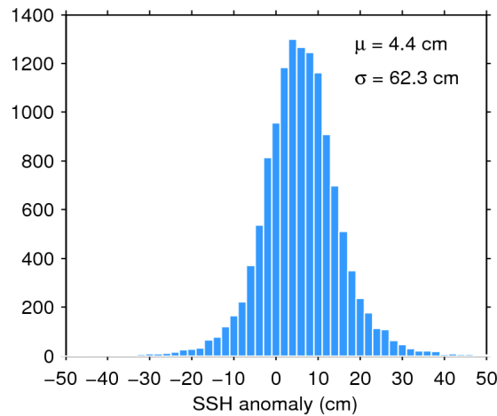
Figure 7. Histogram of flag-valid SSH anomaly over oceans and lakes for 13/08/2019. The mean ( \mu ) and standard deviation ( \sigma ) are also shown. Note that values outside [-50\ 50] cm are excluded from the histogram for the sake of readability but not from the computation of \mu and \sigma .
