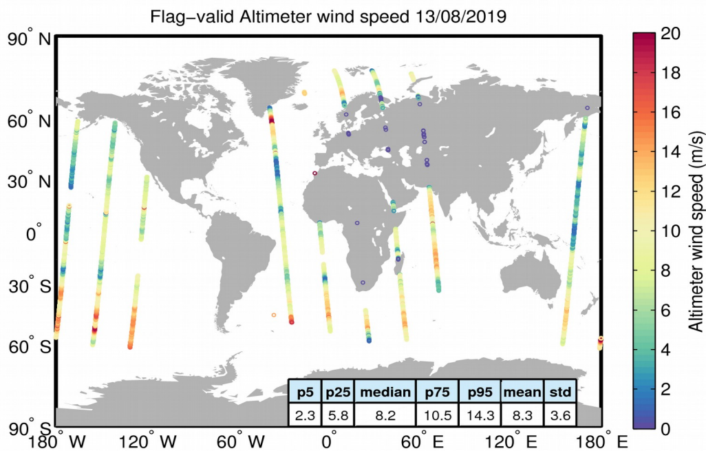
Figure 31. Geographical distribution of flag-valid wind data over oceans and lakes for 13/08/2019. The statistical values shown in the table refer to the wind in m/s and are calculated over all measurements shown in the figure.
