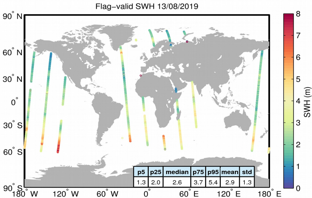
Figure 15. Geographical distribution of flag-valid SWH data over oceans and lakes for 13/08/2019. The statistical values shown in the table refer to the SWH in m and are calculated over all measurements shown in the figure.
