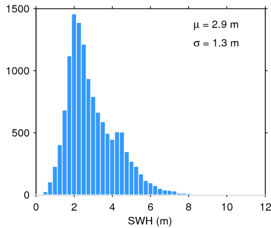
Figure 17. Histogram of flag-valid SWH over oceans and lakes for 13/08/2019. The mean ( \mu ) and standard deviation ( \sigma ) are also shown. Note that values larger than 12 m are excluded from the histogram for the sake of readability but not from the computation of \mu and \sigma .
