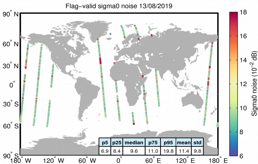
Figure 26. Geographical distribution of flag-valid 20-Hz sigma0 measurement noise over oceans and lakes for 13/08/2019. The statistical values shown in the table refer to the sigma0 noise and are calculated over all measurements shown in the figure.
