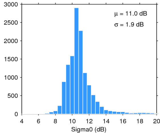
Figure 25. Histogram of flag-valid sigma0 over oceans and lakes for 13/08/2019. The mean ( \mu ) and standard deviation ( \sigma ) are also shown. Note that values outside [4 20] dB are excluded from the histogram for the sake of readability but not from the computation of \mu and \sigma .
