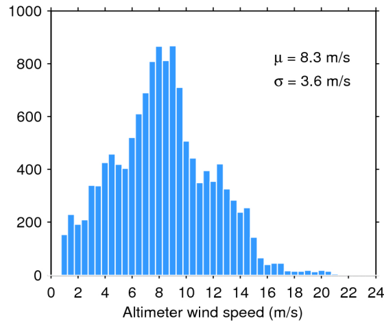
Figure 33. Histogram of flag-valid wind over oceans and lakes for 13/08/2019. The mean ( \mu ) and standard deviation ( \sigma ) are also shown. Note that values larger than 24 m/s are excluded from the histogram for the sake of readability but not from the computation of \mu and \sigma .
