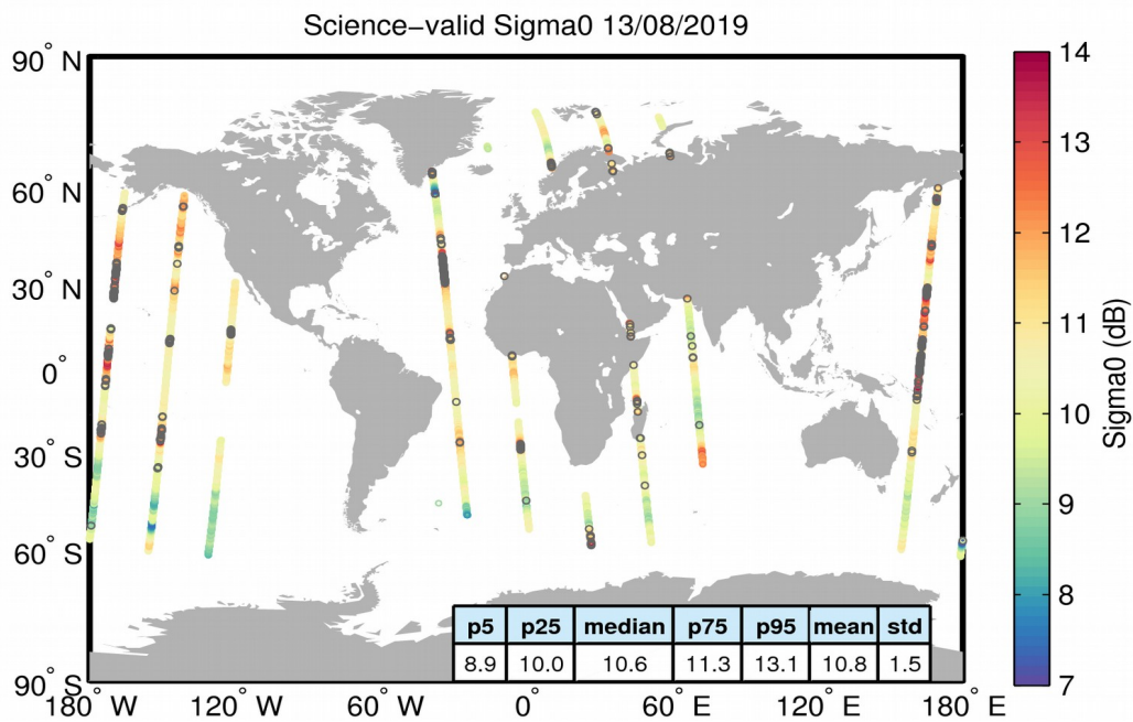
Figure 27. Geographical distribution of science-valid sigma0 data over oceans and lakes for 13/08/2019. The statistical values shown in the table refer to the sigma0 in dB and are calculated over all measurements shown in the figure. Gray circles denote records that have been rejected based on the editing criteria described in Table 4.
