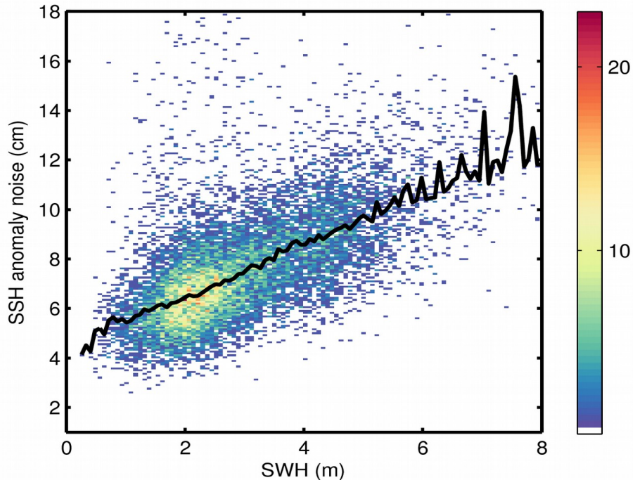
Figure 9. 2D histogram showing flag-valid SSH anomaly noise as a function of SWH for 13/08/2019. The black line denotes the median SSH anomaly noise as a function of SWH.
