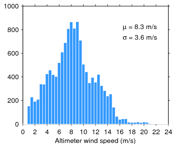
Figure 35. Histogram of science-valid wind over oceans and lakes for 13/08/2019. The mean ( \mu ) and standard deviation ( \sigma ) are also shown. Note that values larger than 24 m/s are excluded from the histogram for the sake of readability but not from the computation of \mu and \sigma .
