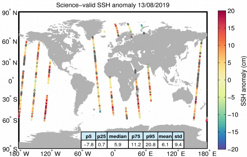
Figure 10. Geographical distribution of science-valid SSH anomaly data over oceans and lakes for 13/08/2019. The statistical values shown in the table refer to the SSH anomaly in cm and are calculated over all measurements shown in the figure. Gray circles denote records that have been rejected based on the editing criteria described in Table 2.
