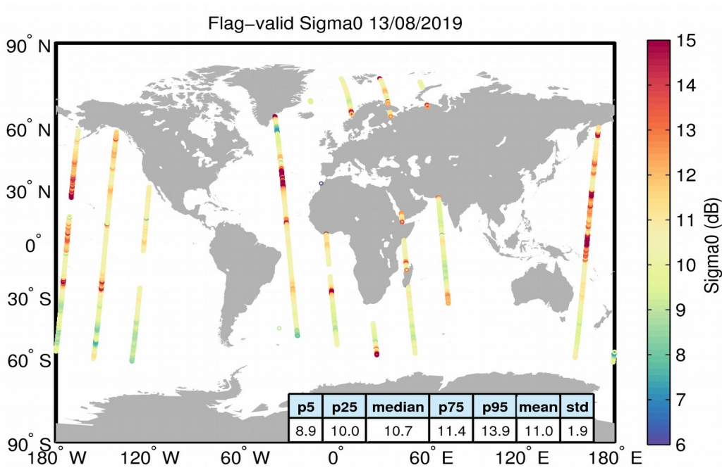
Figure 23. Geographical distribution of flag-valid sigma0 data over oceans and lakes for 13/08/2019. The statistical values shown in the table refer to the sigma0 in dB and are calculated over all measurements shown in the figure.
