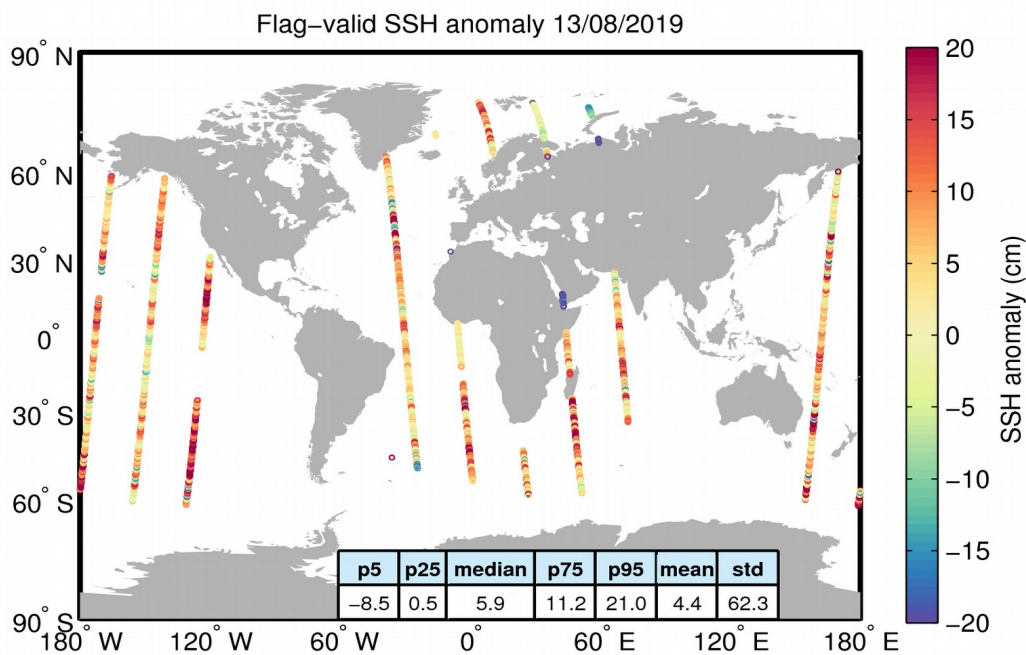
Figure 5. Geographical distribution of flag-valid 1-Hz SSH anomaly data over oceans and lakes for 13/08/2019. The statistical values shown in the table refer to the SSH anomaly in cm and are calculated over all measurements shown in the figure.
