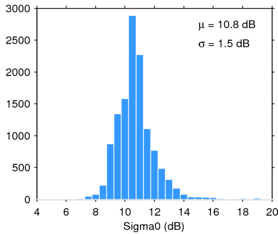
Figure 28. Histogram of science-valid sigma0 over oceans and lakes for 13/08/2019. The mean ( \mu ) and standard deviation ( \sigma ) are also shown. Note that values outside [4 20] dB are excluded from the histogram for the sake of readability but not from the computation of \mu and \sigma .
