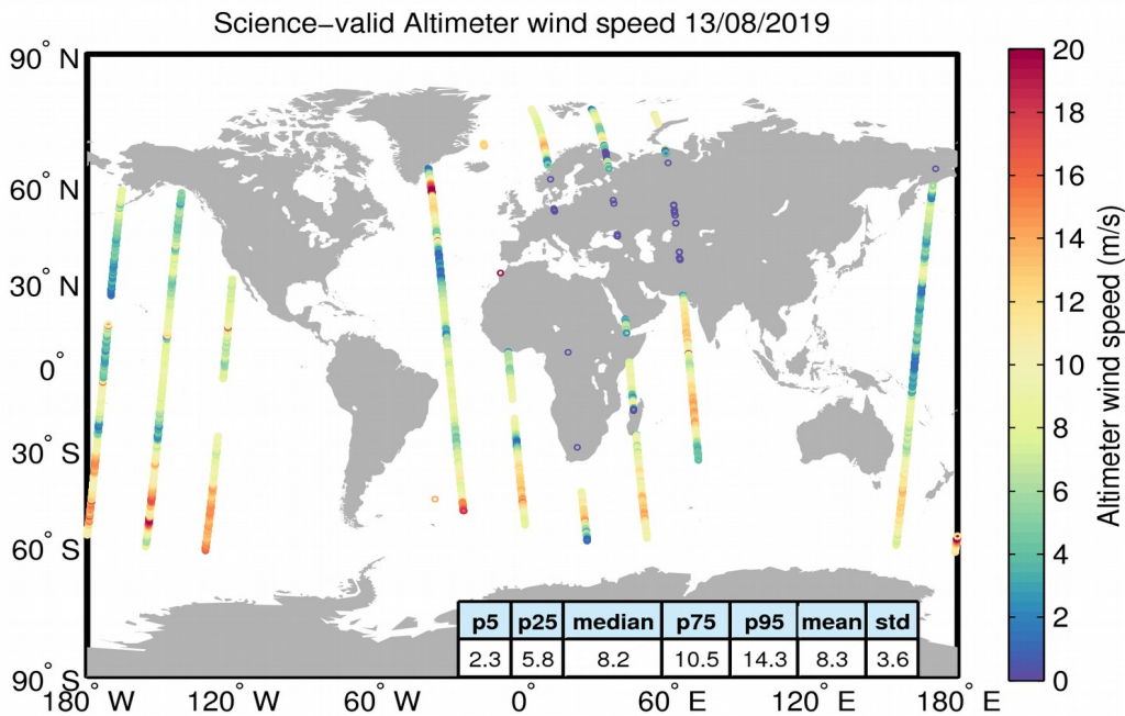
Figure 34. Geographical distribution of science-valid wind data over oceans and lakes for 13/08/2019. The statistical values shown in the table refer to the wind in m/s and are calculated over all measurements shown in the figure. Gray circles denote records that have been rejected based on the editing criteria described in Table 5.
