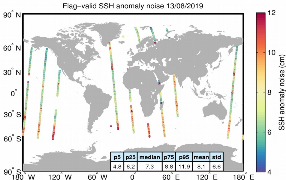
Figure 8. Geographical distribution of flag-valid 20-Hz SSH anomaly measurement noise over oceans and lakes for 13/08/2019. The statistical values shown in the table refer to the SSH anomaly noise and are calculated over all measurements shown in the figure.
