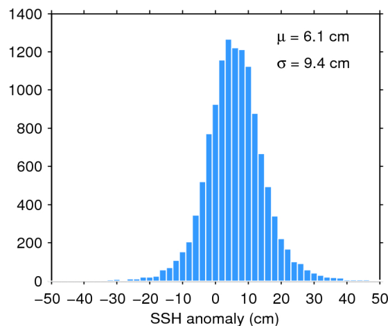
Figure 11. Histogram of science-valid SSH anomaly over oceans and lakes for 13/08/2019. The mean ( \mu ) and standard deviation ( \sigma ) are also shown. Note that values outside [-50 50] cm are excluded from the histogram for the sake of readability but not from the computation of \mu and \sigma .
