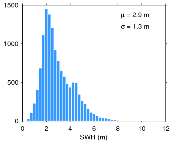
Figure 20. Histogram of science-valid SWH over oceans and lakes for 13/08/2019. The mean ( \mu ) and standard deviation ( \sigma ) are also shown. Note that values larger than 12 m are excluded from the histogram for the sake of readability but not from the computation of \mu and \sigma .
