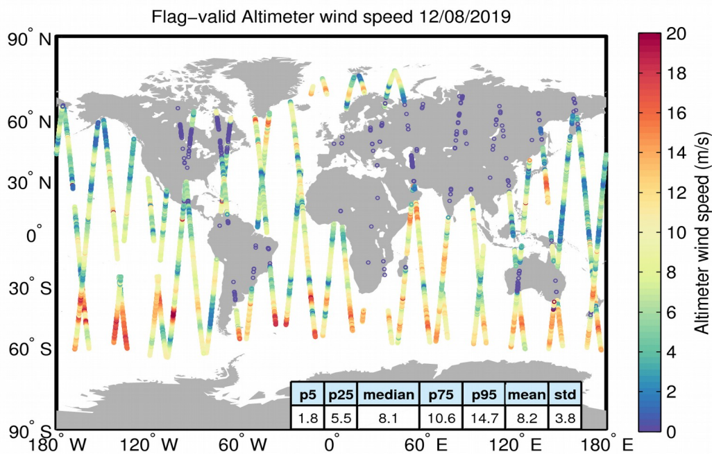
Figure 31. Geographical distribution of flag-valid wind data over oceans and lakes for 12/08/2019. The statistical values shown in the table refer to the wind in m/s and are calculated over all measurements shown in the figure.
