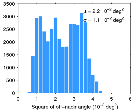
Figure 39. Histogram of flag-valid mispointing over oceans and lakes for 12/08/2019. The mean ( \mu ) and standard deviation ( \sigma ) are also shown. Note that values larger than 6 \cdot 10^{-2} \text{ deg}^2 are excluded from the histogram for the sake of readability but not from the computation of \mu and \sigma .
