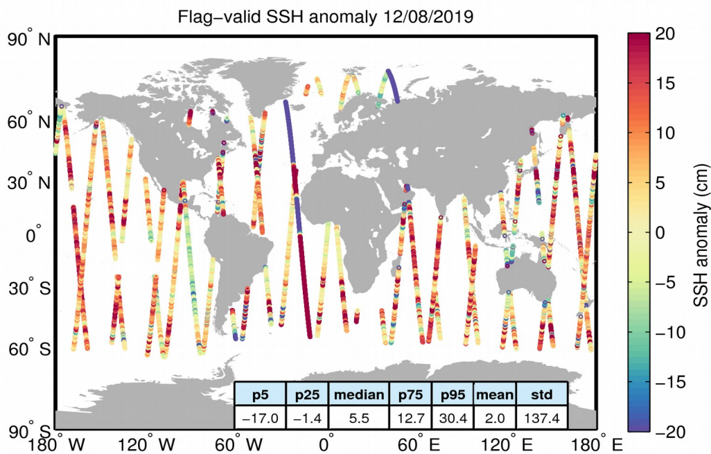
Figure 5. Geographical distribution of flag-valid 1-Hz SSH anomaly data over oceans and lakes for 12/08/2019. The statistical values shown in the table refer to the SSH anomaly in cm and are calculated over all measurements shown in the figure.
