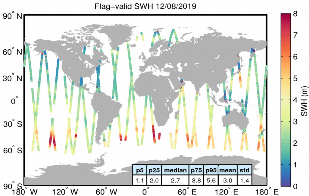
Figure 15. Geographical distribution of flag-valid SWH data over oceans and lakes for 12/08/2019. The statistical values shown in the table refer to the SWH in m and are calculated over all measurements shown in the figure.
