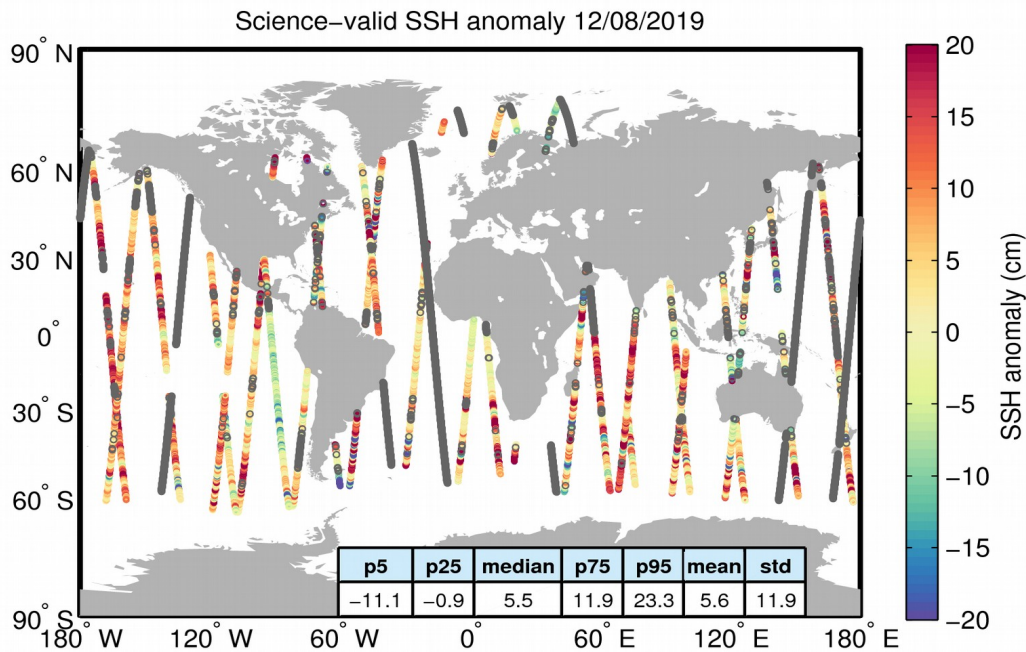
Figure 10. Geographical distribution of science-valid SSH anomaly data over oceans and lakes for 12/08/2019. The statistical values shown in the table refer to the SSH anomaly in cm and are calculated over all measurements shown in the figure. Gray circles denote records that have been rejected based on the editing criteria described in Table 2.
