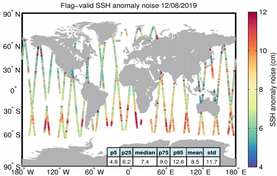
Figure 8. Geographical distribution of flag-valid 20-Hz SSH anomaly measurement noise over oceans and lakes for 12/08/2019. The statistical values shown in the table refer to the SSH anomaly noise and are calculated over all measurements shown in the figure.
