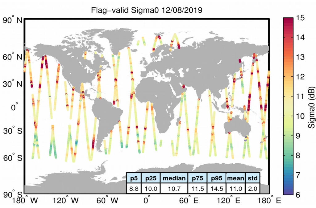
Figure 23. Geographical distribution of flag-valid sigma0 data over oceans and lakes for 12/08/2019. The statistical values shown in the table refer to the sigma0 in dB and are calculated over all measurements shown in the figure.
