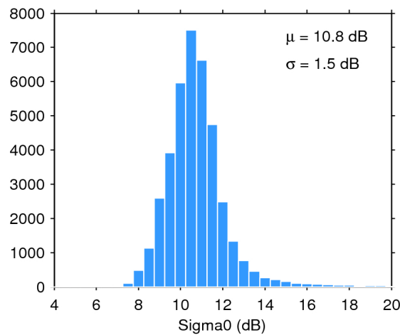
Figure 28. Histogram of science-valid sigma0 over oceans and lakes for 12/08/2019. The mean ( \mu ) and standard deviation ( \sigma ) are also shown. Note that values outside [4 20] dB are excluded from the histogram for the sake of readability but not from the computation of \mu and \sigma .
