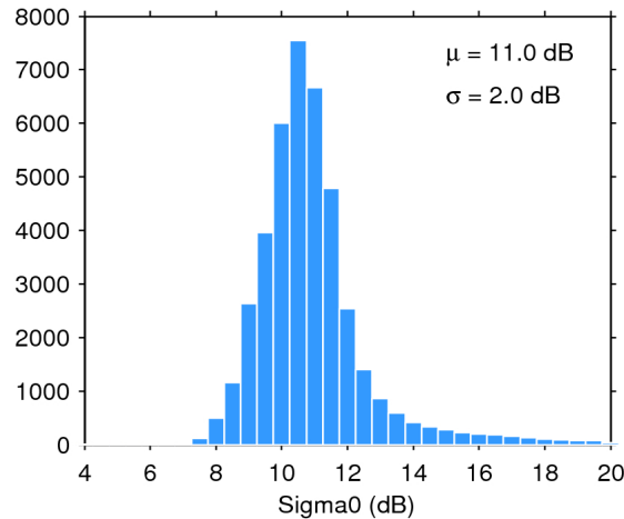
Figure 25. Histogram of flag-valid sigma0 over oceans and lakes for 12/08/2019. The mean ( \mu ) and standard deviation ( \sigma ) are also shown. Note that values outside [4 20] dB are excluded from the histogram for the sake of readability but not from the computation of \mu and \sigma .
