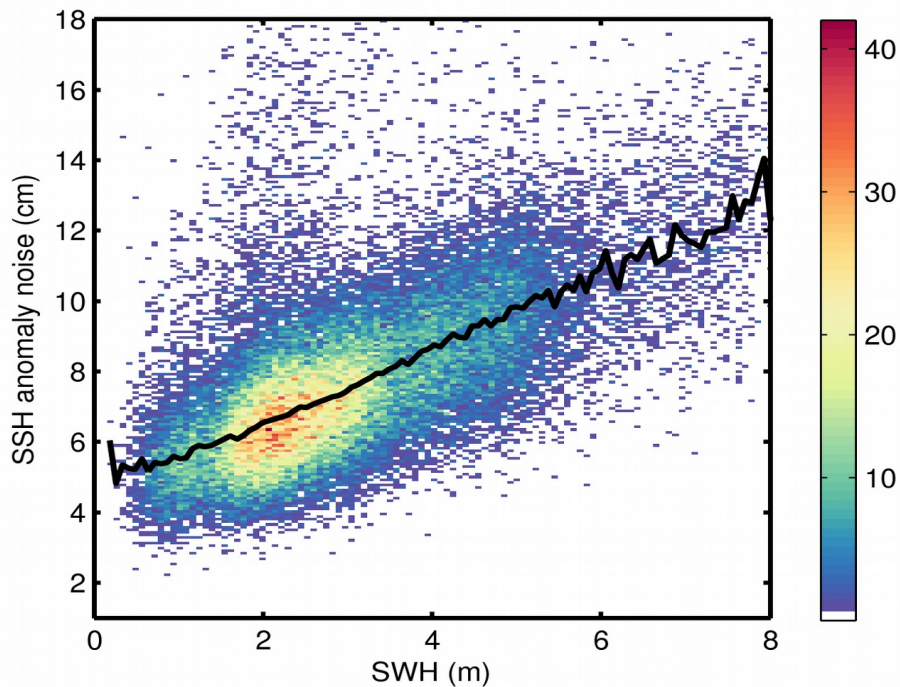
Figure 9. 2D histogram showing flag-valid SSH anomaly noise as a function of SWH for 12/08/2019. The black line denotes the median SSH anomaly noise as a function of SWH.
