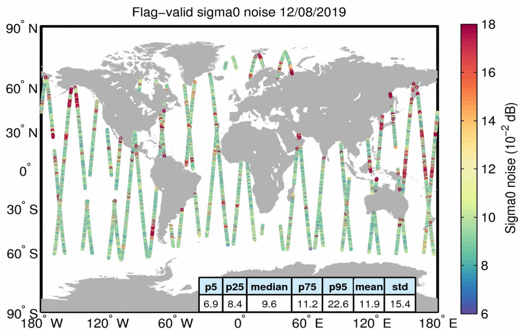
Figure 26. Geographical distribution of flag-valid 20-Hz sigma0 measurement noise over oceans and lakes for 12/08/2019. The statistical values shown in the figure refer to the sigma0 noise and are calculated over all measurements shown in the figure.
