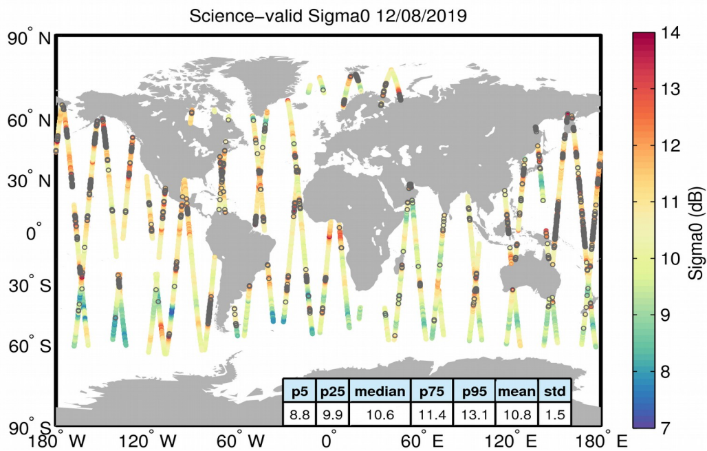
Figure 27. Geographical distribution of science-valid sigma0 data over oceans and lakes for 12/08/2019. The statistical values shown in the table refer to the sigma0 in dB and are calculated over all measurements shown in the figure. Gray circles denote records that have been rejected based on the editing criteria described in Table 4.
