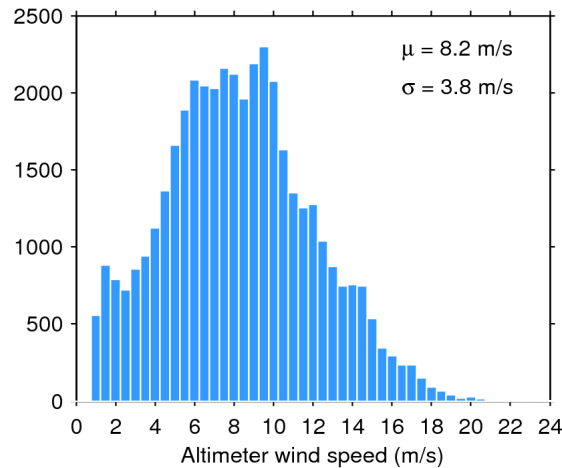
Figure 33. Histogram of flag-valid wind over oceans and lakes for 12/08/2019. The mean ( \mu ) and standard deviation ( \sigma ) are also shown. Note that values larger than 24 m/s are excluded from the histogram for the sake of readability but not from the computation of \mu and \sigma .
