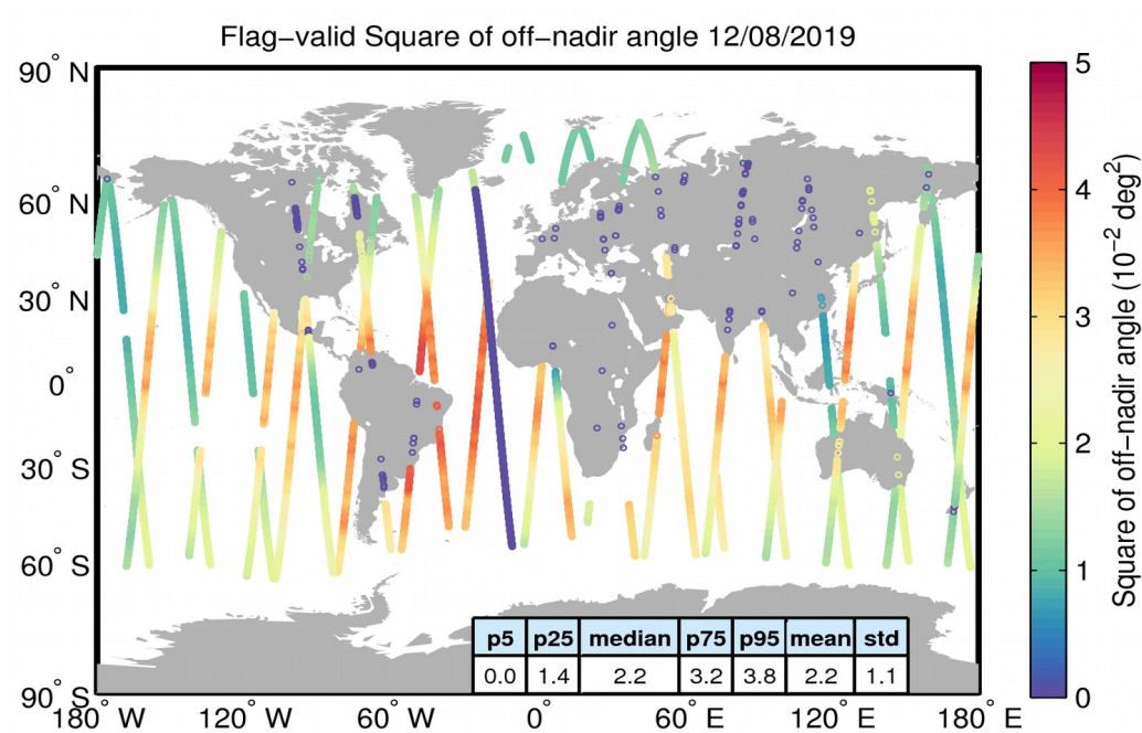
Figure 37. Geographical distribution of flag-valid mispointing data over oceans and lakes for 12/08/2019. The statistical values shown in the table refer to the mispointing in 10^{-2} deg 2 and are calculated over all measurements shown in the figure.
