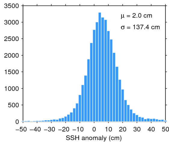
Figure 7. Histogram of flag-valid SSH anomaly over oceans and lakes for 12/08/2019. The mean ( \mu ) and standard deviation ( \sigma ) are also shown. Note that values outside [-50\ 50] cm are excluded from the histogram for the sake of readability but not from the computation of \mu and \sigma .
