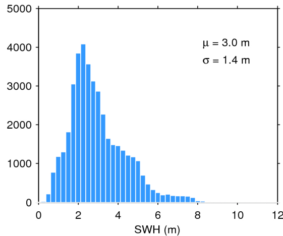
Figure 20. Histogram of science-valid SWH over oceans and lakes for 12/08/2019. The mean ( \mu ) and standard deviation ( \sigma ) are also shown. Note that values larger than 12 m are excluded from the histogram for the sake of readability but not from the computation of \mu and \sigma .
