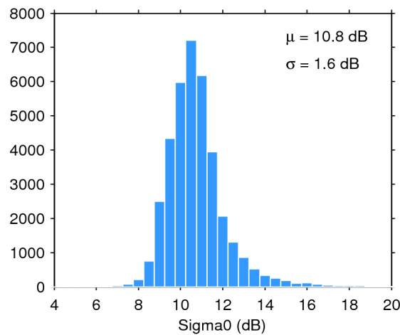
Figure 28. Histogram of science-valid sigma0 over oceans and lakes for 07/08/2019. The mean ( \mu ) and standard deviation ( \sigma ) are also shown. Note that values outside [4 20] dB are excluded from the histogram for the sake of readability but not from the computation of \mu and \sigma .
