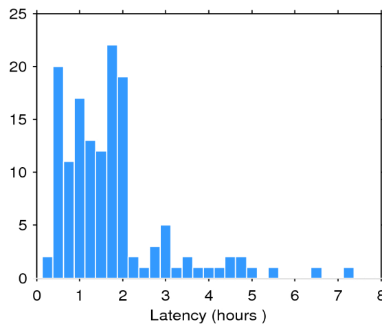
Figure 2. Histogram of the data latency for 07/08/2019. The y-axis denotes the number of files that are made available with a delay of x-hours with respect to the mean time of the records stored in the file.
