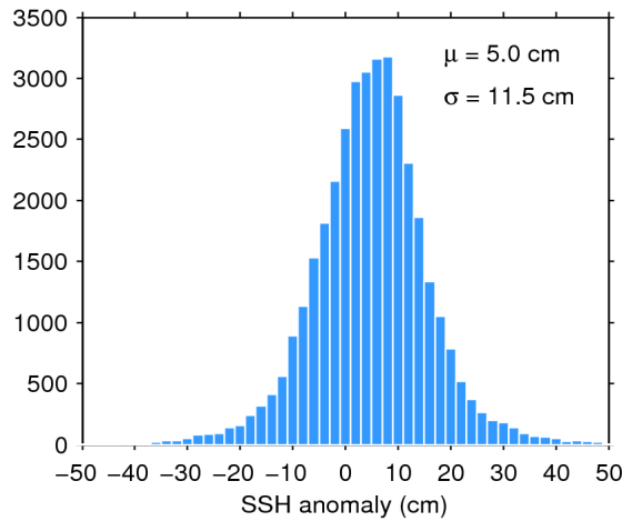
Figure 11. Histogram of science-valid SSH anomaly over oceans and lakes for 07/08/2019. The mean ( \mu ) and standard deviation ( \sigma ) are also shown. Note that values outside [-50 50] cm are excluded from the histogram for the sake of readability but not from the computation of \mu and \sigma .
