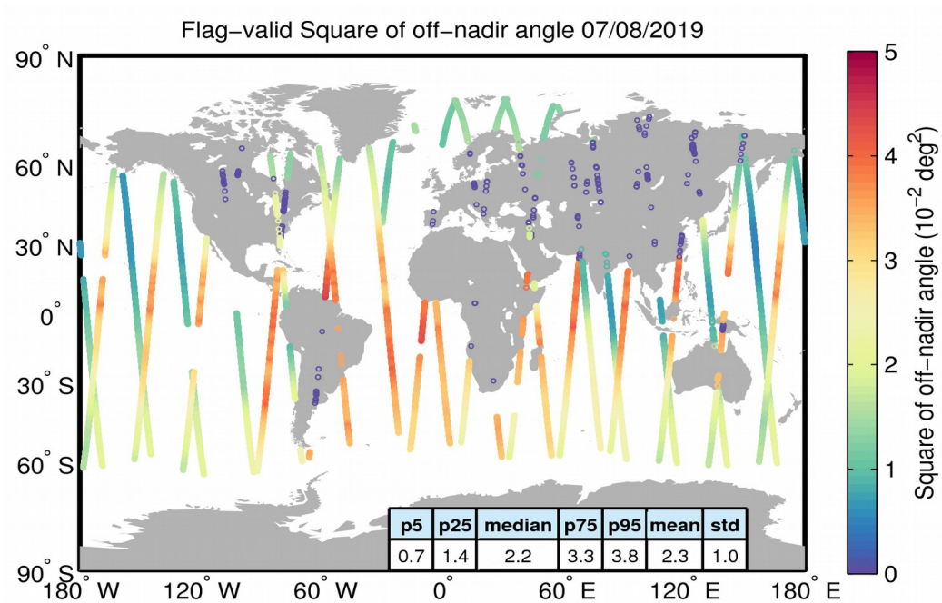
Figure 37. Geographical distribution of flag-valid mispointing data over oceans and lakes for 07/08/2019. The statistical values shown in the table refer to the mispointing in 10^{-2} deg 2 and are calculated over all measurements shown in the figure.
