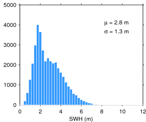
Figure 20. Histogram of science-valid SWH over oceans and lakes for 07/08/2019. The mean ( \mu ) and standard deviation ( \sigma ) are also shown. Note that values larger than 12 m are excluded from the histogram for the sake of readability but not from the computation of \mu and \sigma .
