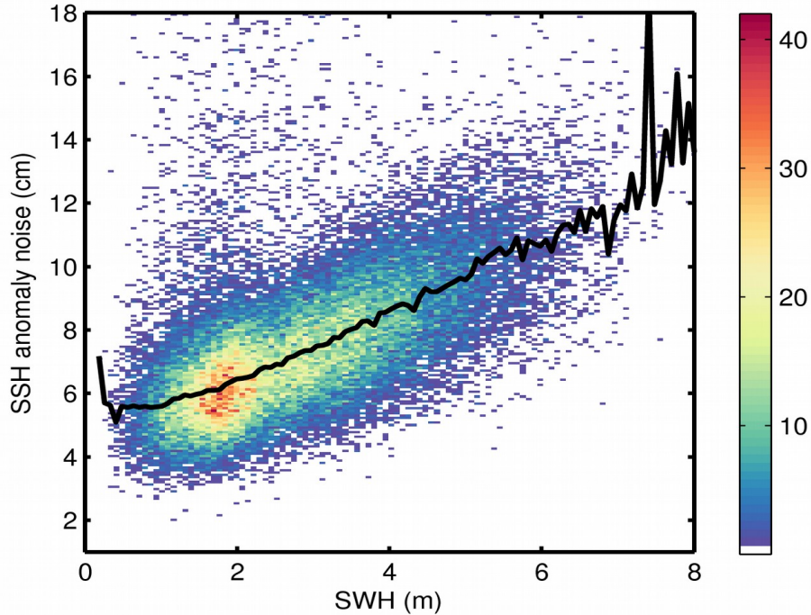
Figure 9. 2D histogram showing flag-valid SSH anomaly noise as a function of SWH for 07/08/2019. The black line denotes the median SSH anomaly noise as a function of SWH.
