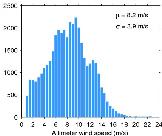
Figure 35. Histogram of science-valid wind over oceans and lakes for 07/08/2019. The mean ( \mu ) and standard deviation ( \sigma ) are also shown. Note that values larger than 24 m/s are excluded from the histogram for the sake of readability but not from the computation of \mu and \sigma .
