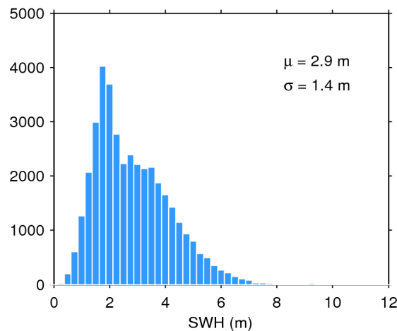
Figure 17. Histogram of flag-valid SWH over oceans and lakes for 07/08/2019. The mean ( \mu ) and standard deviation ( \sigma ) are also shown. Note that values larger than 12 m are excluded from the histogram for the sake of readability but not from the computation of \mu and \sigma .
