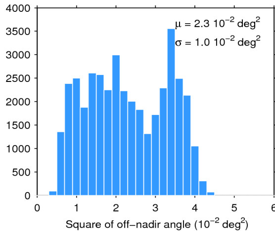
Figure 39. Histogram of flag-valid mispointing over oceans and lakes for 07/08/2019. The mean ( \mu ) and standard deviation ( \sigma ) are also shown. Note that values larger than 6 \cdot 10^{-2} \text{ deg}^2 are excluded from the histogram for the sake of readability but not from the computation of \mu and \sigma .
