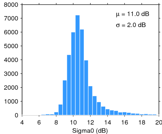
Figure 25. Histogram of flag-valid sigma0 over oceans and lakes for 07/08/2019. The mean ( \mu ) and standard deviation ( \sigma ) are also shown. Note that values outside [4 20] dB are excluded from the histogram for the sake of readability but not from the computation of \mu and \sigma .
