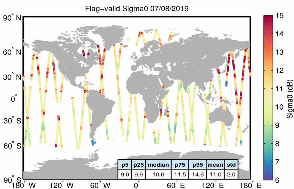
Figure 23. Geographical distribution of flag-valid sigma0 data over oceans and lakes for 07/08/2019. The statistical values shown in the table refer to the sigma0 in dB and are calculated over all measurements shown in the figure.
