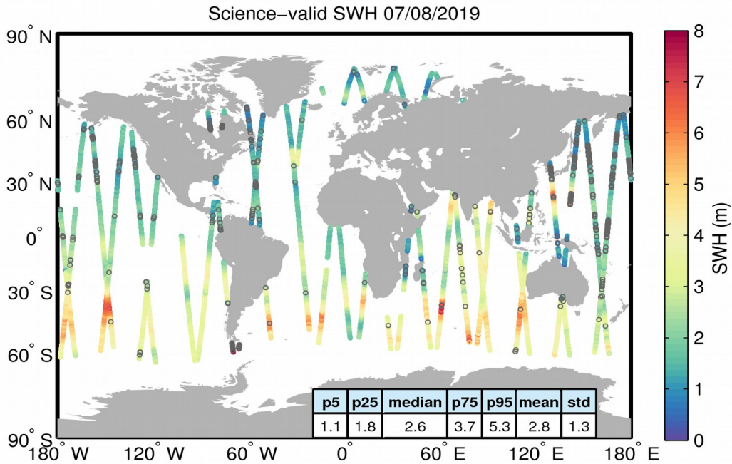
Figure 19. Geographical distribution of science-valid SWH data over oceans and lakes for 07/08/2019. The statistical values shown in the table refer to the SWH in m and are calculated over all measurements shown in the figure. Gray circles denote records that have been rejected based on the editing criteria described in Table 3.
