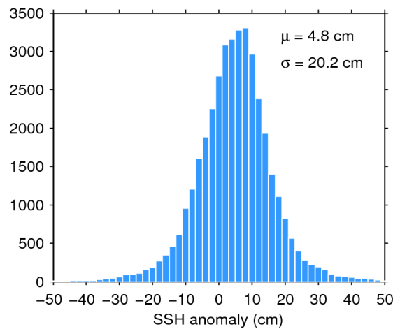
Figure 7. Histogram of flag-valid SSH anomaly over oceans and lakes for 07/08/2019. The mean ( \mu ) and standard deviation ( \sigma ) are also shown. Note that values outside [-50\ 50] cm are excluded from the histogram for the sake of readability but not from the computation of \mu and \sigma .
