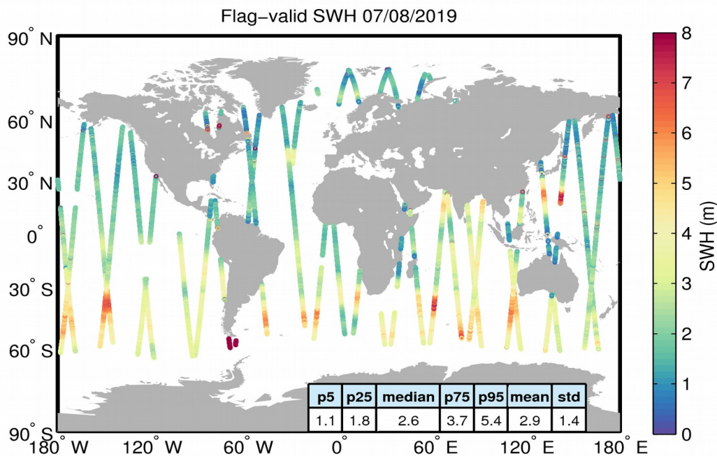
Figure 15. Geographical distribution of flag-valid SWH data over oceans and lakes for 07/08/2019. The statistical values shown in the table refer to the SWH in m and are calculated over all measurements shown in the figure.
