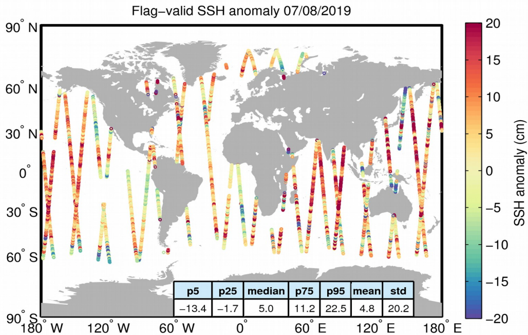
Figure 5. Geographical distribution of flag-valid 1-Hz SSH anomaly data over oceans and lakes for 07/08/2019. The statistical values shown in the table refer to the SSH anomaly in cm and are calculated over all measurements shown in the figure.
