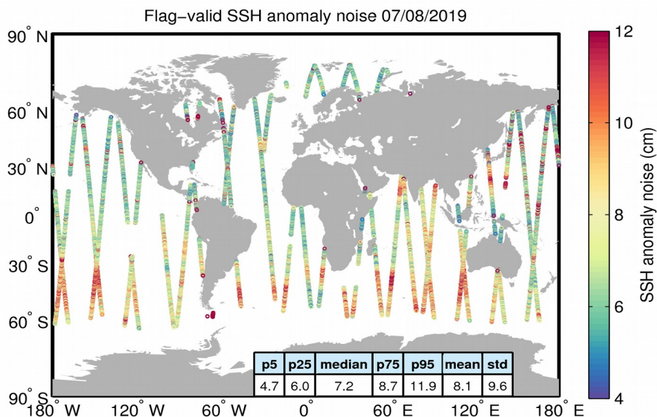
Figure 8. Geographical distribution of flag-valid 20-Hz SSH anomaly measurement noise over oceans and lakes for 07/08/2019. The statistical values shown in the table refer to the SSH anomaly noise and are calculated over all measurements shown in the figure.
