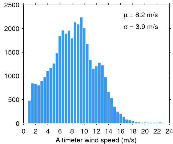
Figure 33. Histogram of flag-valid wind over oceans and lakes for 07/08/2019. The mean ( \mu ) and standard deviation ( \sigma ) are also shown. Note that values larger than 24 m/s are excluded from the histogram for the sake of readability but not from the computation of \mu and \sigma .
