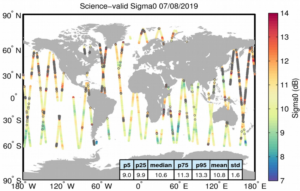
Figure 27. Geographical distribution of science-valid sigma0 data over oceans and lakes for 07/08/2019. The statistical values shown in the table refer to the sigma0 in dB and are calculated over all measurements shown in the figure. Gray circles denote records that have been rejected based on the editing criteria described in Table 4.
