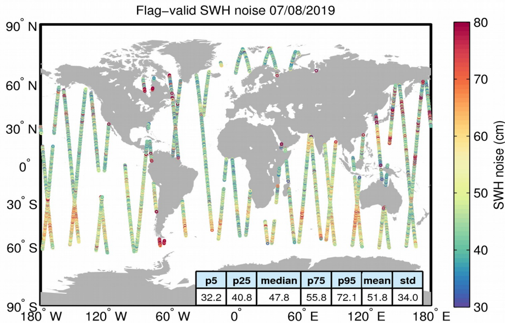
Figure 18. Geographical distribution of flag-valid 20-Hz SWH measurement noise over oceans and lakes for 07/08/2019. The statistical values shown in the table refer to the SWH noise and are calculated over all measurements shown in the figure.
