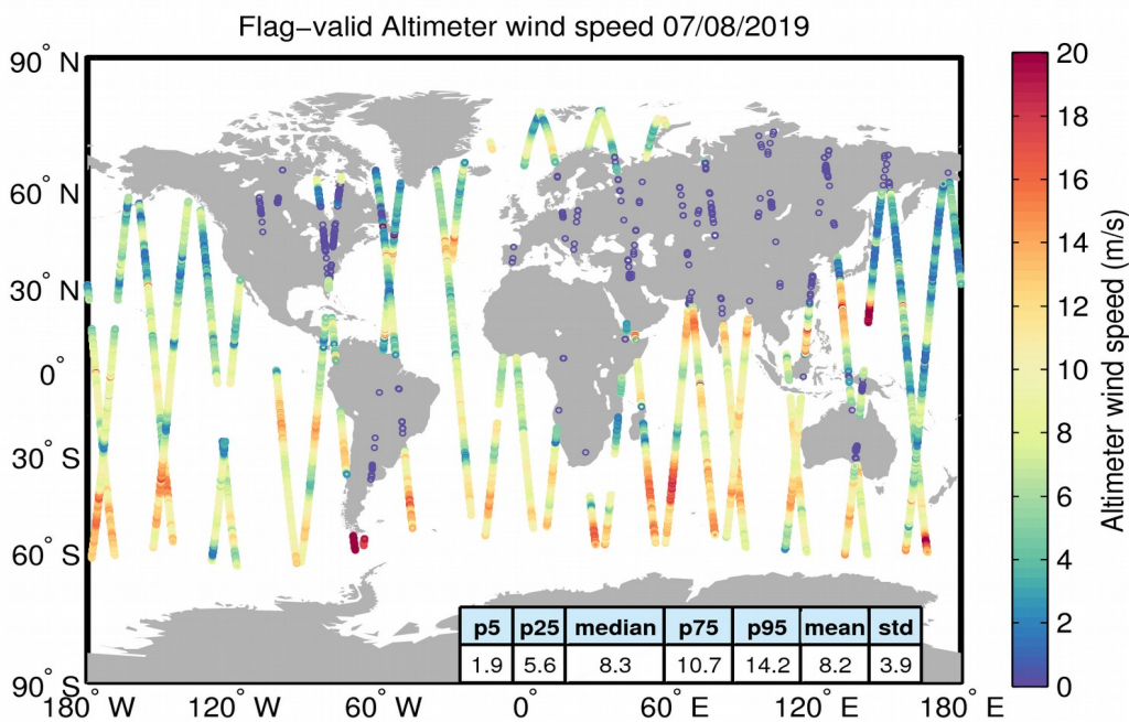
Figure 31. Geographical distribution of flag-valid wind data over oceans and lakes for 07/08/2019. The statistical values shown in the table refer to the wind in m/s and are calculated over all measurements shown in the figure.
