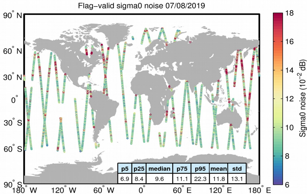
Figure 26. Geographical distribution of flag-valid 20-Hz sigma0 measurement noise over oceans and lakes for 07/08/2019. The statistical values shown in the table refer to the sigma0 noise and are calculated over all measurements shown in the figure.
