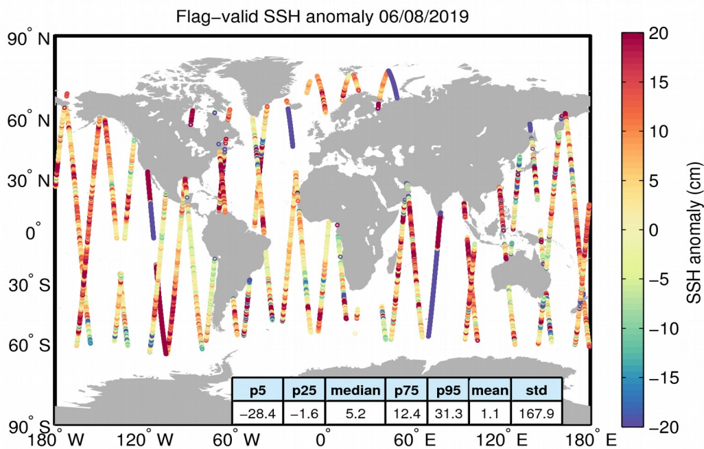
Figure 5. Geographical distribution of flag-valid 1-Hz SSH anomaly data over oceans and lakes for 06/08/2019. The statistical values shown in the table refer to the SSH anomaly in cm and are calculated over all measurements shown in the figure.
