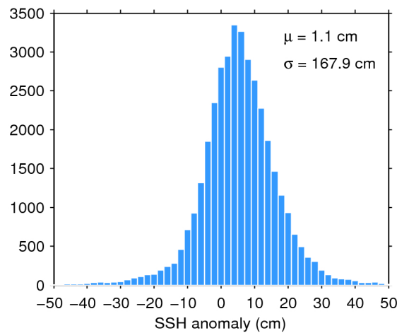
Figure 7. Histogram of flag-valid SSH anomaly over oceans and lakes for 06/08/2019. The mean ( \mu ) and standard deviation ( \sigma ) are also shown. Note that values outside [-50\ 50] cm are excluded from the histogram for the sake of readability but not from the computation of \mu and \sigma .
