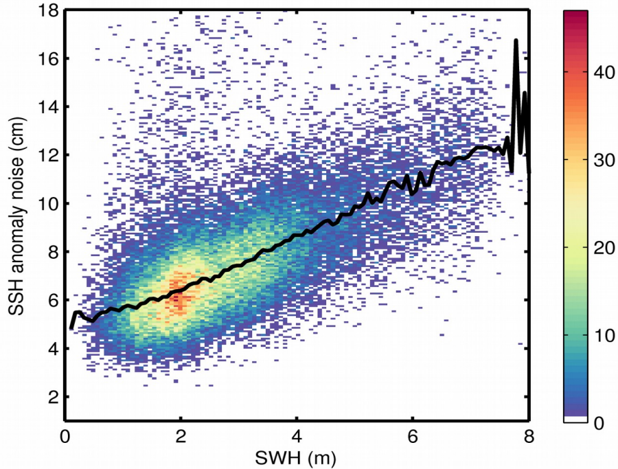
Figure 9. 2D histogram showing flag-valid SSH anomaly noise as a function of SWH for 06/08/2019. The black line denotes the median SSH anomaly noise as a function of SWH.
