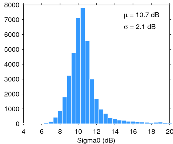
Figure 25. Histogram of flag-valid sigma0 over oceans and lakes for 06/08/2019. The mean ( \mu ) and standard deviation ( \sigma ) are also shown. Note that values outside [4 20] dB are excluded from the histogram for the sake of readability but not from the computation of \mu and \sigma .
