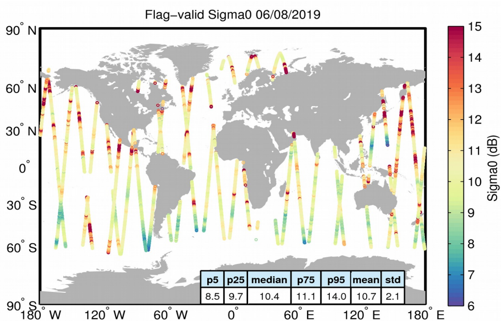
Figure 23. Geographical distribution of flag-valid sigma0 data over oceans and lakes for 06/08/2019. The statistical values shown in the table refer to the sigma0 in dB and are calculated over all measurements shown in the figure.
