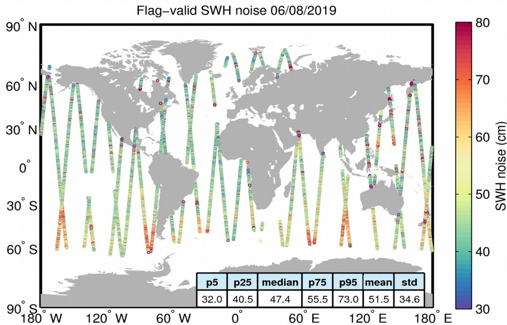
Figure 18. Geographical distribution of flag-valid 20-Hz SWH measurement noise over oceans and lakes for 06/08/2019. The statistical values shown in the figure refer to the SWH noise and are calculated over all measurements shown in the figure.
