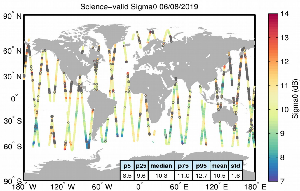
Figure 27. Geographical distribution of science-valid sigma0 data over oceans and lakes for 06/08/2019. The statistical values shown in the table refer to the sigma0 in dB and are calculated over all measurements shown in the figure. Gray circles denote records that have been rejected based on the editing criteria described in Table 4.
