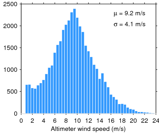
Figure 33. Histogram of flag-valid wind over oceans and lakes for 06/08/2019. The mean ( \mu ) and standard deviation ( \sigma ) are also shown. Note that values larger than 24 m/s are excluded from the histogram for the sake of readability but not from the computation of \mu and \sigma .
