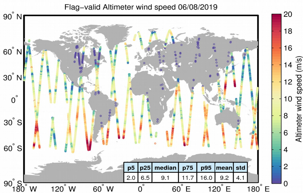
Figure 31. Geographical distribution of flag-valid wind data over oceans and lakes for 06/08/2019. The statistical values shown in the table refer to the wind in m/s and are calculated over all measurements shown in the figure.
