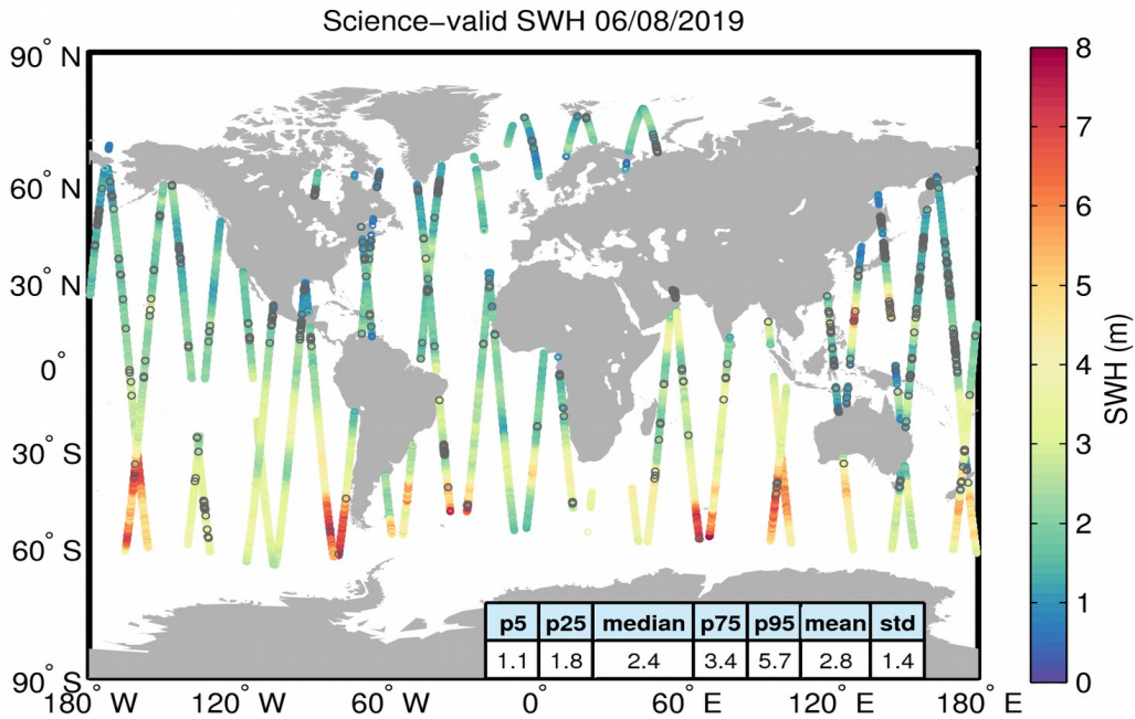
Figure 19. Geographical distribution of science-valid SWH data over oceans and lakes for 06/08/2019. The statistical values shown in the table refer to the SWH in m and are calculated over all measurements shown in the figure. Gray circles denote records that have been rejected based on the editing criteria described in Table 3.
