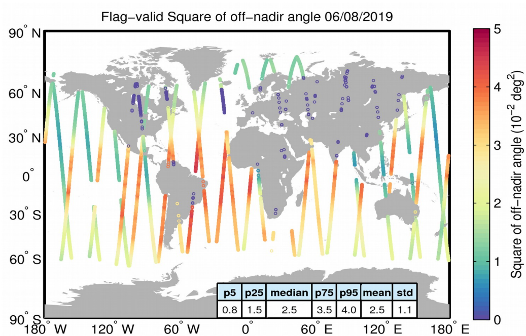
Figure 37. Geographical distribution of flag-valid mispointing data over oceans and lakes for 06/08/2019. The statistical values shown in the table refer to the mispointing in 10^{-2} \text{ deg}^2 and are calculated over all measurements shown in the figure.
