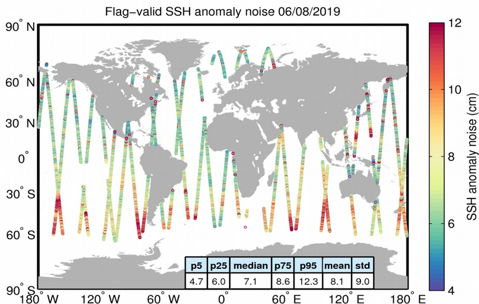
Figure 8. Geographical distribution of flag-valid 20-Hz SSH anomaly measurement noise over oceans and lakes for 06/08/2019. The statistical values shown in the table refer to the SSH anomaly noise and are calculated over all measurements shown in the figure.
