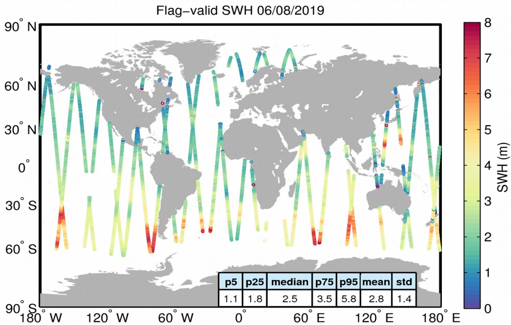
Figure 15. Geographical distribution of flag-valid SWH data over oceans and lakes for 06/08/2019. The statistical values shown in the table refer to the SWH in m and are calculated over all measurements shown in the figure.
