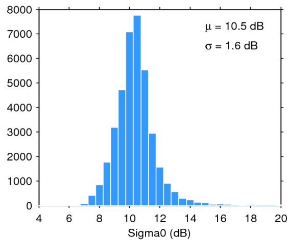
Figure 28. Histogram of science-valid sigma0 over oceans and lakes for 06/08/2019. The mean ( \mu ) and standard deviation ( \sigma ) are also shown. Note that values outside [4 20] dB are excluded from the histogram for the sake of readability but not from the computation of \mu and \sigma .
