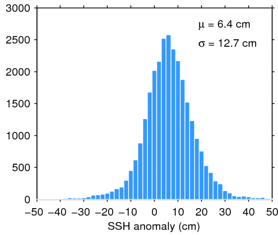
Figure 11. Histogram of science-valid SSH anomaly over oceans and lakes for 06/08/2019. The mean ( \mu ) and standard deviation ( \sigma ) are also shown. Note that values outside [-50 50] cm are excluded from the histogram for the sake of readability but not from the computation of \mu and \sigma .
