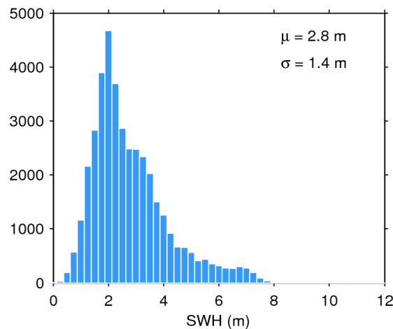
Figure 20. Histogram of science-valid SWH over oceans and lakes for 06/08/2019. The mean ( \mu ) and standard deviation ( \sigma ) are also shown. Note that values larger than 12 m are excluded from the histogram for the sake of readability but not from the computation of \mu and \sigma .
