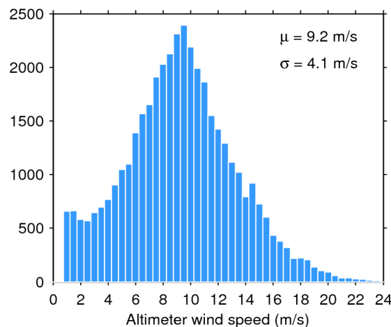
Figure 35. Histogram of science-valid wind over oceans and lakes for 06/08/2019. The mean ( \mu ) and standard deviation ( \sigma ) are also shown. Note that values larger than 24 m/s are excluded from the histogram for the sake of readability but not from the computation of \mu and \sigma .
