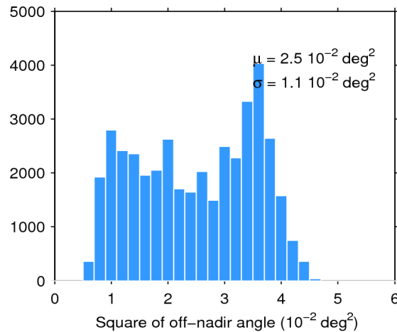
Figure 39. Histogram of flag-valid mispointing over oceans and lakes for 06/08/2019. The mean ( \mu ) and standard deviation ( \sigma ) are also shown. Note that values larger than 6 \cdot 10^{-2} \text{ deg}^2 are excluded from the histogram for the sake of readability but not from the computation of \mu and \sigma .
