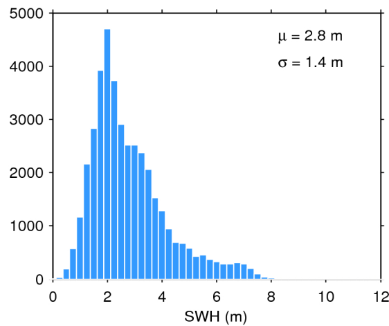
Figure 17. Histogram of flag-valid SWH over oceans and lakes for 06/08/2019. The mean ( \mu ) and standard deviation ( \sigma ) are also shown. Note that values larger than 12 m are excluded from the histogram for the sake of readability but not from the computation of \mu and \sigma .
