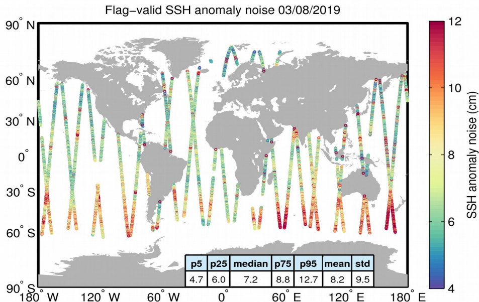
Figure 8. Geographical distribution of flag-valid 20-Hz SSH anomaly measurement noise over oceans and lakes for 03/08/2019. The statistical values shown in the table refer to the SSH anomaly noise and are calculated over all measurements shown in the figure.
