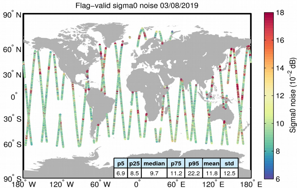
Figure 26. Geographical distribution of flag-valid 20-Hz sigma0 measurement noise over oceans and lakes for 03/08/2019. The statistical values shown in the table refer to the sigma0 noise and are calculated over all measurements shown in the figure.
