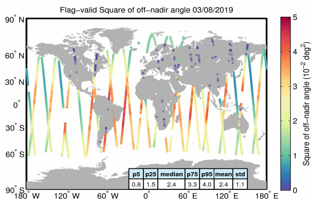
Figure 37. Geographical distribution of flag-valid mispointing data over oceans and lakes for 03/08/2019. The statistical values shown in the table refer to the mispointing in 10^{-2} \text{ deg}^2 and are calculated over all measurements shown in the figure.
