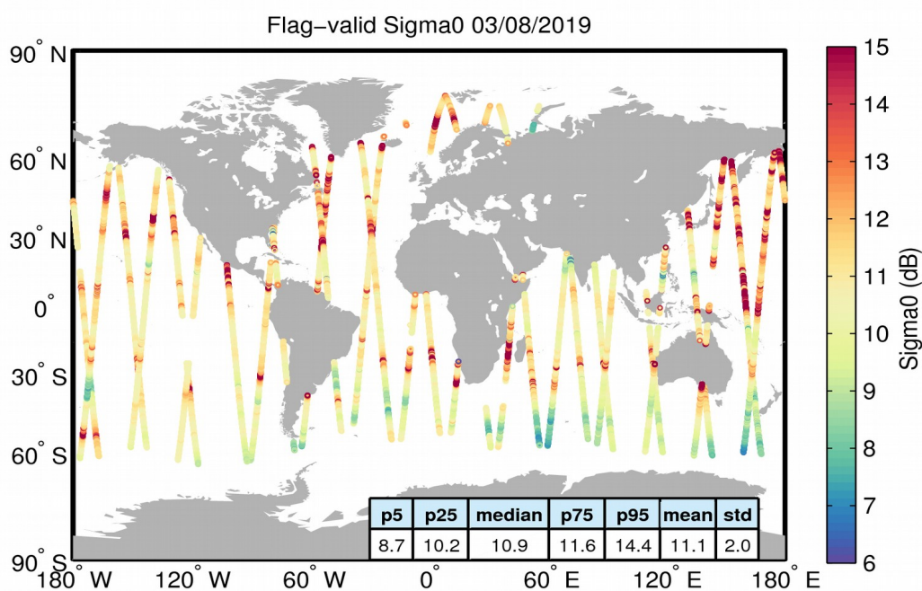
Figure 23. Geographical distribution of flag-valid sigma0 data over oceans and lakes for 03/08/2019. The statistical values shown in the table refer to the sigma0 in dB and are calculated over all measurements shown in the figure.
