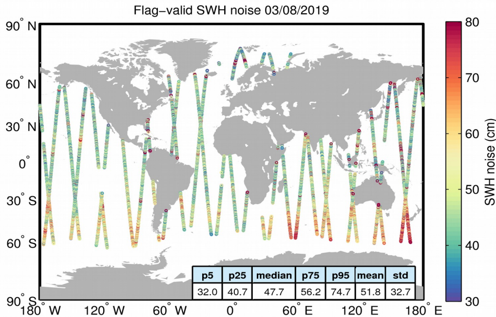
Figure 18. Geographical distribution of flag-valid 20-Hz SWH measurement noise over oceans and lakes for 03/08/2019. The statistical values shown in the table refer to the SWH noise and are calculated over all measurements shown in the figure.
