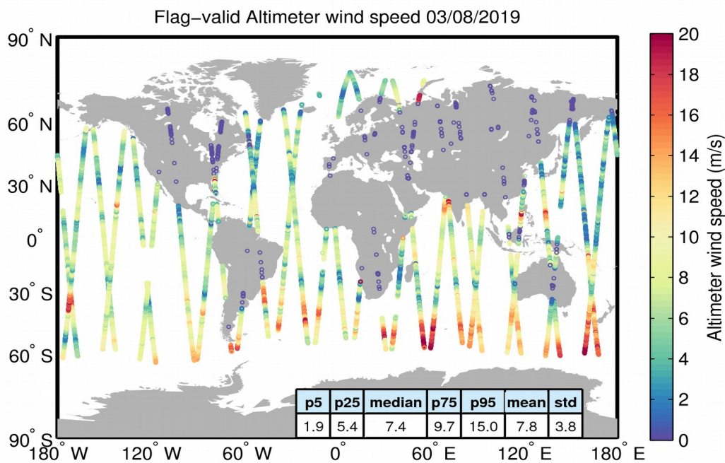
Figure 31. Geographical distribution of flag-valid wind data over oceans and lakes for 03/08/2019. The statistical values shown in the table refer to the wind in m/s and are calculated over all measurements shown in the figure.
