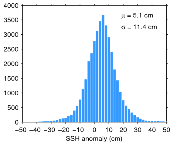
Figure 11. Histogram of science-valid SSH anomaly over oceans and lakes for 03/08/2019. The mean ( \mu ) and standard deviation ( \sigma ) are also shown. Note that values outside [-50 50] cm are excluded from the histogram for the sake of readability but not from the computation of \mu and \sigma .
