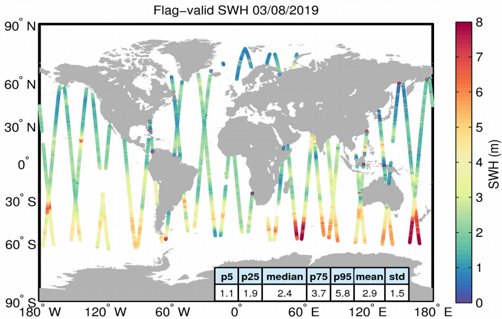
Figure 15. Geographical distribution of flag-valid SWH data over oceans and lakes for 03/08/2019. The statistical values shown in the table refer to the SWH in m and are calculated over all measurements shown in the figure.
