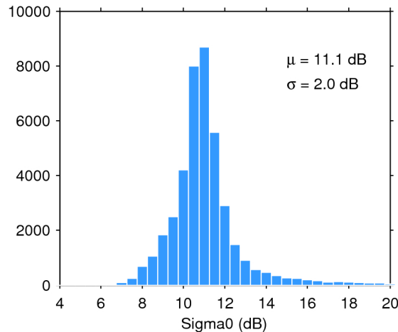
Figure 25. Histogram of flag-valid sigma0 over oceans and lakes for 03/08/2019. The mean ( \mu ) and standard deviation ( \sigma ) are also shown. Note that values outside [4 20] dB are excluded from the histogram for the sake of readability but not from the computation of \mu and \sigma .
