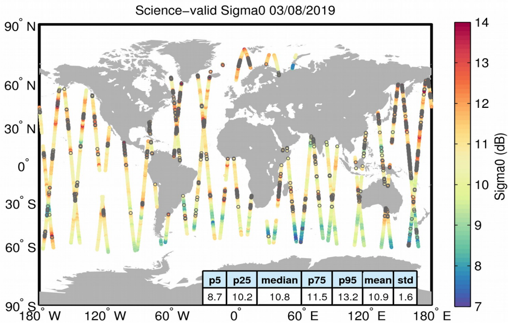
Figure 27. Geographical distribution of science-valid sigma0 data over oceans and lakes for 03/08/2019. The statistical values shown in the table refer to the sigma0 in dB and are calculated over all measurements shown in the figure. Gray circles denote records that have been rejected based on the editing criteria described in Table 4.
