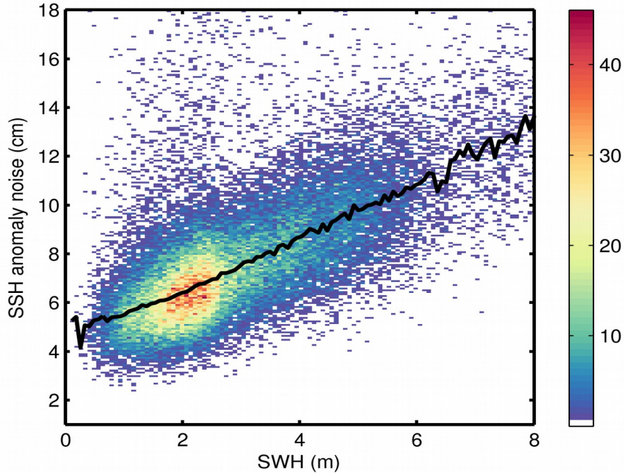
Figure 9. 2D histogram showing flag-valid SSH anomaly noise as a function of SWH for 03/08/2019. The black line denotes the median SSH anomaly noise as a function of SWH.
