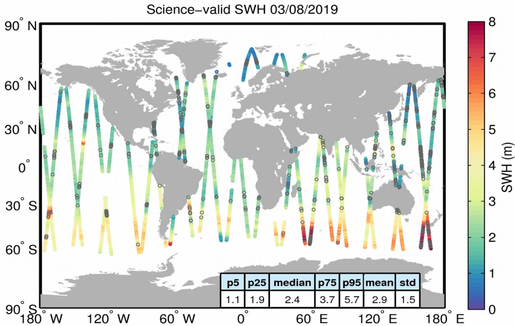
Figure 19. Geographical distribution of science-valid SWH data over oceans and lakes for 03/08/2019. The statistical values shown in the table refer to the SWH in m and are calculated over all measurements shown in the figure. Gray circles denote records that have been rejected based on the editing criteria described in Table 3.
