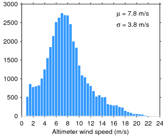
Figure 33. Histogram of flag-valid wind over oceans and lakes for 03/08/2019. The mean ( \mu ) and standard deviation ( \sigma ) are also shown. Note that values larger than 24 m/s are excluded from the histogram for the sake of readability but not from the computation of \mu and \sigma .
