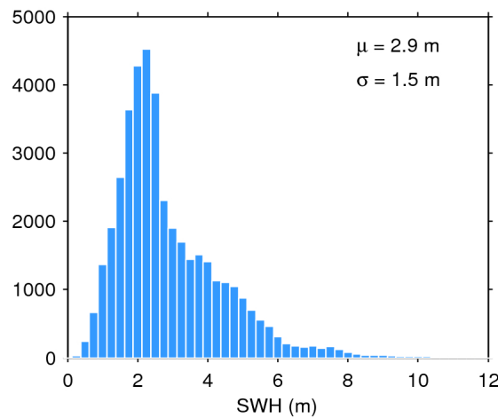
Figure 17. Histogram of flag-valid SWH over oceans and lakes for 03/08/2019. The mean ( \mu ) and standard deviation ( \sigma ) are also shown. Note that values larger than 12 m are excluded from the histogram for the sake of readability but not from the computation of \mu and \sigma .
