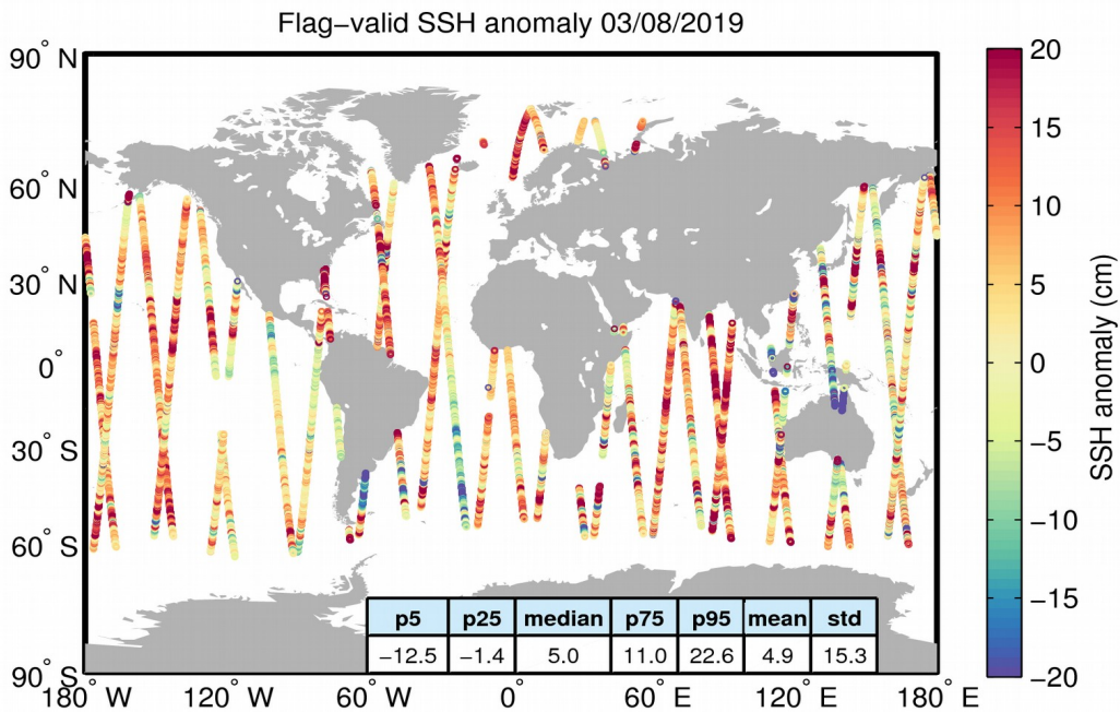
Figure 5. Geographical distribution of flag-valid 1-Hz SSH anomaly data over oceans and lakes for 03/08/2019. The statistical values shown in the table refer to the SSH anomaly in cm and are calculated over all measurements shown in the figure.
