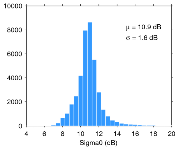
Figure 28. Histogram of science-valid sigma0 over oceans and lakes for 03/08/2019. The mean ( \mu ) and standard deviation ( \sigma ) are also shown. Note that values outside [4 20] dB are excluded from the histogram for the sake of readability but not from the computation of \mu and \sigma .
