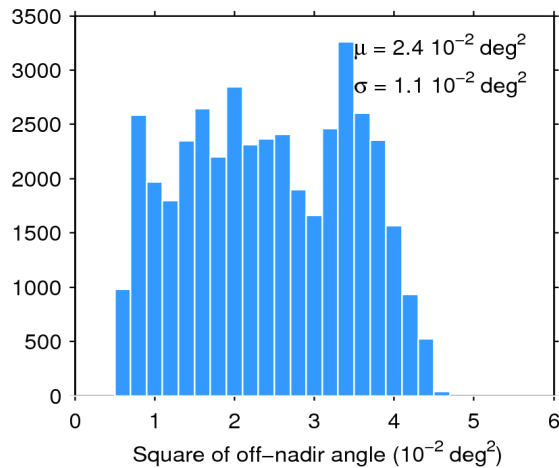
Figure 39. Histogram of flag-valid mispointing over oceans and lakes for 03/08/2019. The mean ( \mu ) and standard deviation ( \sigma ) are also shown. Note that values larger than 6 \cdot 10^{-2} \text{ deg}^2 are excluded from the histogram for the sake of readability but not from the computation of \mu and \sigma .
