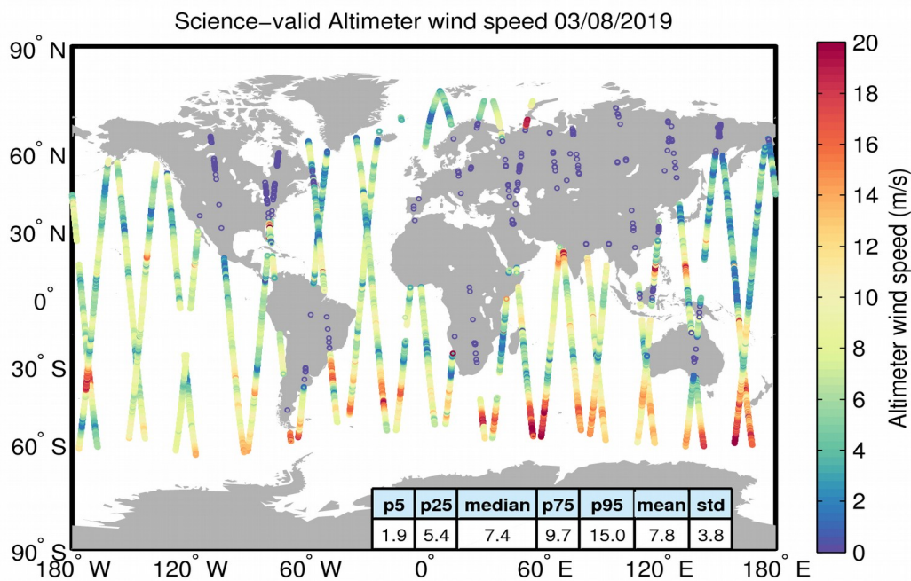
Figure 34. Geographical distribution of science-valid wind data over oceans and lakes for 03/08/2019. The statistical values shown in the table refer to the wind in m/s and are calculated over all measurements shown in the figure. Gray circles denote records that have been rejected based on the editing criteria described in Table 5.
