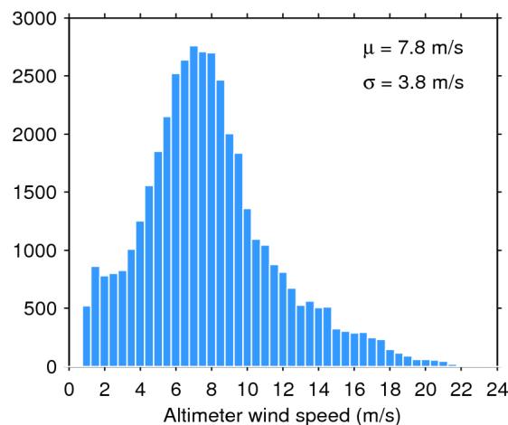
Figure 35. Histogram of science-valid wind over oceans and lakes for 03/08/2019. The mean ( \mu ) and standard deviation ( \sigma ) are also shown. Note that values larger than 24 m/s are excluded from the histogram for the sake of readability but not from the computation of \mu and \sigma .
