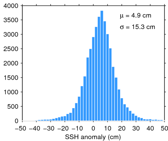
Figure 7. Histogram of flag-valid SSH anomaly over oceans and lakes for 03/08/2019. The mean ( \mu ) and standard deviation ( \sigma ) are also shown. Note that values outside [-50 50] cm are excluded from the histogram for the sake of readability but not from the computation of \mu and \sigma .
