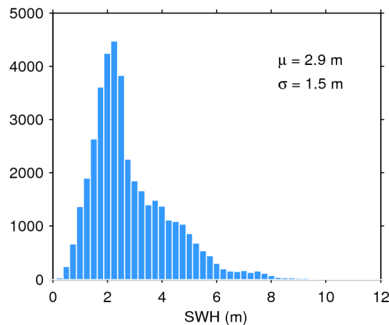
Figure 20. Histogram of science-valid SWH over oceans and lakes for 03/08/2019. The mean ( \mu ) and standard deviation ( \sigma ) are also shown. Note that values larger than 12 m are excluded from the histogram for the sake of readability but not from the computation of \mu and \sigma .
