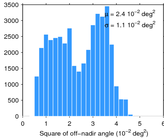
Figure 39. Histogram of flag-valid mispointing over oceans and lakes for 06/07/2019. The mean ( \mu ) and standard deviation ( \sigma ) are also shown. Note that values larger than 6 \cdot 10^{-2} \text{ deg}^2 are excluded from the histogram for the sake of readability but not from the computation of \mu and \sigma .
