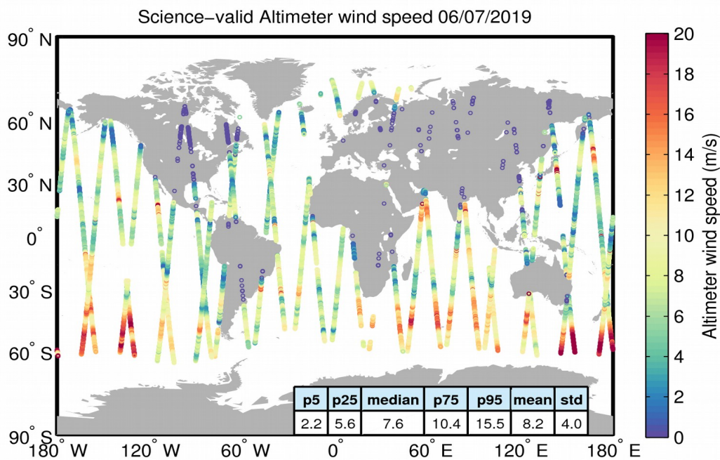
Figure 34. Geographical distribution of science-valid wind data over oceans and lakes for 06/07/2019. The statistical values shown in the table refer to the wind in m/s and are calculated over all measurements shown in the figure. Gray circles denote records that have been rejected based on the editing criteria described in Table 5.
