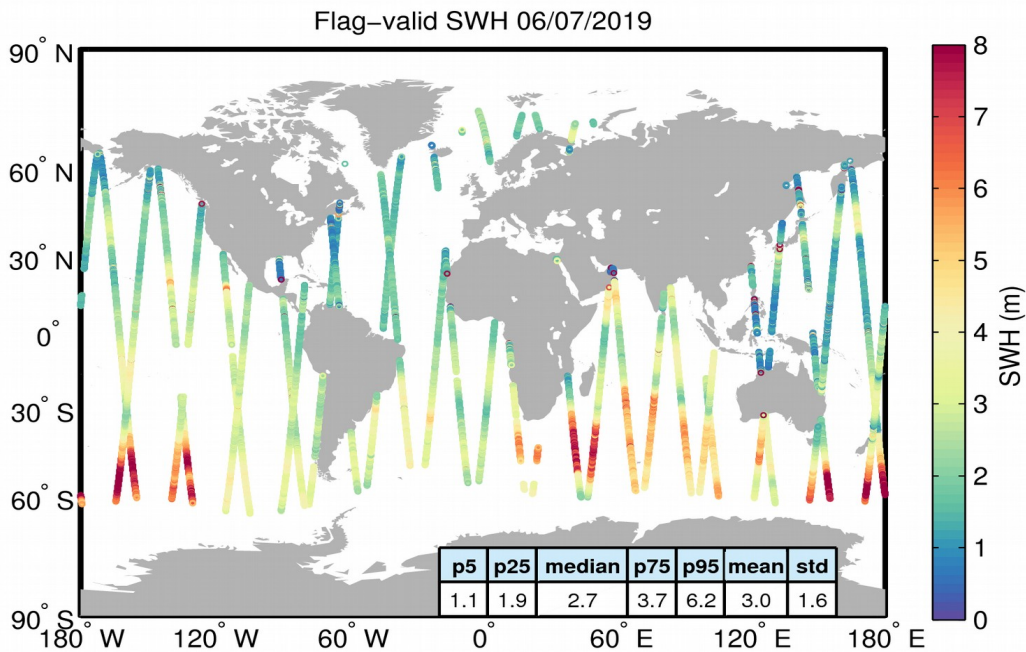
Figure 15. Geographical distribution of flag-valid SWH data over oceans and lakes for 06/07/2019. The statistical values shown in the table refer to the SWH in m and are calculated over all measurements shown in the figure.
