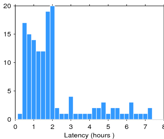
Figure 2. Histogram of the data latency for 06/07/2019. The y-axis denotes the number of files that are made available with a delay of x-hours with respect to the mean time of the records stored in the file.
