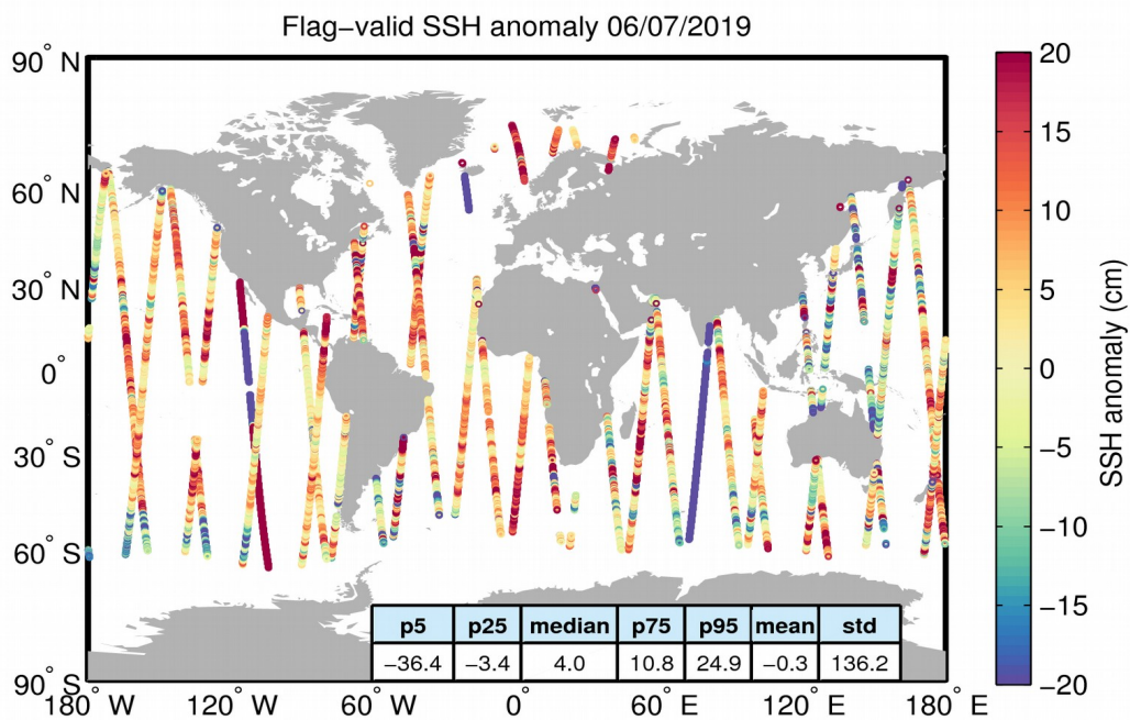
Figure 5. Geographical distribution of flag-valid 1-Hz SSH anomaly data over oceans and lakes for 06/07/2019. The statistical values shown in the table refer to the SSH anomaly in cm and are calculated over all measurements shown in the figure.
