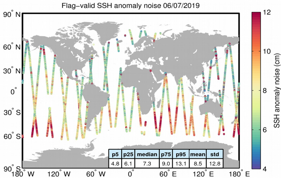
Figure 8. Geographical distribution of flag-valid 20-Hz SSH anomaly measurement noise over oceans and lakes for 06/07/2019. The statistical values shown in the table refer to the SSH anomaly noise and are calculated over all measurements shown in the figure.
