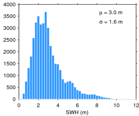
Figure 17. Histogram of flag-valid SWH over oceans and lakes for 06/07/2019. The mean ( \mu ) and standard deviation ( \sigma ) are also shown. Note that values larger than 12 m are excluded from the histogram for the sake of readability but not from the computation of \mu and \sigma .
