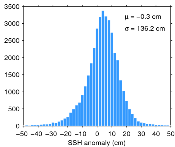
Figure 7. Histogram of flag-valid SSH anomaly over oceans and lakes for 06/07/2019. The mean ( \mu ) and standard deviation ( \sigma ) are also shown. Note that values outside [-50 50] cm are excluded from the histogram for the sake of readability but not from the computation of \mu and \sigma .
