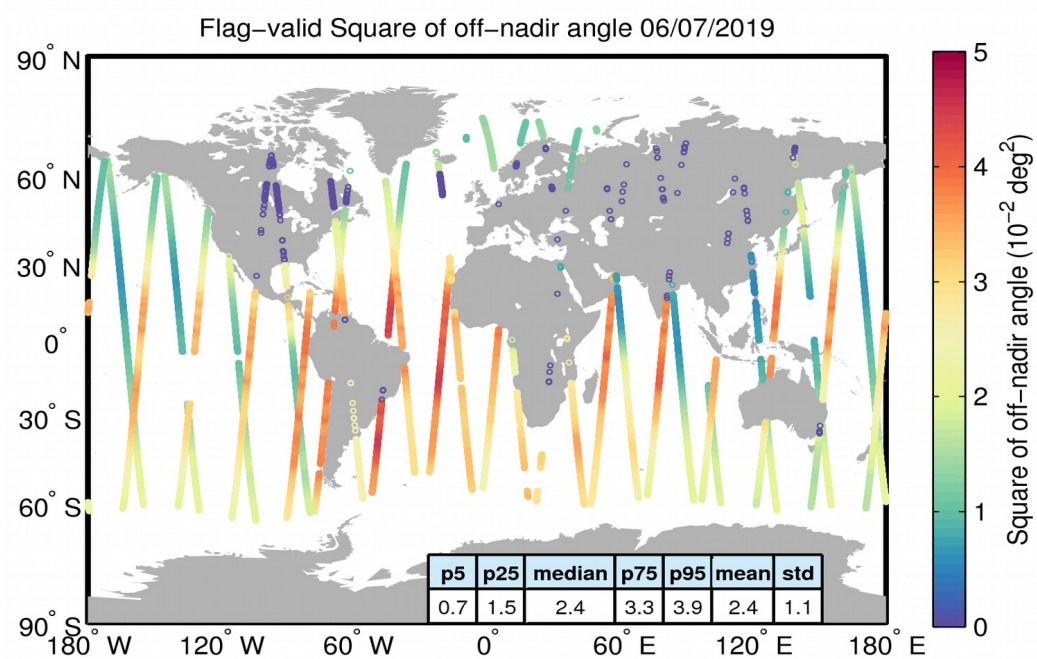
Figure 37. Geographical distribution of flag-valid mispointing data over oceans and lakes for 06/07/2019. The statistical values shown in the table refer to the mispointing in 10^{-2} deg 2 and are calculated over all measurements shown in the figure.
