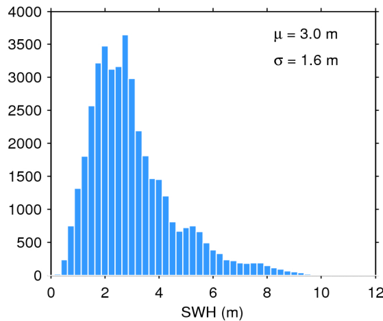
Figure 20. Histogram of science-valid SWH over oceans and lakes for 06/07/2019. The mean ( \mu ) and standard deviation ( \sigma ) are also shown. Note that values larger than 12 m are excluded from the histogram for the sake of readability but not from the computation of \mu and \sigma .
