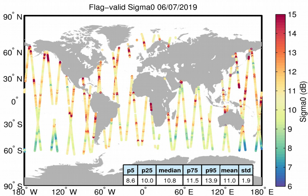
Figure 23. Geographical distribution of flag-valid sigma0 data over oceans and lakes for 06/07/2019. The statistical values shown in the table refer to the sigma0 in dB and are calculated over all measurements shown in the figure.
