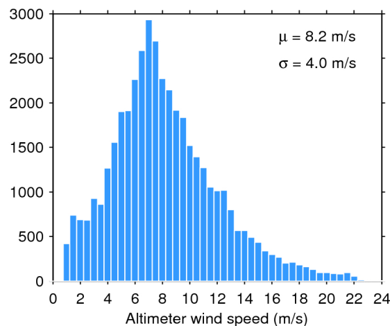
Figure 35. Histogram of science-valid wind over oceans and lakes for 06/07/2019. The mean ( \mu ) and standard deviation ( \sigma ) are also shown. Note that values larger than 24 m/s are excluded from the histogram for the sake of readability but not from the computation of \mu and \sigma .
