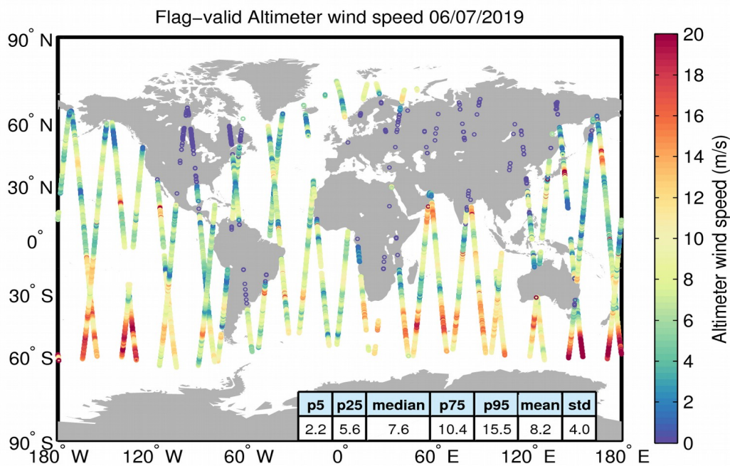
Figure 31. Geographical distribution of flag-valid wind data over oceans and lakes for 06/07/2019. The statistical values shown in the table refer to the wind in m/s and are calculated over all measurements shown in the figure.
