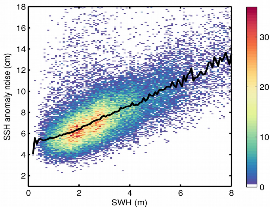
Figure 9. 2D histogram showing flag-valid SSH anomaly noise as a function of SWH for 06/07/2019. The black line denotes the median SSH anomaly noise as a function of SWH.
