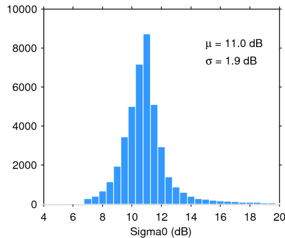
Figure 25. Histogram of flag-valid sigma0 over oceans and lakes for 06/07/2019. The mean ( \mu ) and standard deviation ( \sigma ) are also shown. Note that values outside [4 20] dB are excluded from the histogram for the sake of readability but not from the computation of \mu and \sigma .
