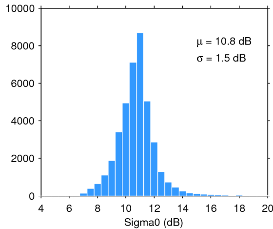
Figure 28. Histogram of science-valid sigma0 over oceans and lakes for 06/07/2019. The mean ( \mu ) and standard deviation ( \sigma ) are also shown. Note that values outside [4 20] dB are excluded from the histogram for the sake of readability but not from the computation of \mu and \sigma .
