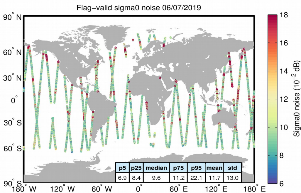
Figure 26. Geographical distribution of flag-valid 20-Hz sigma0 measurement noise over oceans and lakes for 06/07/2019. The statistical values shown in the table refer to the sigma0 noise and are calculated over all measurements shown in the figure.
