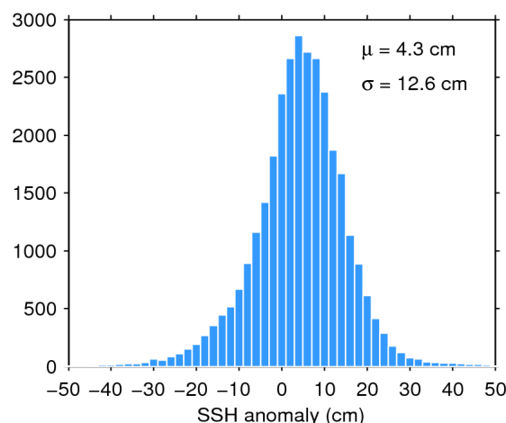
Figure 11. Histogram of science-valid SSH anomaly over oceans and lakes for 06/07/2019. The mean ( \mu ) and standard deviation ( \sigma ) are also shown. Note that values outside [-50 50] cm are excluded from the histogram for the sake of readability but not from the computation of \mu and \sigma .
