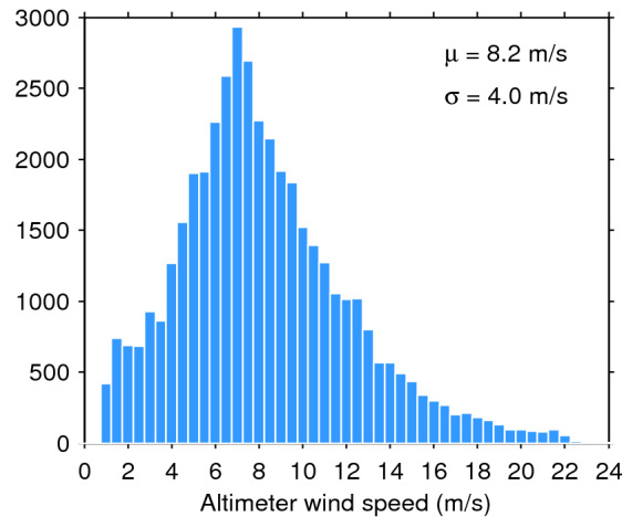
Figure 33. Histogram of flag-valid wind over oceans and lakes for 06/07/2019. The mean ( \mu ) and standard deviation ( \sigma ) are also shown. Note that values larger than 24 m/s are excluded from the histogram for the sake of readability but not from the computation of \mu and \sigma .
