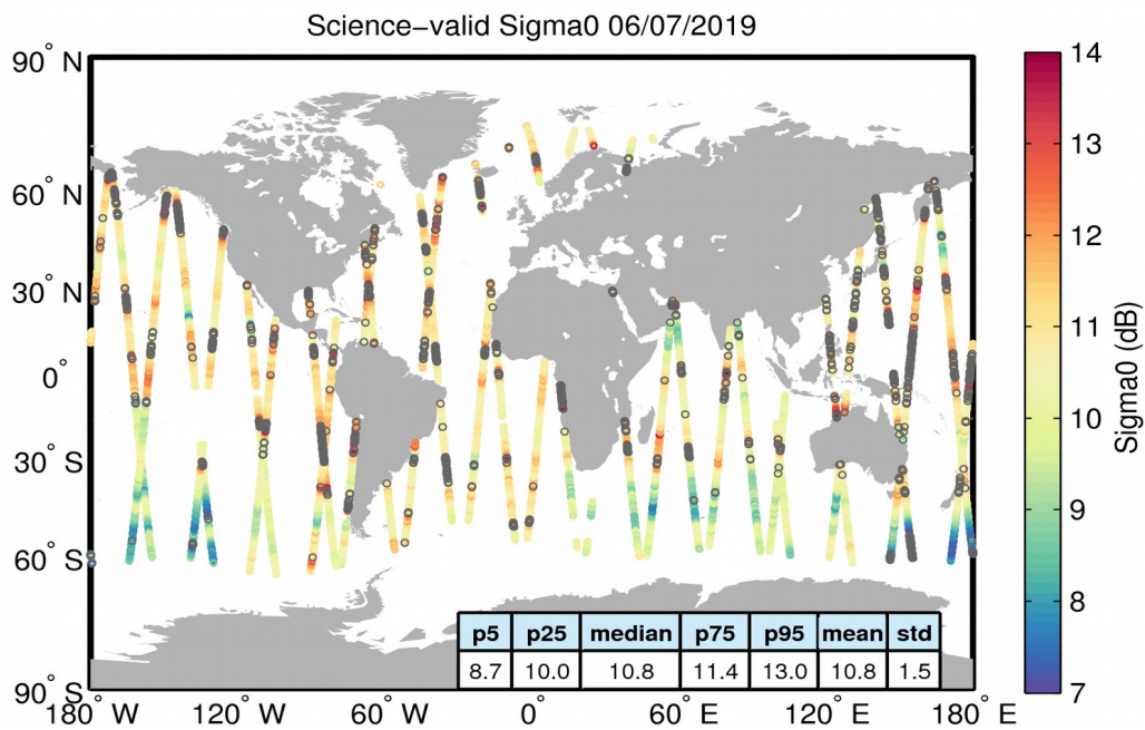
Figure 27. Geographical distribution of science-valid sigma0 data over oceans and lakes for 06/07/2019. The statistical values shown in the table refer to the sigma0 in dB and are calculated over all measurements shown in the figure. Gray circles denote records that have been rejected based on the editing criteria described in Table 4.
