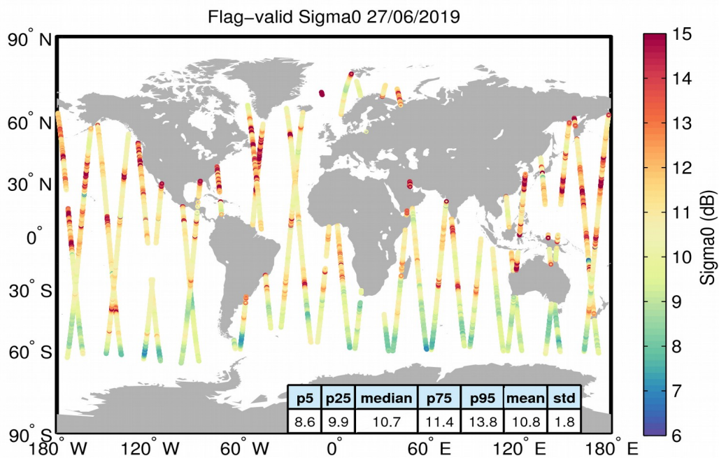
Figure 23. Geographical distribution of flag-valid sigma0 data over oceans and lakes for 27/06/2019. The statistical values shown in the table refer to the sigma0 in dB and are calculated over all measurements shown in the figure.
