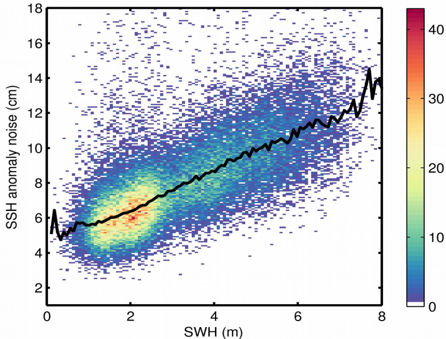
Figure 9. 2D histogram showing flag-valid SSH anomaly noise as a function of SWH for 27/06/2019. The black line denotes the median SSH anomaly noise as a function of SWH.
