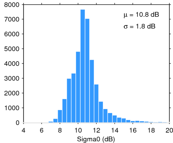
Figure 25. Histogram of flag-valid sigma0 over oceans and lakes for 27/06/2019. The mean ( \mu ) and standard deviation ( \sigma ) are also shown. Note that values outside [4 20] dB are excluded from the histogram for the sake of readability but not from the computation of \mu and \sigma .
