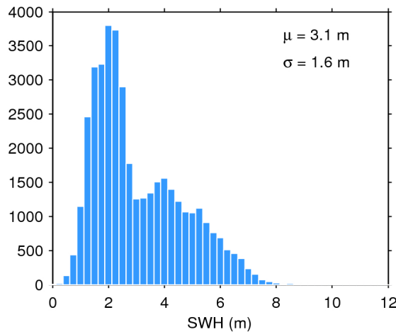
Figure 20. Histogram of science-valid SWH over oceans and lakes for 27/06/2019. The mean ( \mu ) and standard deviation ( \sigma ) are also shown. Note that values larger than 12 m are excluded from the histogram for the sake of readability but not from the computation of \mu and \sigma .
