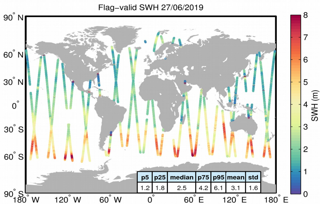
Figure 15. Geographical distribution of flag-valid SWH data over oceans and lakes for 27/06/2019. The statistical values shown in the table refer to the SWH in m and are calculated over all measurements shown in the figure.
