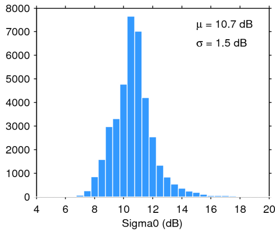
Figure 28. Histogram of science-valid sigma0 over oceans and lakes for 27/06/2019. The mean ( \mu ) and standard deviation ( \sigma ) are also shown. Note that values outside [4 20] dB are excluded from the histogram for the sake of readability but not from the computation of \mu and \sigma .
