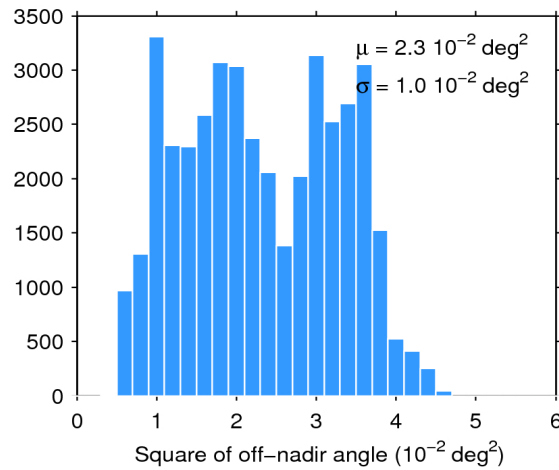
Figure 39. Histogram of flag-valid mispointing over oceans and lakes for 27/06/2019. The mean ( \mu ) and standard deviation ( \sigma ) are also shown. Note that values larger than 6 \cdot 10^{-2} \text{ deg}^2 are excluded from the histogram for the sake of readability but not from the computation of \mu and \sigma .
