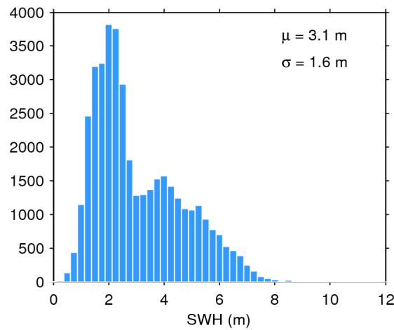
Figure 17. Histogram of flag-valid SWH over oceans and lakes for 27/06/2019. The mean ( \mu ) and standard deviation ( \sigma ) are also shown. Note that values larger than 12 m are excluded from the histogram for the sake of readability but not from the computation of \mu and \sigma .
