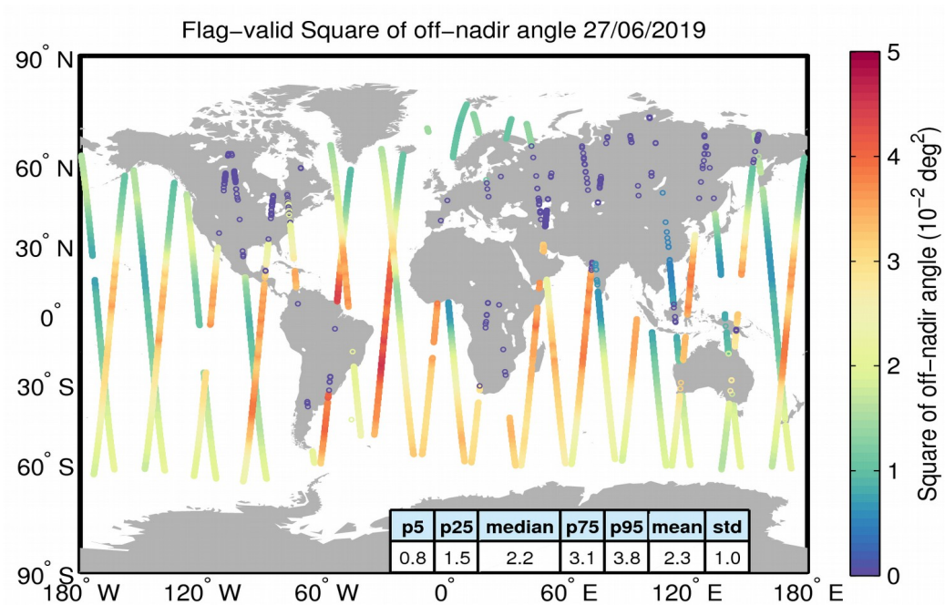
Figure 37. Geographical distribution of flag-valid mispointing data over oceans and lakes for 27/06/2019. The statistical values shown in the table refer to the mispointing in 10^{-2} \text{ deg}^2 and are calculated over all measurements shown in the figure.
