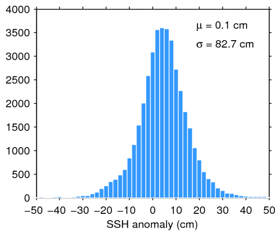
Figure 7. Histogram of flag-valid SSH anomaly over oceans and lakes for 27/06/2019. The mean ( \mu ) and standard deviation ( \sigma ) are also shown. Note that values outside [-50 50] cm are excluded from the histogram for the sake of readability but not from the computation of \mu and \sigma .
