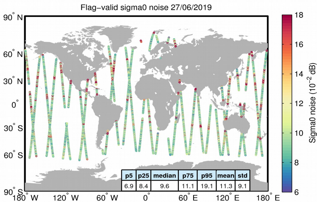
Figure 26. Geographical distribution of flag-valid 20-Hz sigma0 measurement noise over oceans and lakes for 27/06/2019. The statistical values shown in the table refer to the sigma0 noise and are calculated over all measurements shown in the figure.
