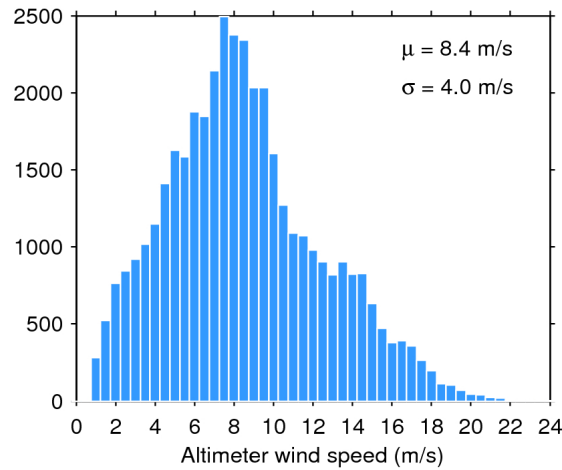
Figure 33. Histogram of flag-valid wind over oceans and lakes for 27/06/2019. The mean ( \mu ) and standard deviation ( \sigma ) are also shown. Note that values larger than 24 m/s are excluded from the histogram for the sake of readability but not from the computation of \mu and \sigma .
