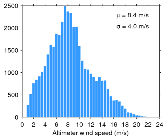
Figure 35. Histogram of science-valid wind over oceans and lakes for 27/06/2019. The mean ( \mu ) and standard deviation ( \sigma ) are also shown. Note that values larger than 24 m/s are excluded from the histogram for the sake of readability but not from the computation of \mu and \sigma .
