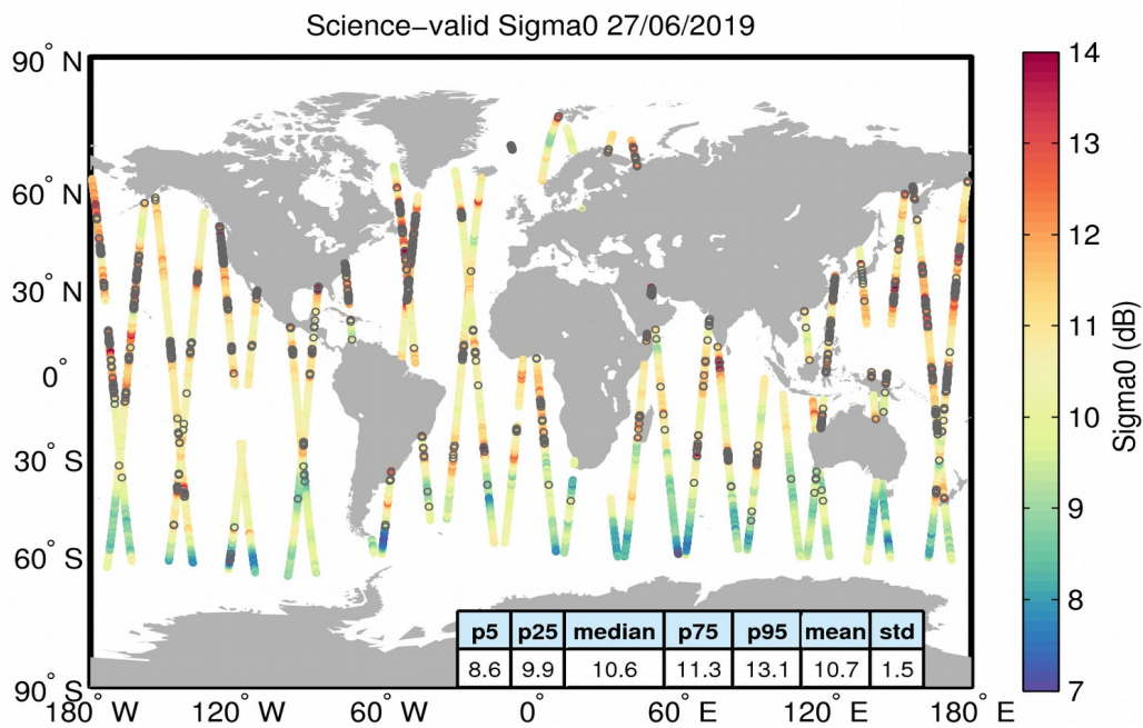
Figure 27. Geographical distribution of science-valid sigma0 data over oceans and lakes for 27/06/2019. The statistical values shown in the table refer to the sigma0 in dB and are calculated over all measurements shown in the figure. Gray circles denote records that have been rejected based on the editing criteria described in Table 4.
