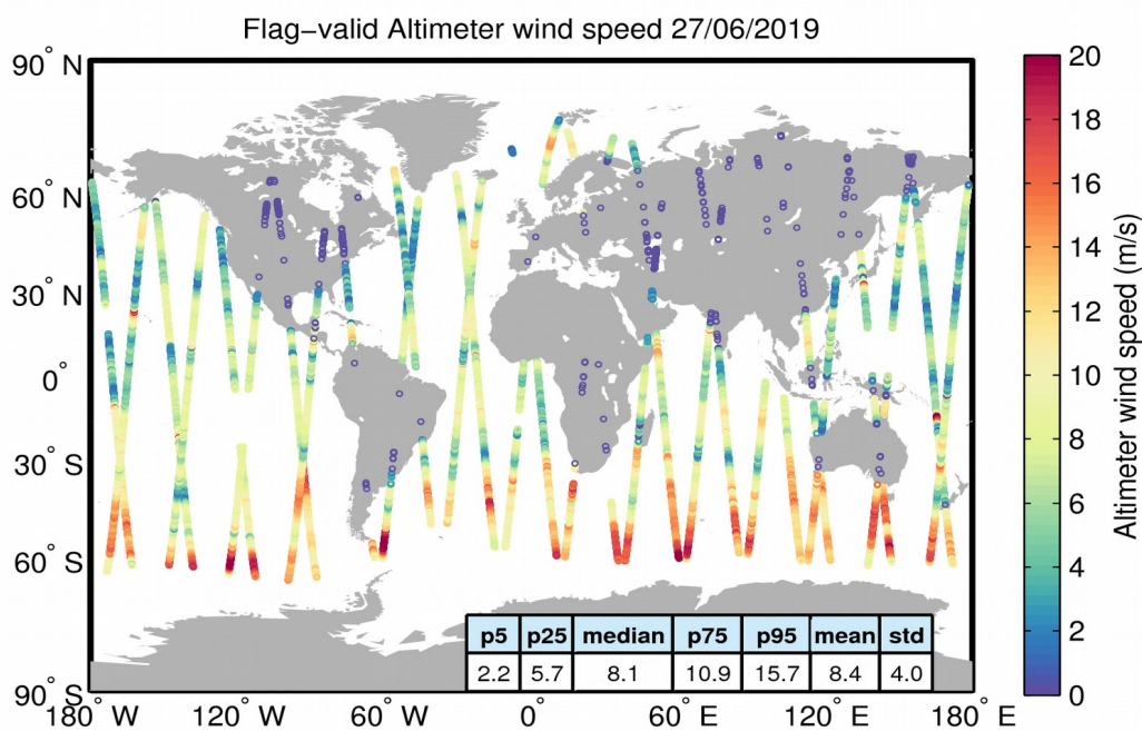
Figure 31. Geographical distribution of flag-valid wind data over oceans and lakes for 27/06/2019. The statistical values shown in the table refer to the wind in m/s and are calculated over all measurements shown in the figure.
