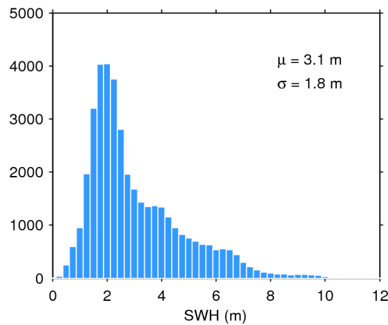
Figure 17. Histogram of flag-valid SWH over oceans and lakes for 25/06/2019. The mean ( \mu ) and standard deviation ( \sigma ) are also shown. Note that values larger than 12 m are excluded from the histogram for the sake of readability but not from the computation of \mu and \sigma .
