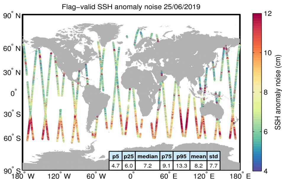
Figure 8. Geographical distribution of flag-valid 20-Hz SSH anomaly measurement noise over oceans and lakes for 25/06/2019. The statistical values shown in the table refer to the SSH anomaly noise and are calculated over all measurements shown in the figure.
