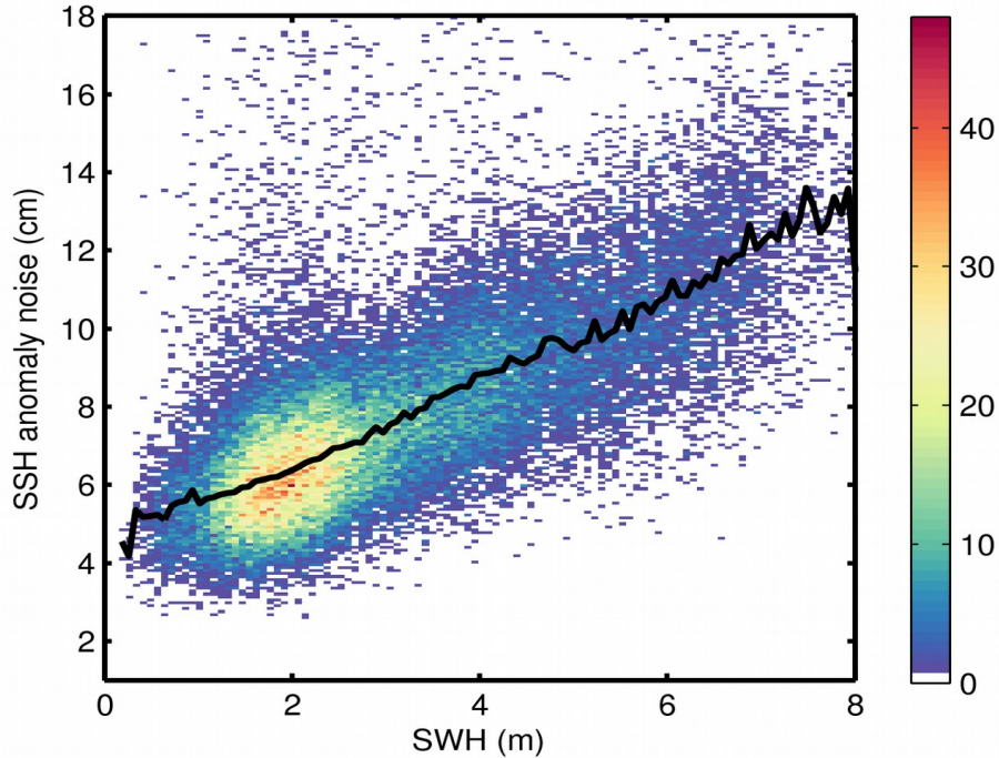
Figure 9. 2D histogram showing flag-valid SSH anomaly noise as a function of SWH for 25/06/2019. The black line denotes the median SSH anomaly noise as a function of SWH.
