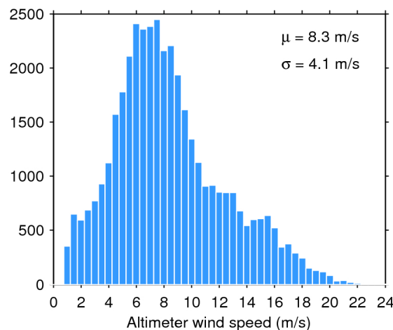
Figure 35. Histogram of science-valid wind over oceans and lakes for 25/06/2019. The mean ( \mu ) and standard deviation ( \sigma ) are also shown. Note that values larger than 24 m/s are excluded from the histogram for the sake of readability but not from the computation of \mu and \sigma .
