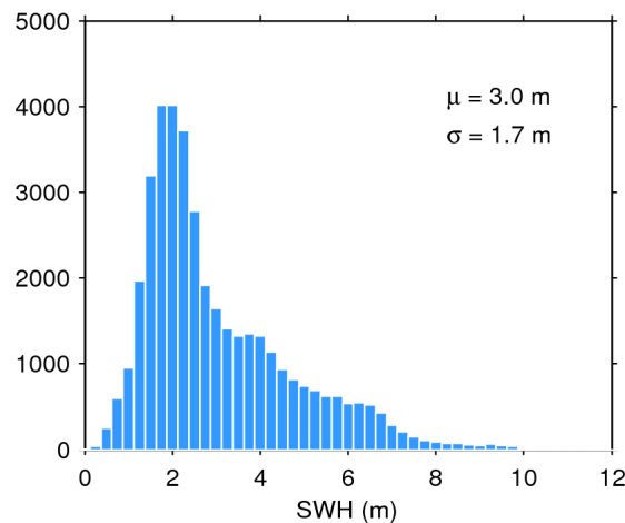
Figure 20. Histogram of science-valid SWH over oceans and lakes for 25/06/2019. The mean ( \mu ) and standard deviation ( \sigma ) are also shown. Note that values larger than 12 m are excluded from the histogram for the sake of readability but not from the computation of \mu and \sigma .
