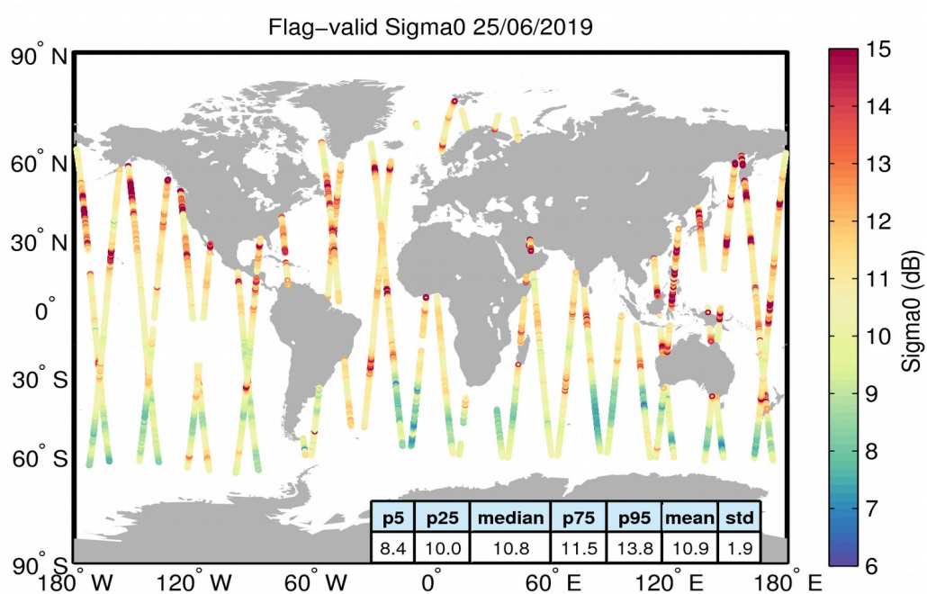
Figure 23. Geographical distribution of flag-valid sigma0 data over oceans and lakes for 25/06/2019. The statistical values shown in the table refer to the sigma0 in dB and are calculated over all measurements shown in the figure.
