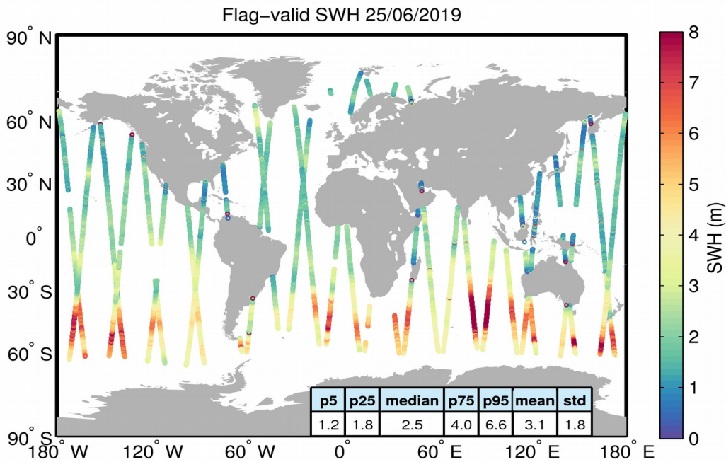
Figure 15. Geographical distribution of flag-valid SWH data over oceans and lakes for 25/06/2019. The statistical values shown in the table refer to the SWH in m and are calculated over all measurements shown in the figure.
