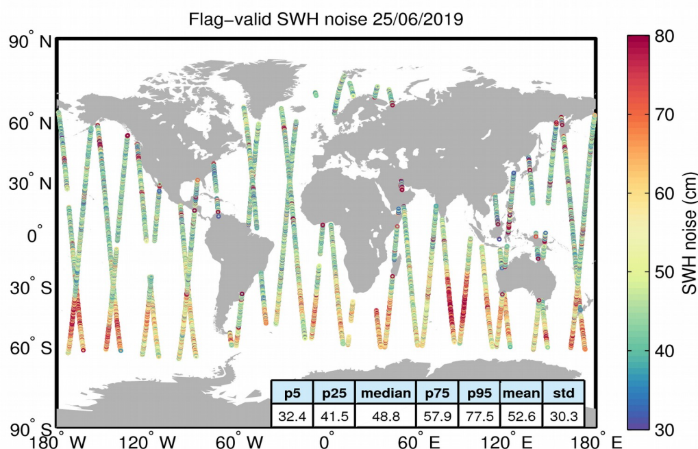
Figure 18. Geographical distribution of flag-valid 20-Hz SWH measurement noise over oceans and lakes for 25/06/2019. The statistical values shown in the table refer to the SWH noise and are calculated over all measurements shown in the figure.
