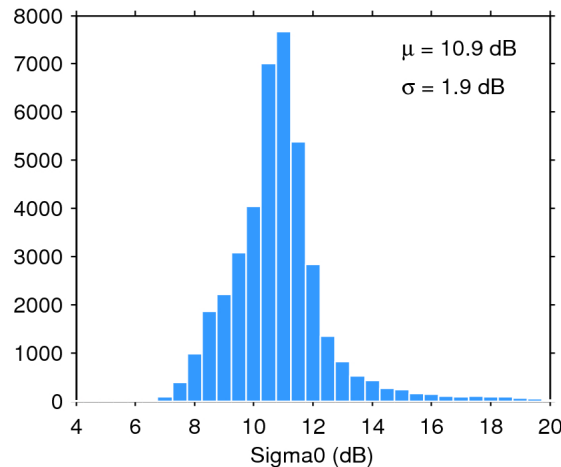
Figure 25. Histogram of flag-valid sigma0 over oceans and lakes for 25/06/2019. The mean ( \mu ) and standard deviation ( \sigma ) are also shown. Note that values outside [4 20] dB are excluded from the histogram for the sake of readability but not from the computation of \mu and \sigma .
