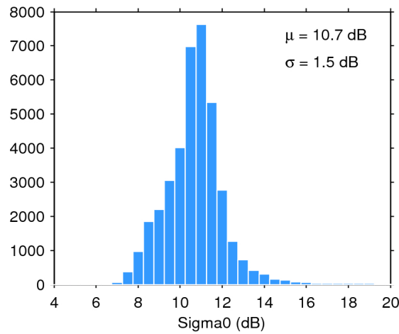
Figure 28. Histogram of science-valid sigma0 over oceans and lakes for 25/06/2019. The mean ( \mu ) and standard deviation ( \sigma ) are also shown. Note that values outside [4 20] dB are excluded from the histogram for the sake of readability but not from the computation of \mu and \sigma .
