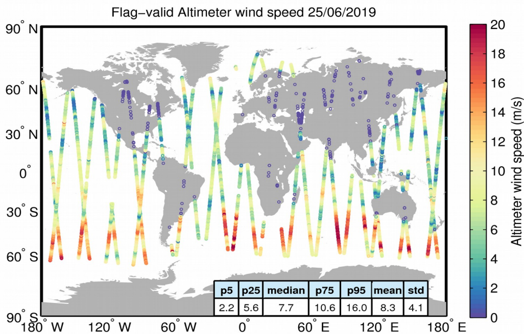
Figure 31. Geographical distribution of flag-valid wind data over oceans and lakes for 25/06/2019. The statistical values shown in the table refer to the wind in m/s and are calculated over all measurements shown in the figure.
