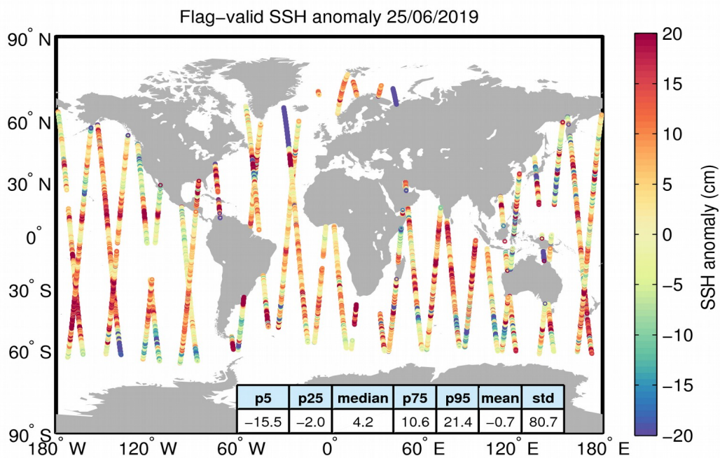
Figure 5. Geographical distribution of flag-valid 1-Hz SSH anomaly data over oceans and lakes for 25/06/2019. The statistical values shown in the table refer to the SSH anomaly in cm and are calculated over all measurements shown in the figure.
