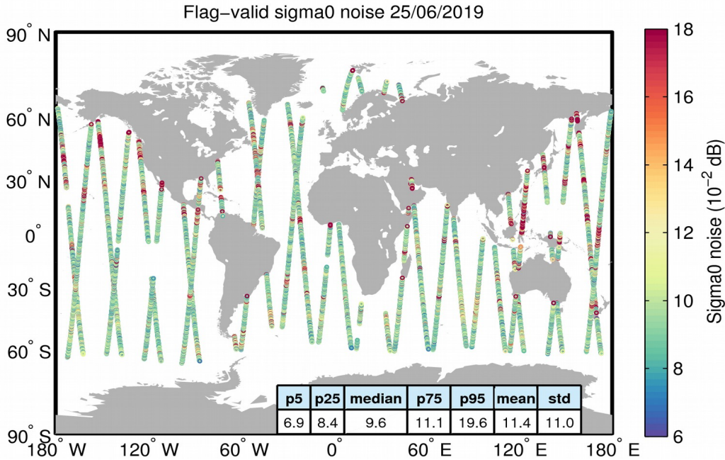
Figure 26. Geographical distribution of flag-valid 20-Hz sigma0 measurement noise over oceans and lakes for 25/06/2019. The statistical values shown in the table refer to the sigma0 noise and are calculated over all measurements shown in the figure.
