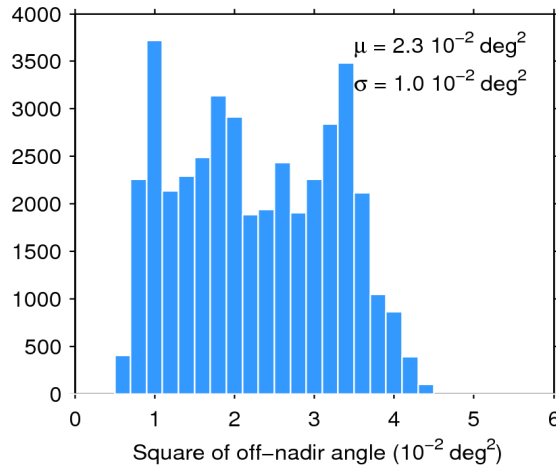
Figure 39. Histogram of flag-valid mispointing over oceans and lakes for 25/06/2019. The mean ( \mu ) and standard deviation ( \sigma ) are also shown. Note that values larger than 6 \cdot 10^{-2} \text{ deg}^2 are excluded from the histogram for the sake of readability but not from the computation of \mu and \sigma .
