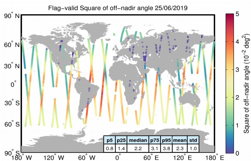
Figure 37. Geographical distribution of flag-valid mispointing data over oceans and lakes for 25/06/2019. The statistical values shown in the table refer to the mispointing in 10^{-2} \text{ deg}^2 and are calculated over all measurements shown in the figure.
