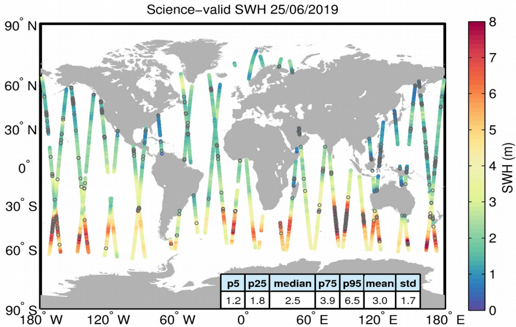
Figure 19. Geographical distribution of science-valid SWH data over oceans and lakes for 25/06/2019. The statistical values shown in the table refer to the SWH in m and are calculated over all measurements shown in the figure. Gray circles denote records that have been rejected based on the editing criteria described in Table 3.
