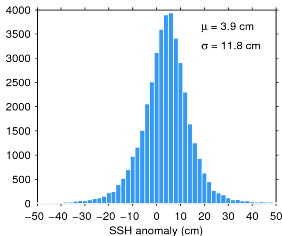
Figure 11. Histogram of science-valid SSH anomaly over oceans and lakes for 24/06/2019. The mean ( \mu ) and standard deviation ( \sigma ) are also shown. Note that values outside [-50 50] cm are excluded from the histogram for the sake of readability but not from the computation of \mu and \sigma .
