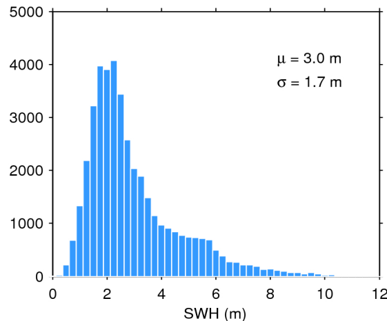
Figure 20. Histogram of science-valid SWH over oceans and lakes for 24/06/2019. The mean ( \mu ) and standard deviation ( \sigma ) are also shown. Note that values larger than 12 m are excluded from the histogram for the sake of readability but not from the computation of \mu and \sigma .
