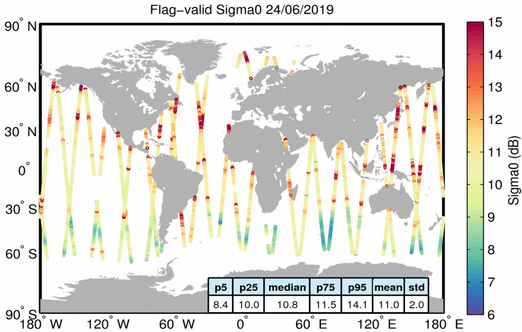
Figure 23. Geographical distribution of flag-valid sigma0 data over oceans and lakes for 24/06/2019. The statistical values shown in the table refer to the sigma0 in dB and are calculated over all measurements shown in the figure.
