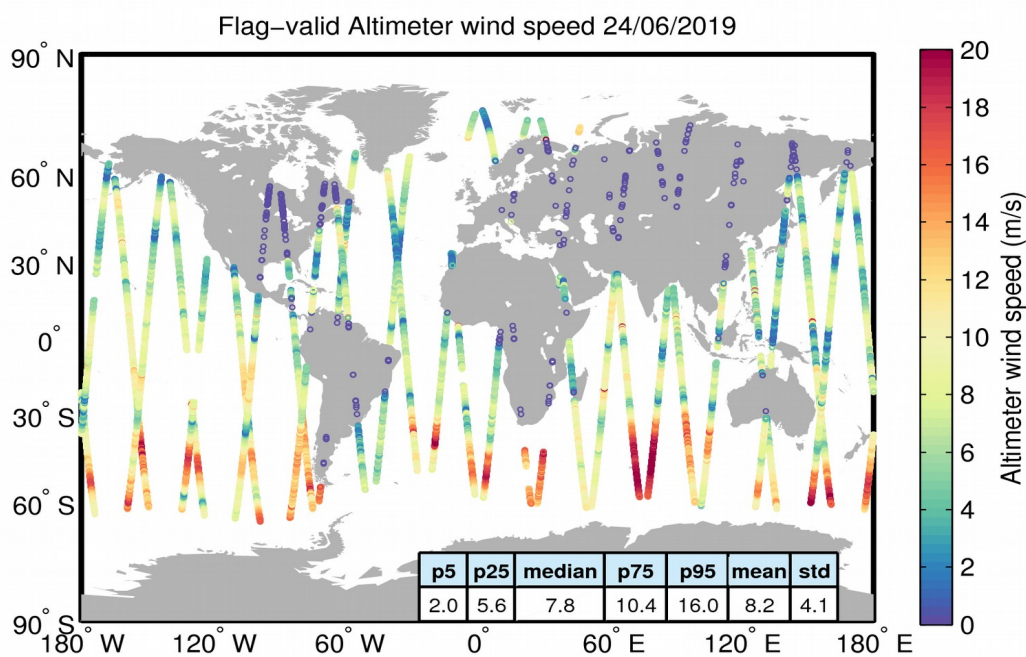
Figure 31. Geographical distribution of flag-valid wind data over oceans and lakes for 24/06/2019. The statistical values shown in the table refer to the wind in m/s and are calculated over all measurements shown in the figure.
