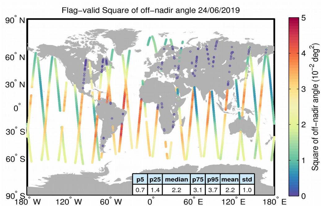
Figure 37. Geographical distribution of flag-valid mispointing data over oceans and lakes for 24/06/2019. The statistical values shown in the table refer to the mispointing in 10^{-2} \text{ deg}^2 and are calculated over all measurements shown in the figure.
