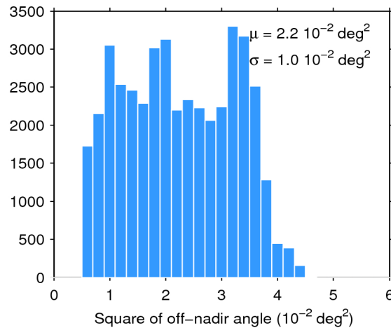
Figure 39. Histogram of flag-valid mispointing over oceans and lakes for 24/06/2019. The mean ( \mu ) and standard deviation ( \sigma ) are also shown. Note that values larger than 6 \cdot 10^{-2} \text{ deg}^2 are excluded from the histogram for the sake of readability but not from the computation of \mu and \sigma .
