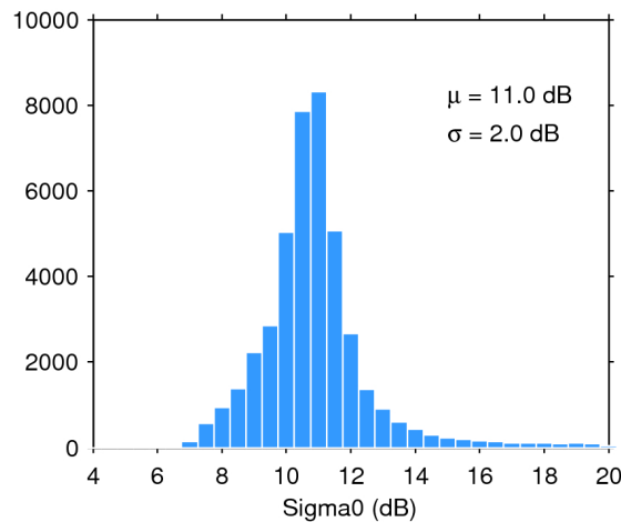
Figure 25. Histogram of flag-valid sigma0 over oceans and lakes for 24/06/2019. The mean ( \mu ) and standard deviation ( \sigma ) are also shown. Note that values outside [4 20] dB are excluded from the histogram for the sake of readability but not from the computation of \mu and \sigma .
