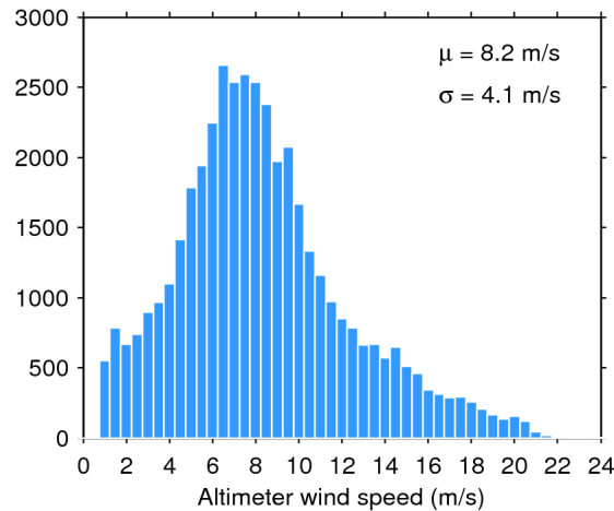
Figure 33. Histogram of flag-valid wind over oceans and lakes for 24/06/2019. The mean ( \mu ) and standard deviation ( \sigma ) are also shown. Note that values larger than 24 m/s are excluded from the histogram for the sake of readability but not from the computation of \mu and \sigma .
