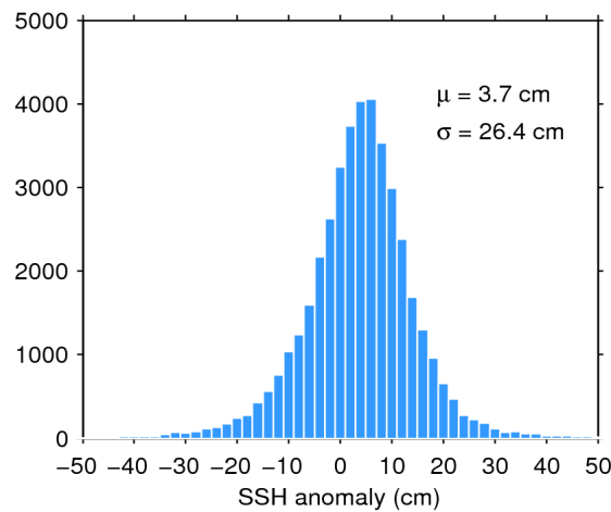
Figure 7. Histogram of flag-valid SSH anomaly over oceans and lakes for 24/06/2019. The mean ( \mu ) and standard deviation ( \sigma ) are also shown. Note that values outside [-50\ 50] cm are excluded from the histogram for the sake of readability but not from the computation of \mu and \sigma .
