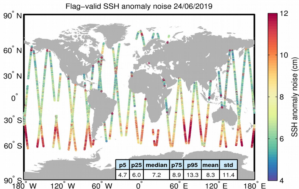
Figure 8. Geographical distribution of flag-valid 20-Hz SSH anomaly measurement noise over oceans and lakes for 24/06/2019. The statistical values shown in the table refer to the SSH anomaly noise and are calculated over all measurements shown in the figure.
