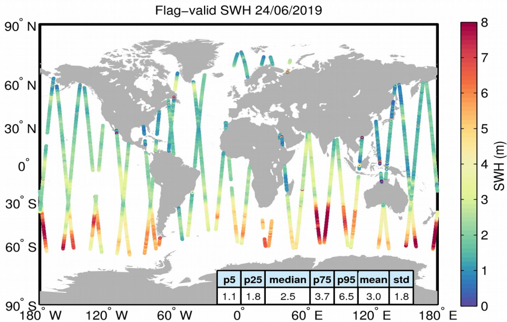
Figure 15. Geographical distribution of flag-valid SWH data over oceans and lakes for 24/06/2019. The statistical values shown in the table refer to the SWH in m and are calculated over all measurements shown in the figure.
