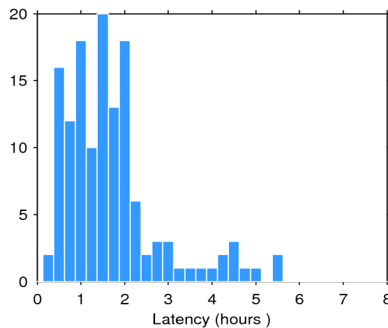
Figure 2. Histogram of the data latency for 24/06/2019. The y-axis denotes the number of files that are made available with a delay of x-hours with respect to the mean time of the records stored in the file.
