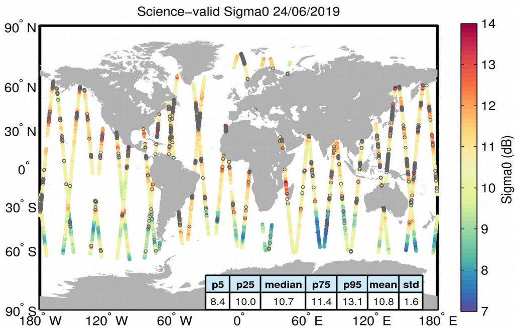
Figure 27. Geographical distribution of science-valid sigma0 data over oceans and lakes for 24/06/2019. The statistical values shown in the table refer to the sigma0 in dB and are calculated over all measurements shown in the figure. Gray circles denote records that have been rejected based on the editing criteria described in Table 4.
