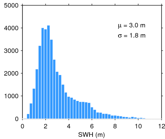
Figure 17. Histogram of flag-valid SWH over oceans and lakes for 24/06/2019. The mean ( \mu ) and standard deviation ( \sigma ) are also shown. Note that values larger than 12 m are excluded from the histogram for the sake of readability but not from the computation of \mu and \sigma .
