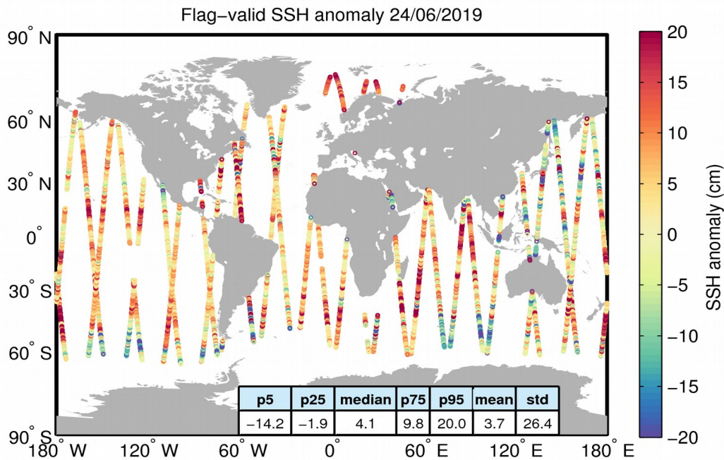
Figure 5. Geographical distribution of flag-valid 1-Hz SSH anomaly data over oceans and lakes for 24/06/2019. The statistical values shown in the table refer to the SSH anomaly in cm and are calculated over all measurements shown in the figure.
