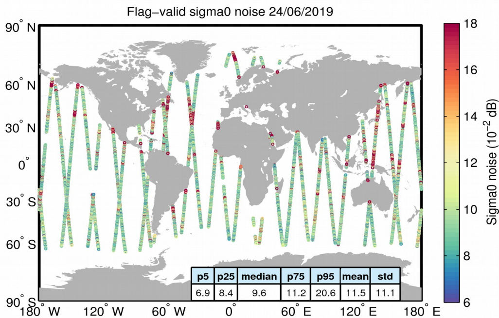
Figure 26. Geographical distribution of flag-valid 20-Hz sigma0 measurement noise over oceans and lakes for 24/06/2019. The statistical values shown in the table refer to the sigma0 noise and are calculated over all measurements shown in the figure.
