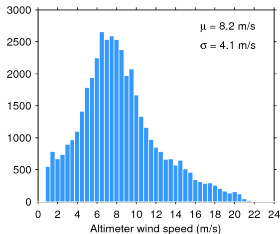
Figure 35. Histogram of science-valid wind over oceans and lakes for 24/06/2019. The mean ( \mu ) and standard deviation ( \sigma ) are also shown. Note that values larger than 24 m/s are excluded from the histogram for the sake of readability but not from the computation of \mu and \sigma .
