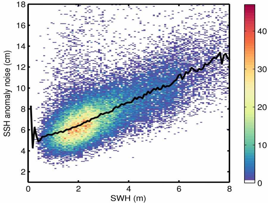
Figure 9. 2D histogram showing flag-valid SSH anomaly noise as a function of SWH for 24/06/2019. The black line denotes the median SSH anomaly noise as a function of SWH.
