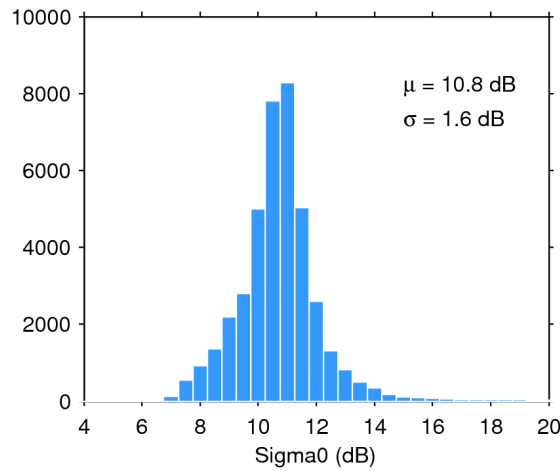
Figure 28. Histogram of science-valid sigma0 over oceans and lakes for 24/06/2019. The mean ( \mu ) and standard deviation ( \sigma ) are also shown. Note that values outside [4 20] dB are excluded from the histogram for the sake of readability but not from the computation of \mu and \sigma .
