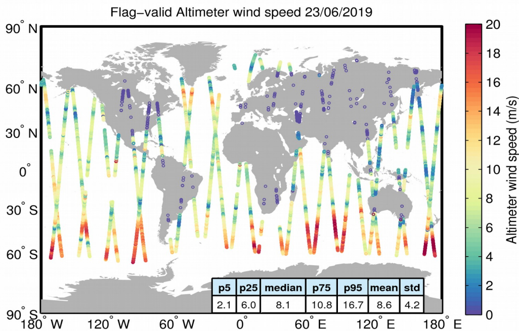
Figure 31. Geographical distribution of flag-valid wind data over oceans and lakes for 23/06/2019. The statistical values shown in the table refer to the wind in m/s and are calculated over all measurements shown in the figure.
