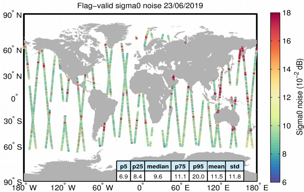
Figure 26. Geographical distribution of flag-valid 20-Hz sigma0 measurement noise over oceans and lakes for 23/06/2019. The statistical values shown in the table refer to the sigma0 noise and are calculated over all measurements shown in the figure.
