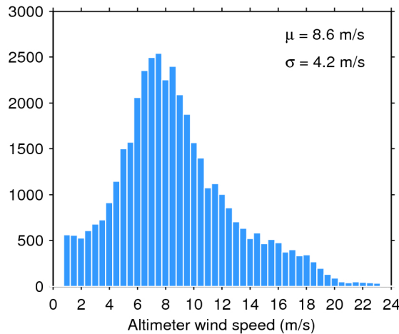
Figure 33. Histogram of flag-valid wind over oceans and lakes for 23/06/2019. The mean ( \mu ) and standard deviation ( \sigma ) are also shown. Note that values larger than 24 m/s are excluded from the histogram for the sake of readability but not from the computation of \mu and \sigma .
