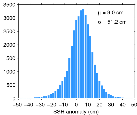
Figure 7. Histogram of flag-valid SSH anomaly over oceans and lakes for 23/06/2019. The mean ( \mu ) and standard deviation ( \sigma ) are also shown. Note that values outside [-50 50] cm are excluded from the histogram for the sake of readability but not from the computation of \mu and \sigma .
