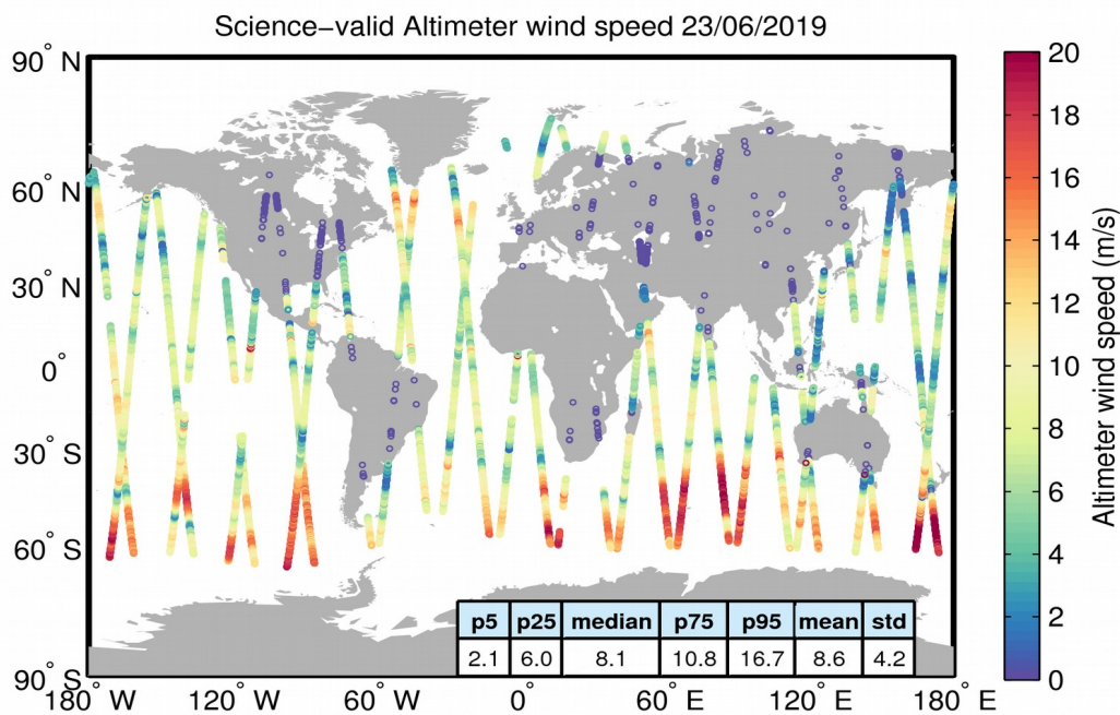
Figure 34. Geographical distribution of science-valid wind data over oceans and lakes for 23/06/2019. The statistical values shown in the table refer to the wind in m/s and are calculated over all measurements shown in the figure. Gray circles denote records that have been rejected based on the editing criteria described in Table 5.
