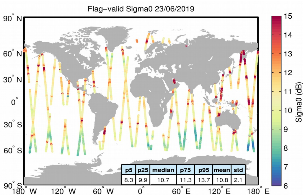
Figure 23. Geographical distribution of flag-valid sigma0 data over oceans and lakes for 23/06/2019. The statistical values shown in the table refer to the sigma0 in dB and are calculated over all measurements shown in the figure.
