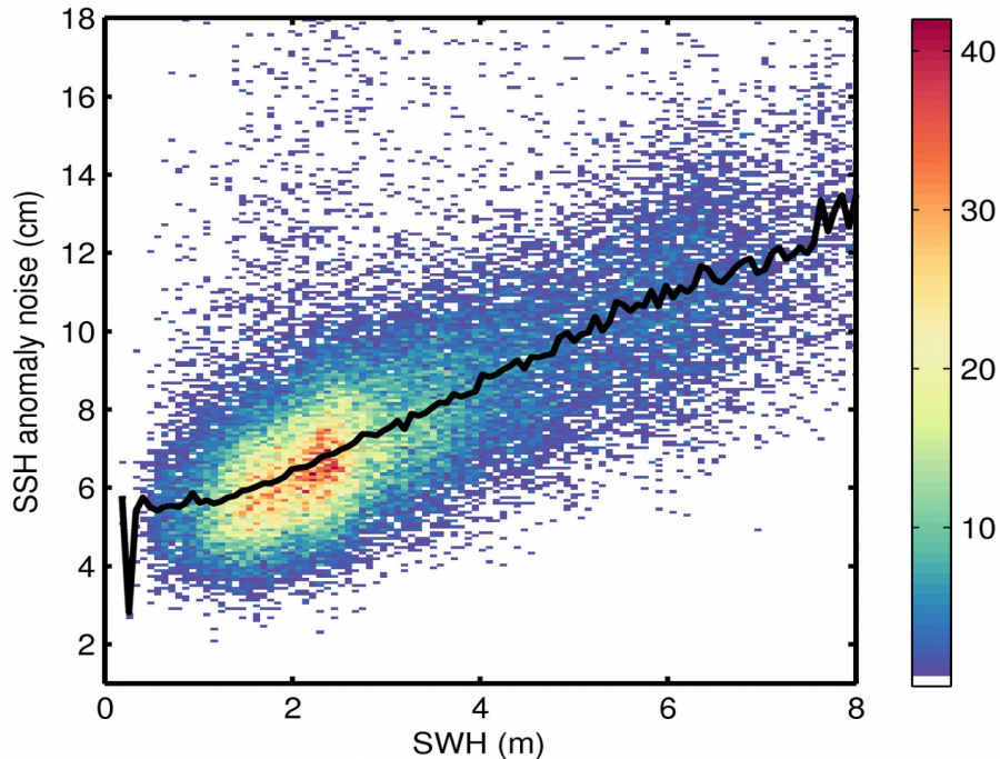
Figure 9. 2D histogram showing flag-valid SSH anomaly noise as a function of SWH for 23/06/2019. The black line denotes the median SSH anomaly noise as a function of SWH.
