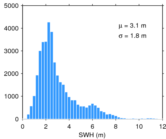
Figure 17. Histogram of flag-valid SWH over oceans and lakes for 23/06/2019. The mean ( \mu ) and standard deviation ( \sigma ) are also shown. Note that values larger than 12 m are excluded from the histogram for the sake of readability but not from the computation of \mu and \sigma .
