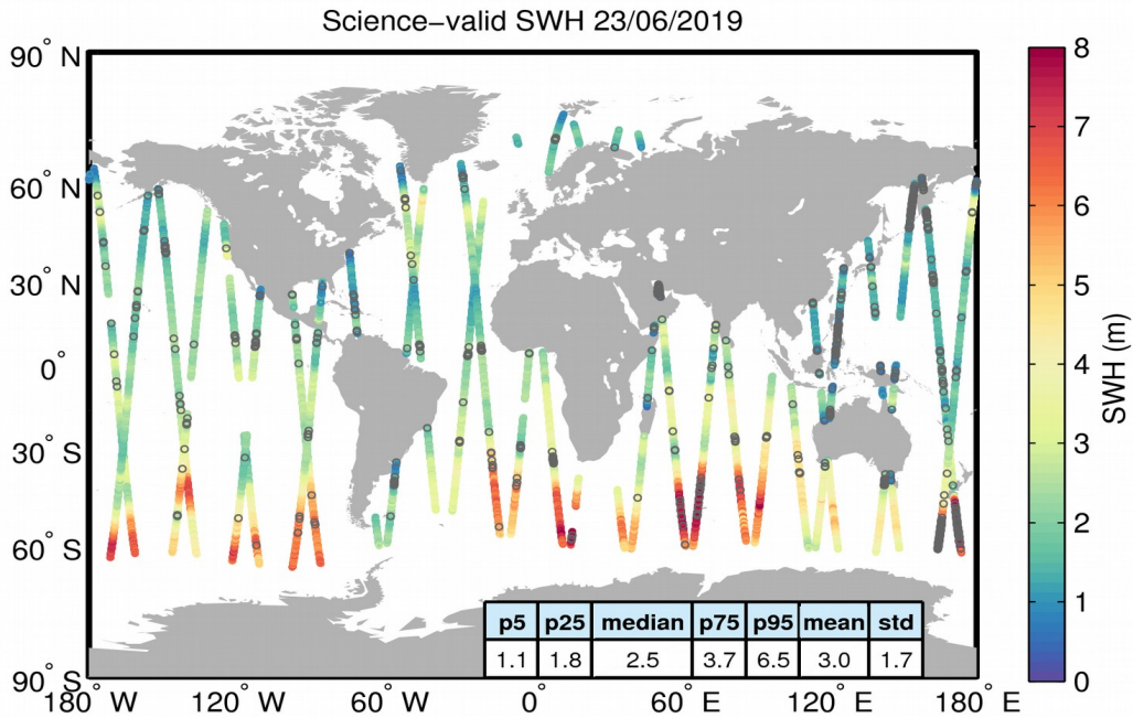
Figure 19. Geographical distribution of science-valid SWH data over oceans and lakes for 23/06/2019. The statistical values shown in the table refer to the SWH in m and are calculated over all measurements shown in the figure. Gray circles denote records that have been rejected based on the editing criteria described in Table 3.
