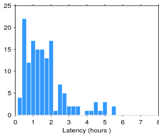
Figure 2. Histogram of the data latency for 23/06/2019. The y-axis denotes the number of files that are made available with a delay of x-hours with respect to the mean time of the records stored in the file.
