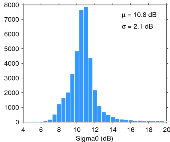
Figure 25. Histogram of flag-valid sigma0 over oceans and lakes for 23/06/2019. The mean ( \mu ) and standard deviation ( \sigma ) are also shown. Note that values outside [4 20] dB are excluded from the histogram for the sake of readability but not from the computation of \mu and \sigma .
