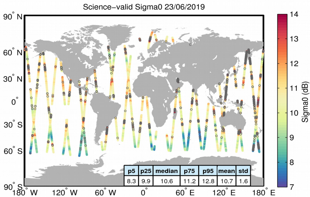
Figure 27. Geographical distribution of science-valid sigma0 data over oceans and lakes for 23/06/2019. The statistical values shown in the table refer to the sigma0 in dB and are calculated over all measurements shown in the figure. Gray circles denote records that have been rejected based on the editing criteria described in Table 4.
