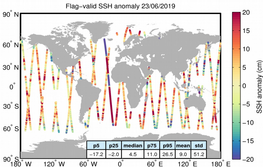
Figure 5. Geographical distribution of flag-valid 1-Hz SSH anomaly data over oceans and lakes for 23/06/2019. The statistical values shown in the table refer to the SSH anomaly in cm and are calculated over all measurements shown in the figure.
