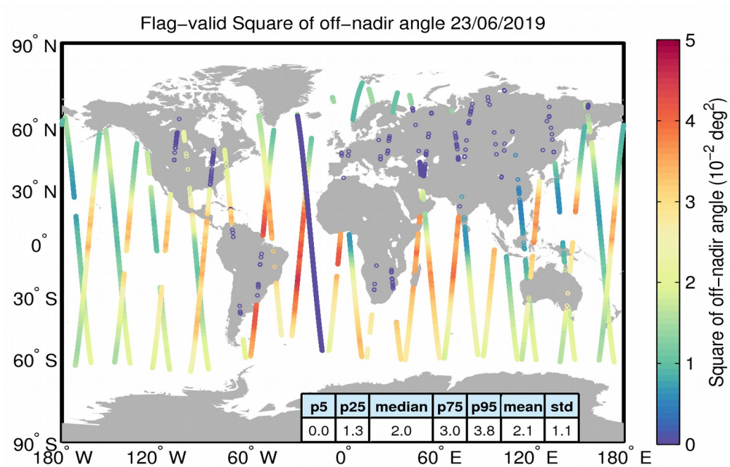
Figure 37. Geographical distribution of flag-valid mispointing data over oceans and lakes for 23/06/2019. The statistical values shown in the table refer to the mispointing in 10^{-2} \text{ deg}^2 and are calculated over all measurements shown in the figure.
