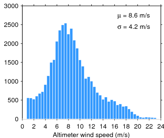
Figure 35. Histogram of science-valid wind over oceans and lakes for 23/06/2019. The mean ( \mu ) and standard deviation ( \sigma ) are also shown. Note that values larger than 24 m/s are excluded from the histogram for the sake of readability but not from the computation of \mu and \sigma .
