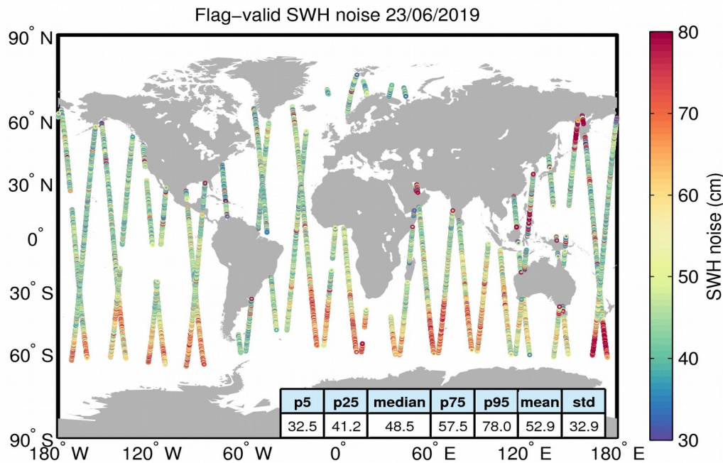
Figure 18. Geographical distribution of flag-valid 20-Hz SWH measurement noise over oceans and lakes for 23/06/2019. The statistical values shown in the figure refer to the SWH noise and are calculated over all measurements shown in the figure.
