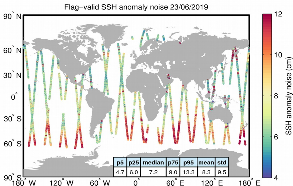
Figure 8. Geographical distribution of flag-valid 20-Hz SSH anomaly measurement noise over oceans and lakes for 23/06/2019. The statistical values shown in the table refer to the SSH anomaly noise and are calculated over all measurements shown in the figure.
