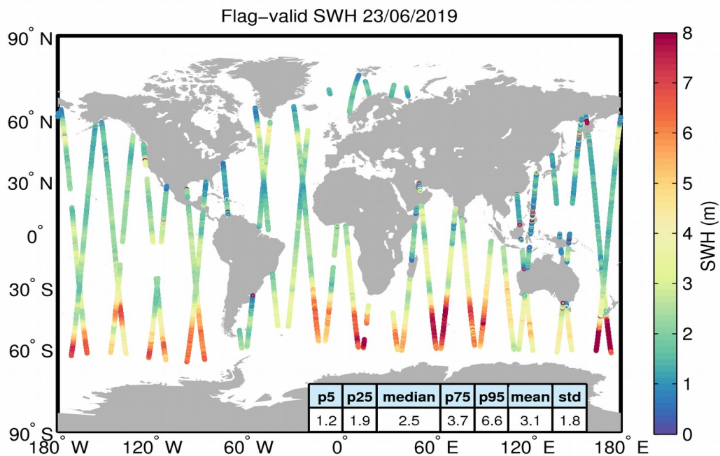
Figure 15. Geographical distribution of flag-valid SWH data over oceans and lakes for 23/06/2019. The statistical values shown in the table refer to the SWH in m and are calculated over all measurements shown in the figure.
