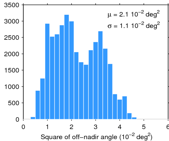
Figure 39. Histogram of flag-valid mispointing over oceans and lakes for 23/06/2019. The mean ( \mu ) and standard deviation ( \sigma ) are also shown. Note that values larger than 6 \cdot 10^{-2} \text{ deg}^2 are excluded from the histogram for the sake of readability but not from the computation of \mu and \sigma .
