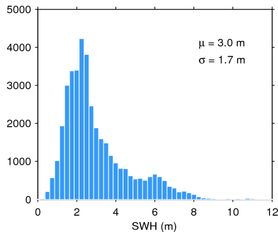
Figure 20. Histogram of science-valid SWH over oceans and lakes for 23/06/2019. The mean ( \mu ) and standard deviation ( \sigma ) are also shown. Note that values larger than 12 m are excluded from the histogram for the sake of readability but not from the computation of \mu and \sigma .
