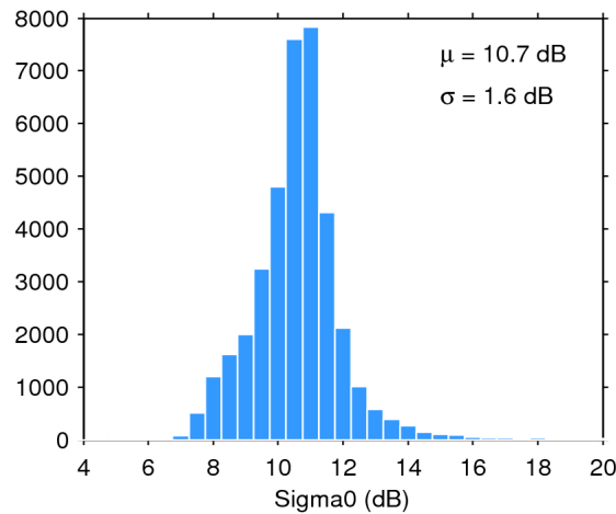
Figure 28. Histogram of science-valid sigma0 over oceans and lakes for 23/06/2019. The mean ( \mu ) and standard deviation ( \sigma ) are also shown. Note that values outside [4 20] dB are excluded from the histogram for the sake of readability but not from the computation of \mu and \sigma .
