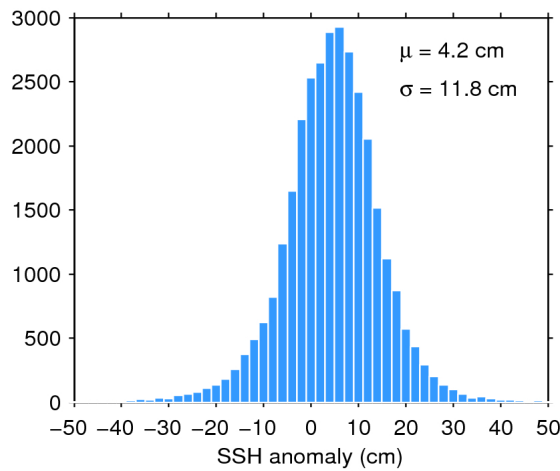
Figure 11. Histogram of science-valid SSH anomaly over oceans and lakes for 23/06/2019. The mean ( \mu ) and standard deviation ( \sigma ) are also shown. Note that values outside [-50 50] cm are excluded from the histogram for the sake of readability but not from the computation of \mu and \sigma .
