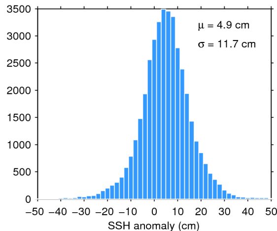
Figure 11. Histogram of science-valid SSH anomaly over oceans and lakes for 20/06/2019. The mean ( \mu ) and standard deviation ( \sigma ) are also shown. Note that values outside [-50 50] cm are excluded from the histogram for the sake of readability but not from the computation of \mu and \sigma .
