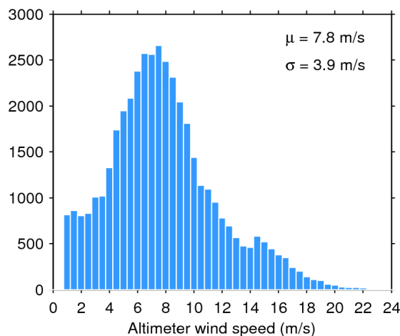
Figure 35. Histogram of science-valid wind over oceans and lakes for 20/06/2019. The mean ( \mu ) and standard deviation ( \sigma ) are also shown. Note that values larger than 24 m/s are excluded from the histogram for the sake of readability but not from the computation of \mu and \sigma .
