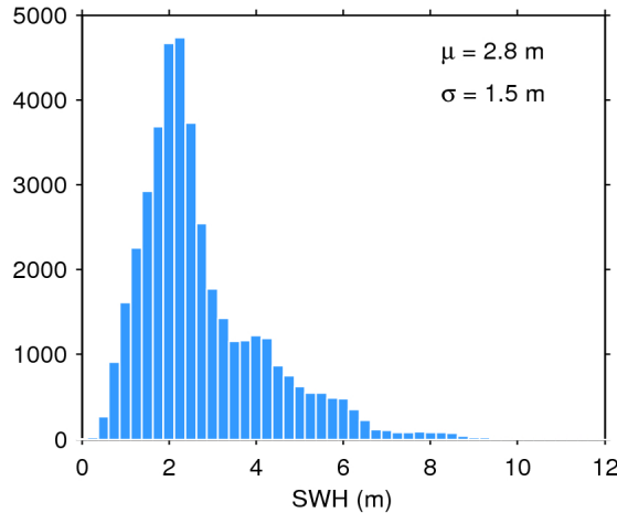
Figure 20. Histogram of science-valid SWH over oceans and lakes for 20/06/2019. The mean ( \mu ) and standard deviation ( \sigma ) are also shown. Note that values larger than 12 m are excluded from the histogram for the sake of readability but not from the computation of \mu and \sigma .
