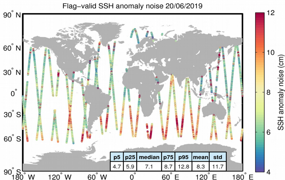
Figure 8. Geographical distribution of flag-valid 20-Hz SSH anomaly measurement noise over oceans and lakes for 20/06/2019. The statistical values shown in the table refer to the SSH anomaly noise and are calculated over all measurements shown in the figure.
