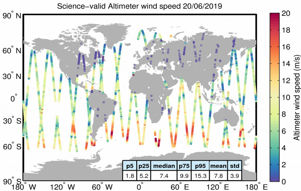
Figure 34. Geographical distribution of science-valid wind data over oceans and lakes for 20/06/2019. The statistical values shown in the table refer to the wind in m/s and are calculated over all measurements shown in the figure. Gray circles denote records that have been rejected based on the editing criteria described in Table 5.
