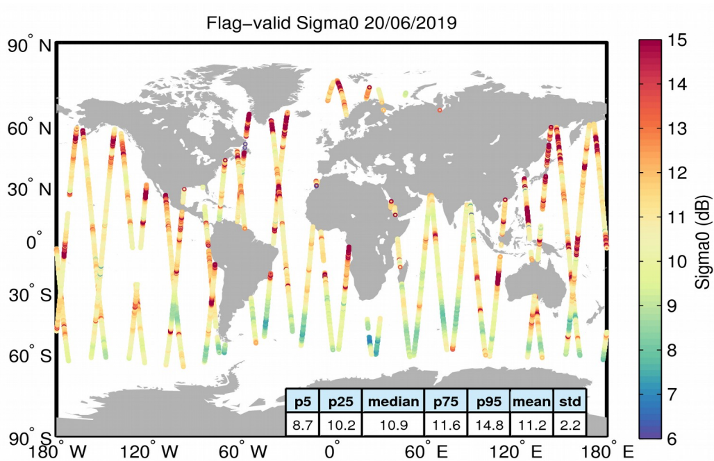
Figure 23. Geographical distribution of flag-valid sigma0 data over oceans and lakes for 20/06/2019. The statistical values shown in the table refer to the sigma0 in dB and are calculated over all measurements shown in the figure.
