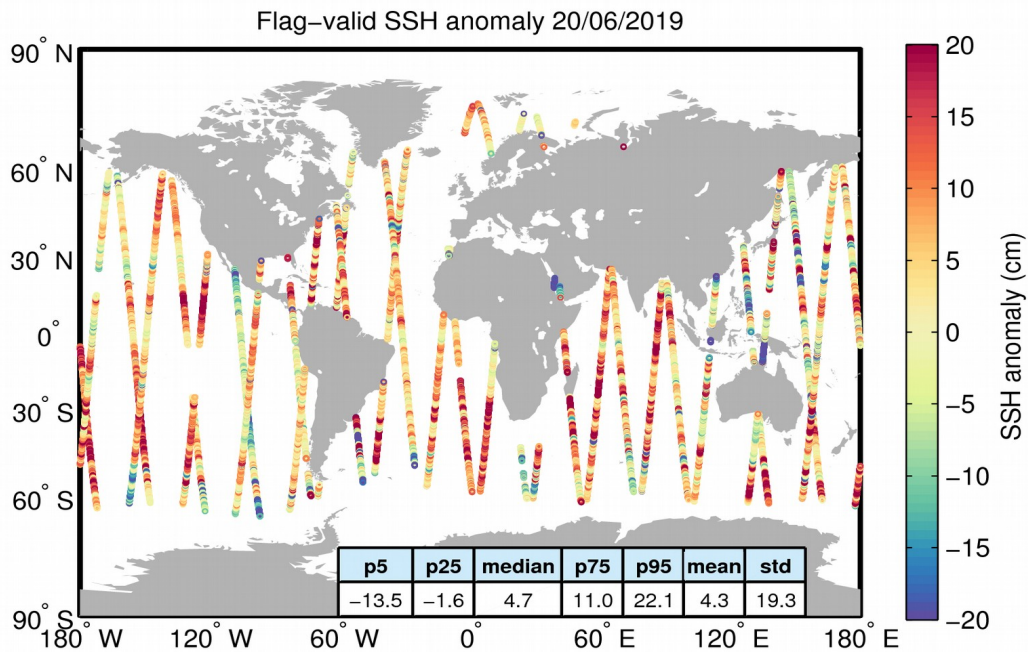
Figure 5. Geographical distribution of flag-valid 1-Hz SSH anomaly data over oceans and lakes for 20/06/2019. The statistical values shown in the table refer to the SSH anomaly in cm and are calculated over all measurements shown in the figure.
