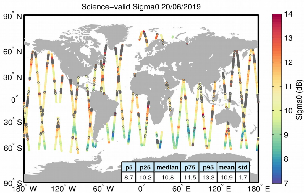
Figure 27. Geographical distribution of science-valid sigma0 data over oceans and lakes for 20/06/2019. The statistical values shown in the table refer to the sigma0 in dB and are calculated over all measurements shown in the figure. Gray circles denote records that have been rejected based on the editing criteria described in Table 4.
