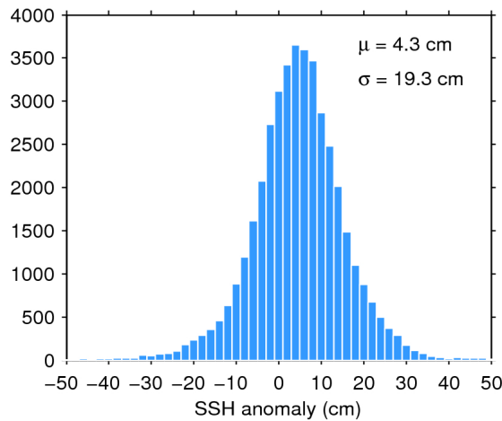
Figure 7. Histogram of flag-valid SSH anomaly over oceans and lakes for 20/06/2019. The mean ( \mu ) and standard deviation ( \sigma ) are also shown. Note that values outside [-50 50] cm are excluded from the histogram for the sake of readability but not from the computation of \mu and \sigma .
