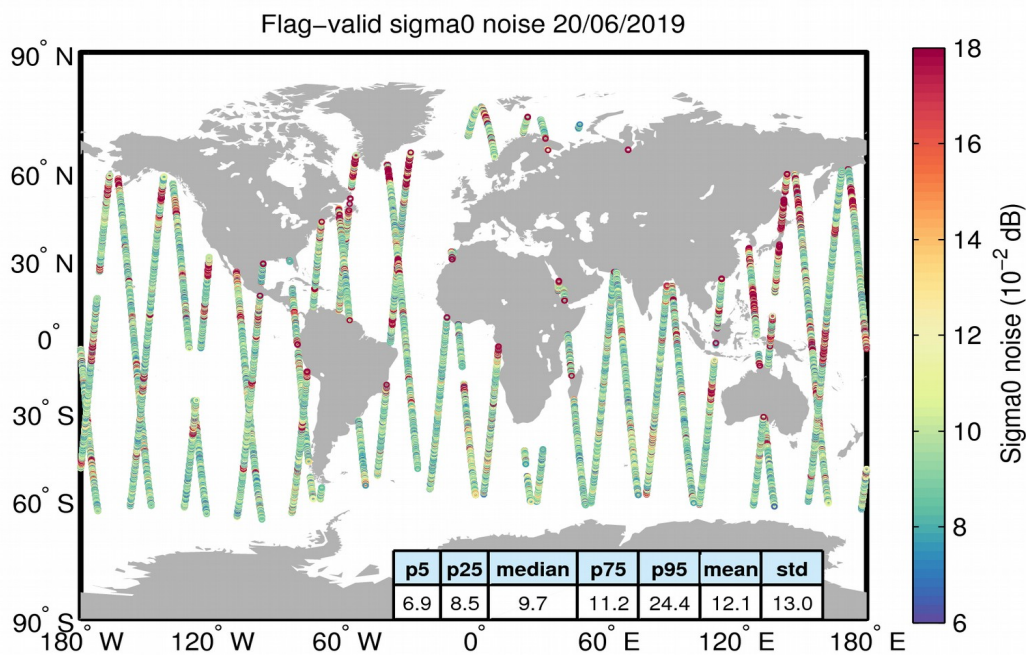
Figure 26. Geographical distribution of flag-valid 20-Hz sigma0 measurement noise over oceans and lakes for 20/06/2019. The statistical values shown in the table refer to the sigma0 noise and are calculated over all measurements shown in the figure.
