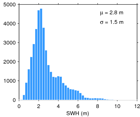
Figure 17. Histogram of flag-valid SWH over oceans and lakes for 20/06/2019. The mean ( \mu ) and standard deviation ( \sigma ) are also shown. Note that values larger than 12 m are excluded from the histogram for the sake of readability but not from the computation of \mu and \sigma .
