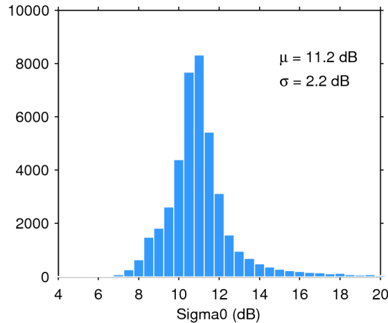
Figure 25. Histogram of flag-valid sigma0 over oceans and lakes for 20/06/2019. The mean ( \mu ) and standard deviation ( \sigma ) are also shown. Note that values outside [4 20] dB are excluded from the histogram for the sake of readability but not from the computation of \mu and \sigma .
