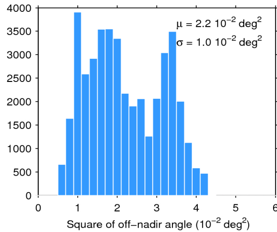
Figure 39. Histogram of flag-valid mispointing over oceans and lakes for 20/06/2019. The mean ( \mu ) and standard deviation ( \sigma ) are also shown. Note that values larger than 6 \cdot 10^{-2} \text{ deg}^2 are excluded from the histogram for the sake of readability but not from the computation of \mu and \sigma .
