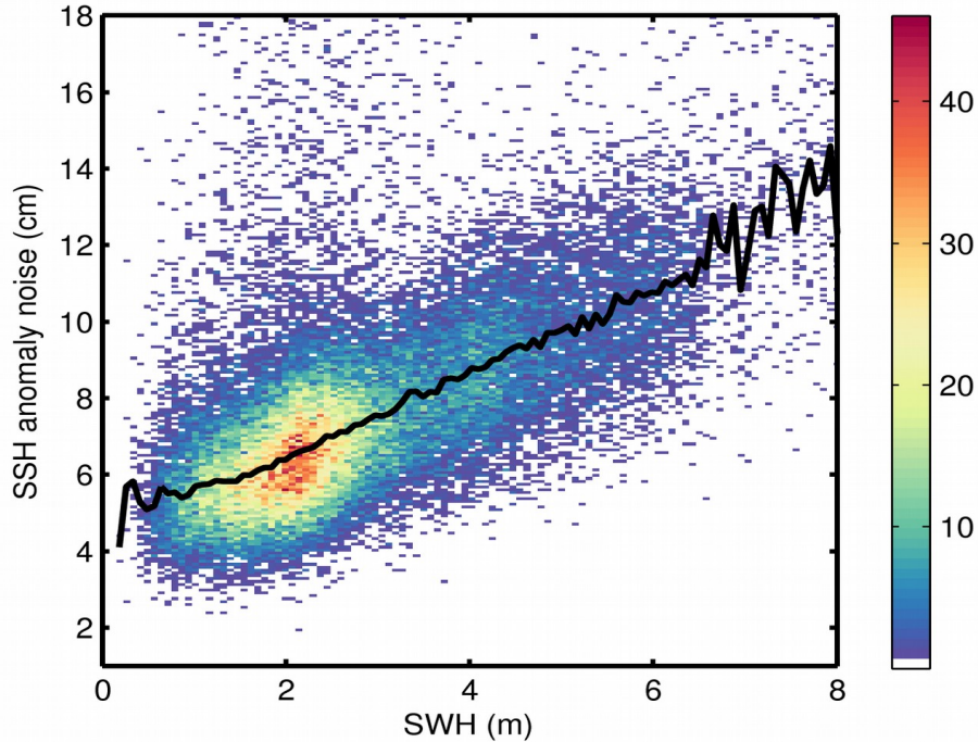
Figure 9. 2D histogram showing flag-valid SSH anomaly noise as a function of SWH for 20/06/2019. The black line denotes the median SSH anomaly noise as a function of SWH.
