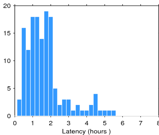
Figure 2. Histogram of the data latency for 20/06/2019. The y-axis denotes the number of files that are made available with a delay of x-hours with respect to the mean time of the records stored in the file.
