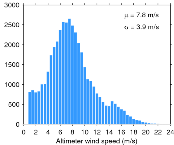
Figure 33. Histogram of flag-valid wind over oceans and lakes for 20/06/2019. The mean ( \mu ) and standard deviation ( \sigma ) are also shown. Note that values larger than 24 m/s are excluded from the histogram for the sake of readability but not from the computation of \mu and \sigma .
