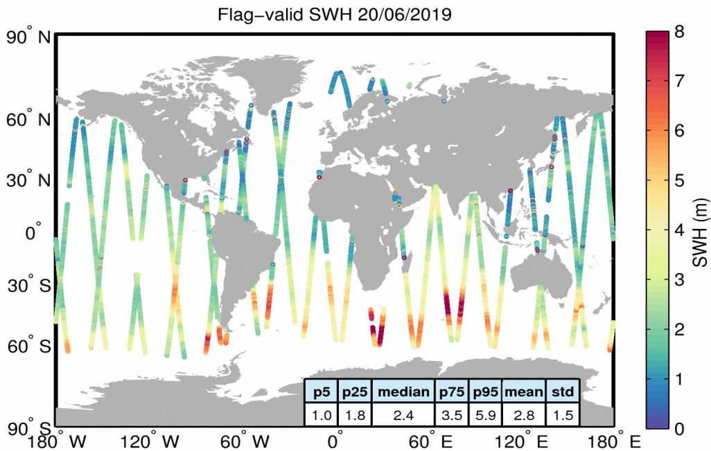
Figure 15. Geographical distribution of flag-valid SWH data over oceans and lakes for 20/06/2019. The statistical values shown in the table refer to the SWH in m and are calculated over all measurements shown in the figure.
