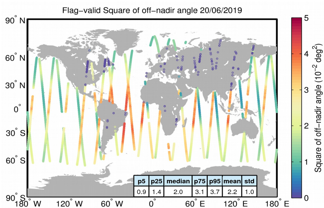
Figure 37. Geographical distribution of flag-valid mispointing data over oceans and lakes for 20/06/2019. The statistical values shown in the table refer to the mispointing in 10^{-2} \text{ deg}^2 and are calculated over all measurements shown in the figure.
