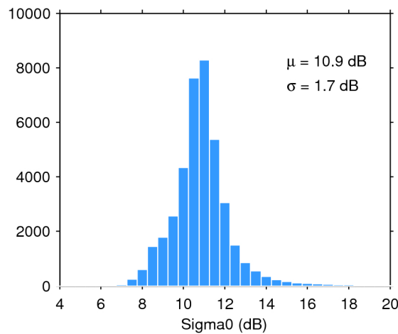
Figure 28. Histogram of science-valid sigma0 over oceans and lakes for 20/06/2019. The mean ( \mu ) and standard deviation ( \sigma ) are also shown. Note that values outside [4 20] dB are excluded from the histogram for the sake of readability but not from the computation of \mu and \sigma .
