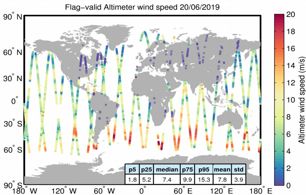
Figure 31. Geographical distribution of flag-valid wind data over oceans and lakes for 20/06/2019. The statistical values shown in the table refer to the wind in m/s and are calculated over all measurements shown in the figure.
