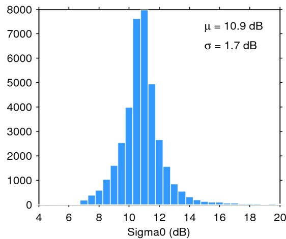
Figure 28. Histogram of science-valid sigma0 over oceans and lakes for 19/06/2019. The mean ( \mu ) and standard deviation ( \sigma ) are also shown. Note that values outside [4 20] dB are excluded from the histogram for the sake of readability but not from the computation of \mu and \sigma .
