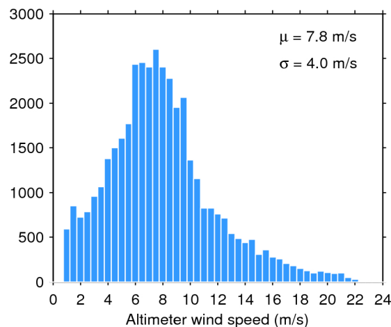
Figure 35. Histogram of science-valid wind over oceans and lakes for 19/06/2019. The mean ( \mu ) and standard deviation ( \sigma ) are also shown. Note that values larger than 24 m/s are excluded from the histogram for the sake of readability but not from the computation of \mu and \sigma .
