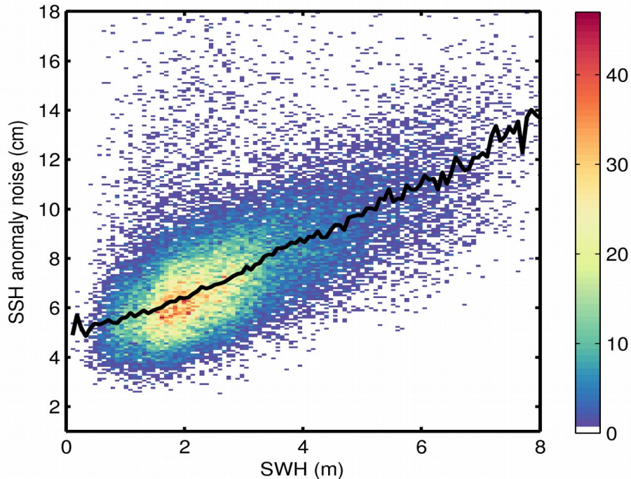
Figure 9. 2D histogram showing flag-valid SSH anomaly noise as a function of SWH for 19/06/2019. The black line denotes the median SSH anomaly noise as a function of SWH.
