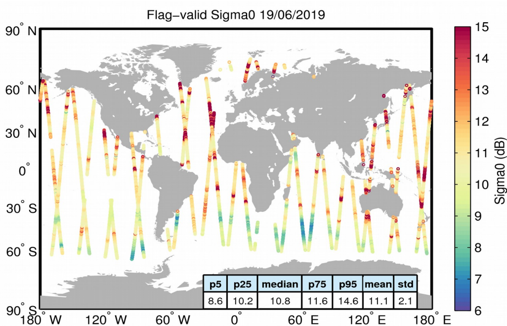
Figure 23. Geographical distribution of flag-valid sigma0 data over oceans and lakes for 19/06/2019. The statistical values shown in the table refer to the sigma0 in dB and are calculated over all measurements shown in the figure.
