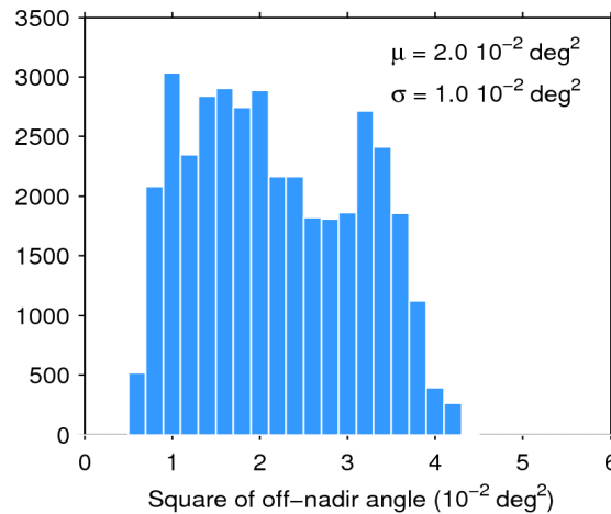
Figure 39. Histogram of flag-valid mispointing over oceans and lakes for 19/06/2019. The mean ( \mu ) and standard deviation ( \sigma ) are also shown. Note that values larger than 6 \cdot 10^{-2} \text{ deg}^2 are excluded from the histogram for the sake of readability but not from the computation of \mu and \sigma .
