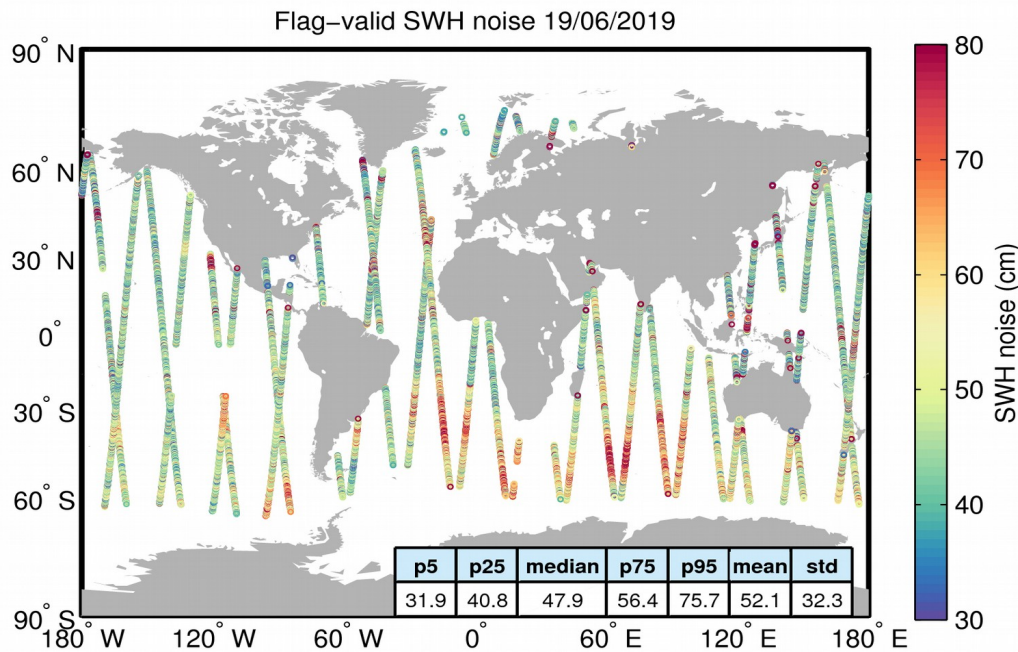
Figure 18. Geographical distribution of flag-valid 20-Hz SWH measurement noise over oceans and lakes for 19/06/2019. The statistical values shown in the table refer to the SWH noise and are calculated over all measurements shown in the figure.
