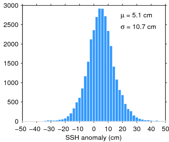
Figure 11. Histogram of science-valid SSH anomaly over oceans and lakes for 19/06/2019. The mean ( \mu ) and standard deviation ( \sigma ) are also shown. Note that values outside [-50 50] cm are excluded from the histogram for the sake of readability but not from the computation of \mu and \sigma .
