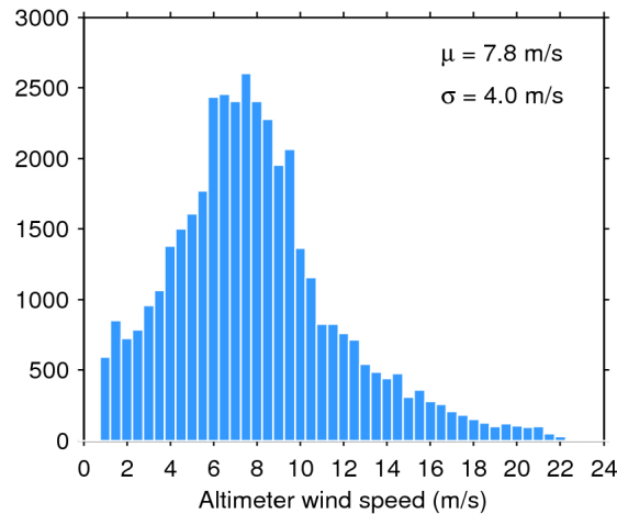
Figure 33. Histogram of flag-valid wind over oceans and lakes for 19/06/2019. The mean ( \mu ) and standard deviation ( \sigma ) are also shown. Note that values larger than 24 m/s are excluded from the histogram for the sake of readability but not from the computation of \mu and \sigma .
