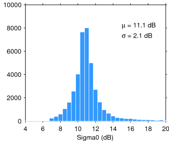
Figure 25. Histogram of flag-valid sigma0 over oceans and lakes for 19/06/2019. The mean ( \mu ) and standard deviation ( \sigma ) are also shown. Note that values outside [4 20] dB are excluded from the histogram for the sake of readability but not from the computation of \mu and \sigma .
