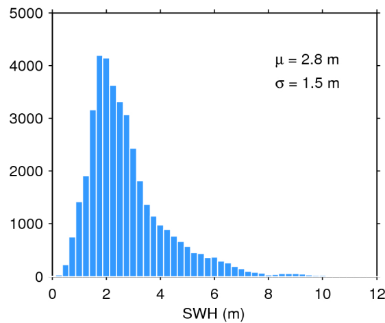
Figure 17. Histogram of flag-valid SWH over oceans and lakes for 19/06/2019. The mean ( \mu ) and standard deviation ( \sigma ) are also shown. Note that values larger than 12 m are excluded from the histogram for the sake of readability but not from the computation of \mu and \sigma .
