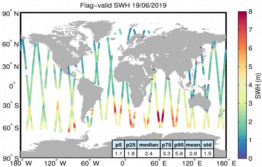
Figure 15. Geographical distribution of flag-valid SWH data over oceans and lakes for 19/06/2019. The statistical values shown in the table refer to the SWH in m and are calculated over all measurements shown in the figure.
