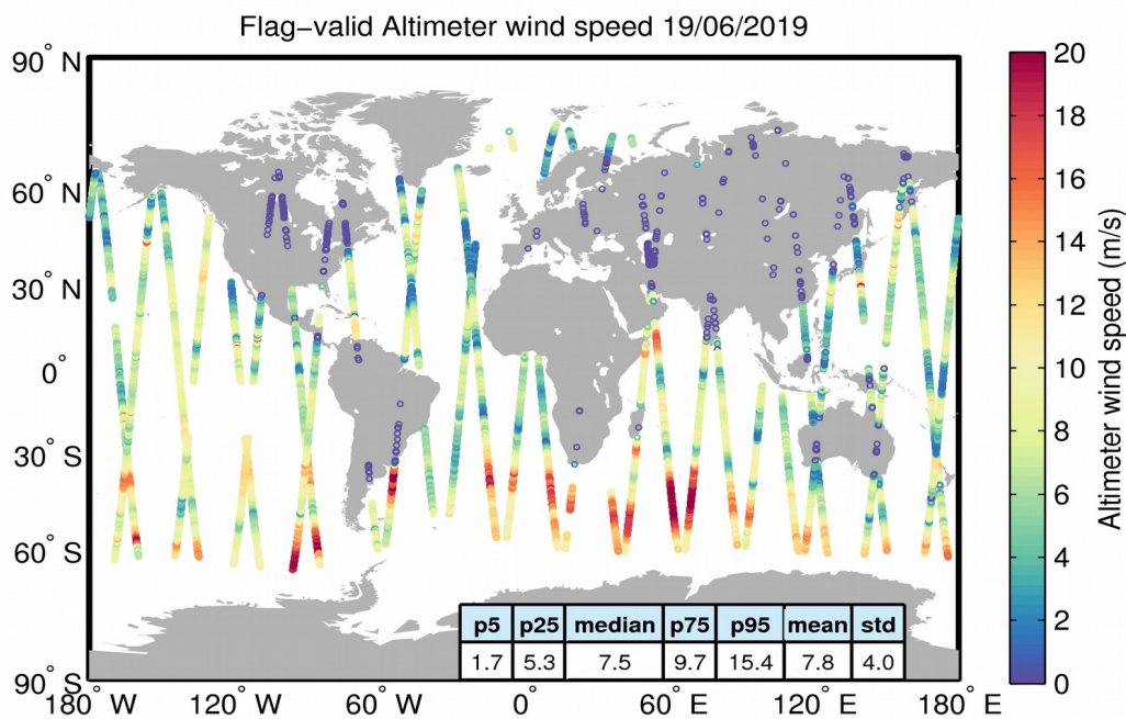
Figure 31. Geographical distribution of flag-valid wind data over oceans and lakes for 19/06/2019. The statistical values shown in the table refer to the wind in m/s and are calculated over all measurements shown in the figure.
