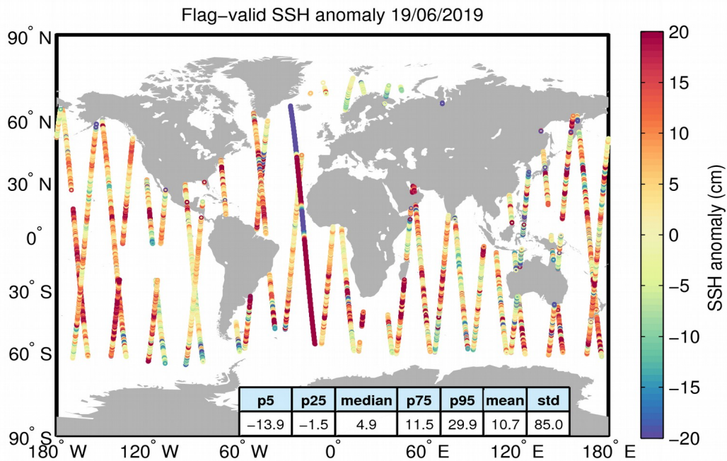
Figure 5. Geographical distribution of flag-valid 1-Hz SSH anomaly data over oceans and lakes for 19/06/2019. The statistical values shown in the table refer to the SSH anomaly in cm and are calculated over all measurements shown in the figure.
