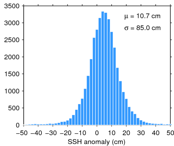
Figure 7. Histogram of flag-valid SSH anomaly over oceans and lakes for 19/06/2019. The mean ( \mu ) and standard deviation ( \sigma ) are also shown. Note that values outside [-50\ 50] cm are excluded from the histogram for the sake of readability but not from the computation of \mu and \sigma .
