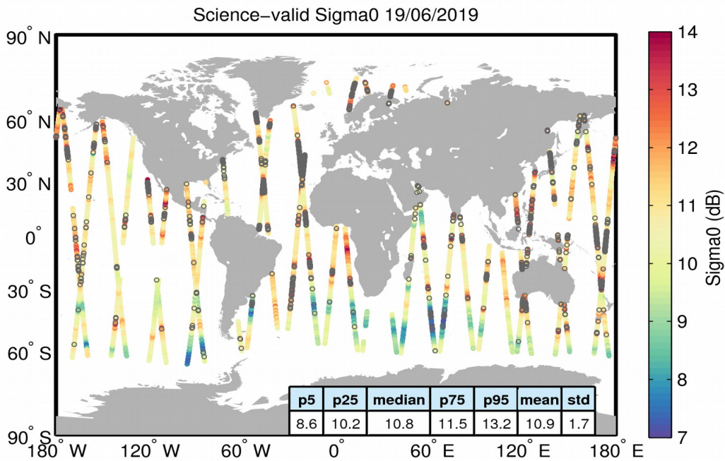
Figure 27. Geographical distribution of science-valid sigma0 data over oceans and lakes for 19/06/2019. The statistical values shown in the table refer to the sigma0 in dB and are calculated over all measurements shown in the figure. Gray circles denote records that have been rejected based on the editing criteria described in Table 4.
