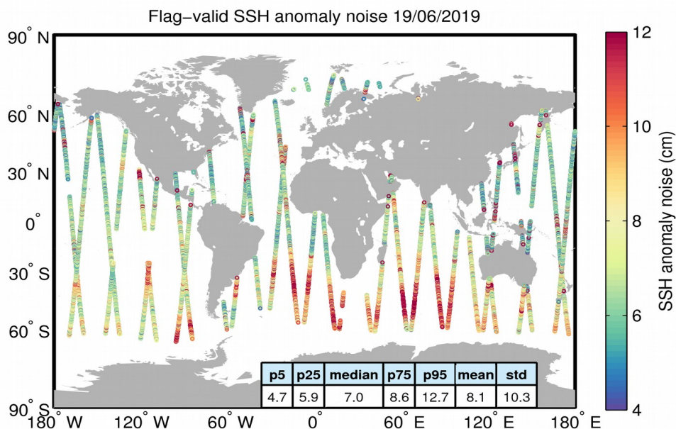
Figure 8. Geographical distribution of flag-valid 20-Hz SSH anomaly measurement noise over oceans and lakes for 19/06/2019. The statistical values shown in the table refer to the SSH anomaly noise and are calculated over all measurements shown in the figure.
