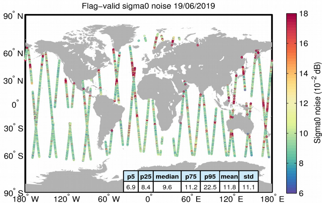
Figure 26. Geographical distribution of flag-valid 20-Hz sigma0 measurement noise over oceans and lakes for 19/06/2019. The statistical values shown in the table refer to the sigma0 noise and are calculated over all measurements shown in the figure.
