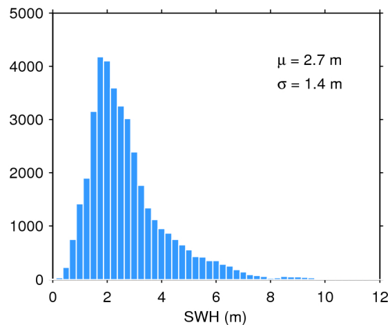
Figure 20. Histogram of science-valid SWH over oceans and lakes for 19/06/2019. The mean ( \mu ) and standard deviation ( \sigma ) are also shown. Note that values larger than 12 m are excluded from the histogram for the sake of readability but not from the computation of \mu and \sigma .
