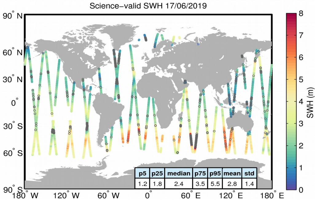
Figure 19. Geographical distribution of science-valid SWH data over oceans and lakes for 17/06/2019. The statistical values shown in the table refer to the SWH in m and are calculated over all measurements shown in the figure. Gray circles denote records that have been rejected based on the editing criteria described in Table 3.
