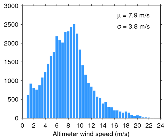
Figure 35. Histogram of science-valid wind over oceans and lakes for 17/06/2019. The mean ( \mu ) and standard deviation ( \sigma ) are also shown. Note that values larger than 24 m/s are excluded from the histogram for the sake of readability but not from the computation of \mu and \sigma .
