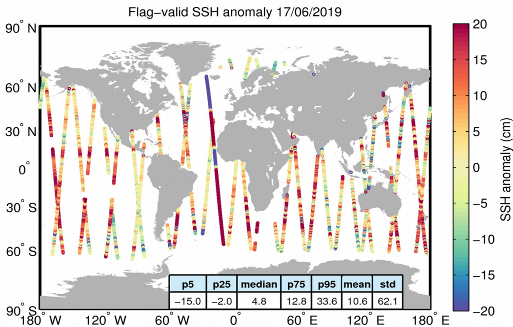
Figure 5. Geographical distribution of flag-valid 1-Hz SSH anomaly data over oceans and lakes for 17/06/2019. The statistical values shown in the table refer to the SSH anomaly in cm and are calculated over all measurements shown in the figure.
