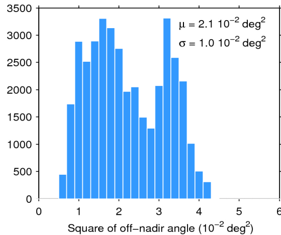
Figure 39. Histogram of flag-valid mispointing over oceans and lakes for 17/06/2019. The mean ( \mu ) and standard deviation ( \sigma ) are also shown. Note that values larger than 6 \cdot 10^{-2} \text{ deg}^2 are excluded from the histogram for the sake of readability but not from the computation of \mu and \sigma .
