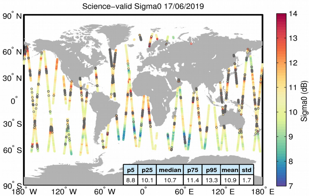
Figure 27. Geographical distribution of science-valid sigma0 data over oceans and lakes for 17/06/2019. The statistical values shown in the table refer to the sigma0 in dB and are calculated over all measurements shown in the figure. Gray circles denote records that have been rejected based on the editing criteria described in Table 4.
