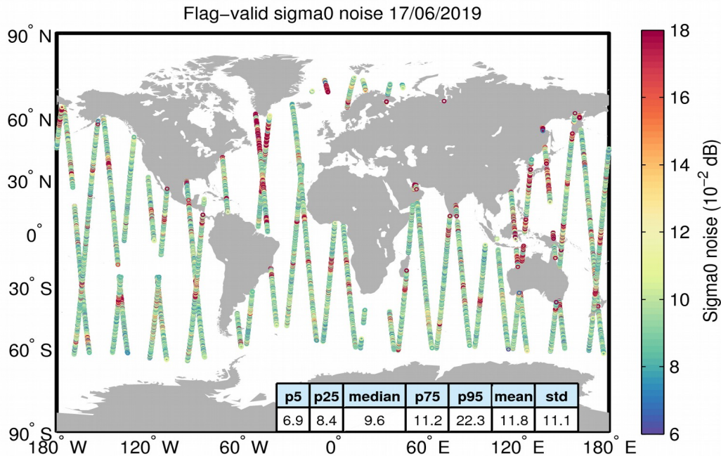
Figure 26. Geographical distribution of flag-valid 20-Hz sigma0 measurement noise over oceans and lakes for 17/06/2019. The statistical values shown in the table refer to the sigma0 noise and are calculated over all measurements shown in the figure.
