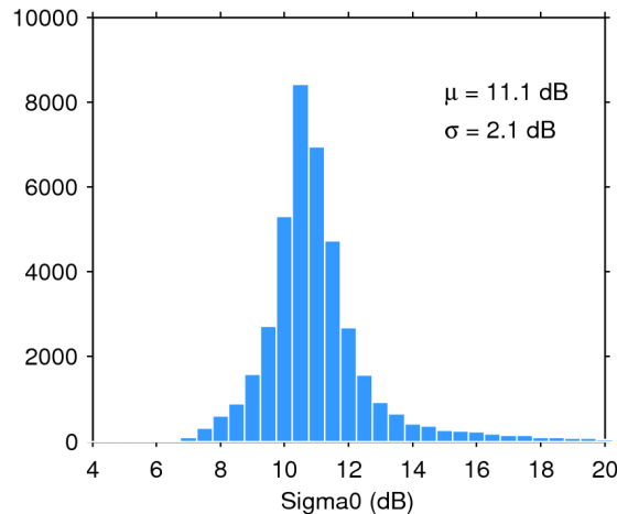
Figure 25. Histogram of flag-valid sigma0 over oceans and lakes for 17/06/2019. The mean ( \mu ) and standard deviation ( \sigma ) are also shown. Note that values outside [4 20] dB are excluded from the histogram for the sake of readability but not from the computation of \mu and \sigma .
