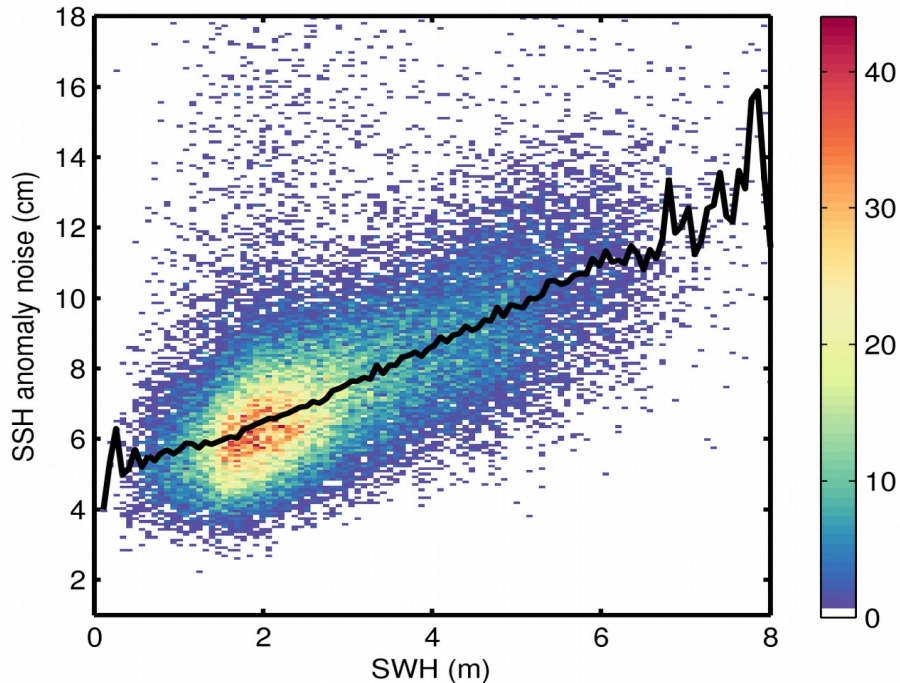
Figure 9. 2D histogram showing flag-valid SSH anomaly noise as a function of SWH for 17/06/2019. The black line denotes the median SSH anomaly noise as a function of SWH.
