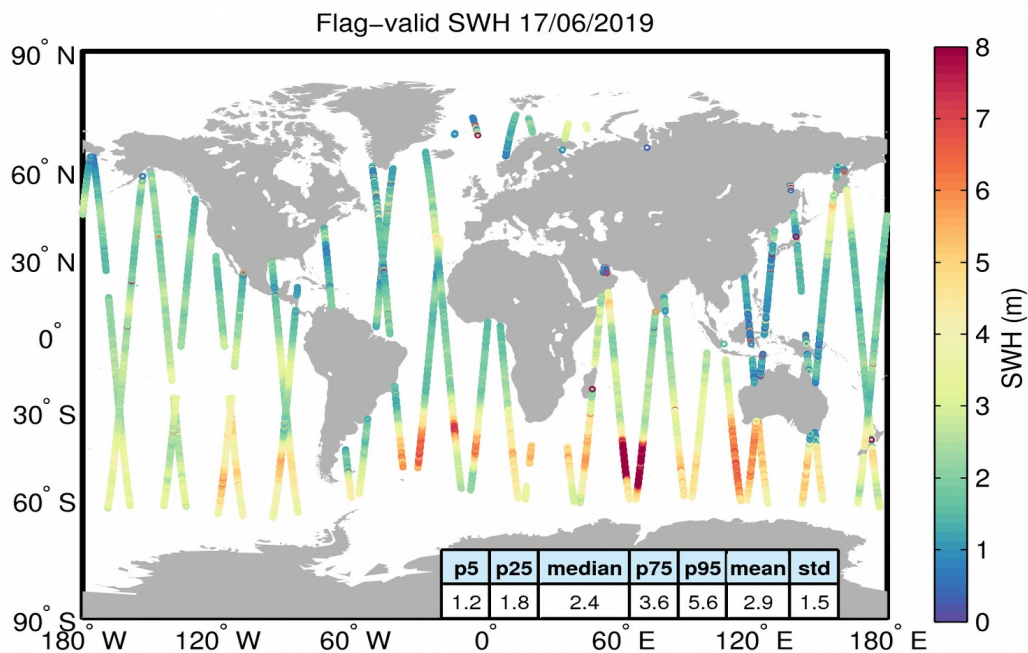
Figure 15. Geographical distribution of flag-valid SWH data over oceans and lakes for 17/06/2019. The statistical values shown in the table refer to the SWH in m and are calculated over all measurements shown in the figure.
