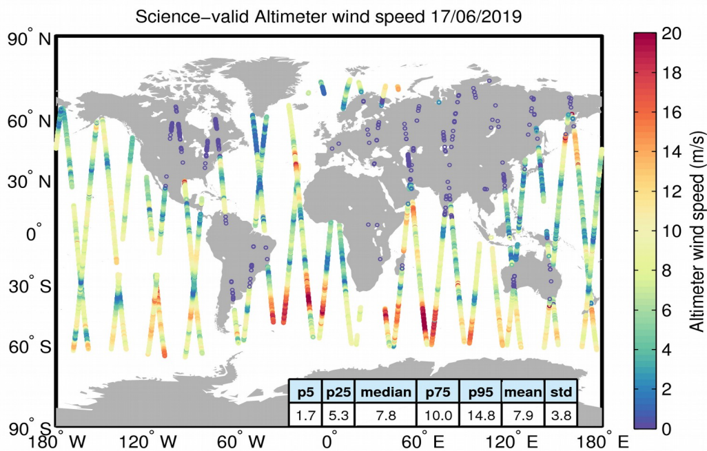
Figure 34. Geographical distribution of science-valid wind data over oceans and lakes for 17/06/2019. The statistical values shown in the table refer to the wind in m/s and are calculated over all measurements shown in the figure. Gray circles denote records that have been rejected based on the editing criteria described in Table 5.
