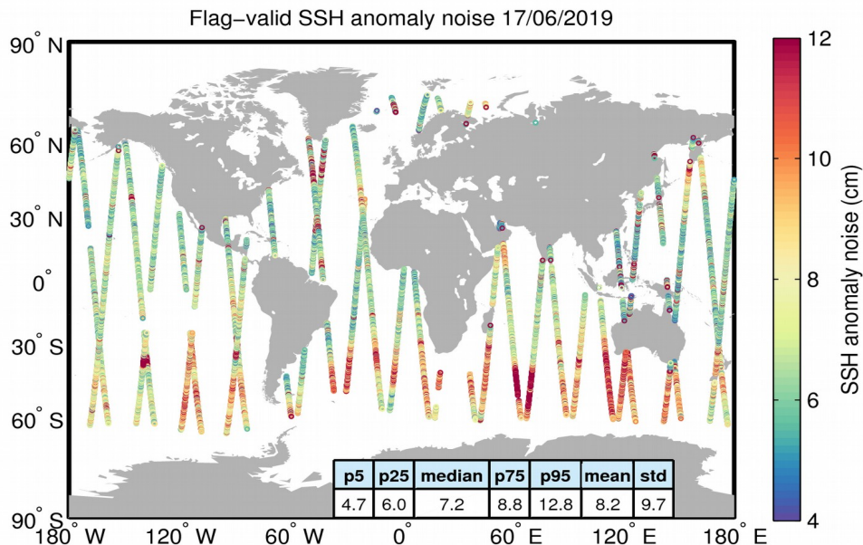
Figure 8. Geographical distribution of flag-valid 20-Hz SSH anomaly measurement noise over oceans and lakes for 17/06/2019. The statistical values shown in the table refer to the SSH anomaly noise and are calculated over all measurements shown in the figure.
