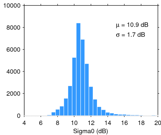
Figure 28. Histogram of science-valid sigma0 over oceans and lakes for 17/06/2019. The mean ( \mu ) and standard deviation ( \sigma ) are also shown. Note that values outside [4 20] dB are excluded from the histogram for the sake of readability but not from the computation of \mu and \sigma .
