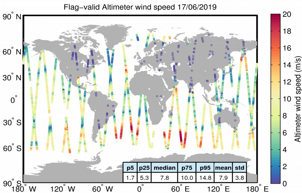
Figure 31. Geographical distribution of flag-valid wind data over oceans and lakes for 17/06/2019. The statistical values shown in the table refer to the wind in m/s and are calculated over all measurements shown in the figure.
