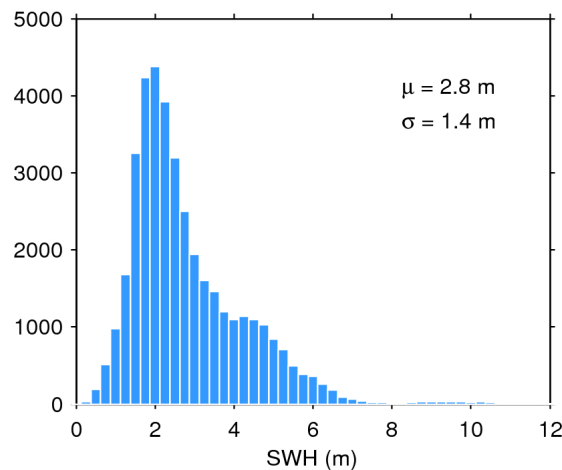
Figure 20. Histogram of science-valid SWH over oceans and lakes for 17/06/2019. The mean ( \mu ) and standard deviation ( \sigma ) are also shown. Note that values larger than 12 m are excluded from the histogram for the sake of readability but not from the computation of \mu and \sigma .
