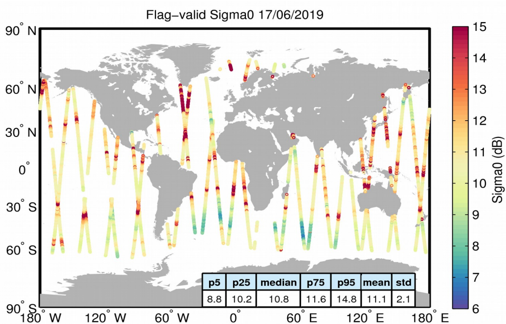
Figure 23. Geographical distribution of flag-valid sigma0 data over oceans and lakes for 17/06/2019. The statistical values shown in the table refer to the sigma0 in dB and are calculated over all measurements shown in the figure.
