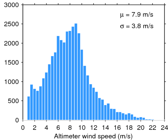
Figure 33. Histogram of flag-valid wind over oceans and lakes for 17/06/2019. The mean ( \mu ) and standard deviation ( \sigma ) are also shown. Note that values larger than 24 m/s are excluded from the histogram for the sake of readability but not from the computation of \mu and \sigma .
