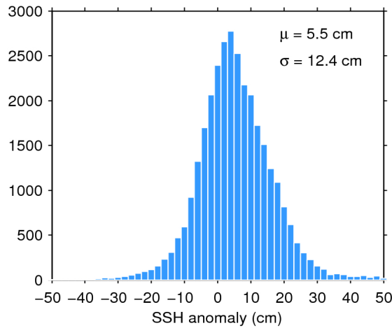
Figure 11. Histogram of science-valid SSH anomaly over oceans and lakes for 17/06/2019. The mean ( \mu ) and standard deviation ( \sigma ) are also shown. Note that values outside [-50 50] cm are excluded from the histogram for the sake of readability but not from the computation of \mu and \sigma .
