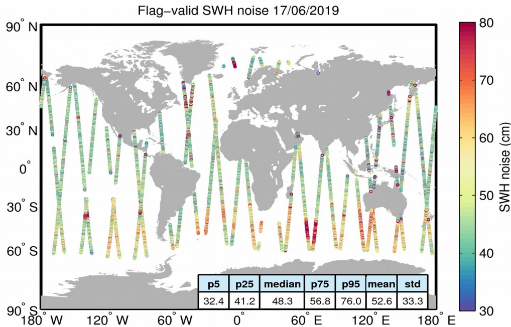
Figure 18. Geographical distribution of flag-valid 20-Hz SWH measurement noise over oceans and lakes for 17/06/2019. The statistical values shown in the figure refer to the SWH noise and are calculated over all measurements shown in the figure.
