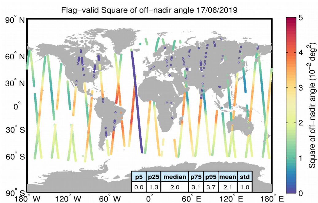
Figure 37. Geographical distribution of flag-valid mispointing data over oceans and lakes for 17/06/2019. The statistical values shown in the table refer to the mispointing in 10^{-2} deg 2 and are calculated over all measurements shown in the figure.
