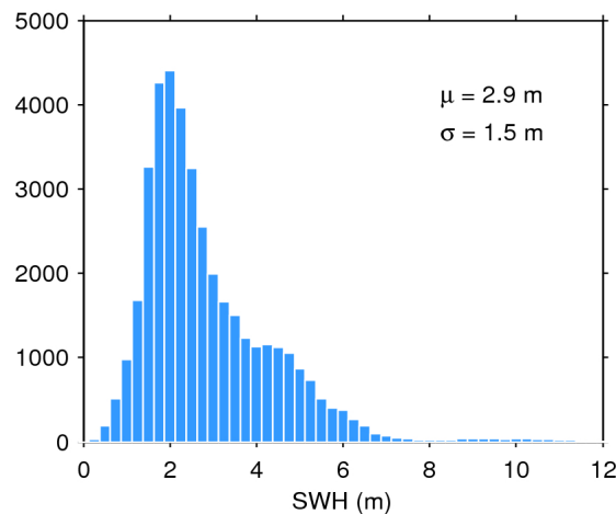
Figure 17. Histogram of flag-valid SWH over oceans and lakes for 17/06/2019. The mean ( \mu ) and standard deviation ( \sigma ) are also shown. Note that values larger than 12 m are excluded from the histogram for the sake of readability but not from the computation of \mu and \sigma .
