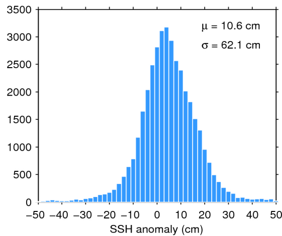
Figure 7. Histogram of flag-valid SSH anomaly over oceans and lakes for 17/06/2019. The mean ( \mu ) and standard deviation ( \sigma ) are also shown. Note that values outside [-50\ 50] cm are excluded from the histogram for the sake of readability but not from the computation of \mu and \sigma .
