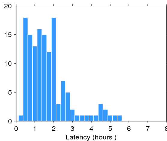
Figure 2. Histogram of the data latency for 17/06/2019. The y-axis denotes the number of files that are made available with a delay of x-hours with respect to the mean time of the records stored in the file.
