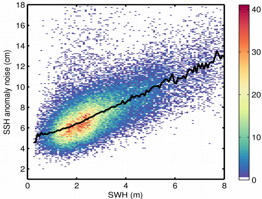
Figure 9. 2D histogram showing flag-valid SSH anomaly noise as a function of SWH for 15/06/2019. The black line denotes the median SSH anomaly noise as a function of SWH.
