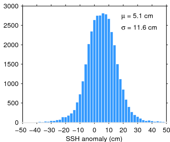
Figure 11. Histogram of science-valid SSH anomaly over oceans and lakes for 15/06/2019. The mean ( \mu ) and standard deviation ( \sigma ) are also shown. Note that values outside [-50 50] cm are excluded from the histogram for the sake of readability but not from the computation of \mu and \sigma .
