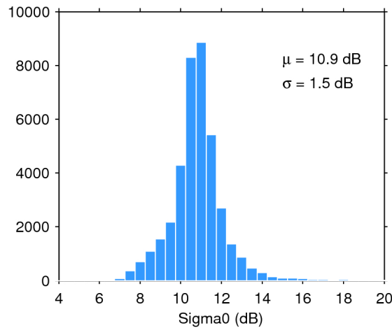
Figure 28. Histogram of science-valid sigma0 over oceans and lakes for 15/06/2019. The mean ( \mu ) and standard deviation ( \sigma ) are also shown. Note that values outside [4 20] dB are excluded from the histogram for the sake of readability but not from the computation of \mu and \sigma .
