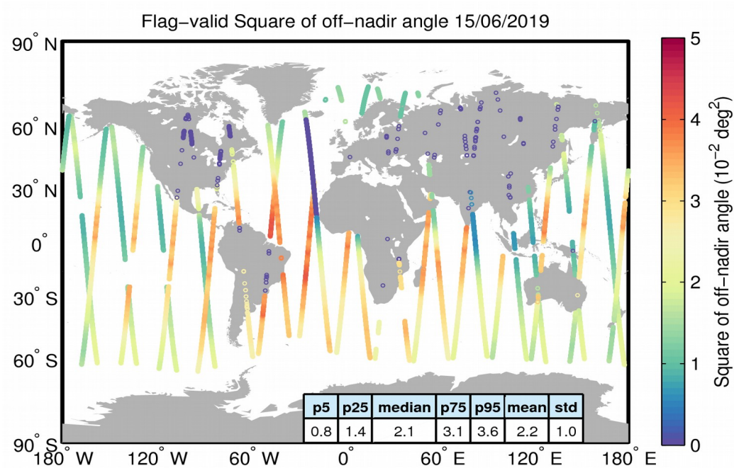
Figure 37. Geographical distribution of flag-valid mispointing data over oceans and lakes for 15/06/2019. The statistical values shown in the table refer to the mispointing in 10^{-2} \text{ deg}^2 and are calculated over all measurements shown in the figure.
