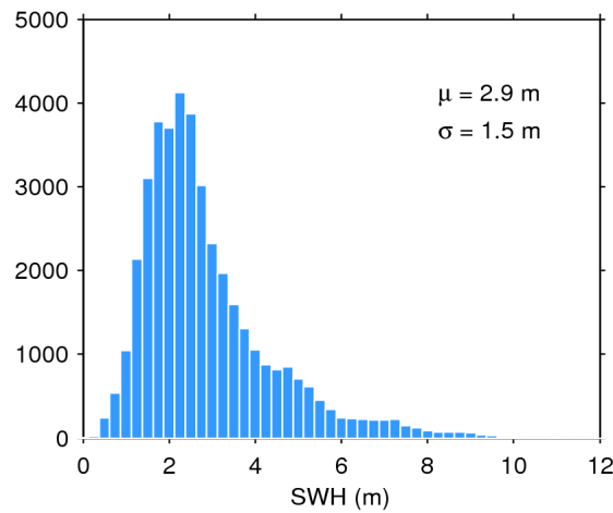
Figure 17. Histogram of flag-valid SWH over oceans and lakes for 15/06/2019. The mean ( \mu ) and standard deviation ( \sigma ) are also shown. Note that values larger than 12 m are excluded from the histogram for the sake of readability but not from the computation of \mu and \sigma .
