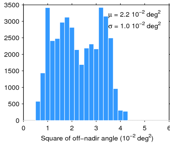
Figure 39. Histogram of flag-valid mispointing over oceans and lakes for 15/06/2019. The mean ( \mu ) and standard deviation ( \sigma ) are also shown. Note that values larger than 6 \cdot 10^{-2} \text{ deg}^2 are excluded from the histogram for the sake of readability but not from the computation of \mu and \sigma .
