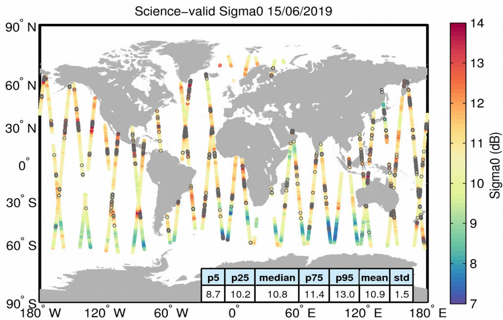
Figure 27. Geographical distribution of science-valid sigma0 data over oceans and lakes for 15/06/2019. The statistical values shown in the table refer to the sigma0 in dB and are calculated over all measurements shown in the figure. Gray circles denote records that have been rejected based on the editing criteria described in Table 4.
