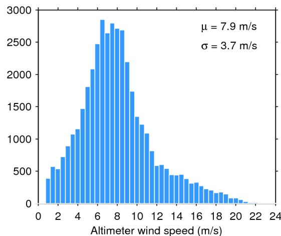
Figure 35. Histogram of science-valid wind over oceans and lakes for 15/06/2019. The mean ( \mu ) and standard deviation ( \sigma ) are also shown. Note that values larger than 24 m/s are excluded from the histogram for the sake of readability but not from the computation of \mu and \sigma .
