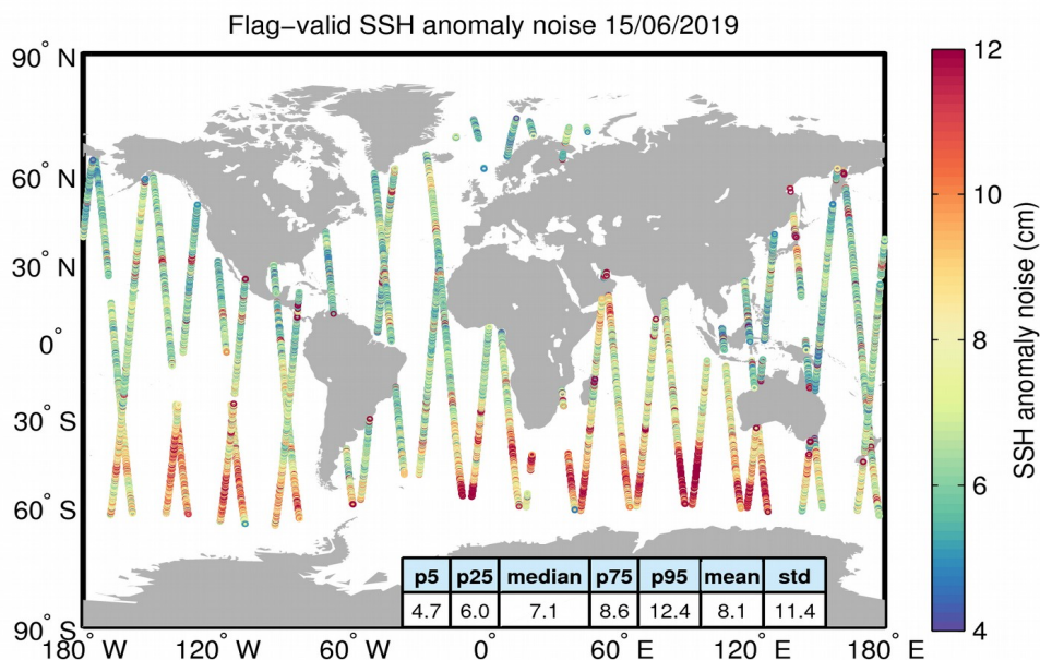
Figure 8. Geographical distribution of flag-valid 20-Hz SSH anomaly measurement noise over oceans and lakes for 15/06/2019. The statistical values shown in the table refer to the SSH anomaly noise and are calculated over all measurements shown in the figure.
