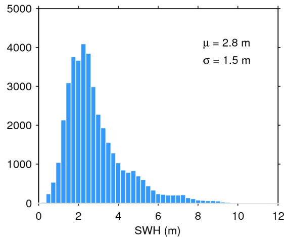
Figure 20. Histogram of science-valid SWH over oceans and lakes for 15/06/2019. The mean ( \mu ) and standard deviation ( \sigma ) are also shown. Note that values larger than 12 m are excluded from the histogram for the sake of readability but not from the computation of \mu and \sigma .
