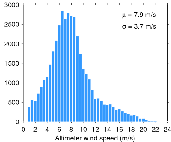
Figure 33. Histogram of flag-valid wind over oceans and lakes for 15/06/2019. The mean ( \mu ) and standard deviation ( \sigma ) are also shown. Note that values larger than 24 m/s are excluded from the histogram for the sake of readability but not from the computation of \mu and \sigma .
