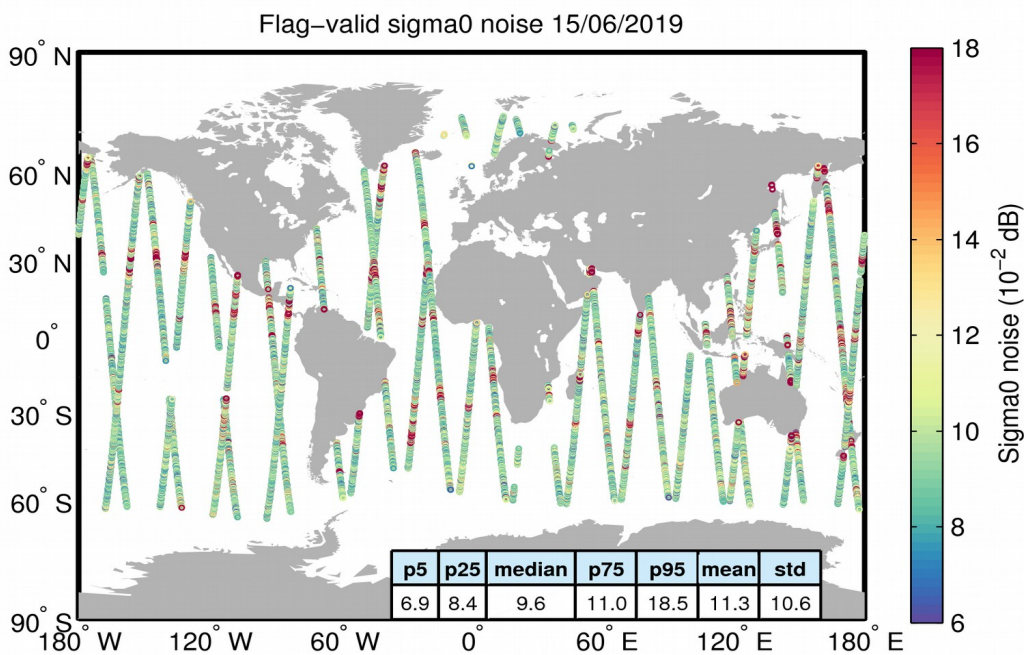
Figure 26. Geographical distribution of flag-valid 20-Hz sigma0 measurement noise over oceans and lakes for 15/06/2019. The statistical values shown in the table refer to the sigma0 noise and are calculated over all measurements shown in the figure.
