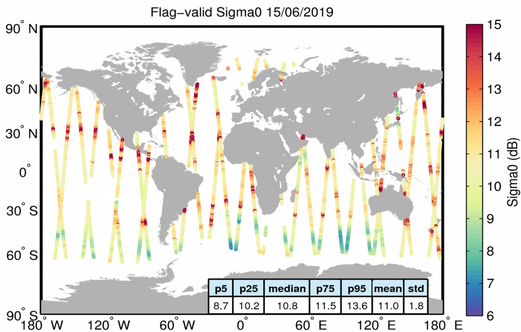
Figure 23. Geographical distribution of flag-valid sigma0 data over oceans and lakes for 15/06/2019. The statistical values shown in the table refer to the sigma0 in dB and are calculated over all measurements shown in the figure.
