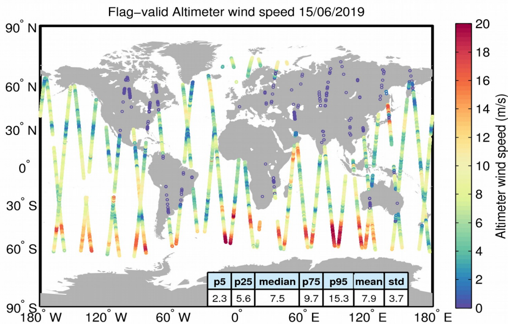
Figure 31. Geographical distribution of flag-valid wind data over oceans and lakes for 15/06/2019. The statistical values shown in the table refer to the wind in m/s and are calculated over all measurements shown in the figure.
