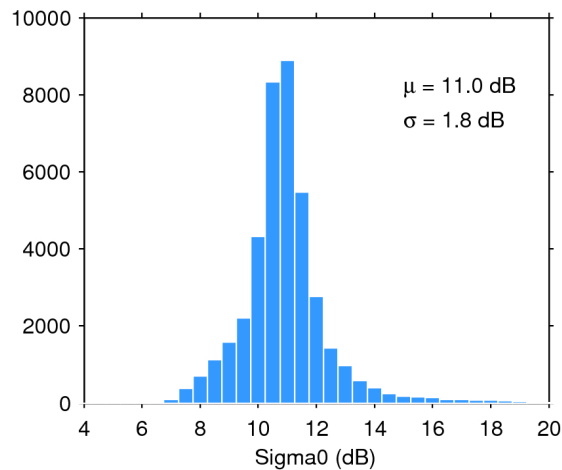
Figure 25. Histogram of flag-valid sigma0 over oceans and lakes for 15/06/2019. The mean ( \mu ) and standard deviation ( \sigma ) are also shown. Note that values outside [4 20] dB are excluded from the histogram for the sake of readability but not from the computation of \mu and \sigma .
