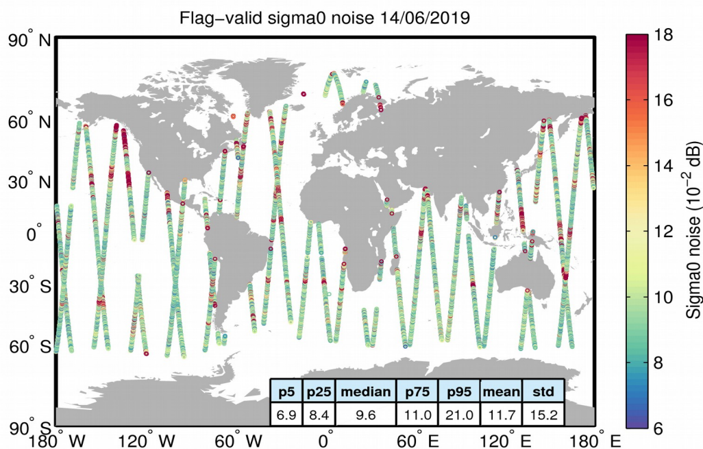
Figure 26. Geographical distribution of flag-valid 20-Hz sigma0 measurement noise over oceans and lakes for 14/06/2019. The statistical values shown in the table refer to the sigma0 noise and are calculated over all measurements shown in the figure.
