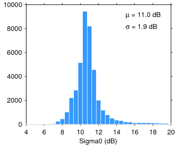
Figure 25. Histogram of flag-valid sigma0 over oceans and lakes for 14/06/2019. The mean ( \mu ) and standard deviation ( \sigma ) are also shown. Note that values outside [4 20] dB are excluded from the histogram for the sake of readability but not from the computation of \mu and \sigma .
