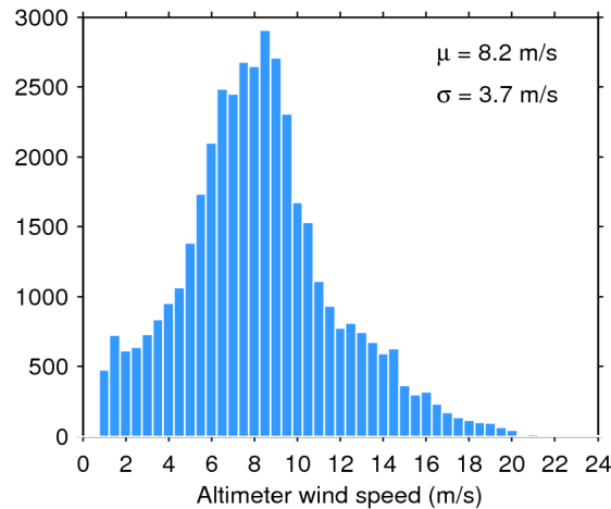
Figure 33. Histogram of flag-valid wind over oceans and lakes for 14/06/2019. The mean ( \mu ) and standard deviation ( \sigma ) are also shown. Note that values larger than 24 m/s are excluded from the histogram for the sake of readability but not from the computation of \mu and \sigma .
