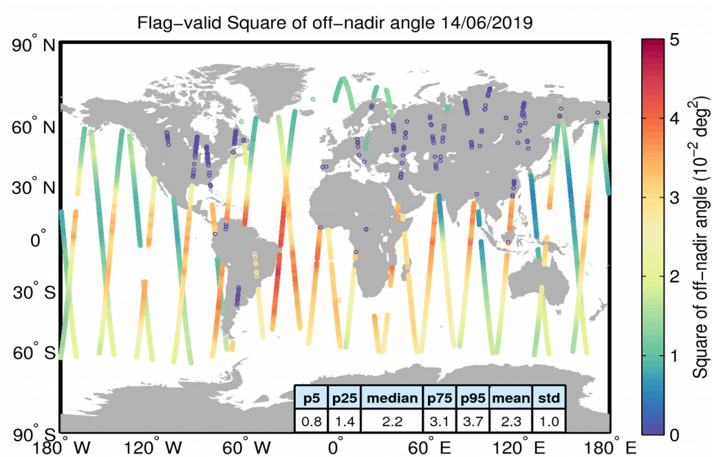
Figure 37. Geographical distribution of flag-valid mispointing data over oceans and lakes for 14/06/2019. The statistical values shown in the table refer to the mispointing in 10^{-2} deg 2 and are calculated over all measurements shown in the figure.
