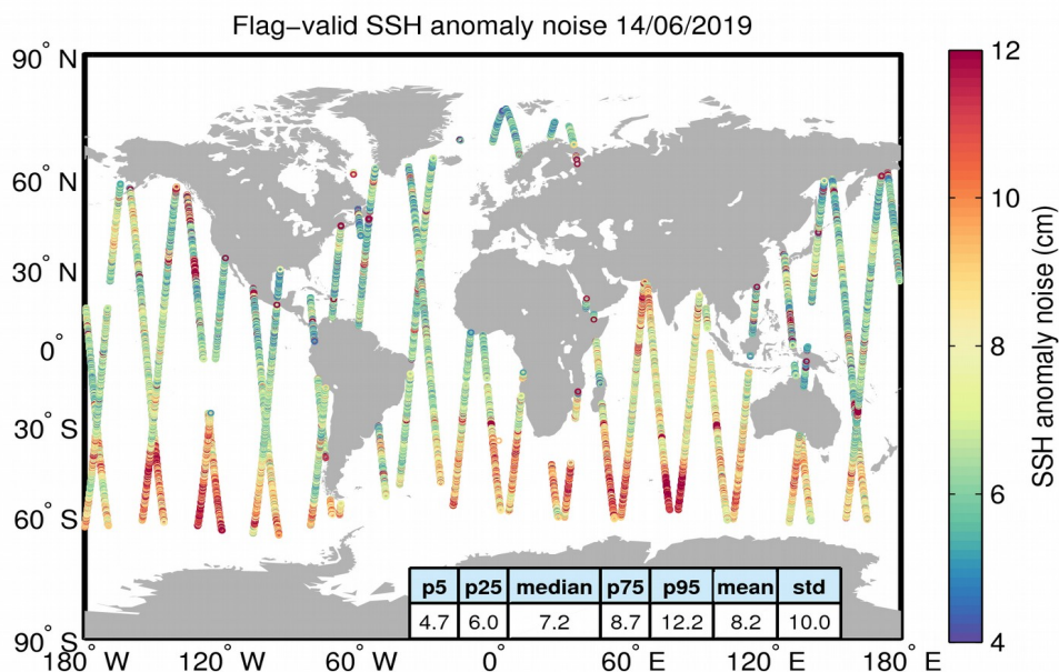
Figure 8. Geographical distribution of flag-valid 20-Hz SSH anomaly measurement noise over oceans and lakes for 14/06/2019. The statistical values shown in the table refer to the SSH anomaly noise and are calculated over all measurements shown in the figure.
