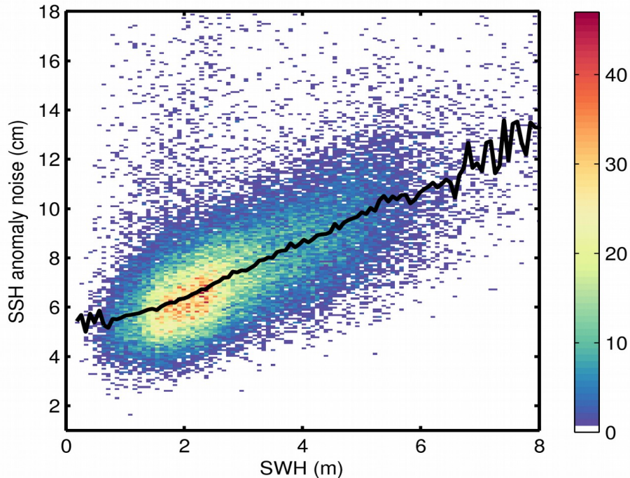
Figure 9. 2D histogram showing flag-valid SSH anomaly noise as a function of SWH for 14/06/2019. The black line denotes the median SSH anomaly noise as a function of SWH.
