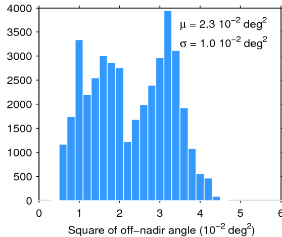
Figure 39. Histogram of flag-valid mispointing over oceans and lakes for 14/06/2019. The mean ( \mu ) and standard deviation ( \sigma ) are also shown. Note that values larger than 6 \cdot 10^{-2} \text{ deg}^2 are excluded from the histogram for the sake of readability but not from the computation of \mu and \sigma .
