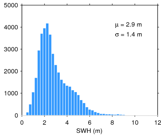
Figure 17. Histogram of flag-valid SWH over oceans and lakes for 14/06/2019. The mean ( \mu ) and standard deviation ( \sigma ) are also shown. Note that values larger than 12 m are excluded from the histogram for the sake of readability but not from the computation of \mu and \sigma .
