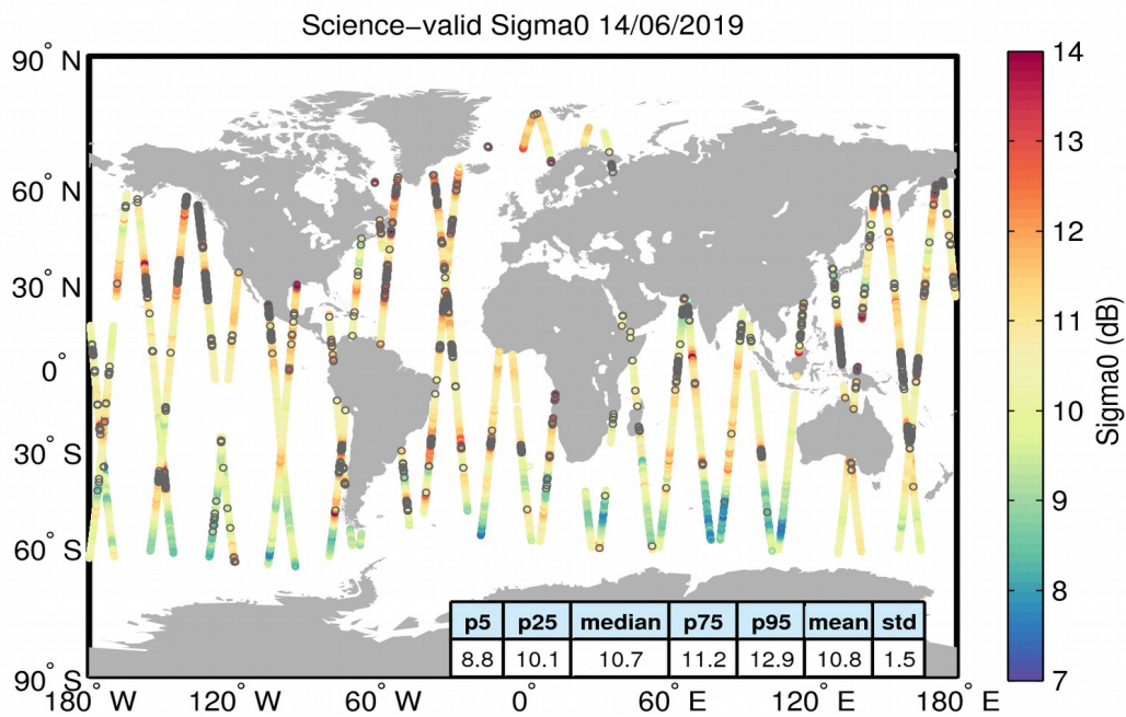
Figure 27. Geographical distribution of science-valid sigma0 data over oceans and lakes for 14/06/2019. The statistical values shown in the table refer to the sigma0 in dB and are calculated over all measurements shown in the figure. Gray circles denote records that have been rejected based on the editing criteria described in Table 4.
