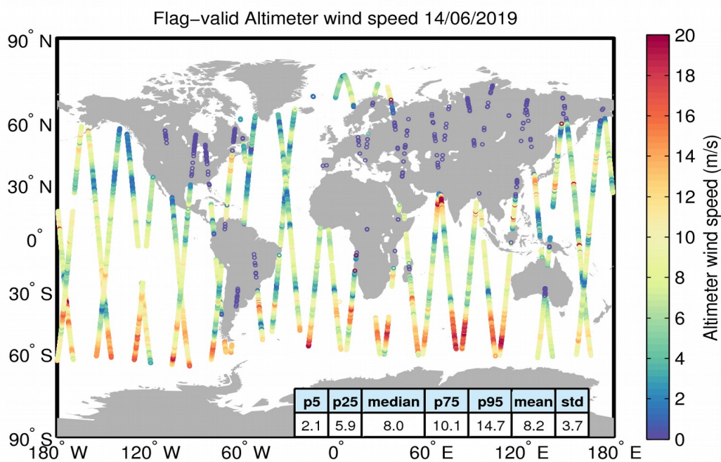
Figure 31. Geographical distribution of flag-valid wind data over oceans and lakes for 14/06/2019. The statistical values shown in the table refer to the wind in m/s and are calculated over all measurements shown in the figure.
