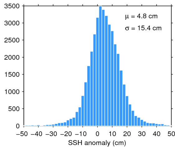
Figure 7. Histogram of flag-valid SSH anomaly over oceans and lakes for 14/06/2019. The mean ( \mu ) and standard deviation ( \sigma ) are also shown. Note that values outside [-50\ 50] cm are excluded from the histogram for the sake of readability but not from the computation of \mu and \sigma .
