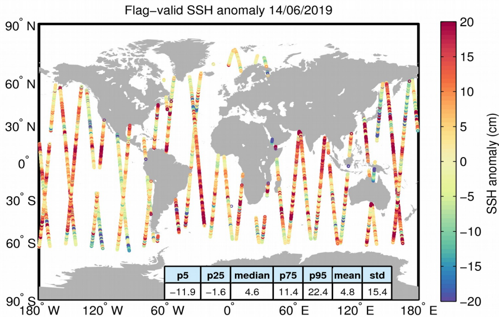
Figure 5. Geographical distribution of flag-valid 1-Hz SSH anomaly data over oceans and lakes for 14/06/2019. The statistical values shown in the table refer to the SSH anomaly in cm and are calculated over all measurements shown in the figure.
