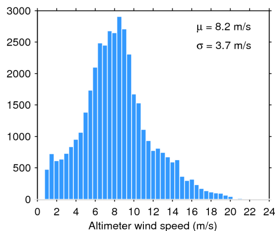
Figure 35. Histogram of science-valid wind over oceans and lakes for 14/06/2019. The mean ( \mu ) and standard deviation ( \sigma ) are also shown. Note that values larger than 24 m/s are excluded from the histogram for the sake of readability but not from the computation of \mu and \sigma .
