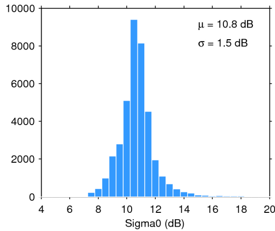
Figure 28. Histogram of science-valid sigma0 over oceans and lakes for 14/06/2019. The mean ( \mu ) and standard deviation ( \sigma ) are also shown. Note that values outside [4 20] dB are excluded from the histogram for the sake of readability but not from the computation of \mu and \sigma .
