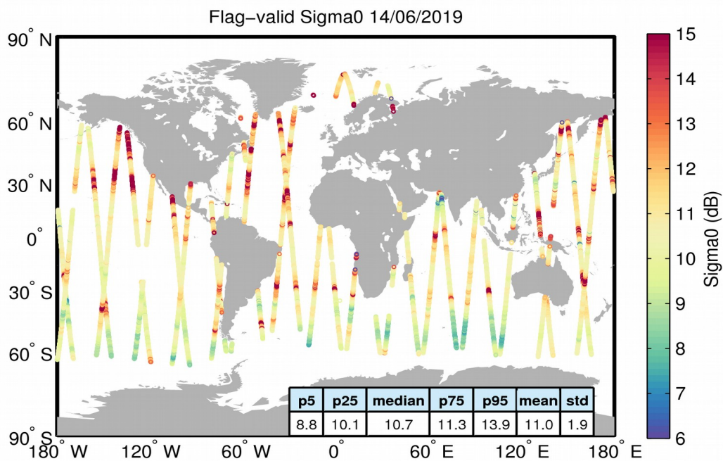
Figure 23. Geographical distribution of flag-valid sigma0 data over oceans and lakes for 14/06/2019. The statistical values shown in the table refer to the sigma0 in dB and are calculated over all measurements shown in the figure.
