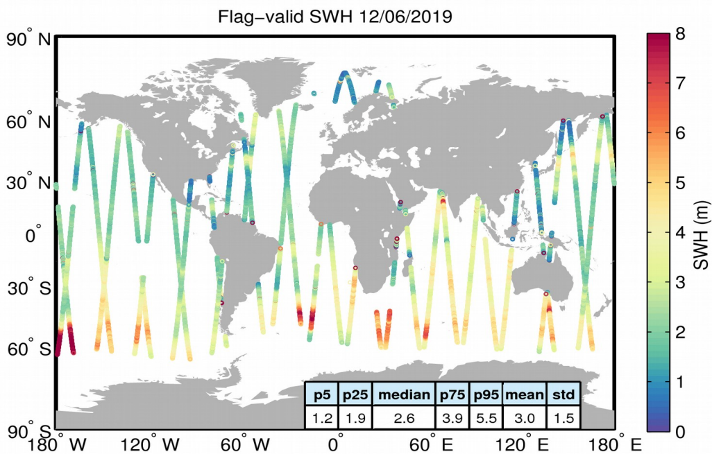
Figure 15. Geographical distribution of flag-valid SWH data over oceans and lakes for 12/06/2019. The statistical values shown in the table refer to the SWH in m and are calculated over all measurements shown in the figure.
