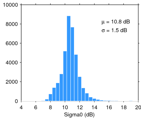
Figure 28. Histogram of science-valid sigma0 over oceans and lakes for 12/06/2019. The mean ( \mu ) and standard deviation ( \sigma ) are also shown. Note that values outside [4 20] dB are excluded from the histogram for the sake of readability but not from the computation of \mu and \sigma .
