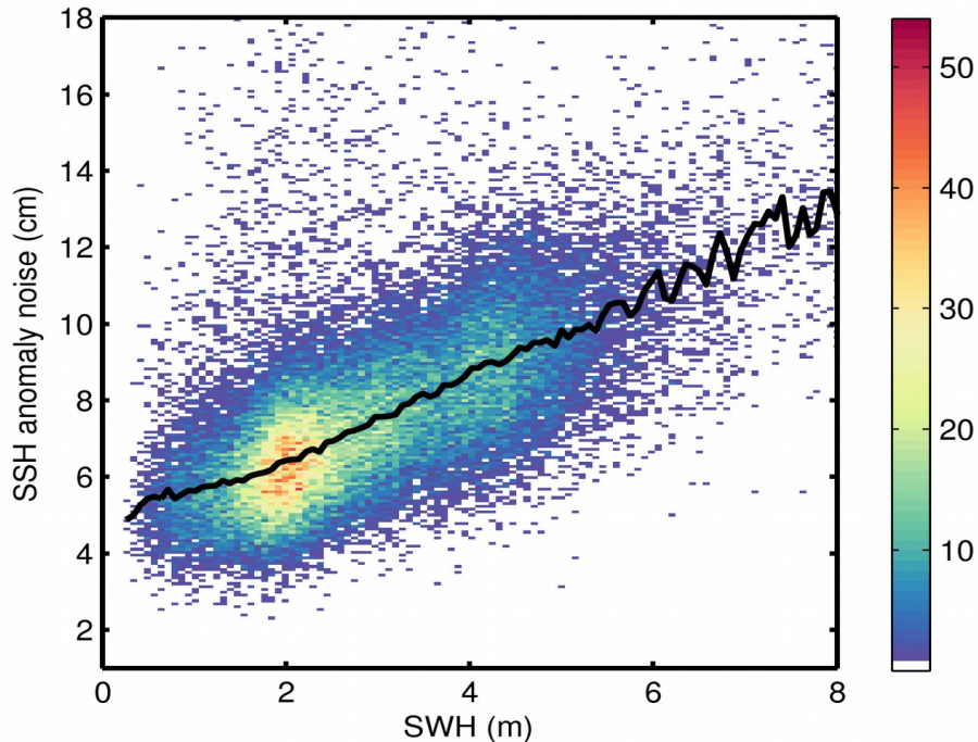
Figure 9. 2D histogram showing flag-valid SSH anomaly noise as a function of SWH for 12/06/2019. The black line denotes the median SSH anomaly noise as a function of SWH.
