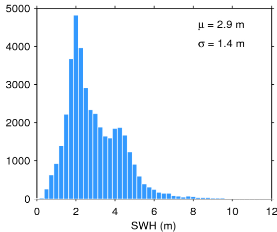
Figure 20. Histogram of science-valid SWH over oceans and lakes for 12/06/2019. The mean ( \mu ) and standard deviation ( \sigma ) are also shown. Note that values larger than 12 m are excluded from the histogram for the sake of readability but not from the computation of \mu and \sigma .
