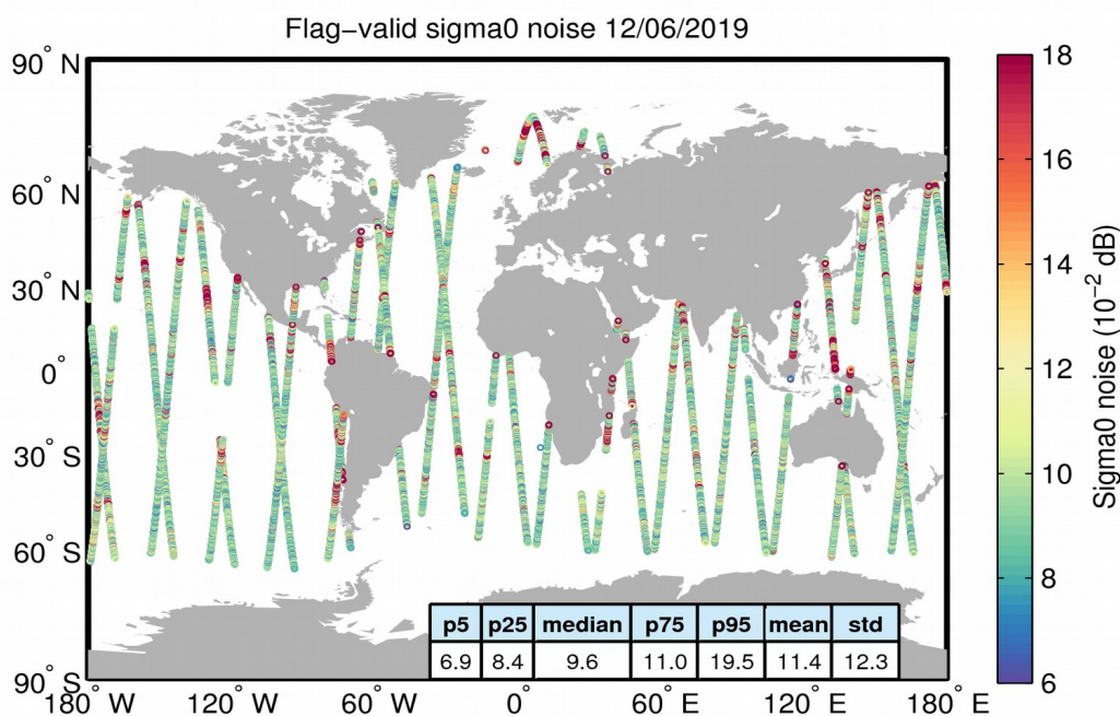
Figure 26. Geographical distribution of flag-valid 20-Hz sigma0 measurement noise over oceans and lakes for 12/06/2019. The statistical values shown in the table refer to the sigma0 noise and are calculated over all measurements shown in the figure.
