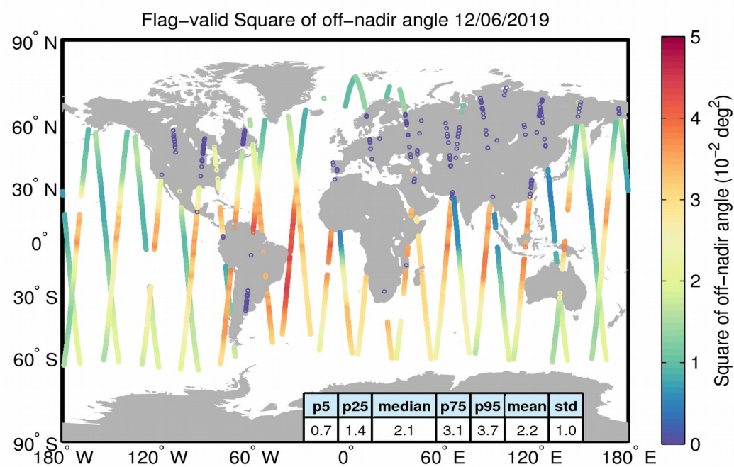
Figure 37. Geographical distribution of flag-valid mispointing data over oceans and lakes for 12/06/2019. The statistical values shown in the table refer to the mispointing in 10^{-2} \text{ deg}^2 and are calculated over all measurements shown in the figure.
