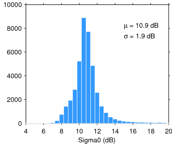
Figure 25. Histogram of flag-valid sigma0 over oceans and lakes for 12/06/2019. The mean ( \mu ) and standard deviation ( \sigma ) are also shown. Note that values outside [4 20] dB are excluded from the histogram for the sake of readability but not from the computation of \mu and \sigma .
