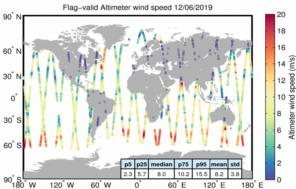
Figure 31. Geographical distribution of flag-valid wind data over oceans and lakes for 12/06/2019. The statistical values shown in the table refer to the wind in m/s and are calculated over all measurements shown in the figure.
