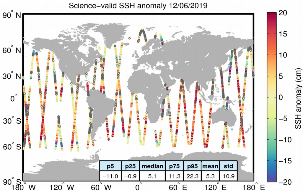
Figure 10. Geographical distribution of science-valid SSH anomaly data over oceans and lakes for 12/06/2019. The statistical values shown in the table refer to the SSH anomaly in cm and are calculated over all measurements shown in the figure. Gray circles denote records that have been rejected based on the editing criteria described in Table 2.
