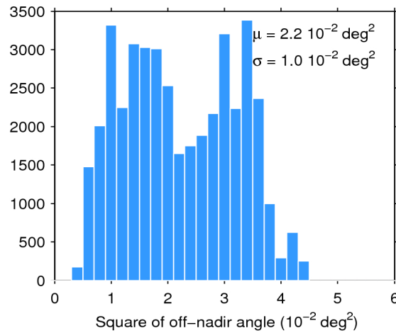
Figure 39. Histogram of flag-valid mispointing over oceans and lakes for 12/06/2019. The mean ( \mu ) and standard deviation ( \sigma ) are also shown. Note that values larger than 6 \cdot 10^{-2} \text{ deg}^2 are excluded from the histogram for the sake of readability but not from the computation of \mu and \sigma .
