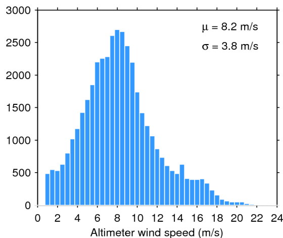
Figure 35. Histogram of science-valid wind over oceans and lakes for 12/06/2019. The mean ( \mu ) and standard deviation ( \sigma ) are also shown. Note that values larger than 24 m/s are excluded from the histogram for the sake of readability but not from the computation of \mu and \sigma .
