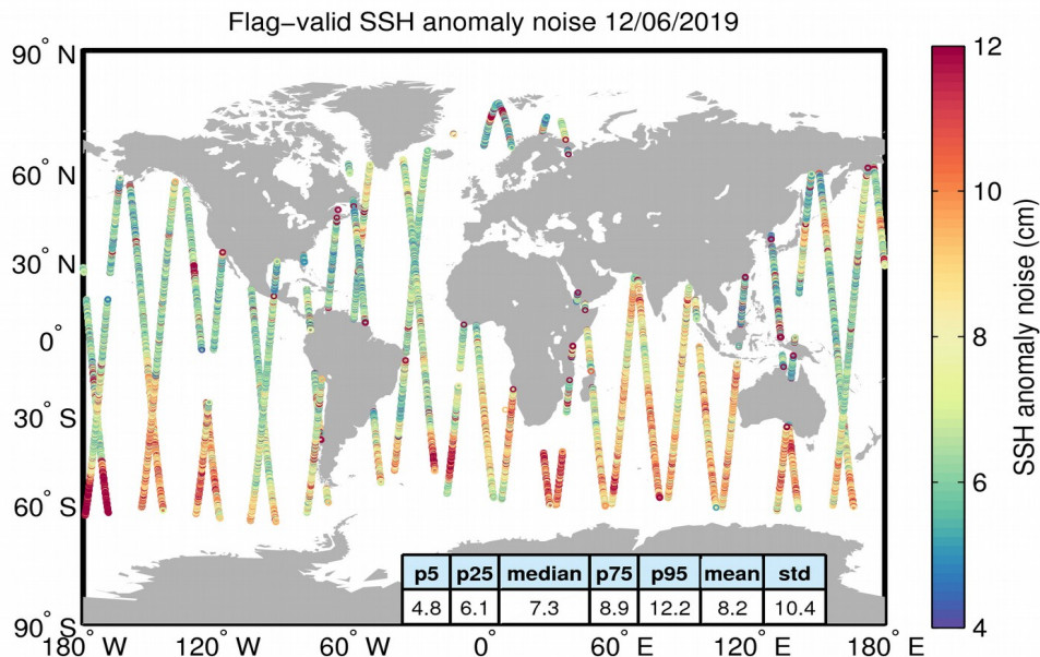
Figure 8. Geographical distribution of flag-valid 20-Hz SSH anomaly measurement noise over oceans and lakes for 12/06/2019. The statistical values shown in the table refer to the SSH anomaly noise and are calculated over all measurements shown in the figure.
