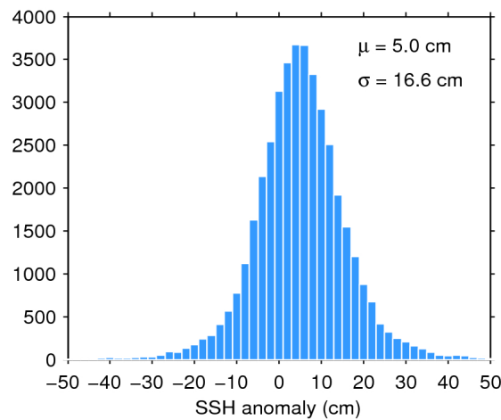
Figure 7. Histogram of flag-valid SSH anomaly over oceans and lakes for 12/06/2019. The mean ( \mu ) and standard deviation ( \sigma ) are also shown. Note that values outside [-50 50] cm are excluded from the histogram for the sake of readability but not from the computation of \mu and \sigma .
