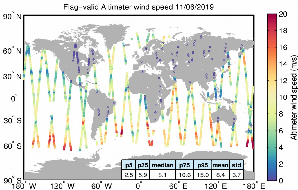
Figure 31. Geographical distribution of flag-valid wind data over oceans and lakes for 11/06/2019. The statistical values shown in the table refer to the wind in m/s and are calculated over all measurements shown in the figure.
