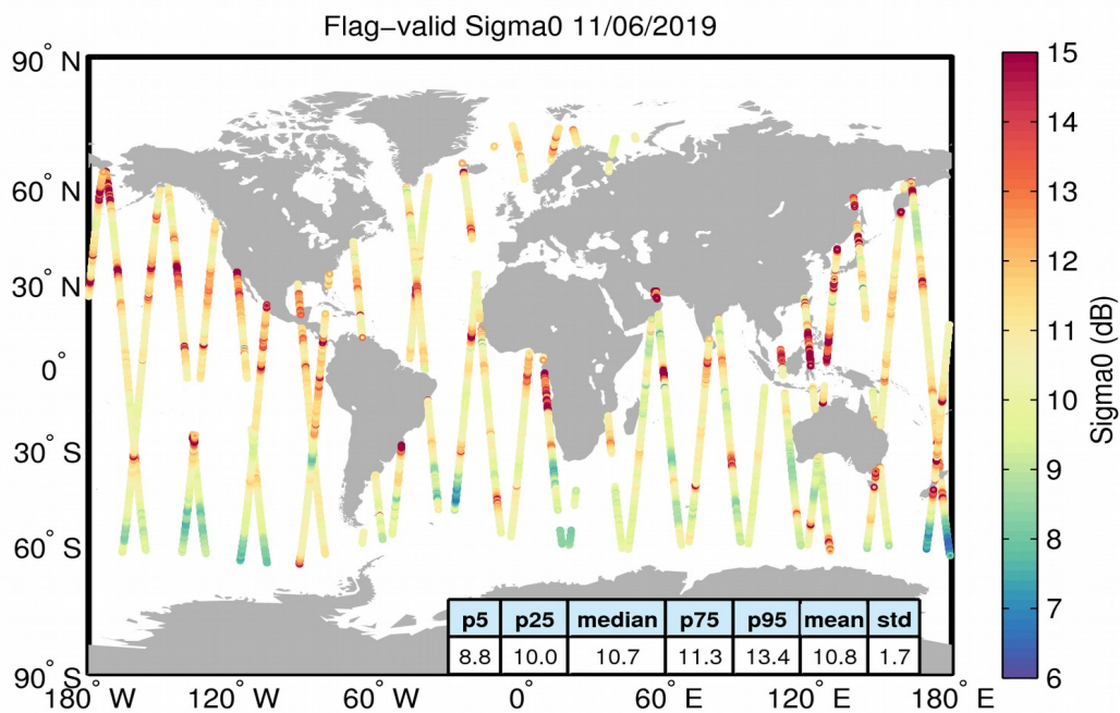
Figure 23. Geographical distribution of flag-valid sigma0 data over oceans and lakes for 11/06/2019. The statistical values shown in the table refer to the sigma0 in dB and are calculated over all measurements shown in the figure.
