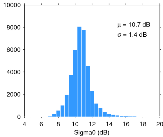
Figure 28. Histogram of science-valid sigma0 over oceans and lakes for 11/06/2019. The mean ( \mu ) and standard deviation ( \sigma ) are also shown. Note that values outside [4 20] dB are excluded from the histogram for the sake of readability but not from the computation of \mu and \sigma .
