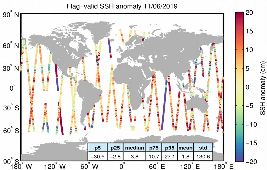
Figure 5. Geographical distribution of flag-valid 1-Hz SSH anomaly data over oceans and lakes for 11/06/2019. The statistical values shown in the table refer to the SSH anomaly in cm and are calculated over all measurements shown in the figure.
