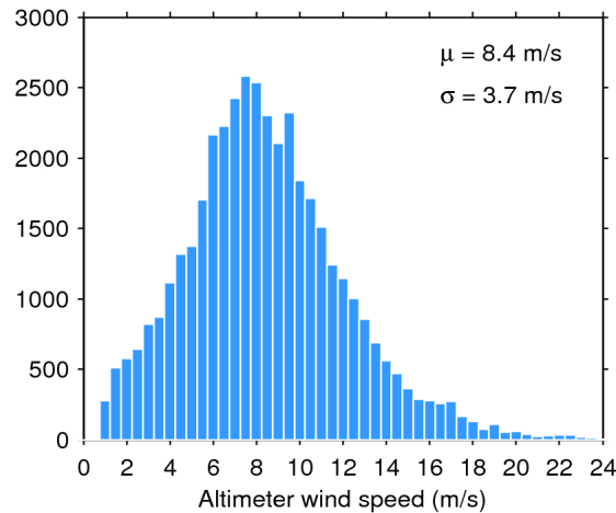
Figure 33. Histogram of flag-valid wind over oceans and lakes for 11/06/2019. The mean ( \mu ) and standard deviation ( \sigma ) are also shown. Note that values larger than 24 m/s are excluded from the histogram for the sake of readability but not from the computation of \mu and \sigma .
