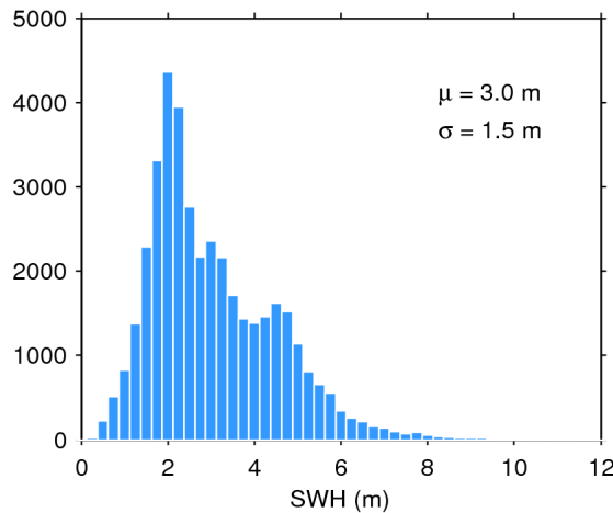
Figure 20. Histogram of science-valid SWH over oceans and lakes for 11/06/2019. The mean ( \mu ) and standard deviation ( \sigma ) are also shown. Note that values larger than 12 m are excluded from the histogram for the sake of readability but not from the computation of \mu and \sigma .
