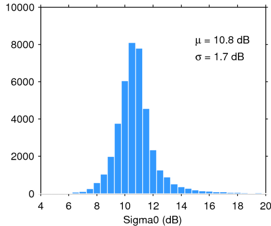
Figure 25. Histogram of flag-valid sigma0 over oceans and lakes for 11/06/2019. The mean ( \mu ) and standard deviation ( \sigma ) are also shown. Note that values outside [4 20] dB are excluded from the histogram for the sake of readability but not from the computation of \mu and \sigma .
