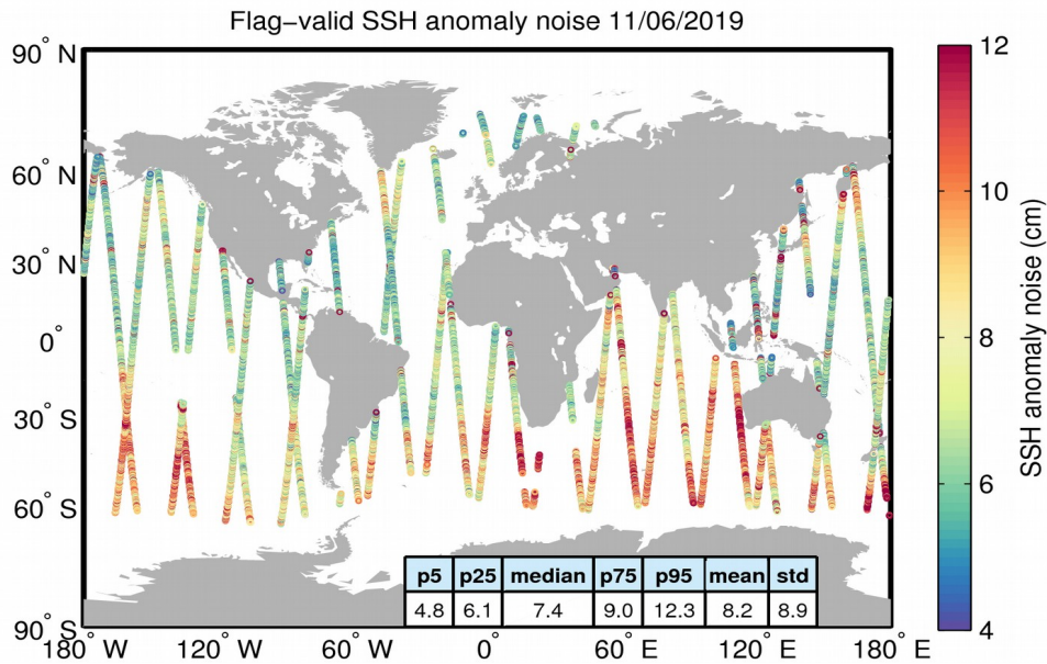
Figure 8. Geographical distribution of flag-valid 20-Hz SSH anomaly measurement noise over oceans and lakes for 11/06/2019. The statistical values shown in the table refer to the SSH anomaly noise and are calculated over all measurements shown in the figure.
