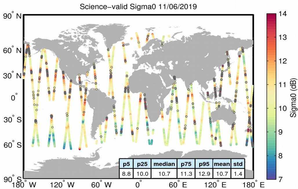
Figure 27. Geographical distribution of science-valid sigma0 data over oceans and lakes for 11/06/2019. The statistical values shown in the table refer to the sigma0 in dB and are calculated over all measurements shown in the figure. Gray circles denote records that have been rejected based on the editing criteria described in Table 4.
