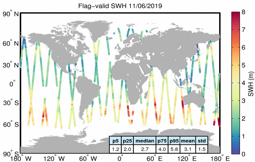
Figure 15. Geographical distribution of flag-valid SWH data over oceans and lakes for 11/06/2019. The statistical values shown in the table refer to the SWH in m and are calculated over all measurements shown in the figure.
