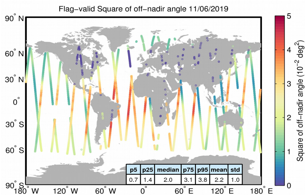
Figure 37. Geographical distribution of flag-valid mispointing data over oceans and lakes for 11/06/2019. The statistical values shown in the table refer to the mispointing in 10^{-2} \text{ deg}^2 and are calculated over all measurements shown in the figure.
