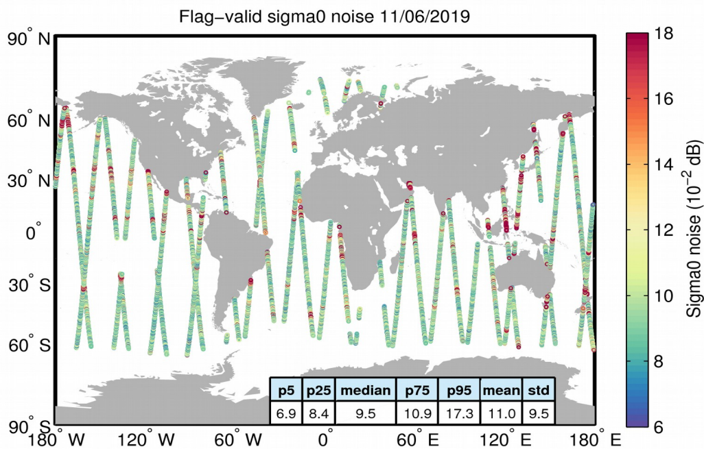
Figure 26. Geographical distribution of flag-valid 20-Hz sigma0 measurement noise over oceans and lakes for 11/06/2019. The statistical values shown in the table refer to the sigma0 noise and are calculated over all measurements shown in the figure.
