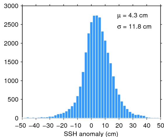
Figure 11. Histogram of science-valid SSH anomaly over oceans and lakes for 11/06/2019. The mean ( \mu ) and standard deviation ( \sigma ) are also shown. Note that values outside [-50 50] cm are excluded from the histogram for the sake of readability but not from the computation of \mu and \sigma .
