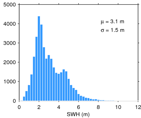
Figure 17. Histogram of flag-valid SWH over oceans and lakes for 11/06/2019. The mean ( \mu ) and standard deviation ( \sigma ) are also shown. Note that values larger than 12 m are excluded from the histogram for the sake of readability but not from the computation of \mu and \sigma .
