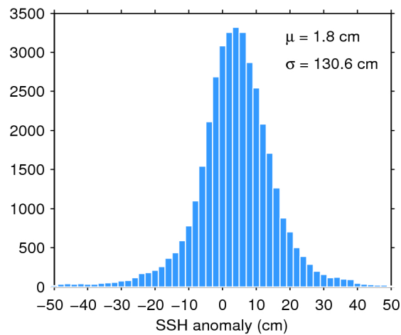
Figure 7. Histogram of flag-valid SSH anomaly over oceans and lakes for 11/06/2019. The mean ( \mu ) and standard deviation ( \sigma ) are also shown. Note that values outside [-50 50] cm are excluded from the histogram for the sake of readability but not from the computation of \mu and \sigma .
