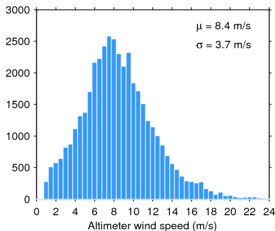
Figure 35. Histogram of science-valid wind over oceans and lakes for 11/06/2019. The mean ( \mu ) and standard deviation ( \sigma ) are also shown. Note that values larger than 24 m/s are excluded from the histogram for the sake of readability but not from the computation of \mu and \sigma .
