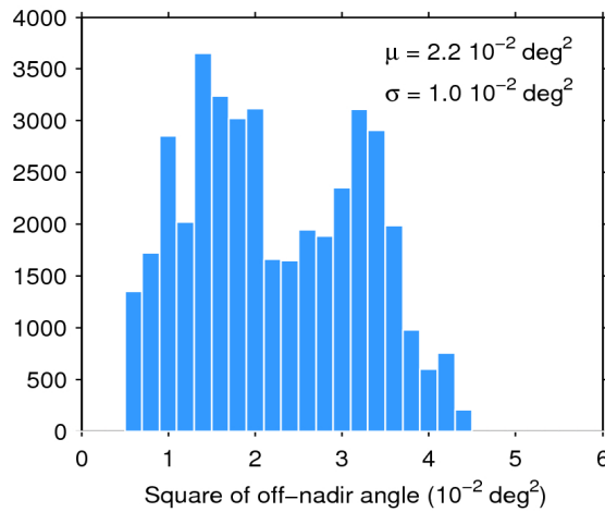
Figure 39. Histogram of flag-valid mispointing over oceans and lakes for 11/06/2019. The mean ( \mu ) and standard deviation ( \sigma ) are also shown. Note that values larger than 6 \cdot 10^{-2} \text{ deg}^2 are excluded from the histogram for the sake of readability but not from the computation of \mu and \sigma .
