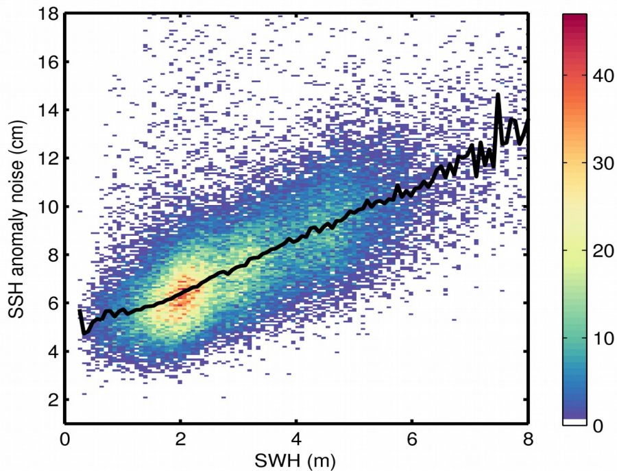
Figure 9. 2D histogram showing flag-valid SSH anomaly noise as a function of SWH for 11/06/2019. The black line denotes the median SSH anomaly noise as a function of SWH.
